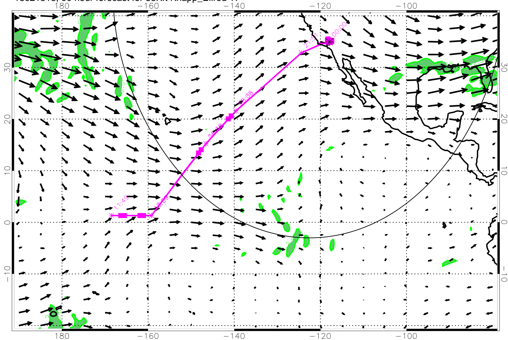
13021518, 90 hour forecast for 53Kft Knapp_Ellrod TI
