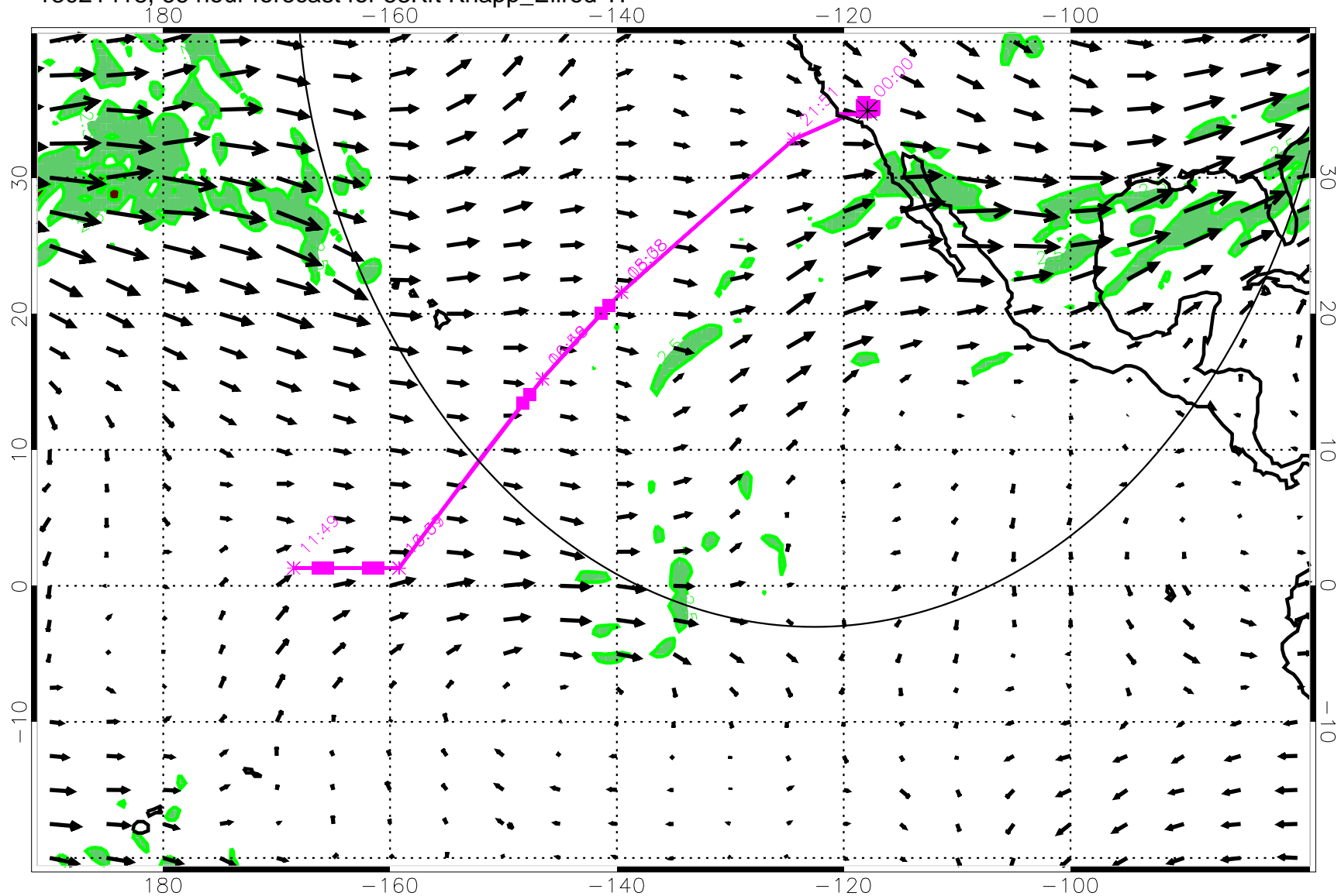
13021418, 66 hour forecast for 53Kft Knapp_Ellrod TI
