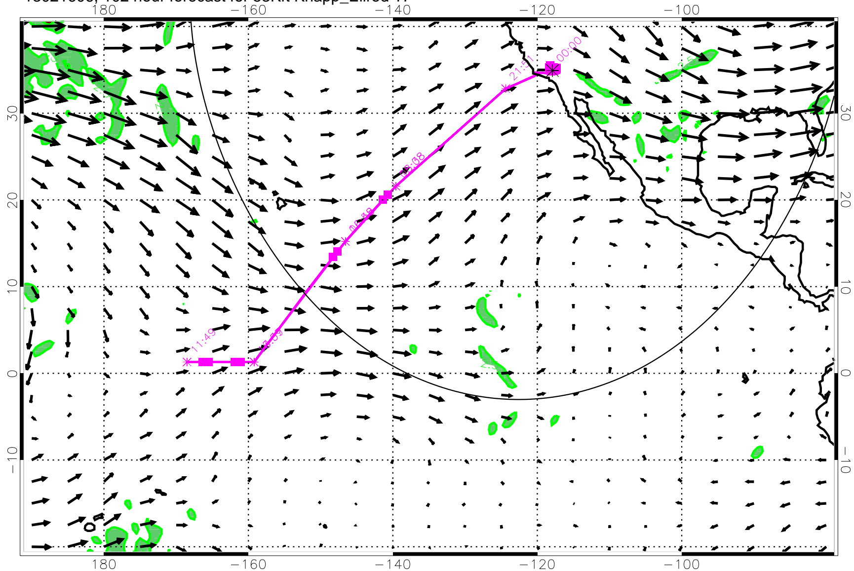
13021606, 102 hour forecast for 53Kft Knapp_Ellrod T1
