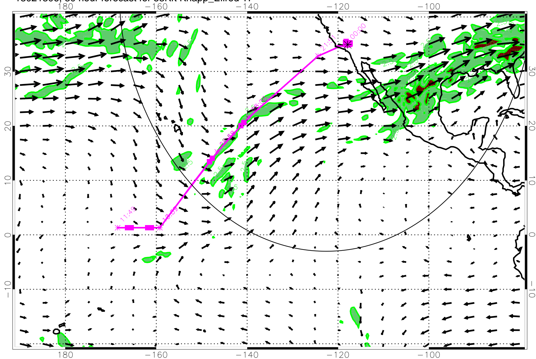
13021306, 30 hour forecast for 53Kft Knapp_Ellrod TI
