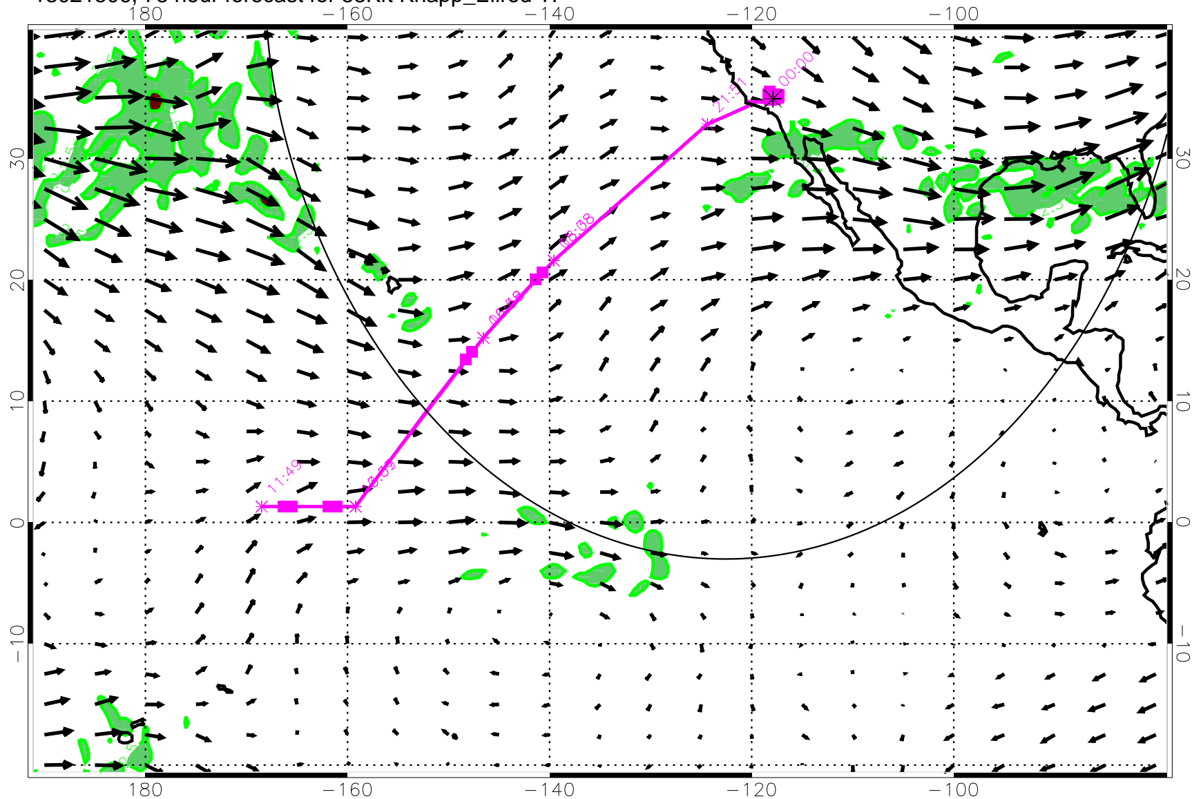
13021506, 78 hour forecast for 53Kft Knapp_Ellrod TI
