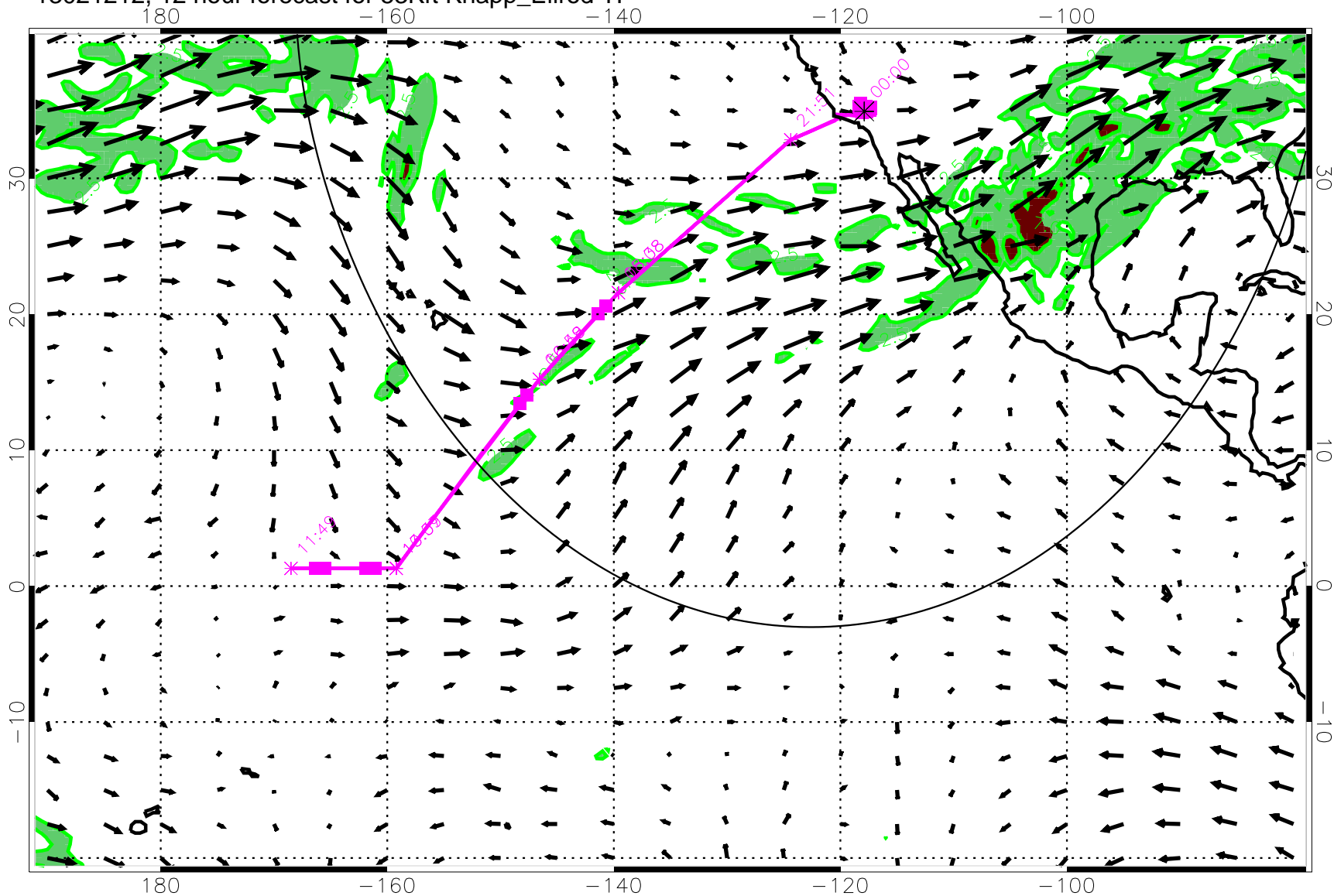
13021212, 12 hour forecast for 53Kft Knapp_Ellrod TI
