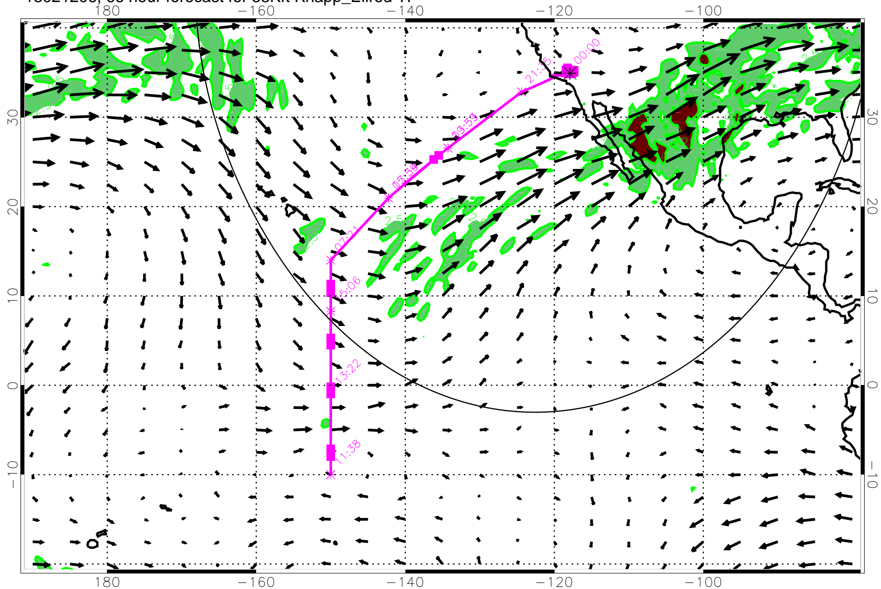
13021206, 66 hour forecast for 53Kft Knapp_Ellrod TI
