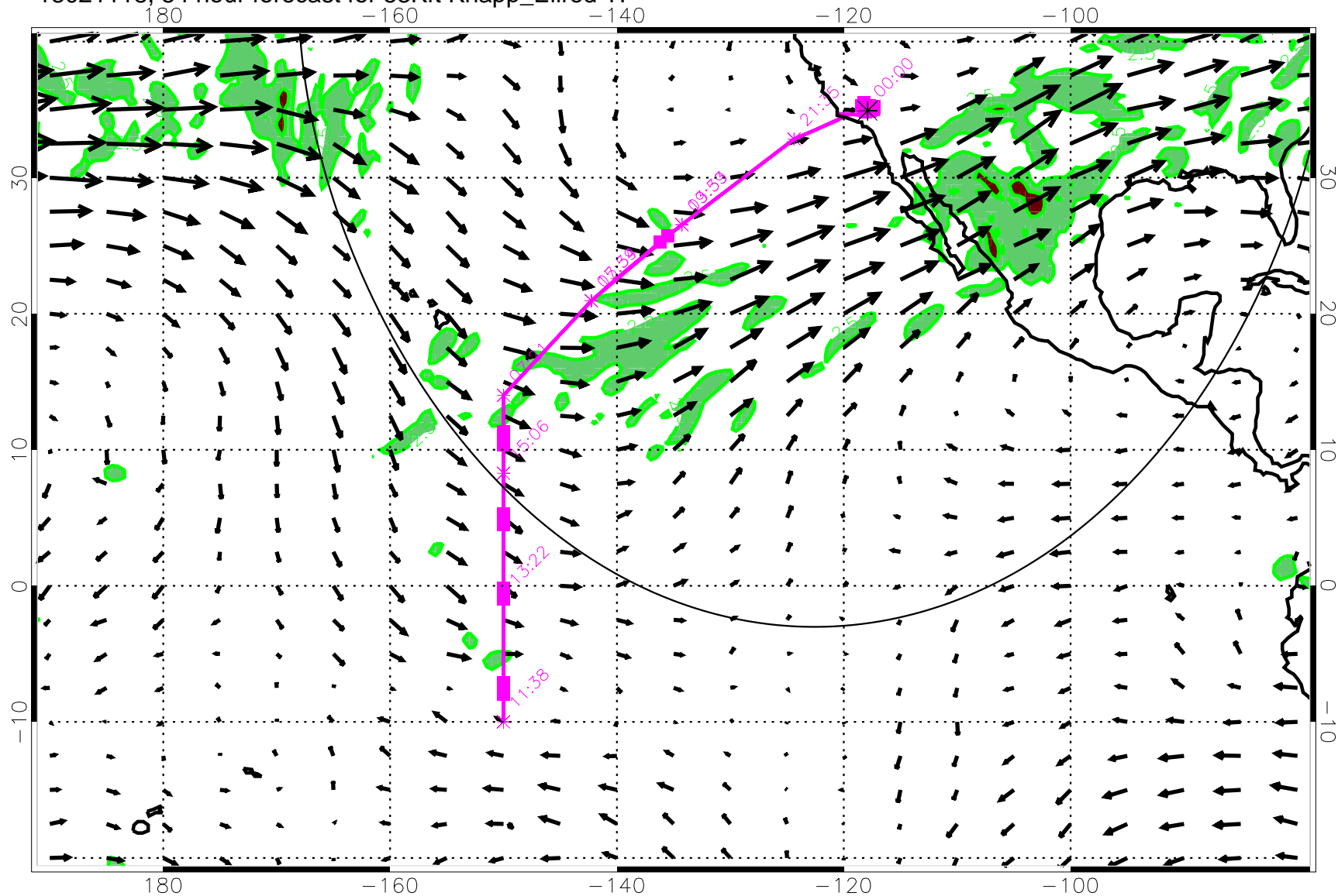
13021118, 54 hour forecast for 53Kft Knapp_Ellrod TI
