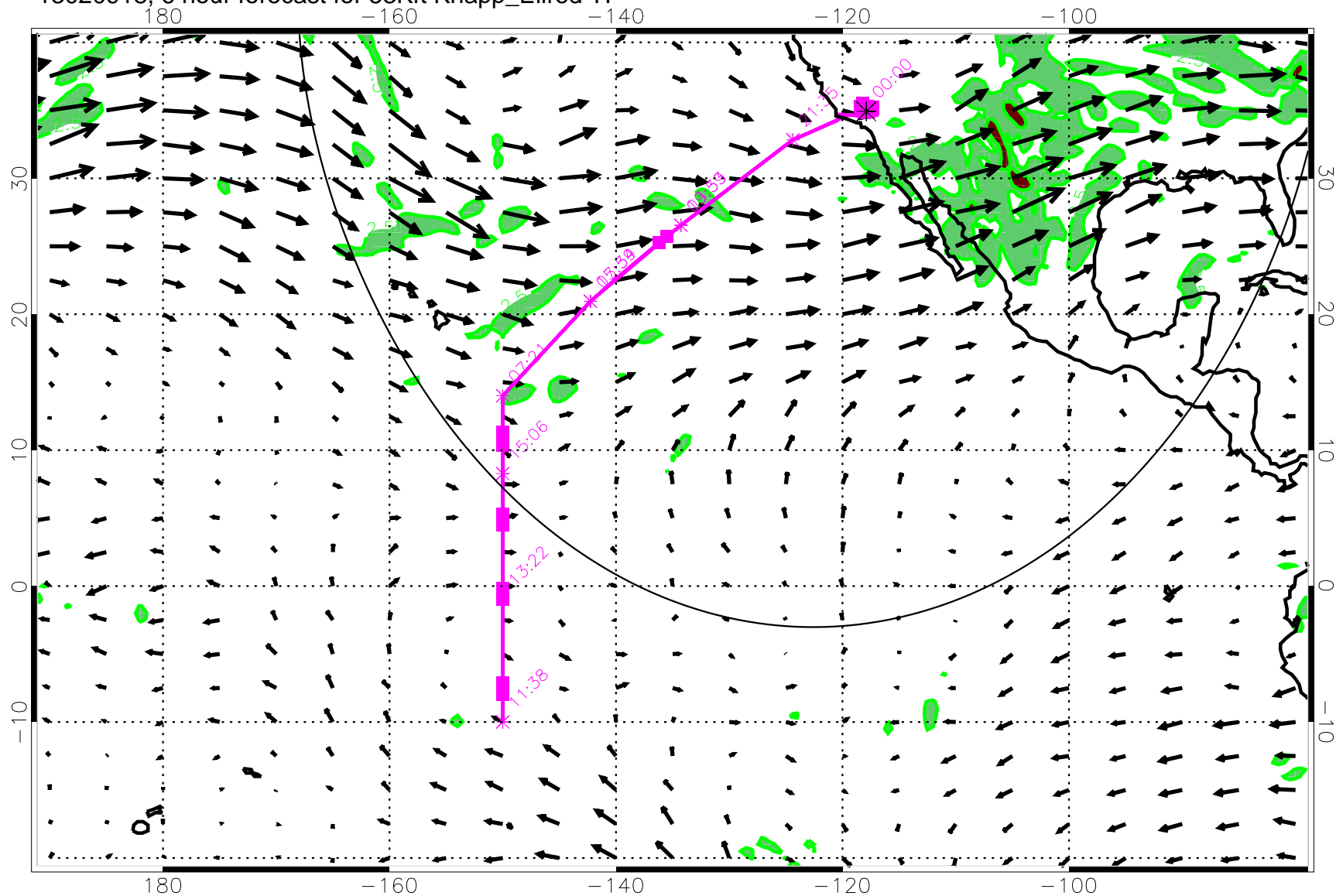
13020918, 6 hour forecast for 53Kft Knapp_Ellrod TI
