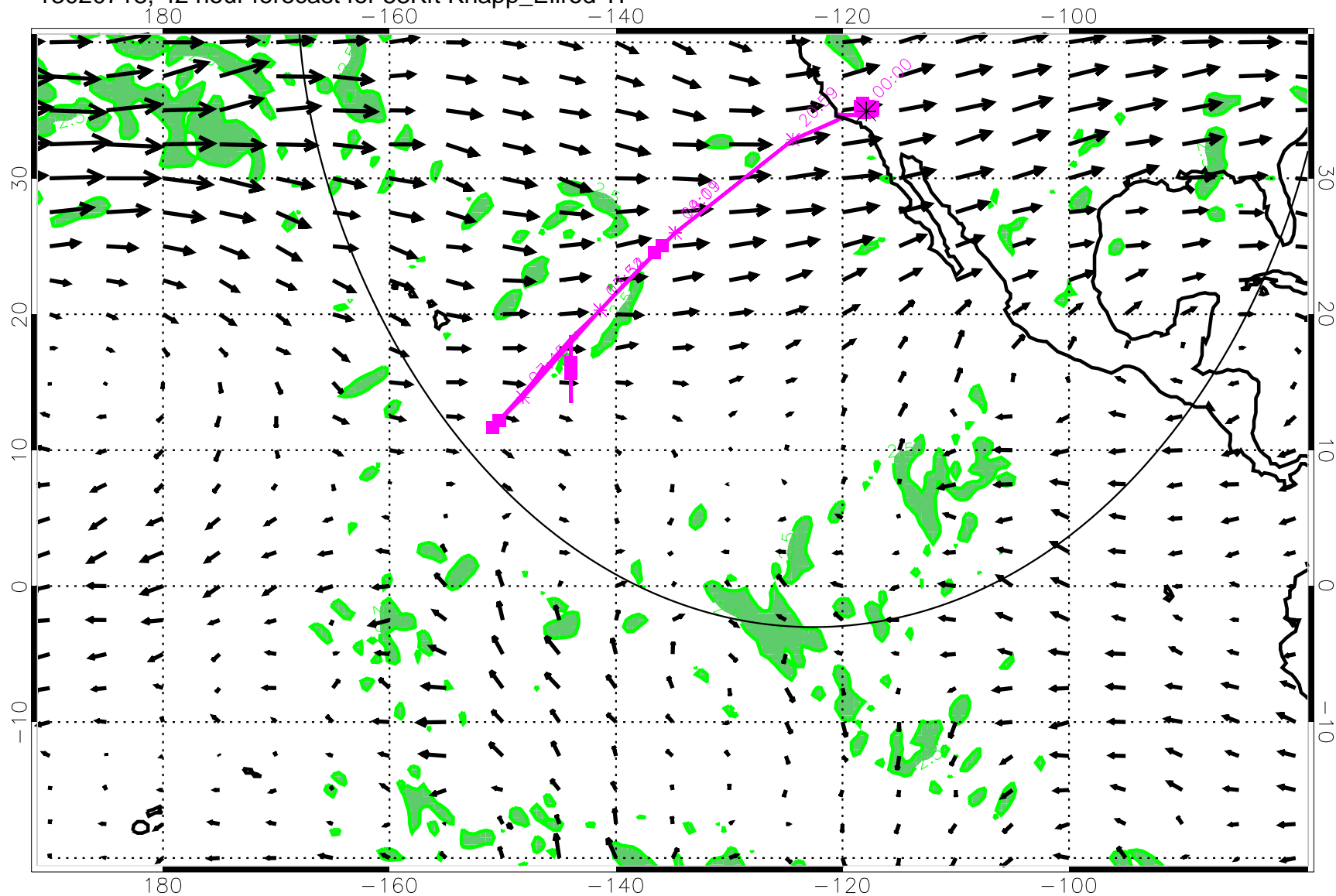
13020718, 42 hour forecast for 53Kft Knapp_Ellrod TI
