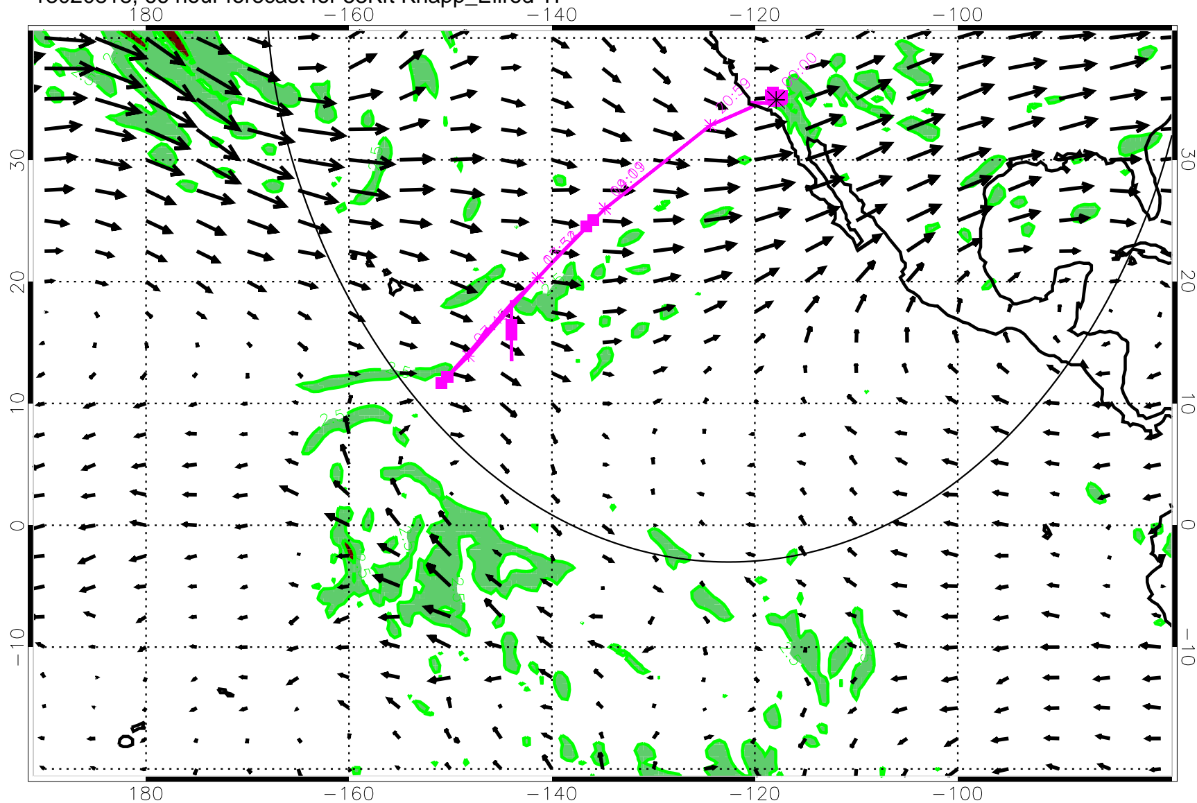
13020818, 66 hour forecast for 53Kft Knapp_Ellrod TI
