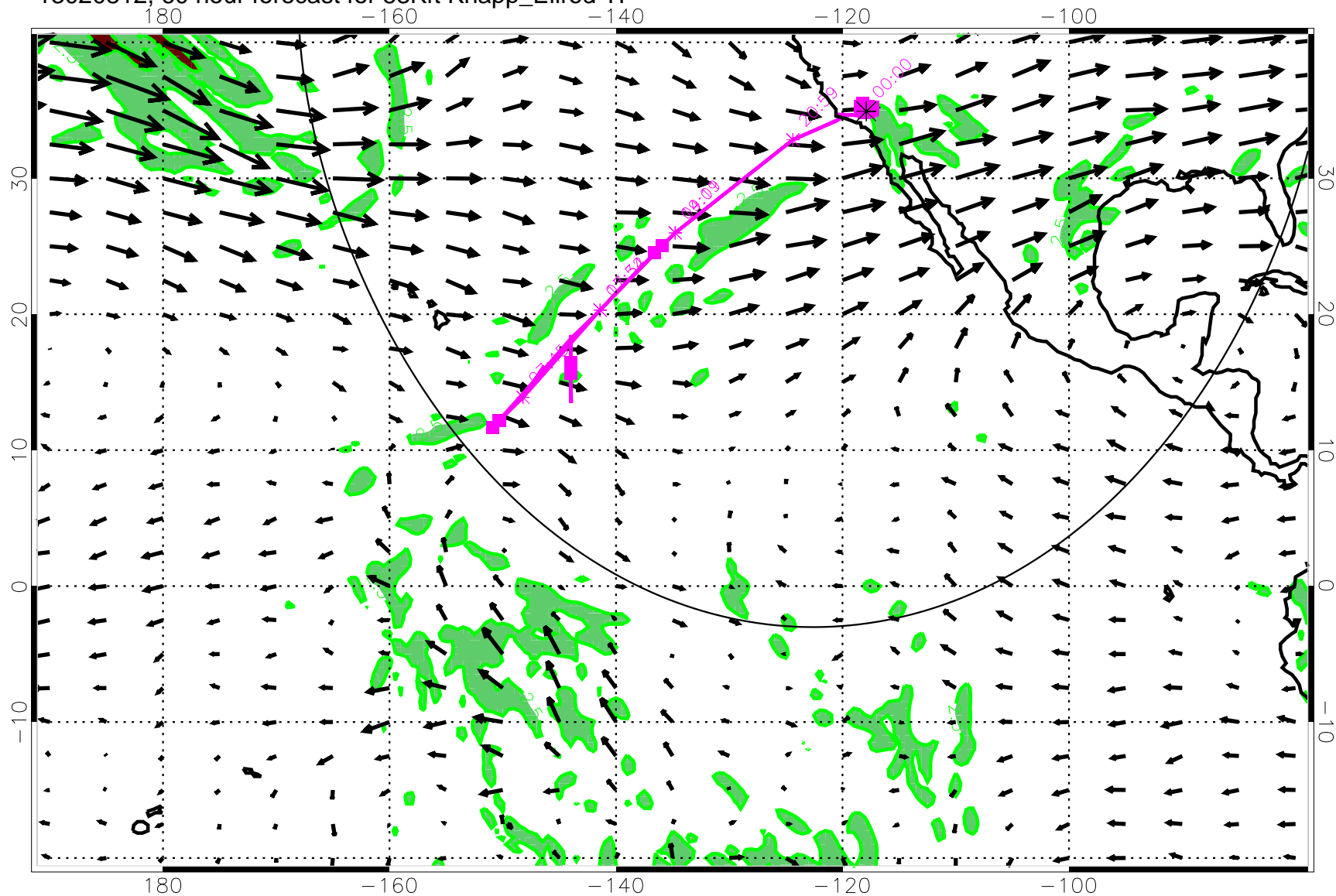
13020812, 60 hour forecast for 53Kft Knapp_Ellrod TI
