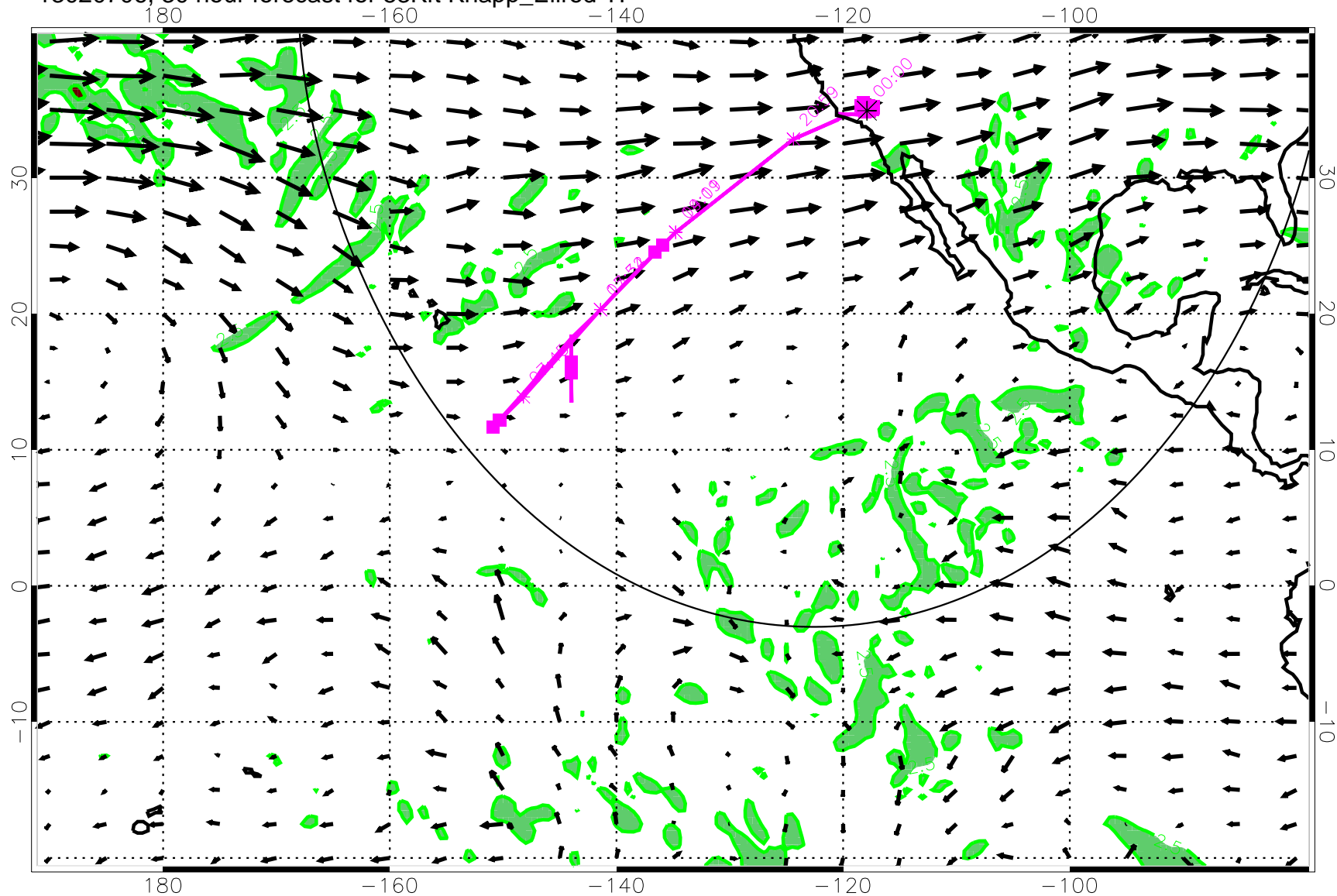
13020706, 30 hour forecast for 53Kft Knapp_Ellrod TI
