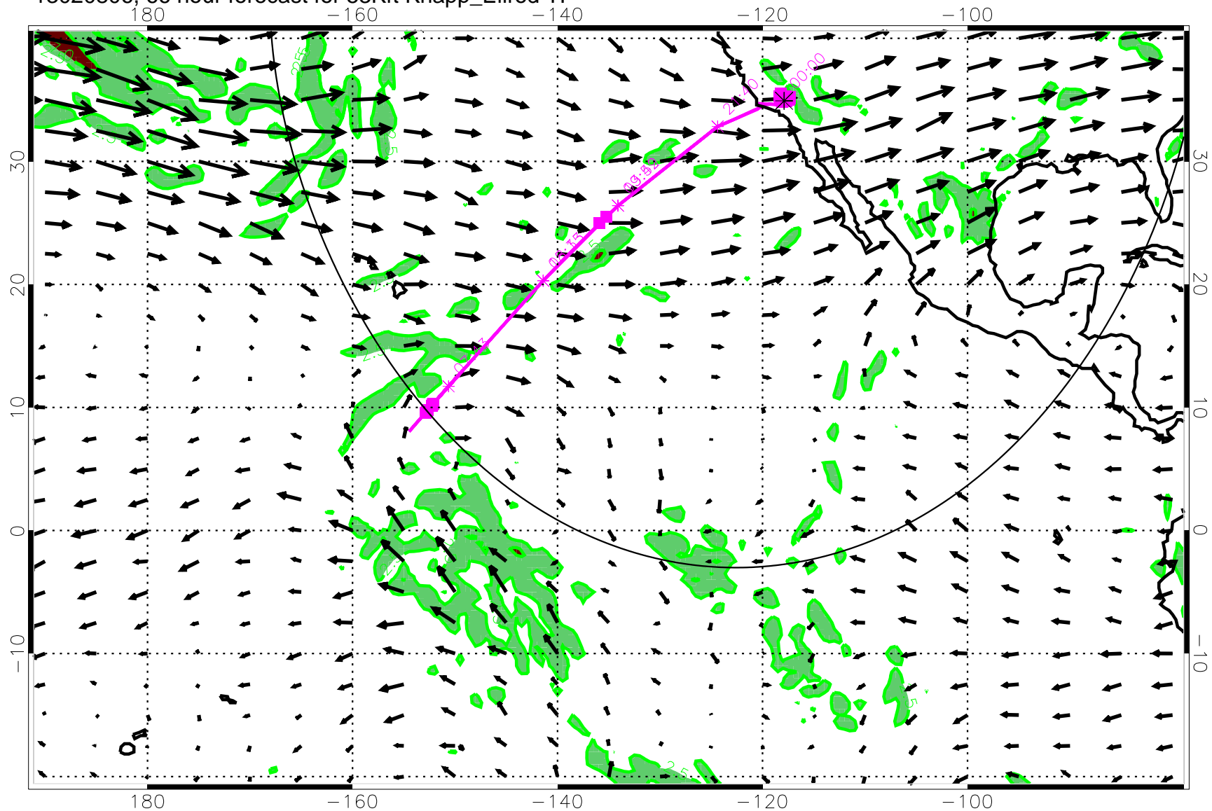
13020806, 66 hour forecast for 53Kft Knapp_Ellrod TI
