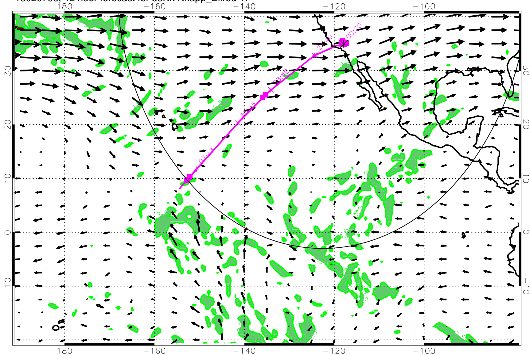
13020706, 42 hour forecast for 53Kft Knapp_Ellrod TI
