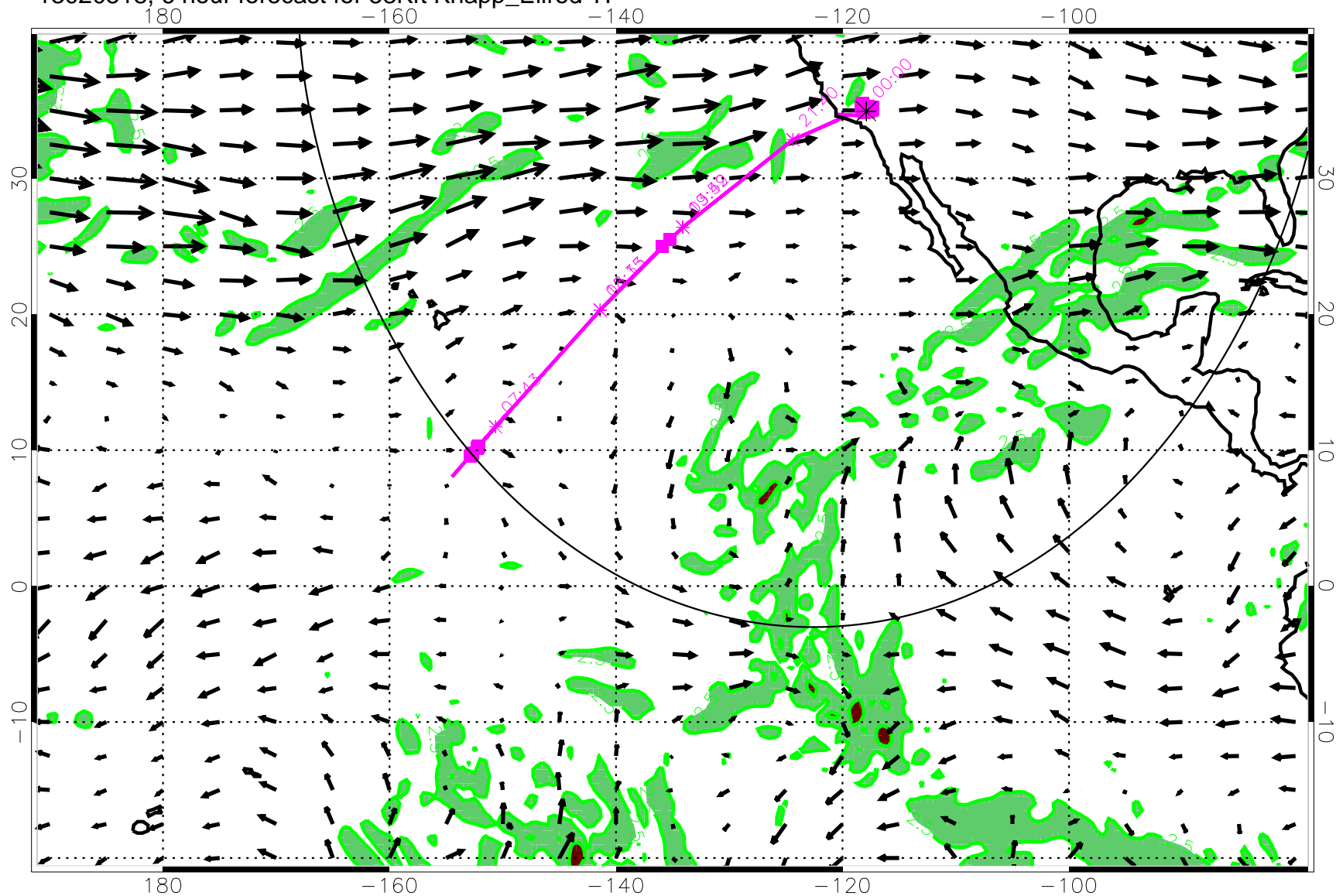
13020518, 6 hour forecast for 53Kft Knapp_Ellrod TI
