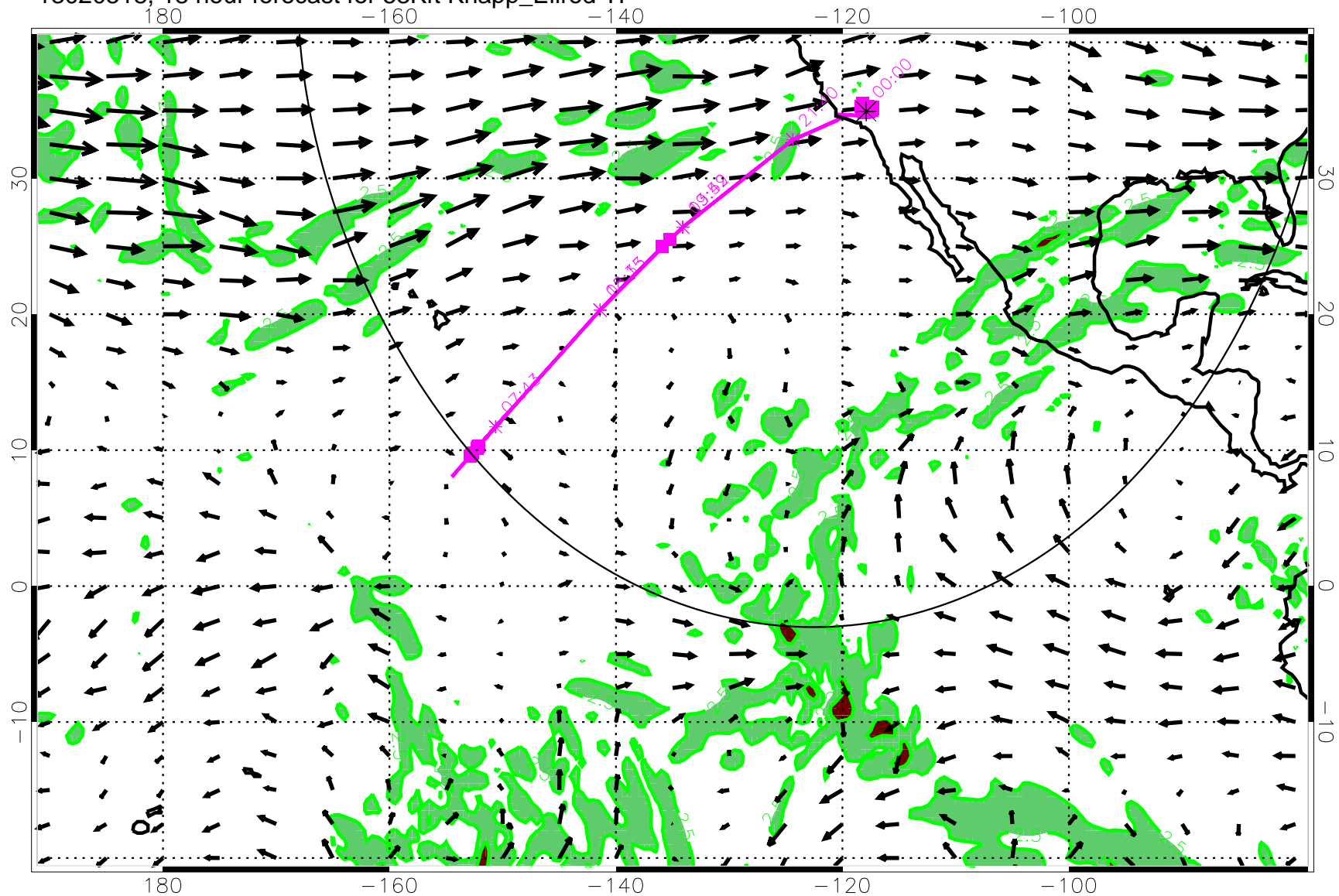
13020518, 18 hour forecast for 53Kft Knapp_Ellrod TI
