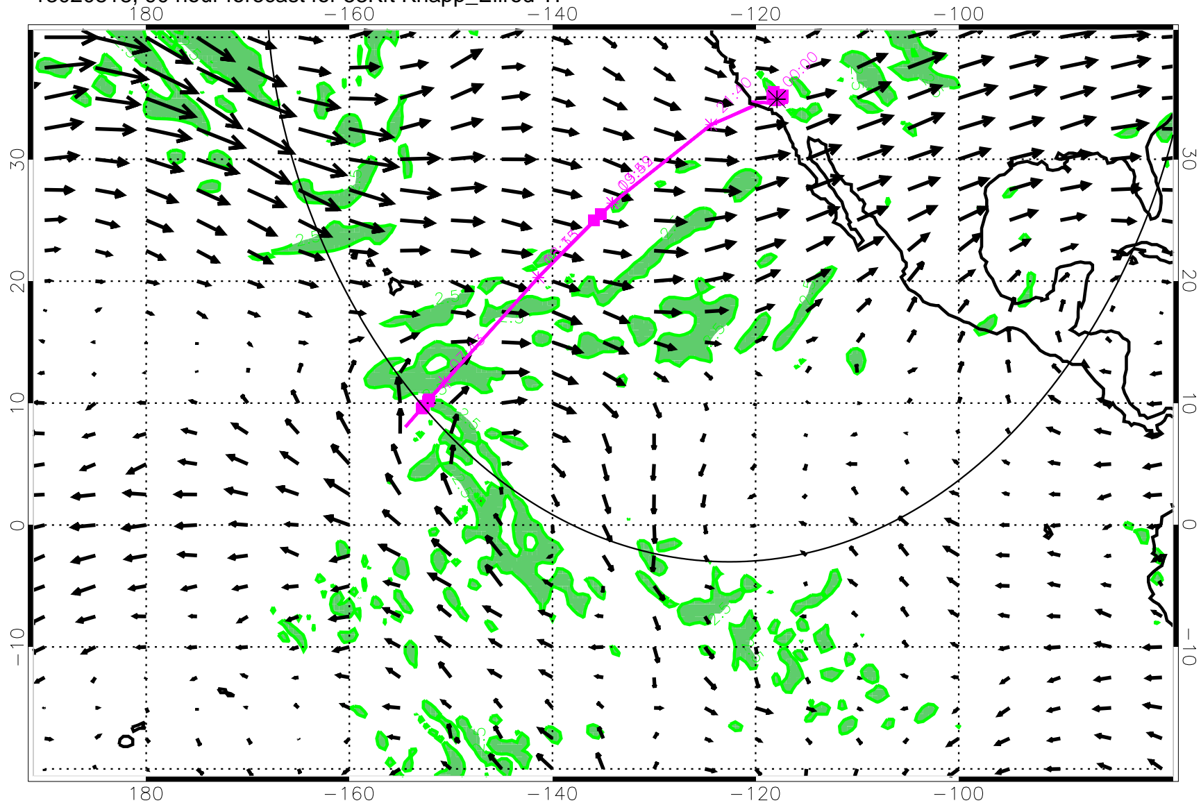
13020818, 90 hour forecast for 53Kft Knapp_Ellrod TI
