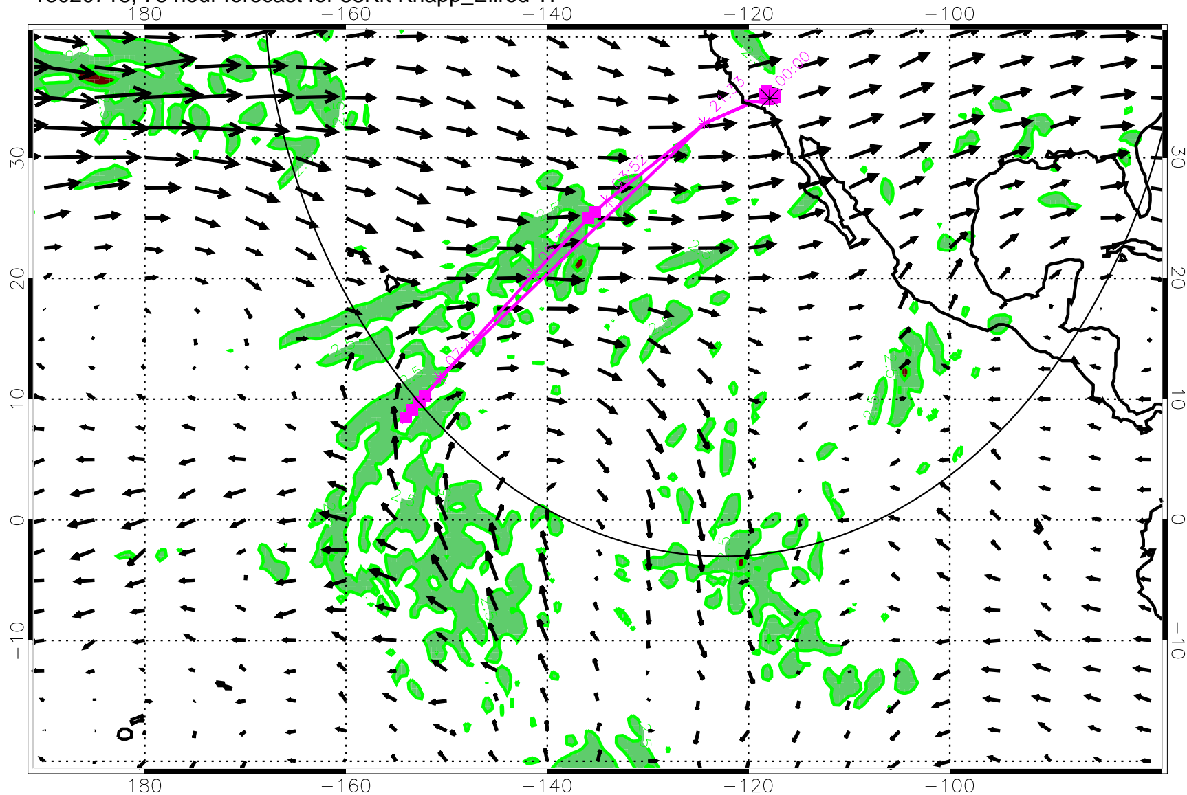
13020718, 78 hour forecast for 53Kft Knapp_Ellrod TI
