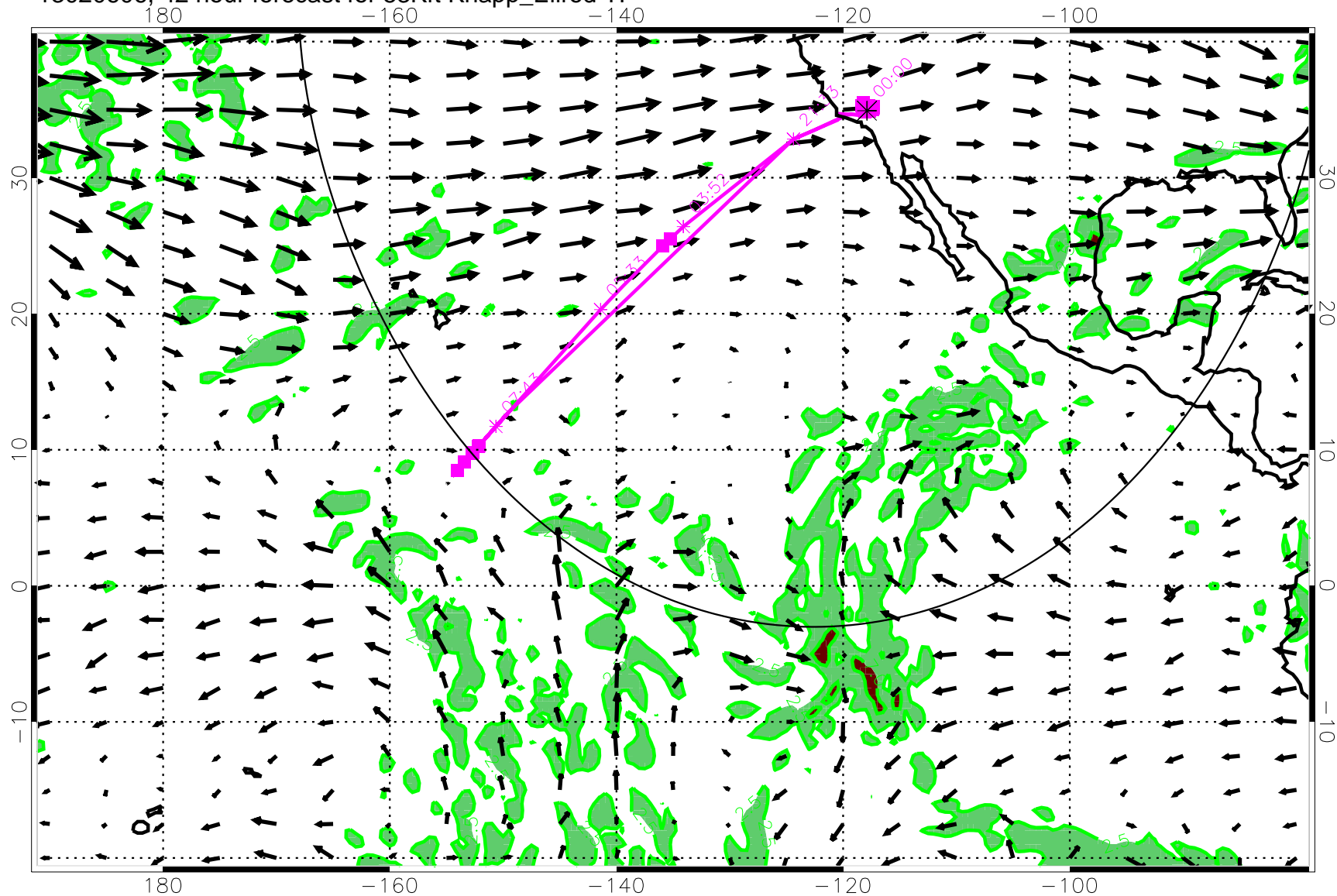
13020606, 42 hour forecast for 53Kft Knapp_Ellrod TI
