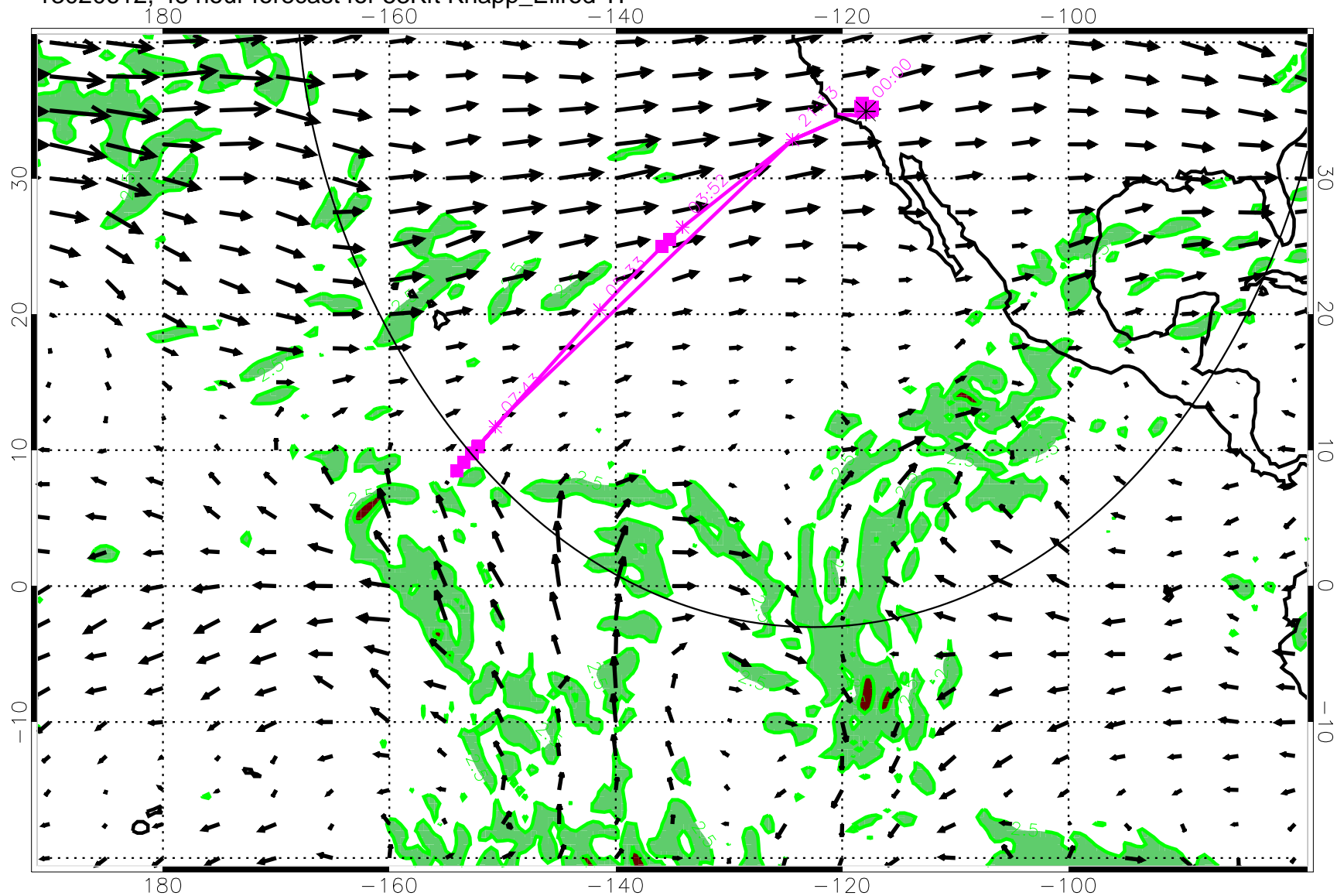
13020612, 48 hour forecast for 53Kft Knapp_Ellrod TI
