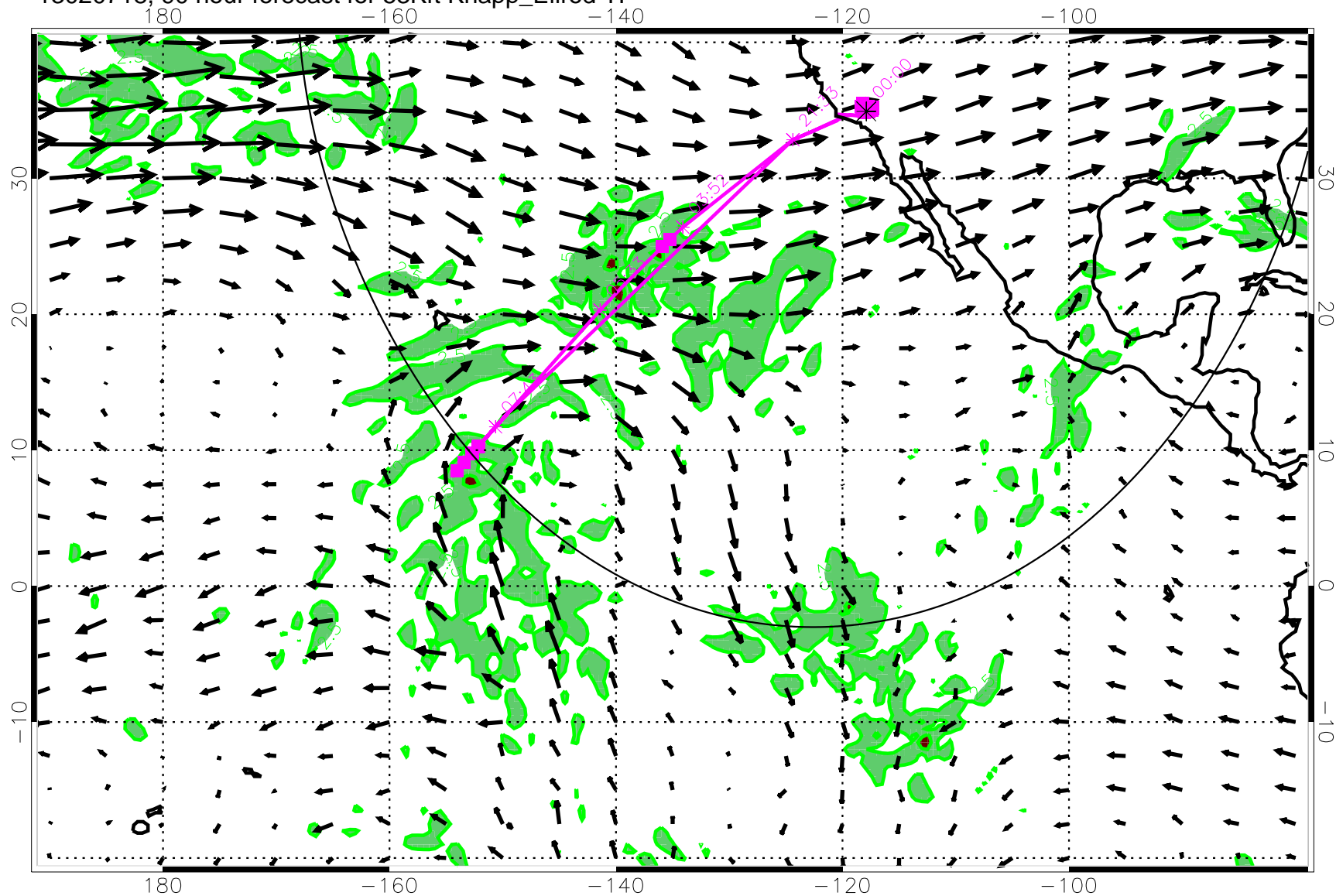
13020718, 90 hour forecast for 53Kft Knapp_Ellrod TI
