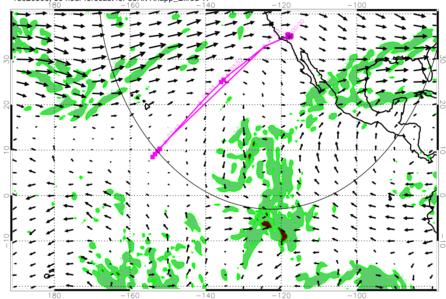
13020506, 30 hour forecast for 53Kft Knapp_Ellrod TI
