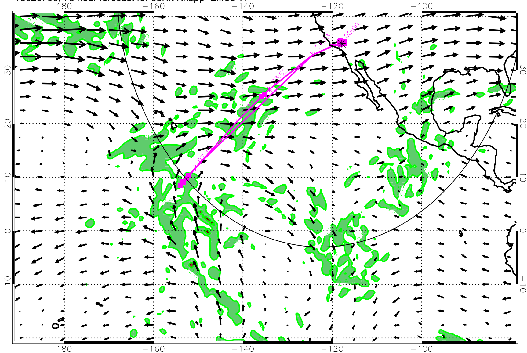
13020706, 78 hour forecast for 53Kft Knapp_Ellrod TI
