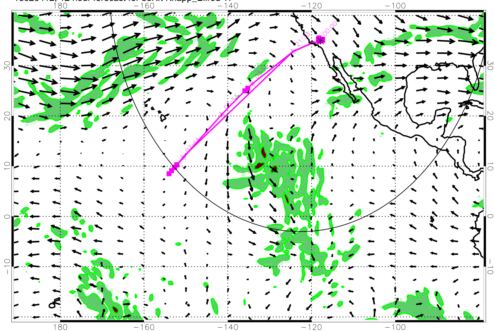
13020412, 12 hour forecast for 53Kft Knapp_Ellrod TI
