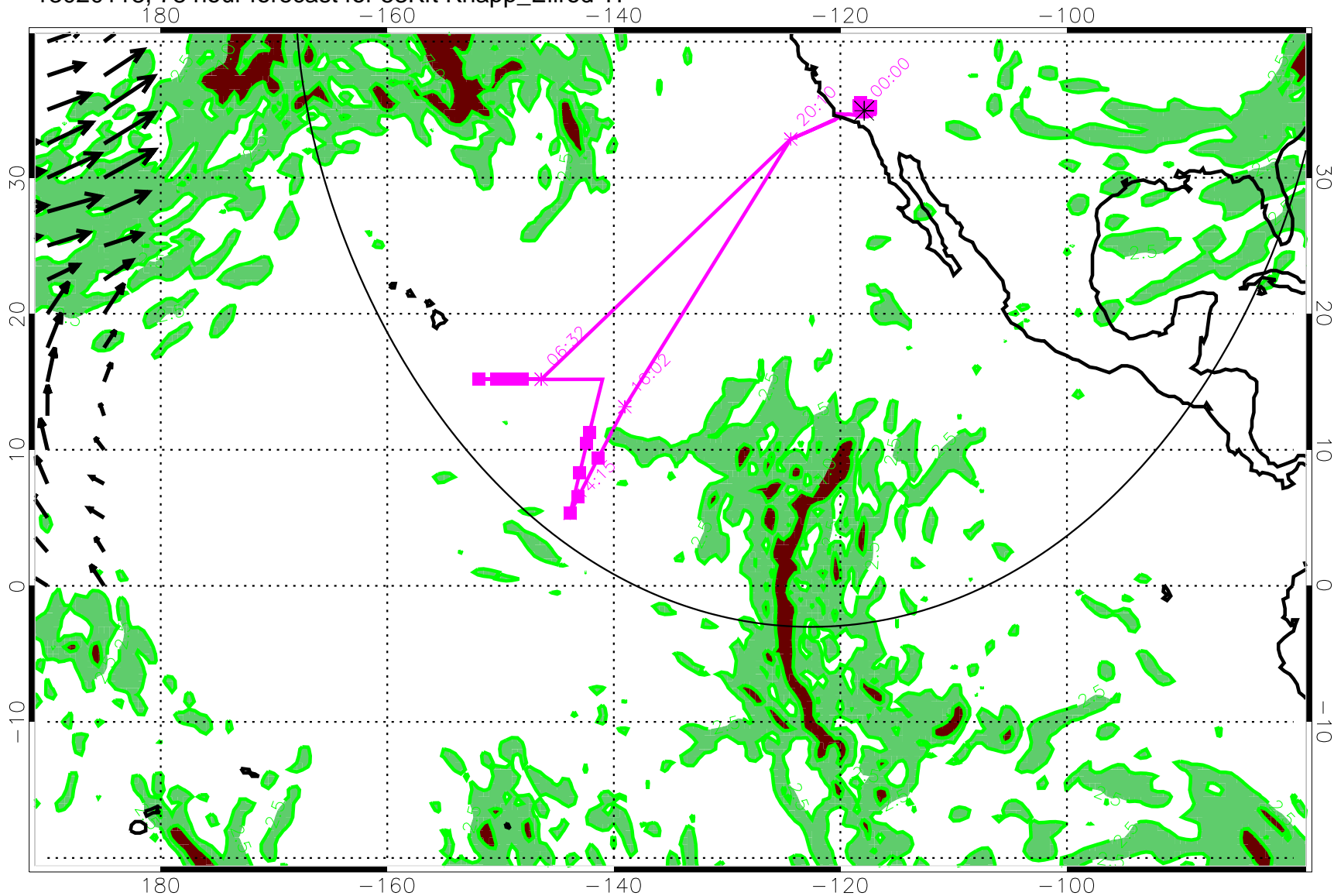
13020118, 78 hour forecast for 53Kft Knapp_Ellrod TI
