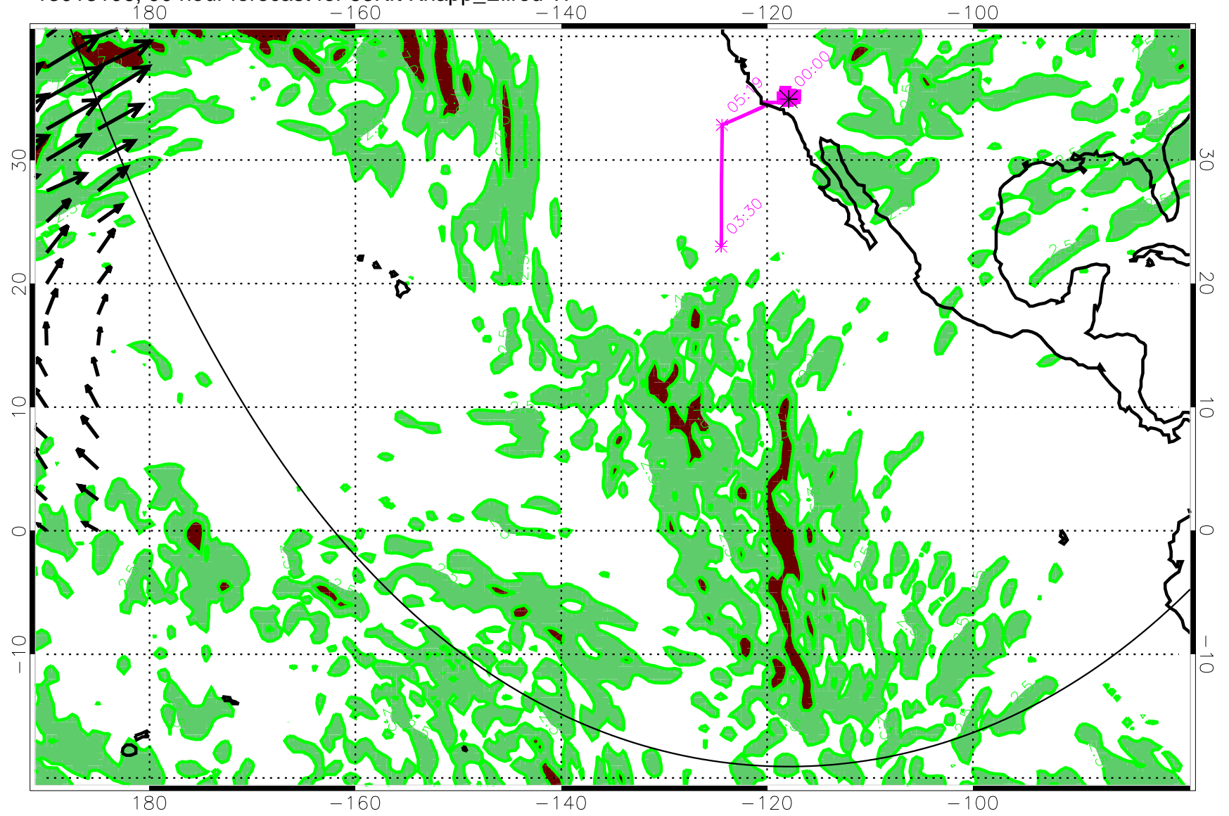
13013106, 90 hour forecast for 53Kft Knapp_Ellrod TI
