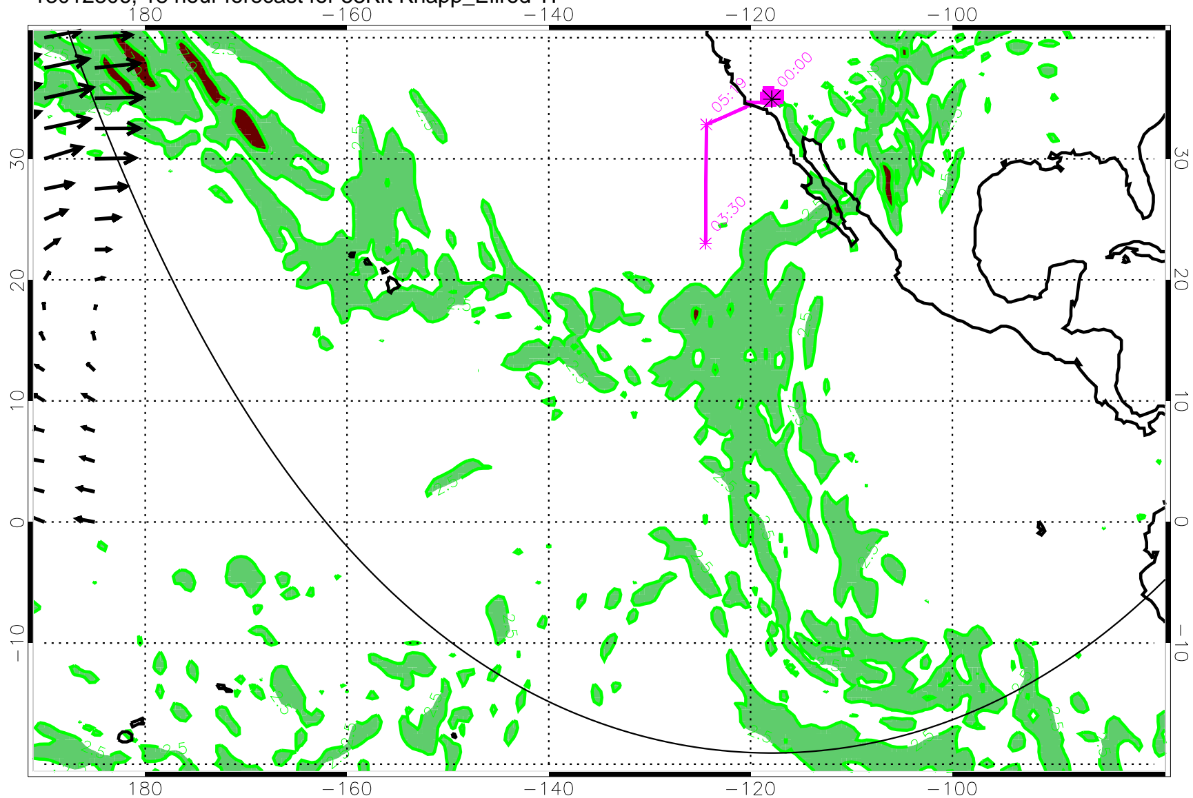
13012806, 18 hour forecast for 53Kft Knapp_Ellrod TI
