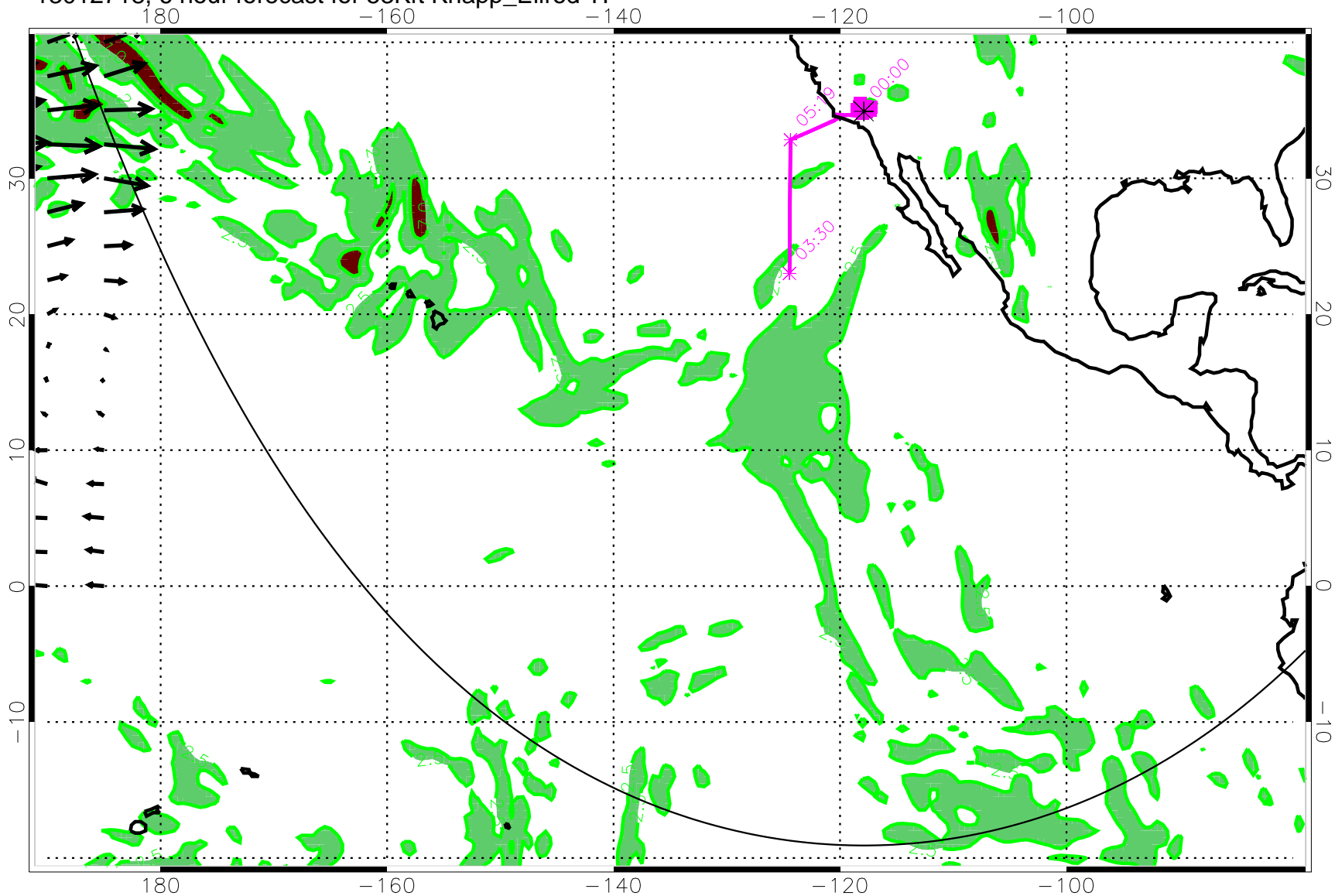
13012718, 6 hour forecast for 53Kft Knapp_Ellrod TI
