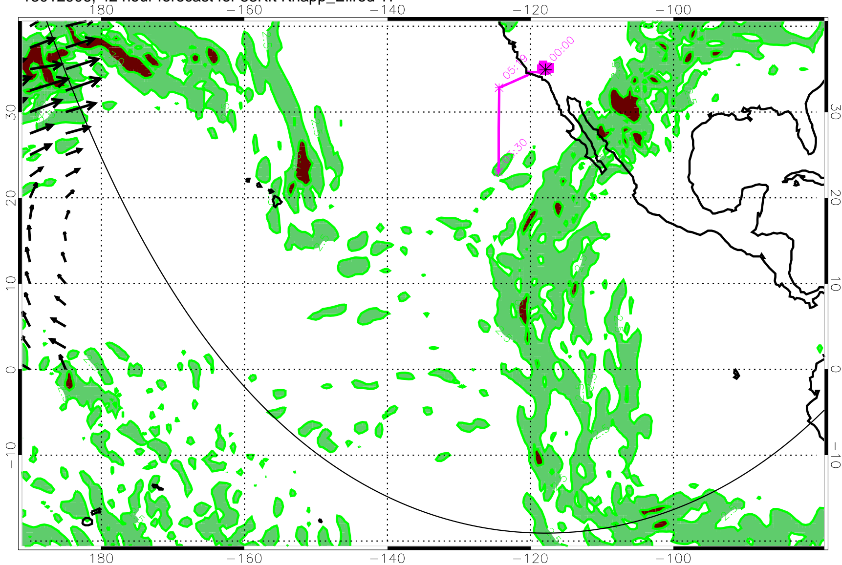
13012906, 42 hour forecast for 53Kft Knapp_Ellrod TI
