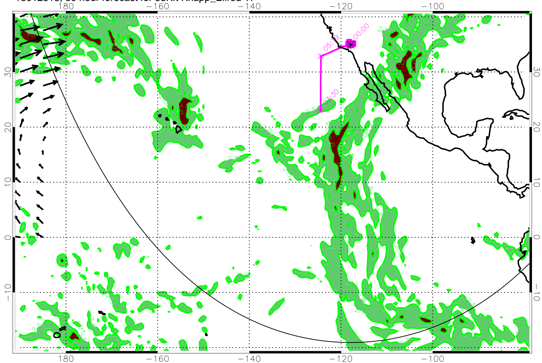
13012818, 30 hour forecast for 53Kft Knapp_Ellrod TI
