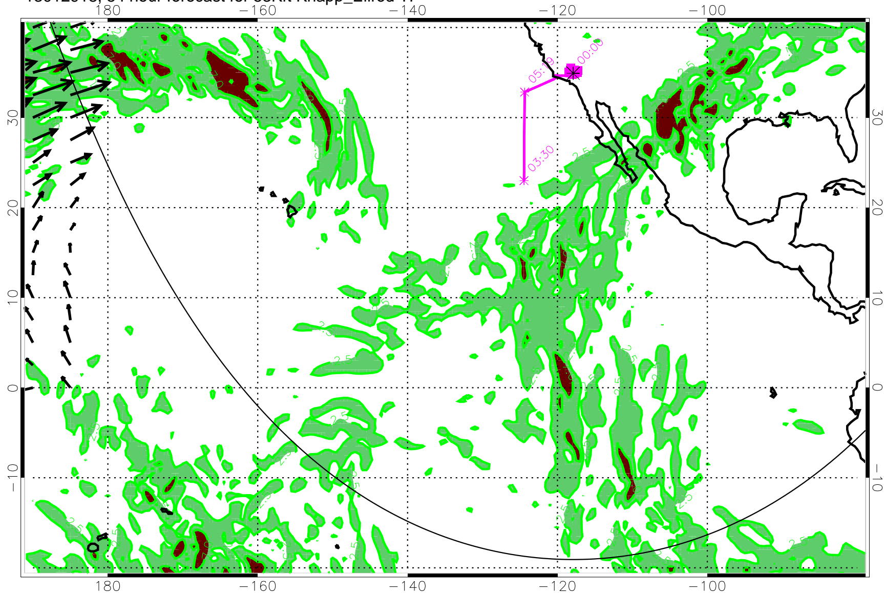
13012918, 54 hour forecast for 53Kft Knapp_Ellrod TI
