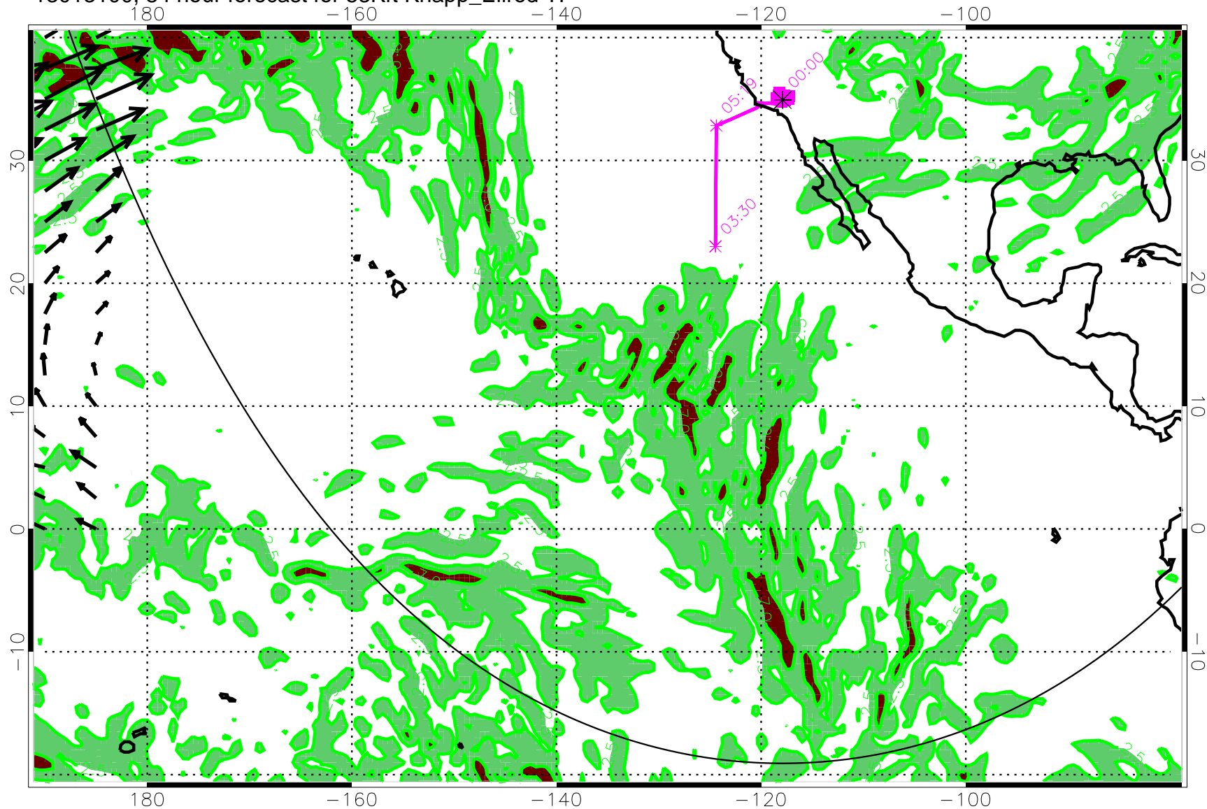
13013100, 84 hour forecast for 53Kft Knapp_Ellrod TI
