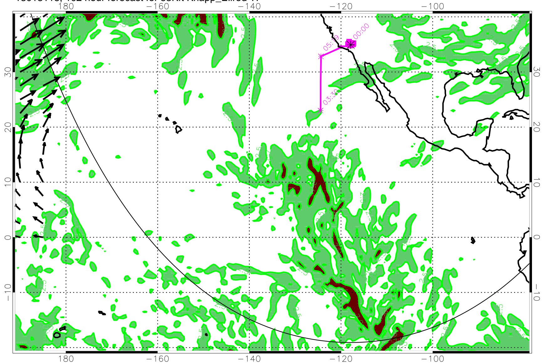
13013118, 102 hour forecast for 53Kft Knapp_Ellrod T1
