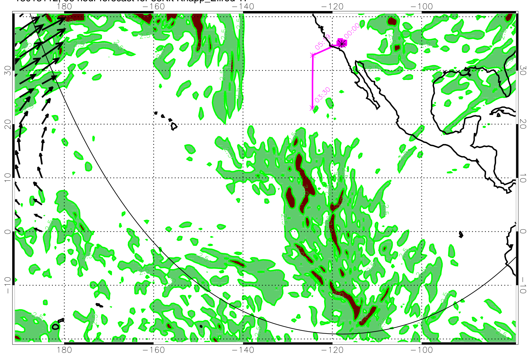
13013112, 96 hour forecast for 53Kft Knapp_Ellrod TI
