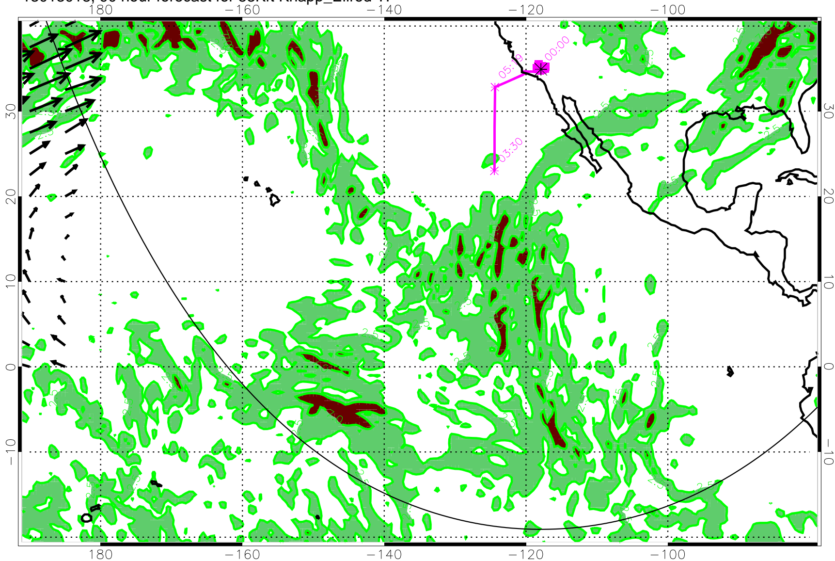
13013018, 90 hour forecast for 53Kft Knapp_Ellrod TI
