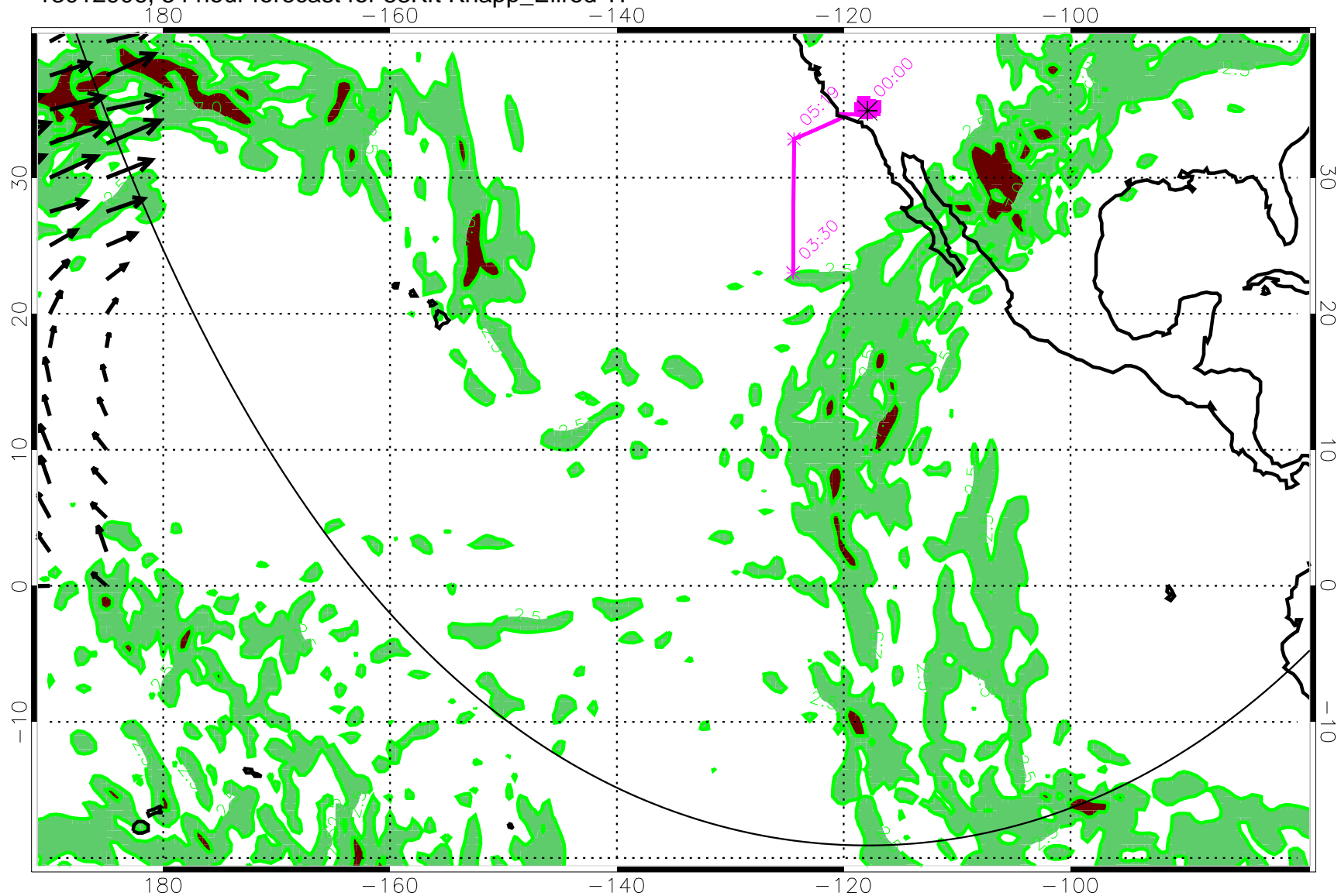
13012906, 54 hour forecast for 53Kft Knapp_Ellrod TI
