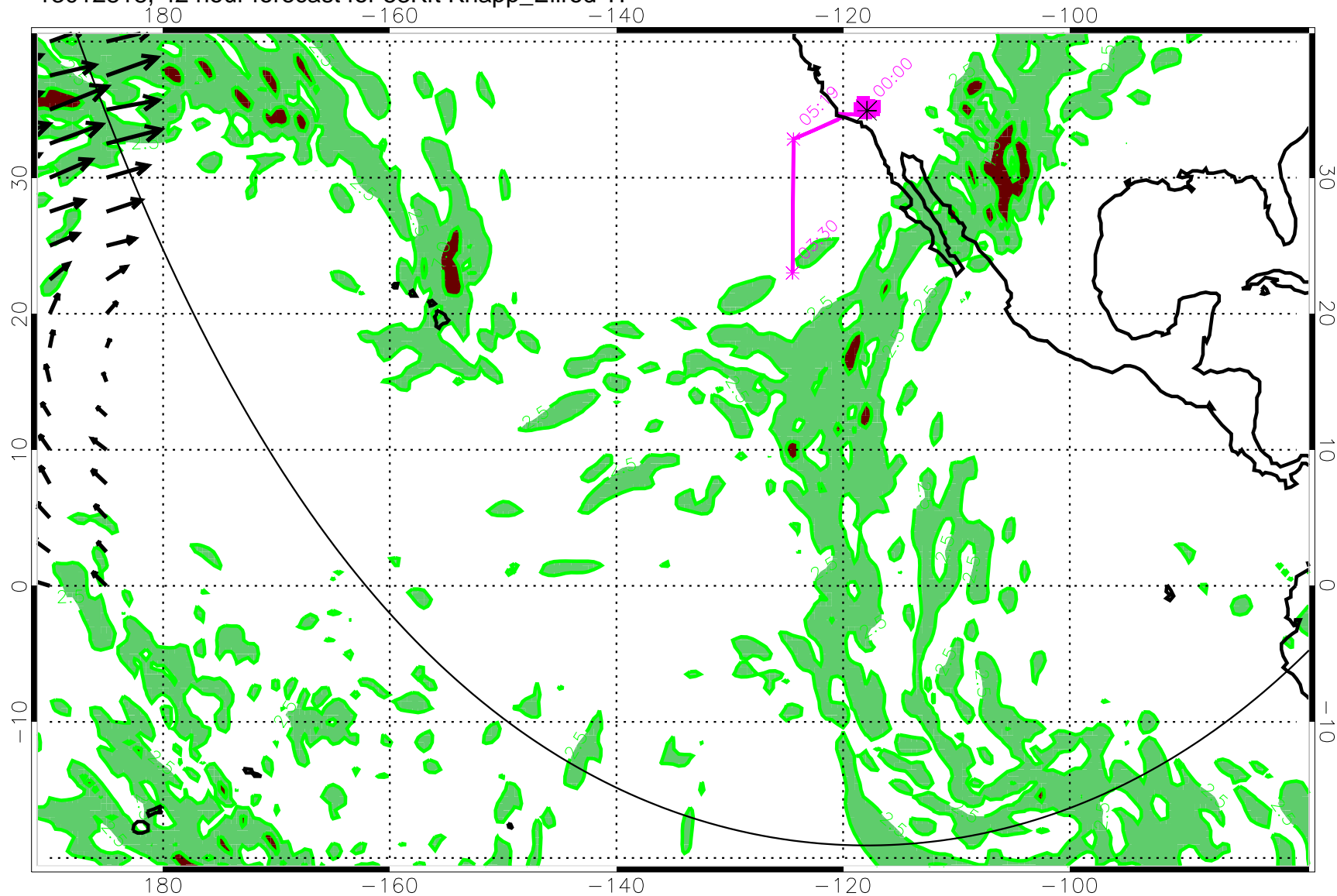
13012818, 42 hour forecast for 53Kft Knapp_Ellrod TI
