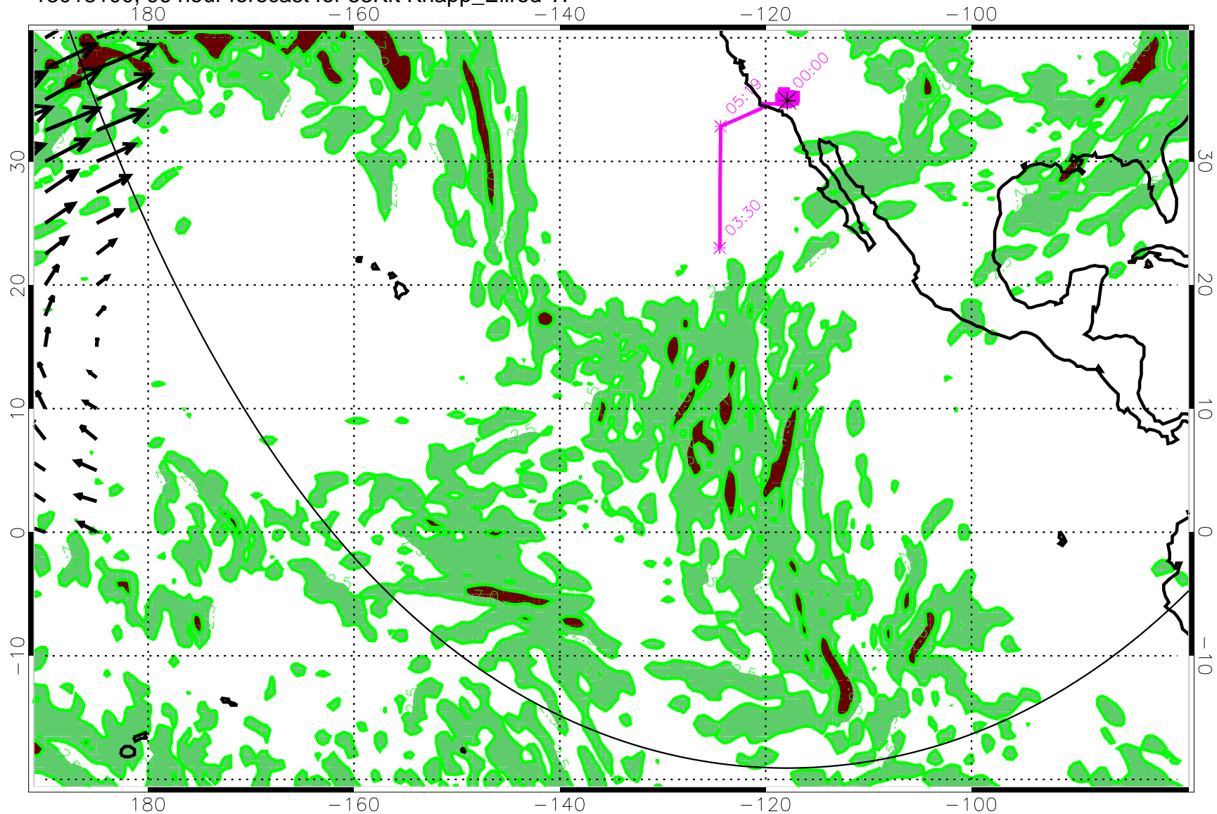
13013100, 96 hour forecast for 53Kft Knapp_Ellrod TI
