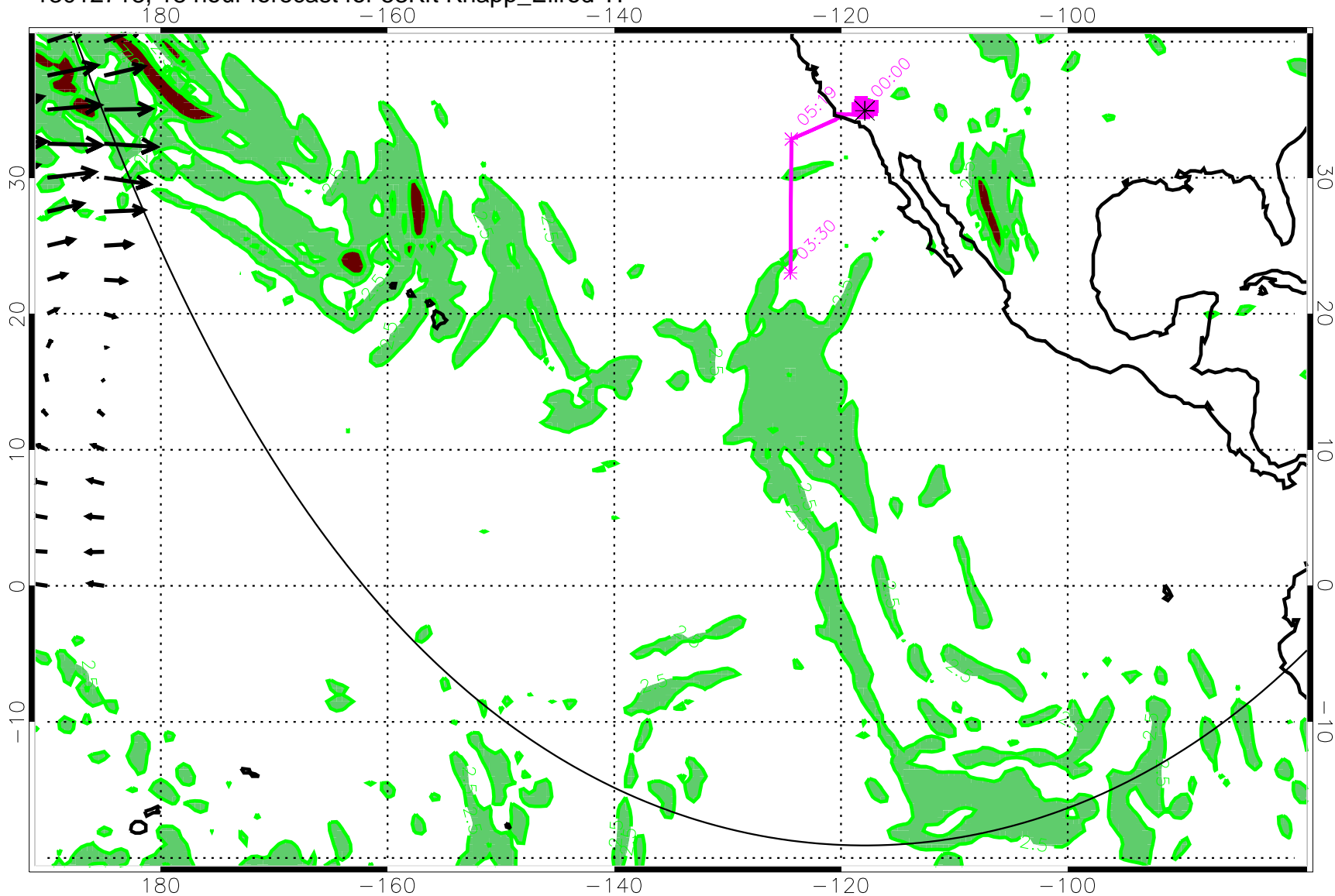
13012718, 18 hour forecast for 53Kft Knapp_Ellrod TI
