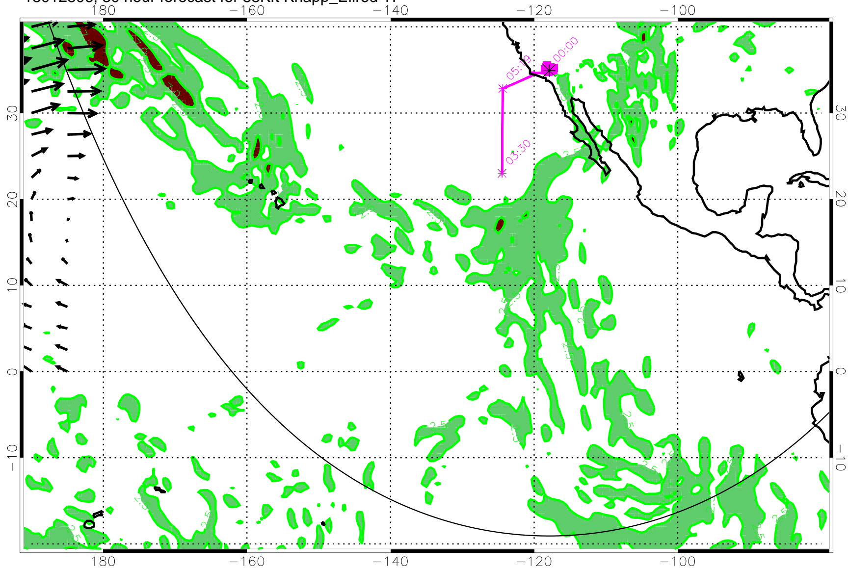
13012806, 30 hour forecast for 53Kft Knapp_Ellrod TI
