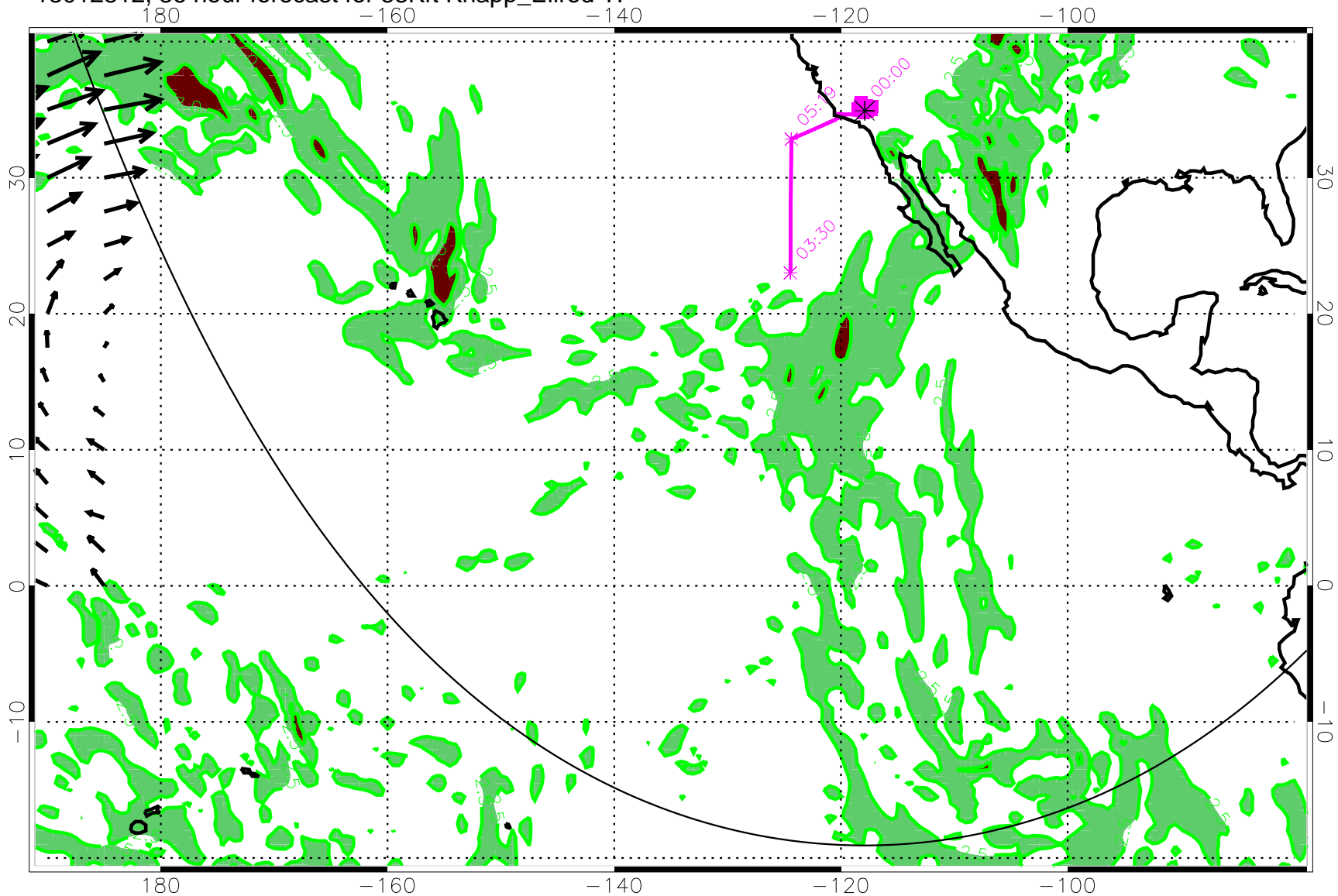
13012812, 36 hour forecast for 53Kft Knapp_Ellrod TI
