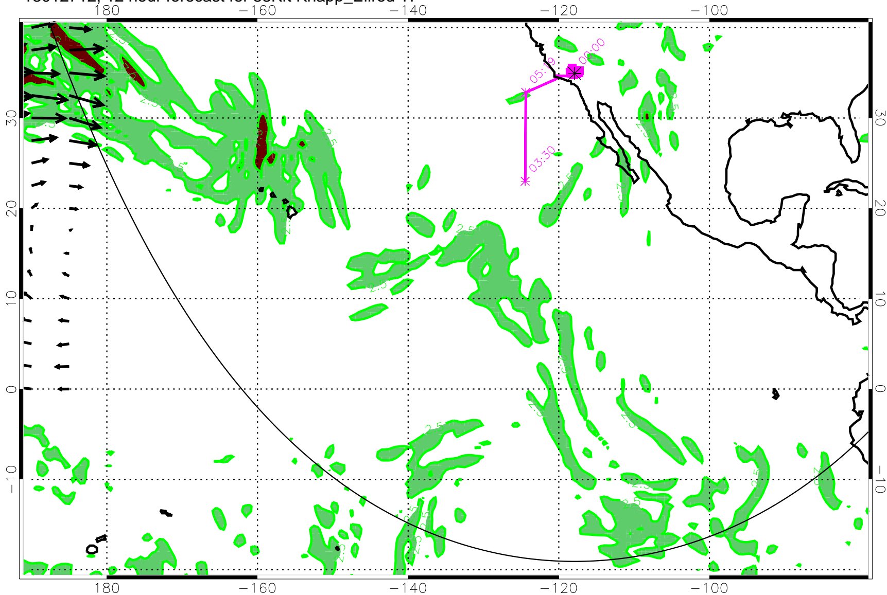
13012712, 12 hour forecast for 53Kft Knapp_Ellrod TI
