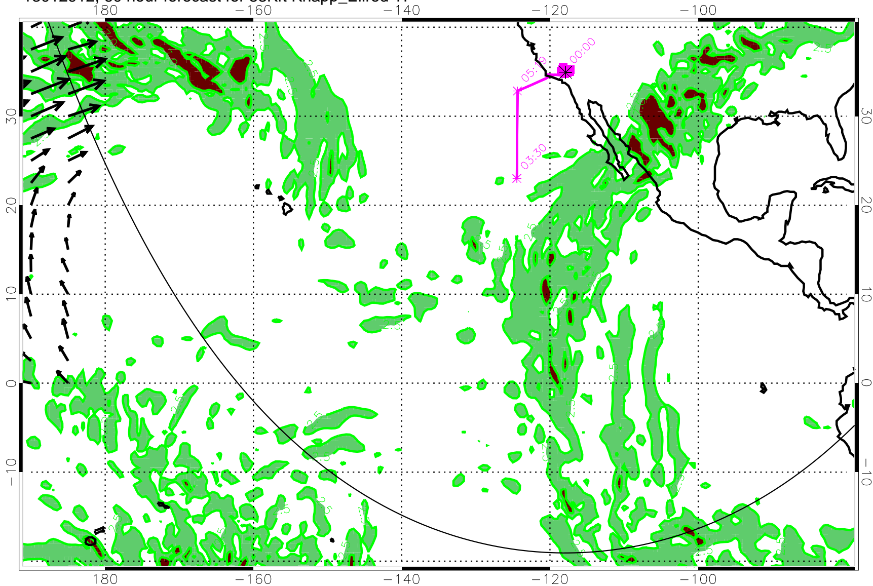
13012912, 60 hour forecast for 53Kft Knapp_Ellrod TI
