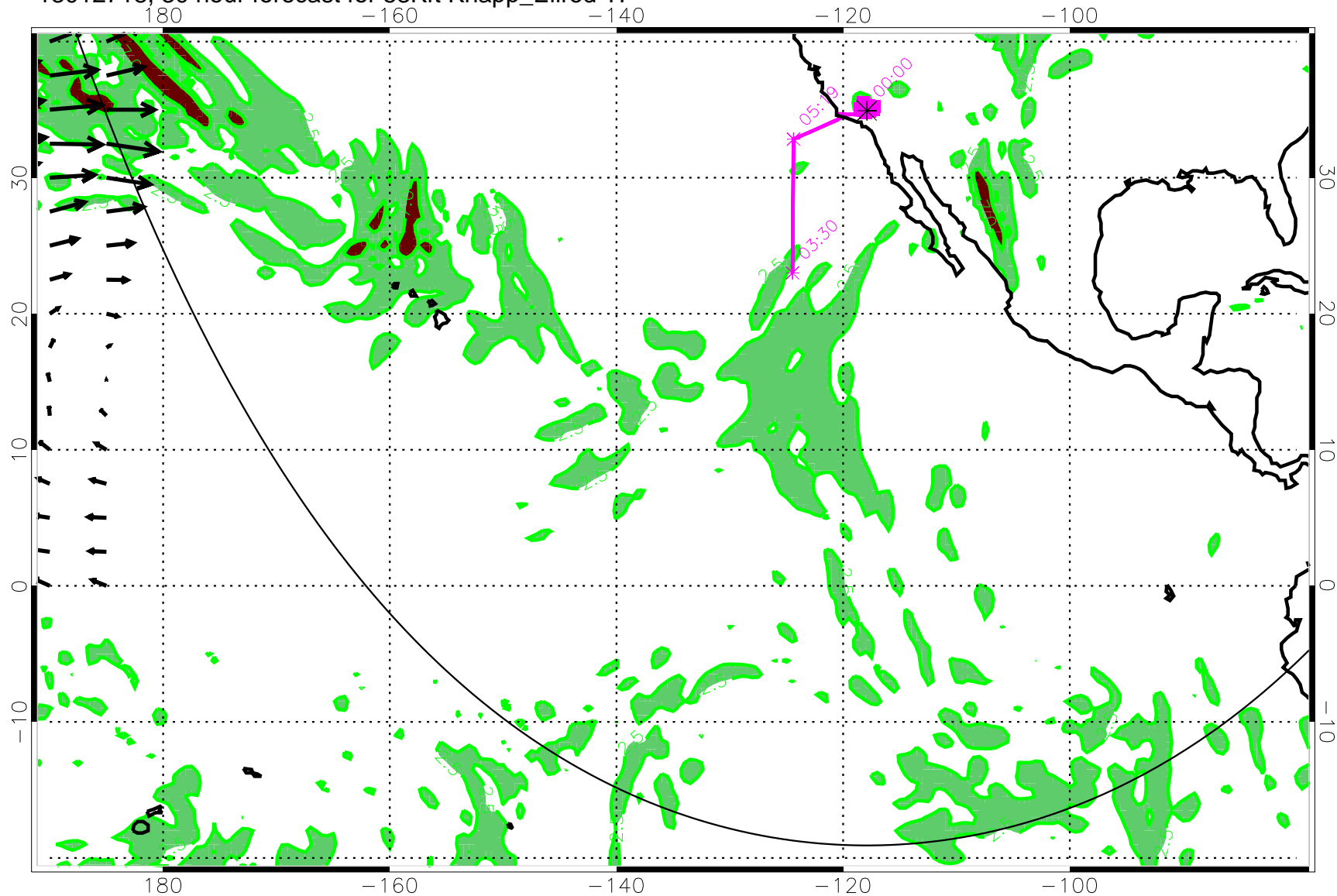
13012718, 30 hour forecast for 53Kft Knapp_Ellrod TI
