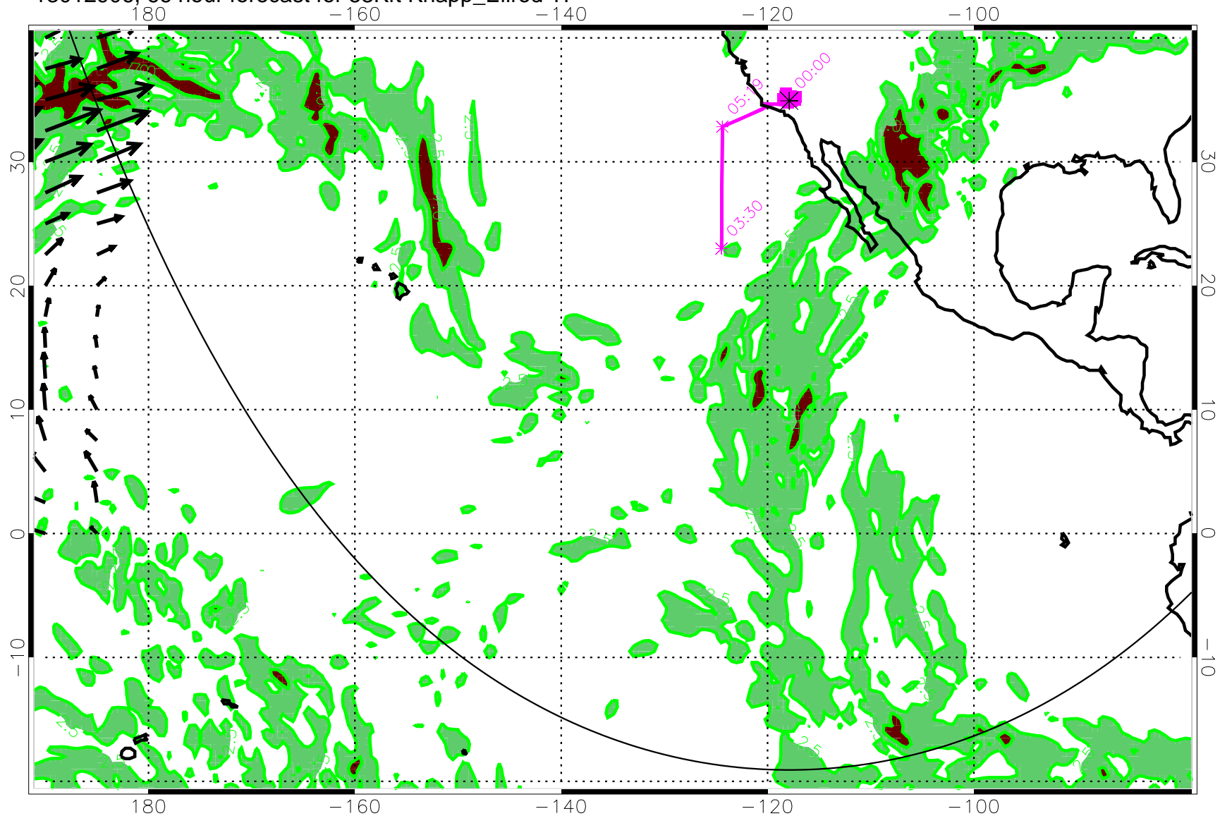
13012906, 66 hour forecast for 53Kft Knapp_Ellrod TI
