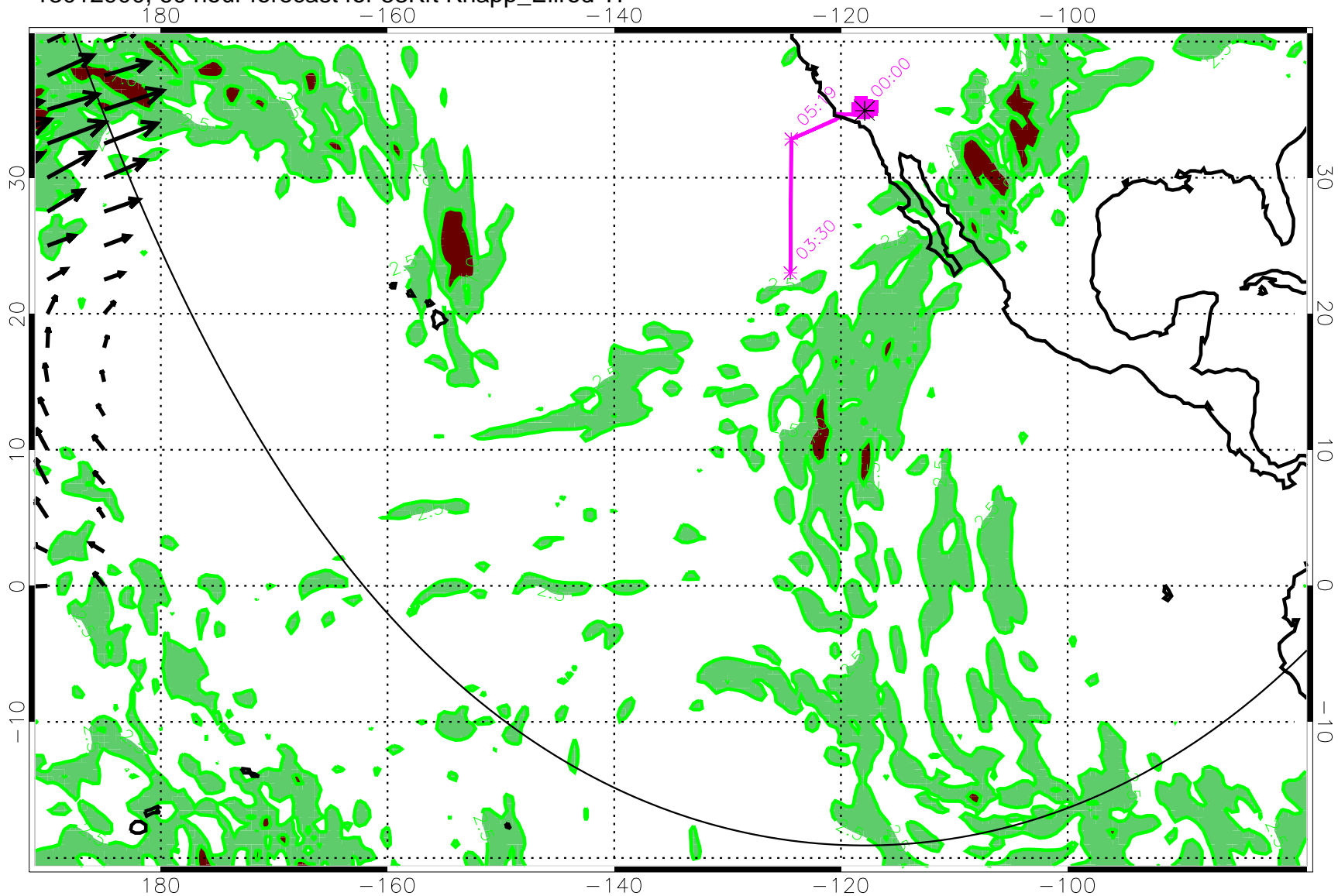
13012900, 60 hour forecast for 53Kft Knapp_Ellrod TI
