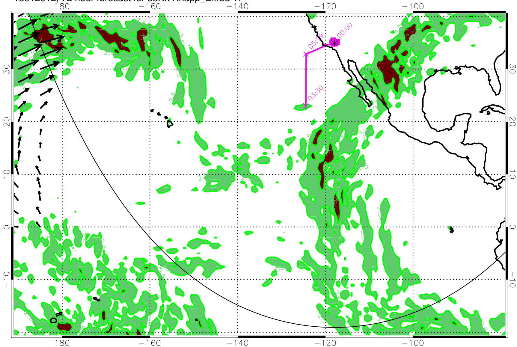
13012912, 72 hour forecast for 53Kft Knapp_Ellrod TI
