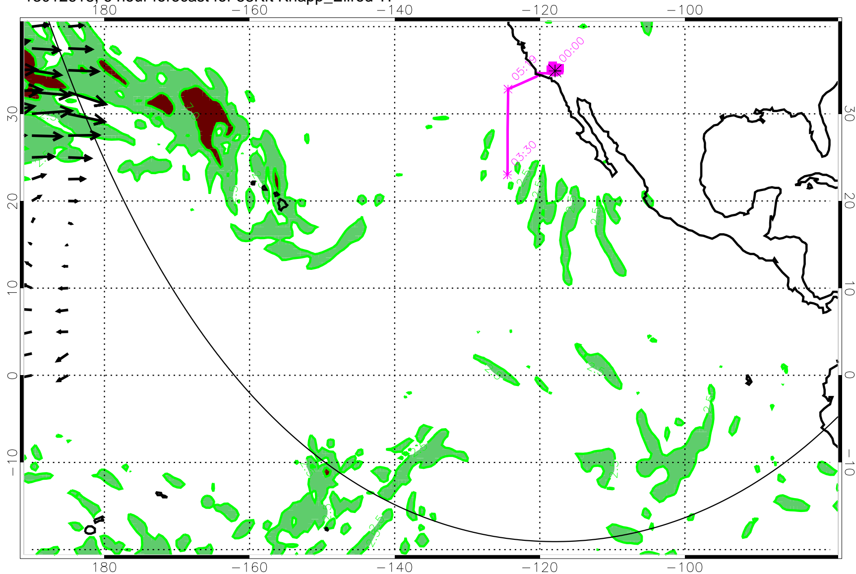
13012618, 6 hour forecast for 53Kft Knapp_Ellrod TI
