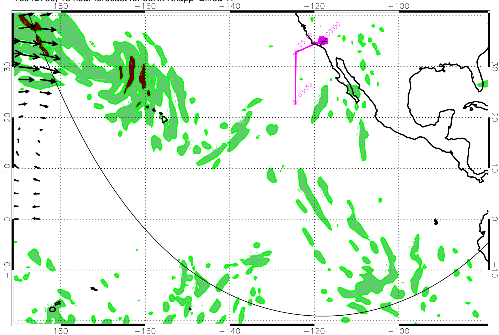
13012706, 18 hour forecast for 53Kft Knapp_Ellrod TI
