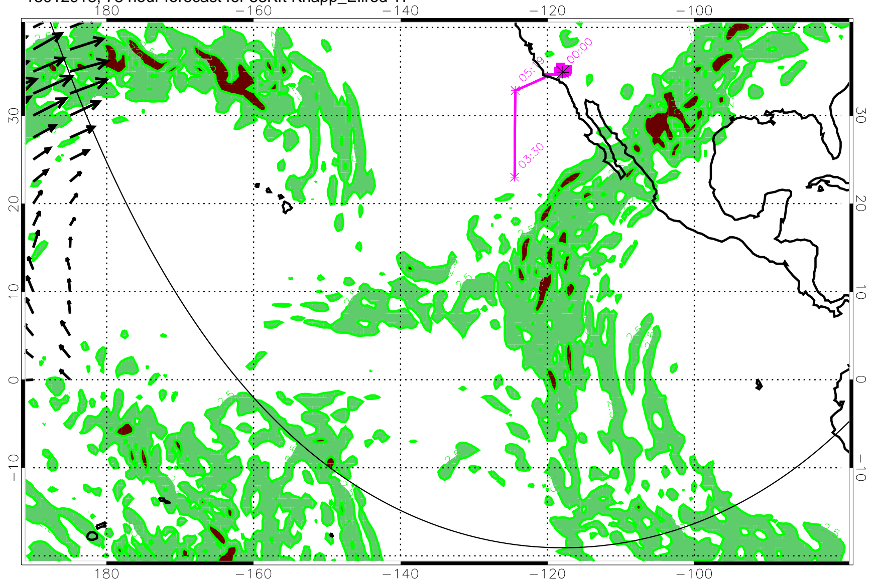
13012918, 78 hour forecast for 53Kft Knapp_Ellrod TI
