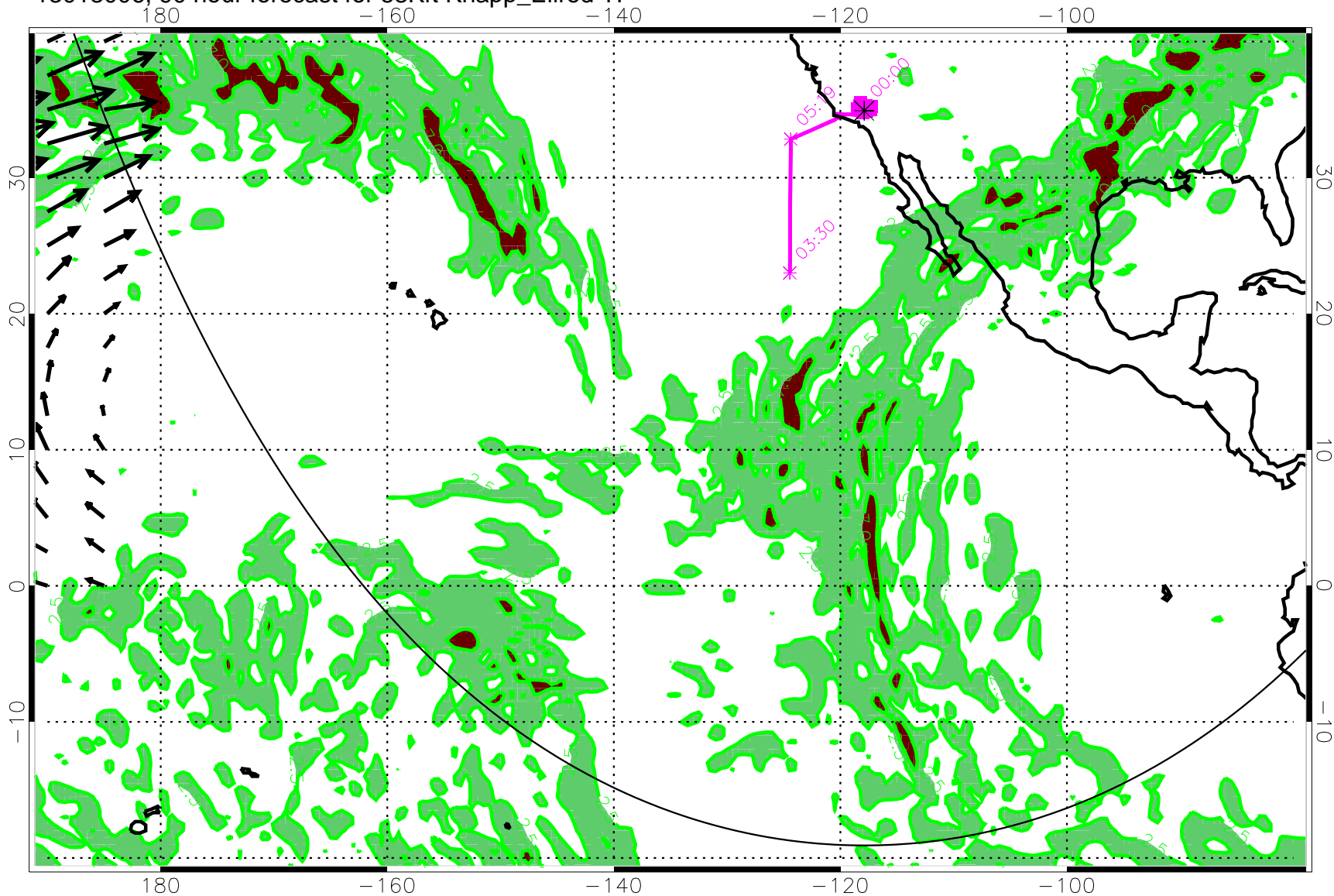
13013006, 90 hour forecast for 53Kft Knapp_Ellrod TI
