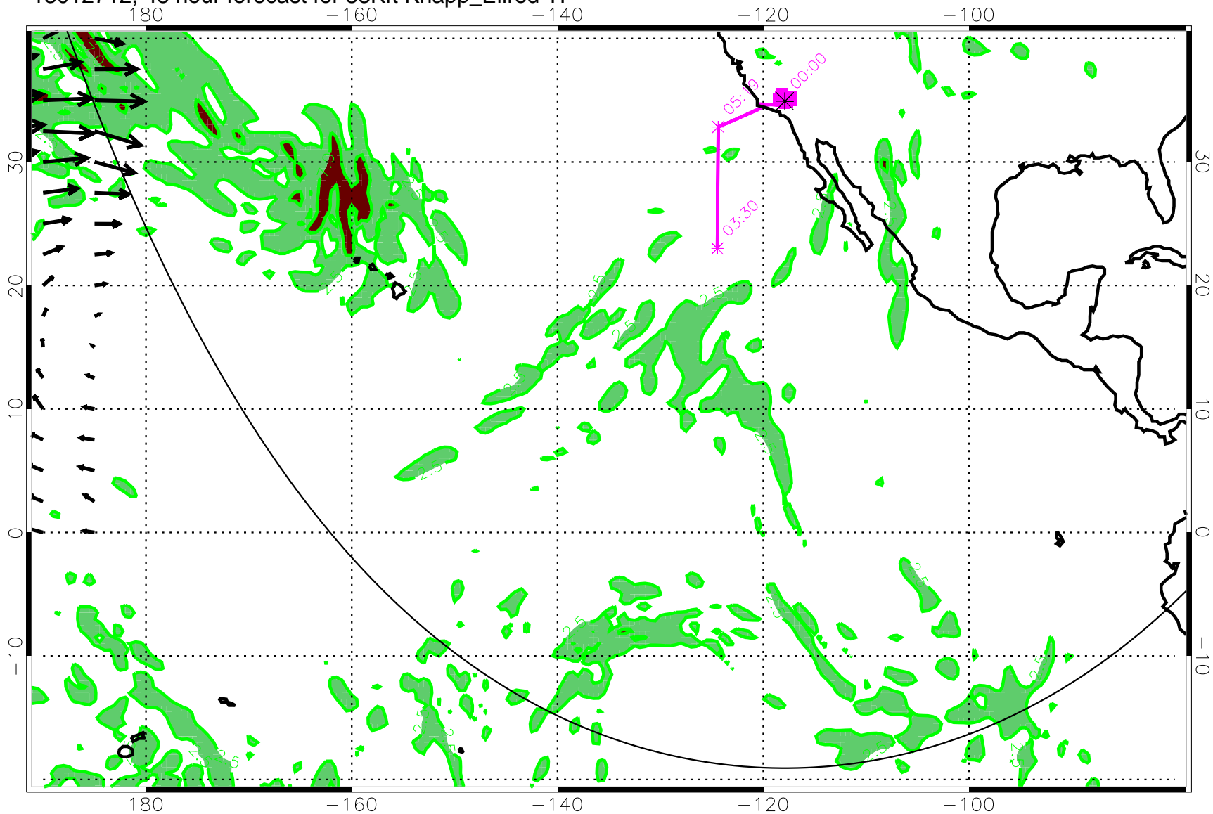
13012712, 48 hour forecast for 53Kft Knapp_Ellrod TI
