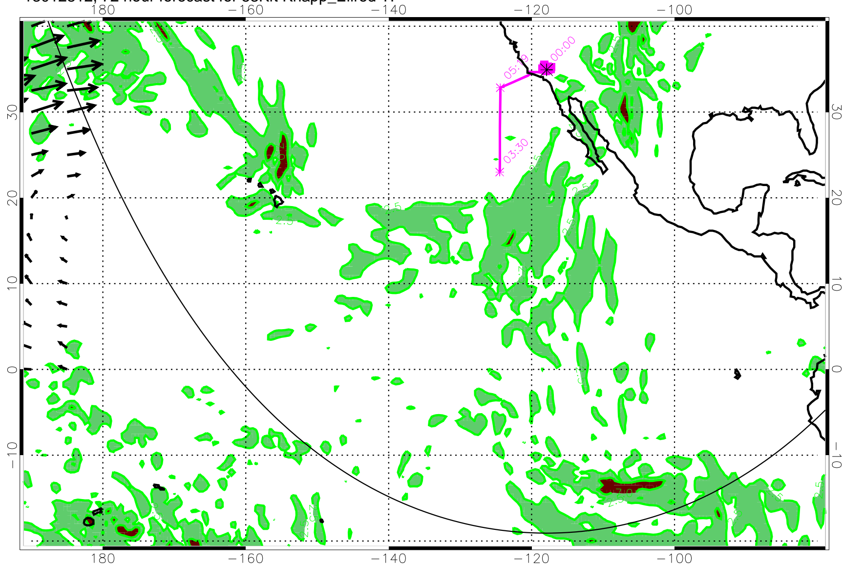
13012812, 72 hour forecast for 53Kft Knapp_Ellrod TI
