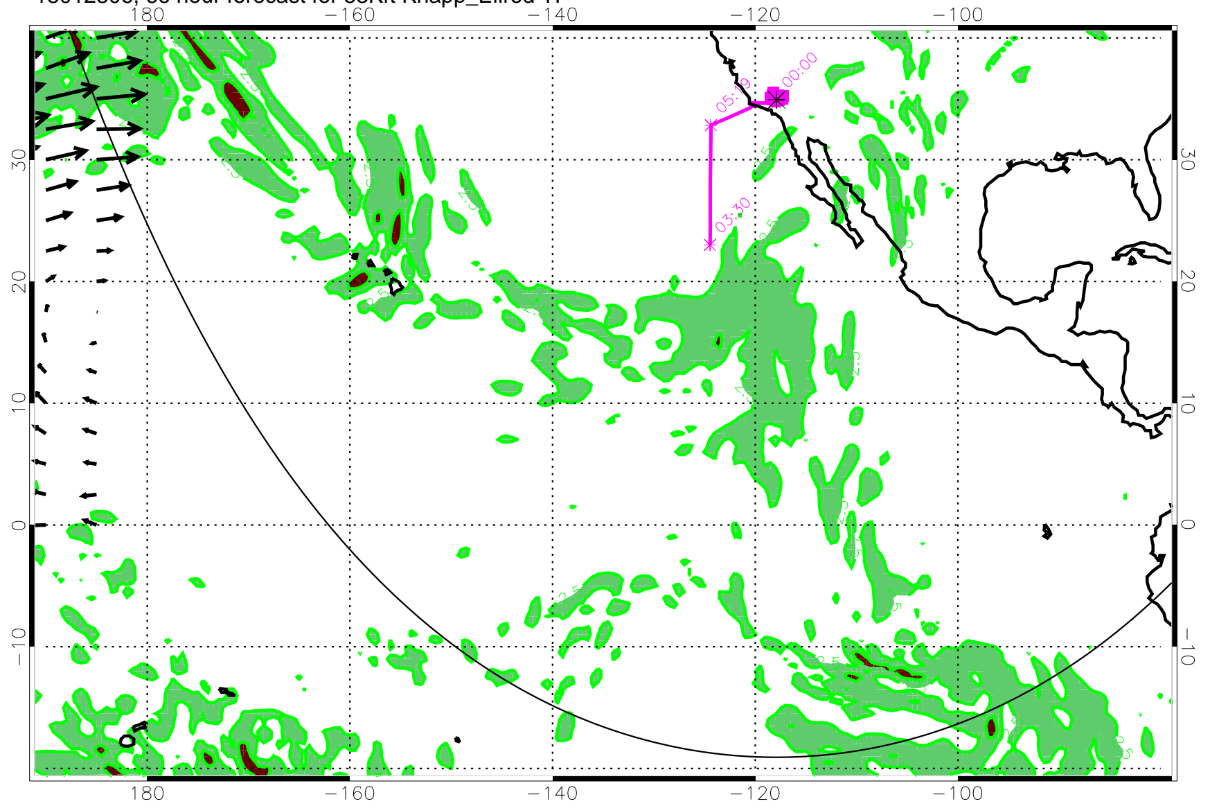
13012806, 66 hour forecast for 53Kft Knapp_Ellrod TI
