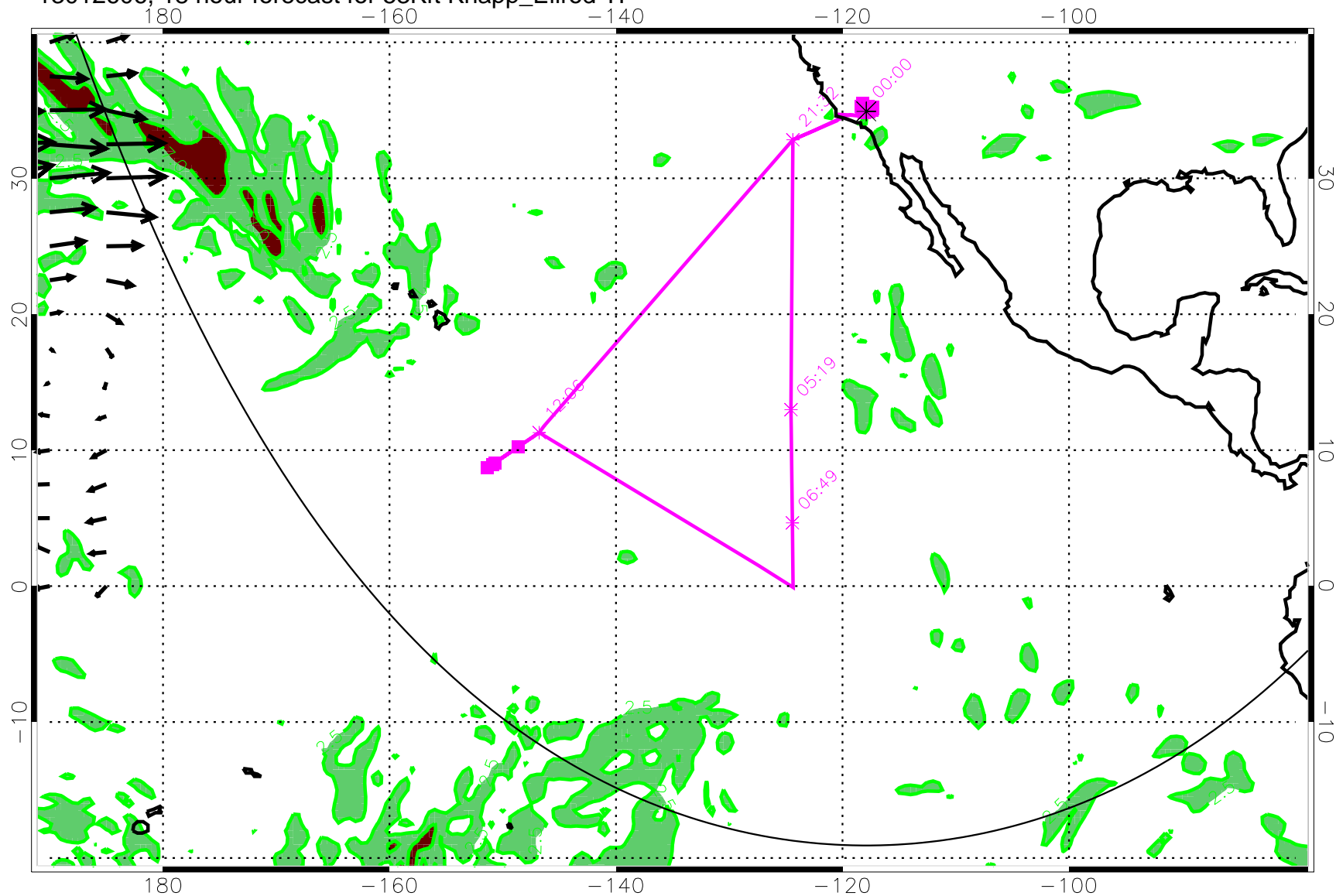
13012606, 18 hour forecast for 53Kft Knapp_Ellrod TI
