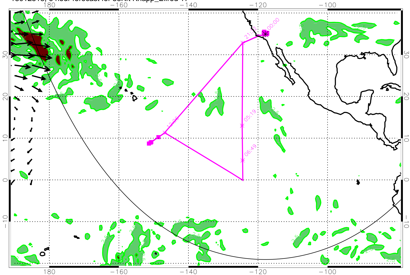
13012518, 6 hour forecast for 53Kft Knapp_Ellrod TI
