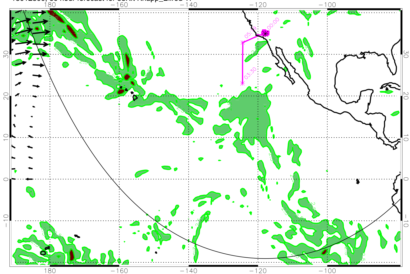
13012800, 60 hour forecast for 53Kft Knapp_Ellrod TI
