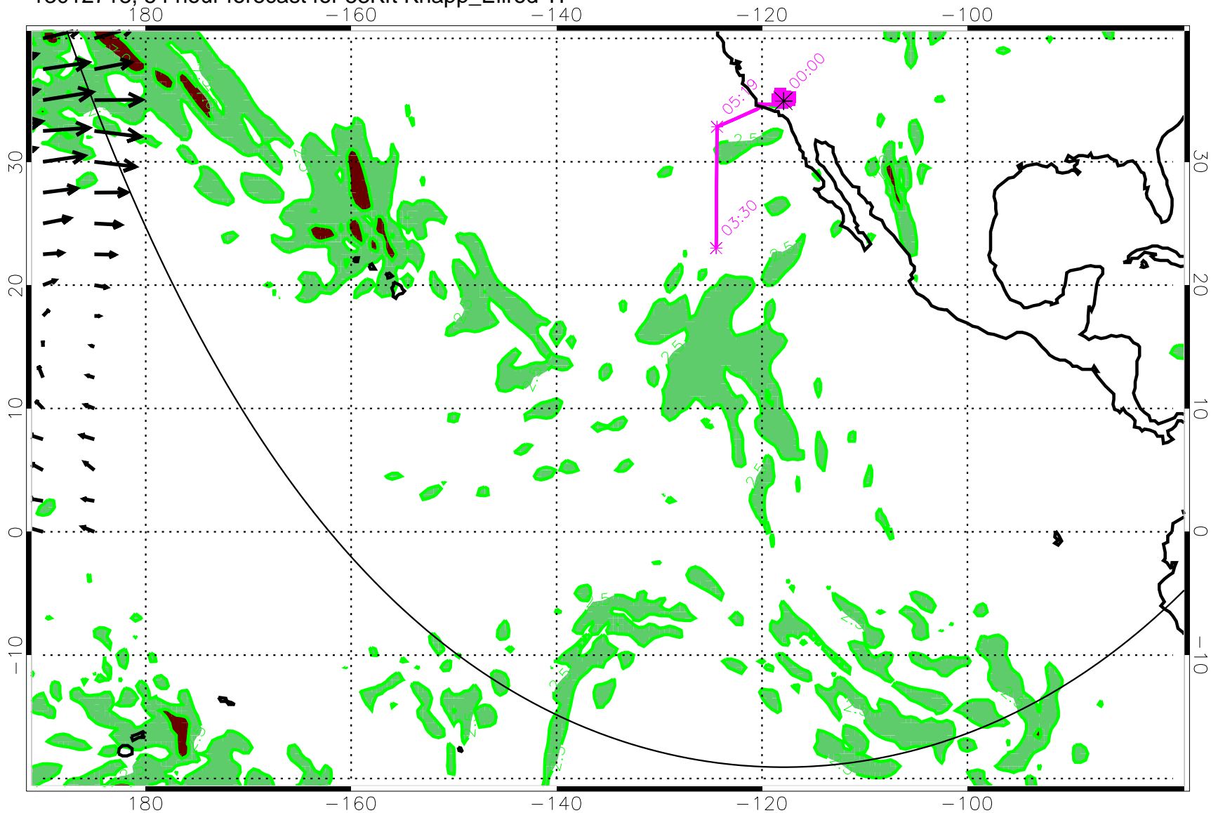
13012718, 54 hour forecast for 53Kft Knapp_Ellrod TI
