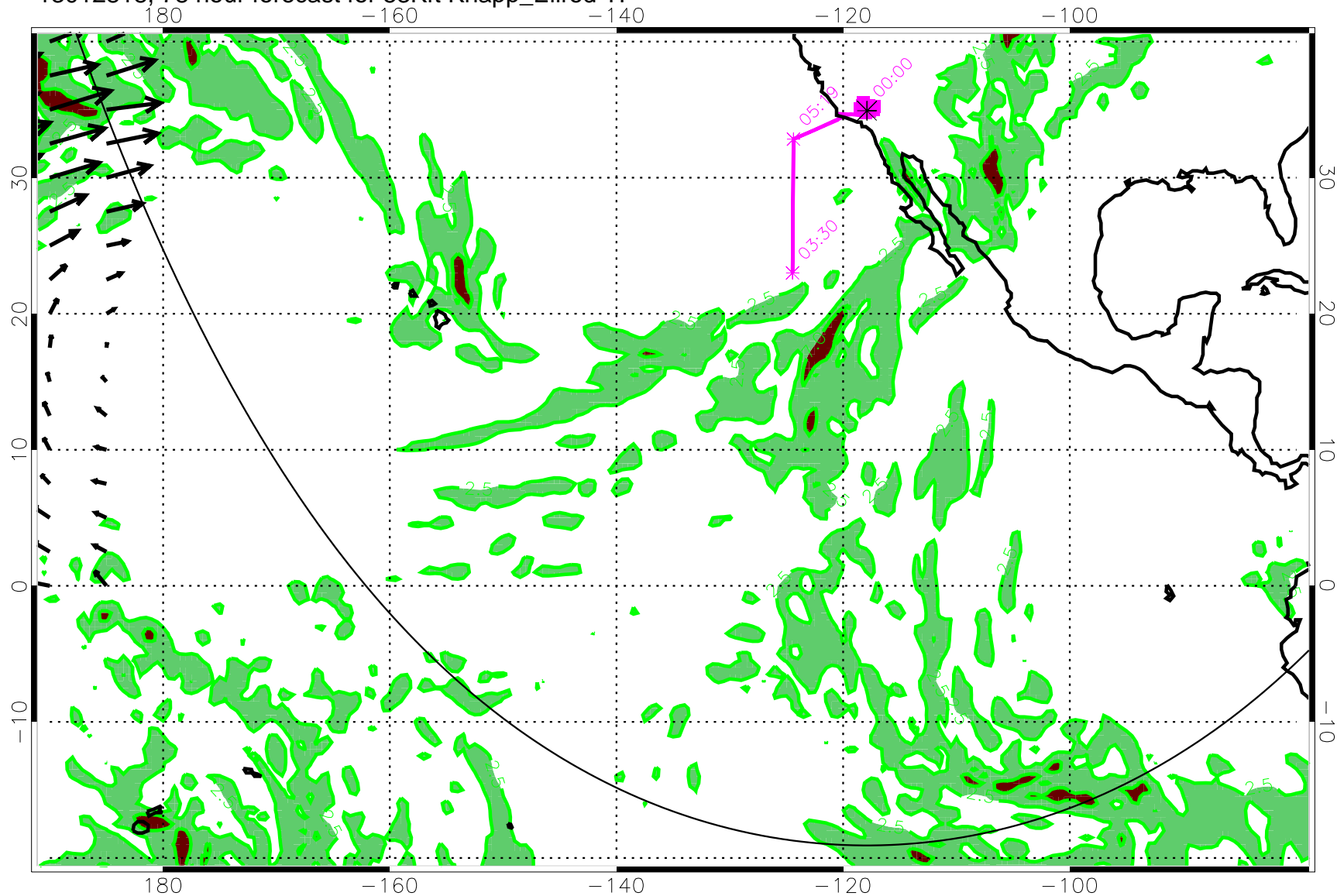
13012818, 78 hour forecast for 53Kft Knapp_Ellrod TI
