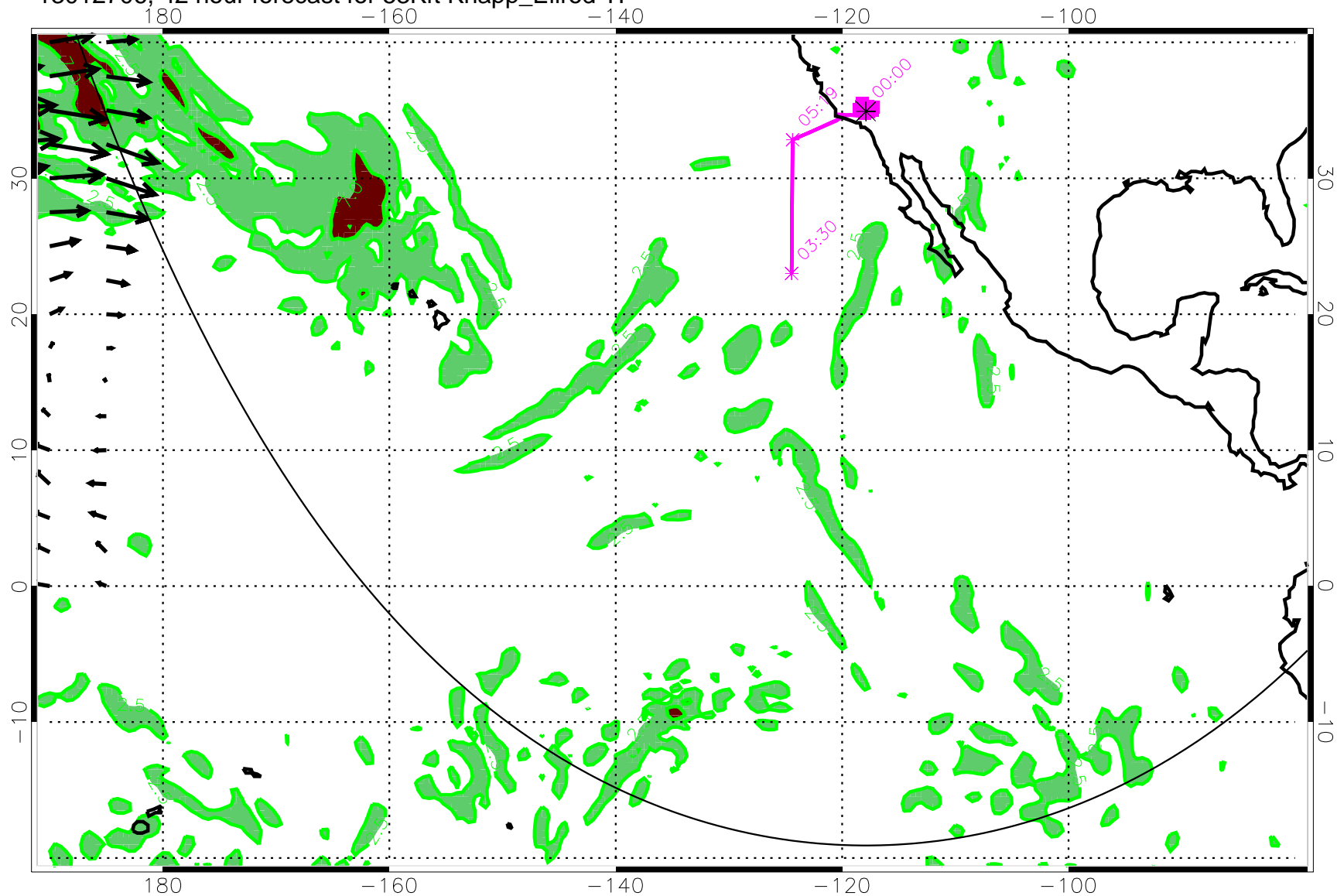
13012706, 42 hour forecast for 53Kft Knapp_Ellrod TI
