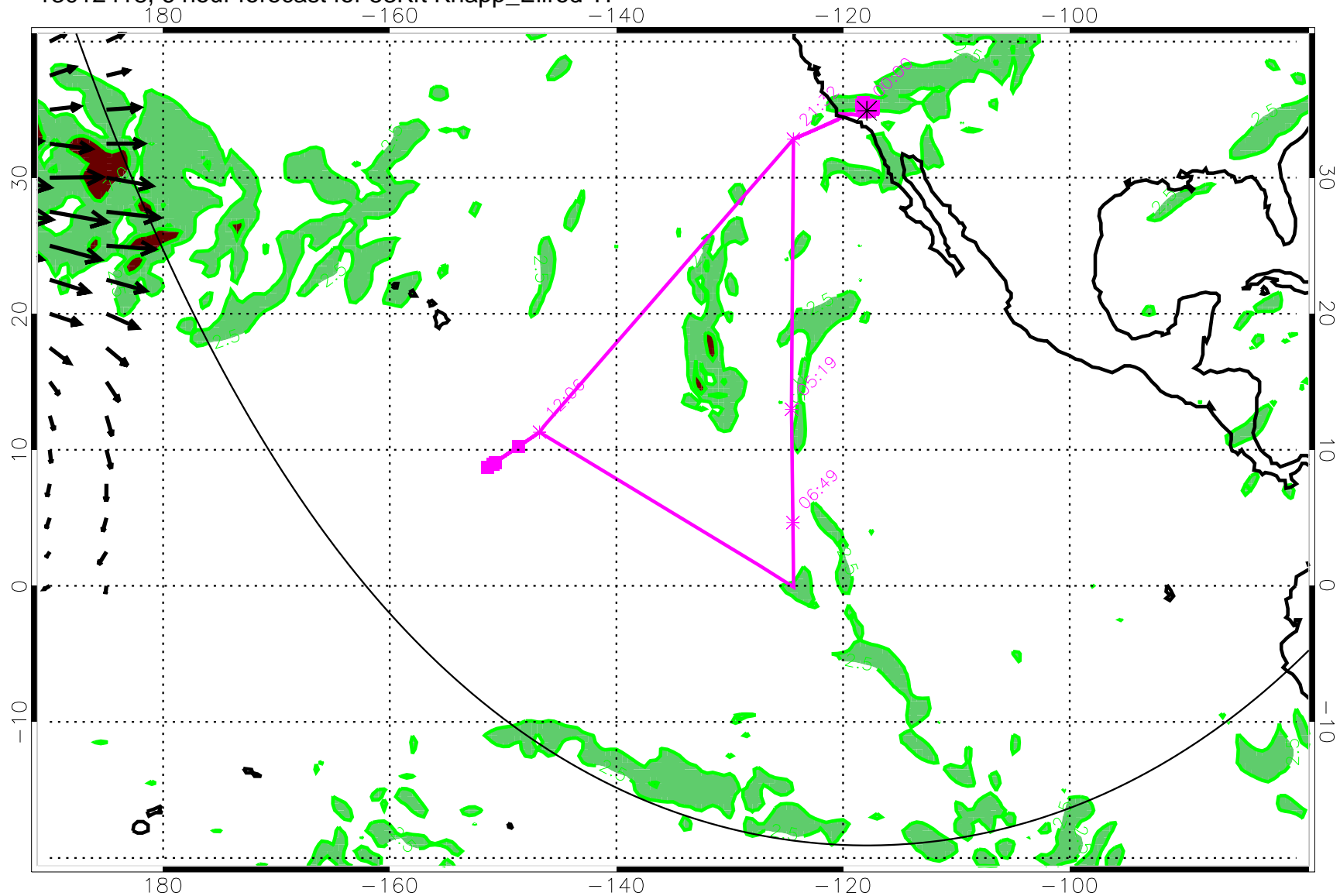
13012418, 6 hour forecast for 53Kft Knapp_Ellrod TI
