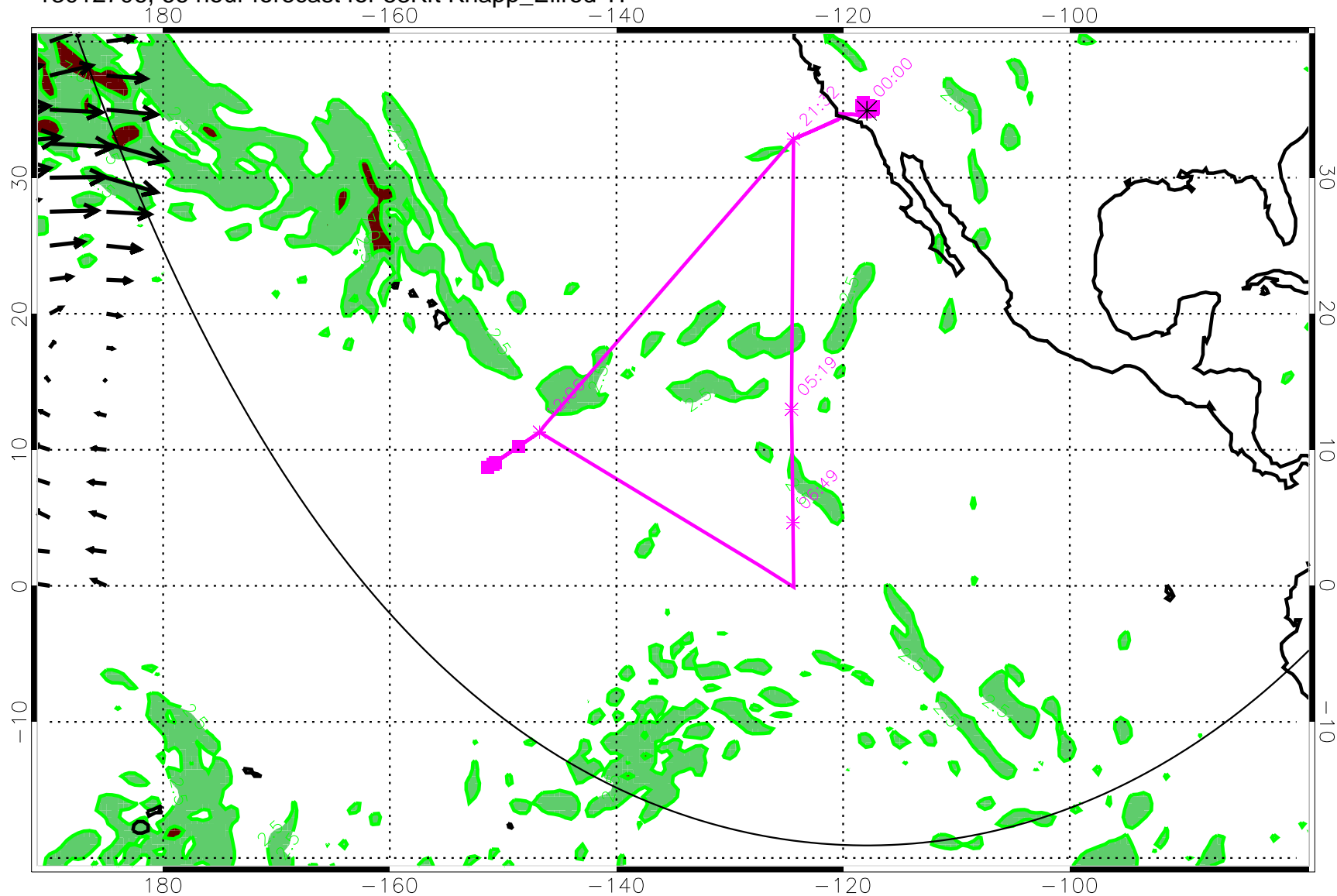
13012706, 66 hour forecast for 53Kft Knapp_Ellrod TI
