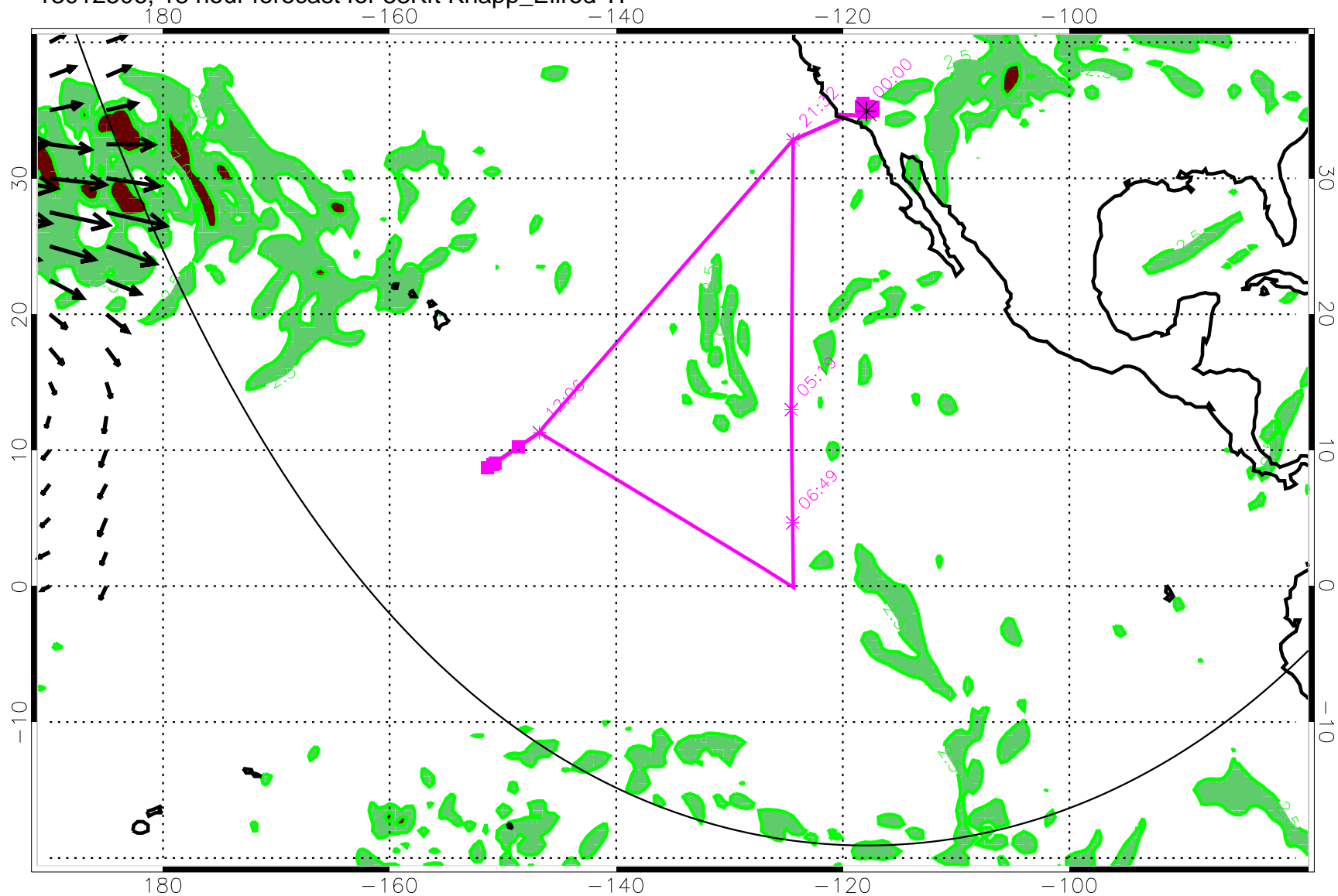
13012506, 18 hour forecast for 53Kft Knapp_Ellrod TI
