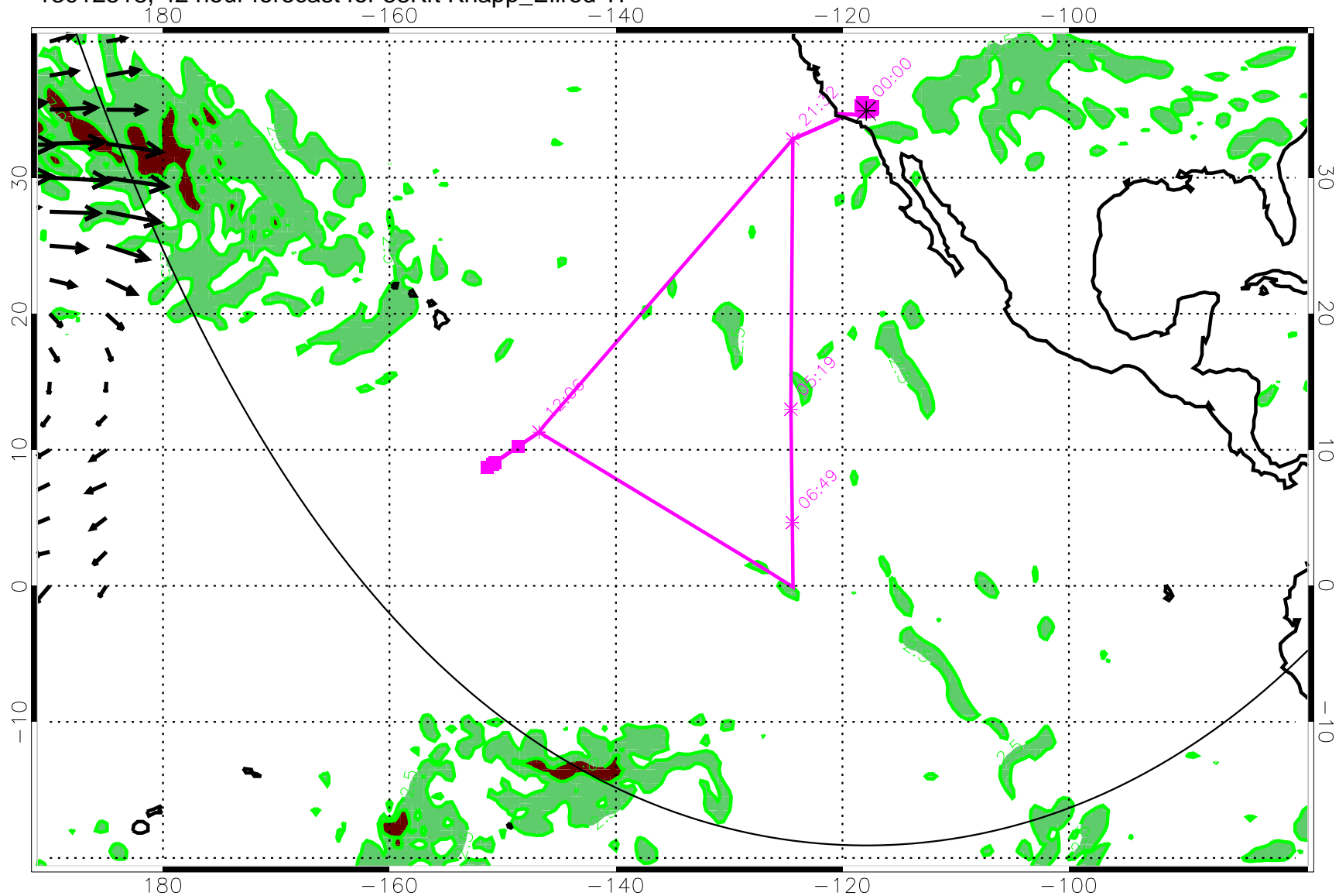
13012518, 42 hour forecast for 53Kft Knapp_Ellrod TI
