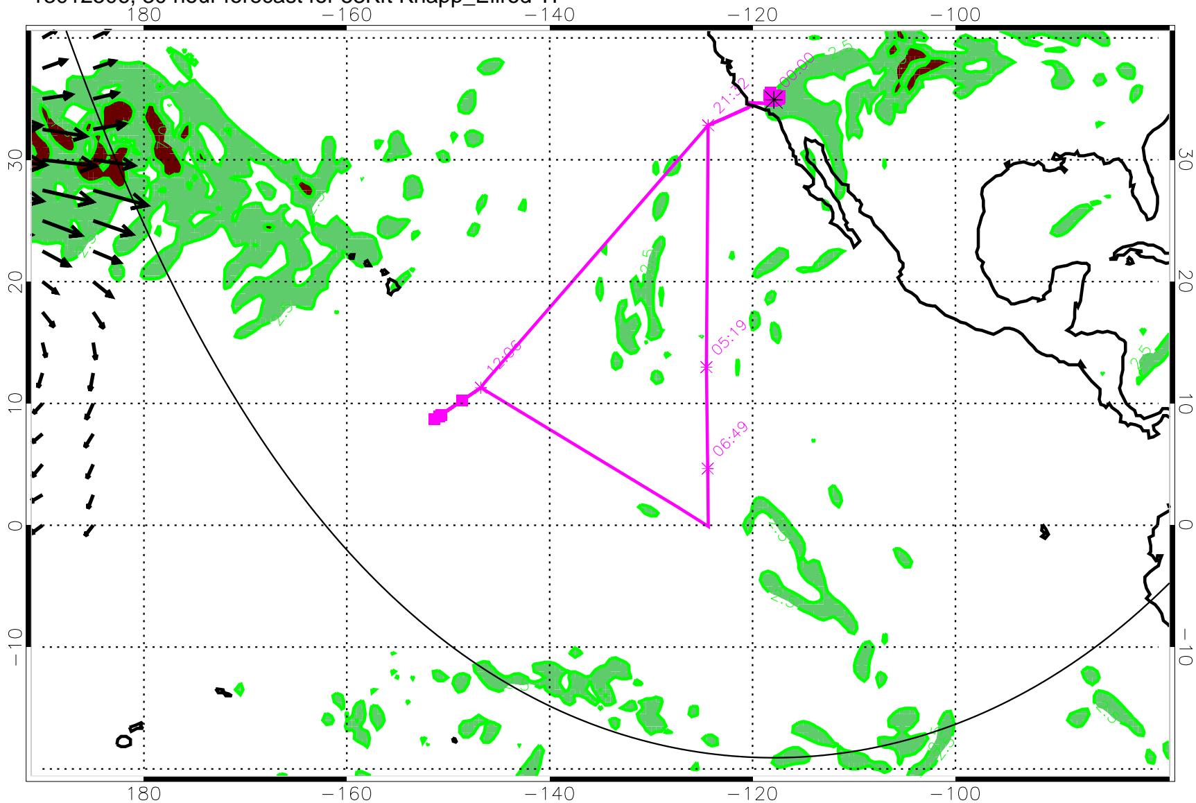
13012506, 30 hour forecast for 53Kft Knapp_Ellrod TI
