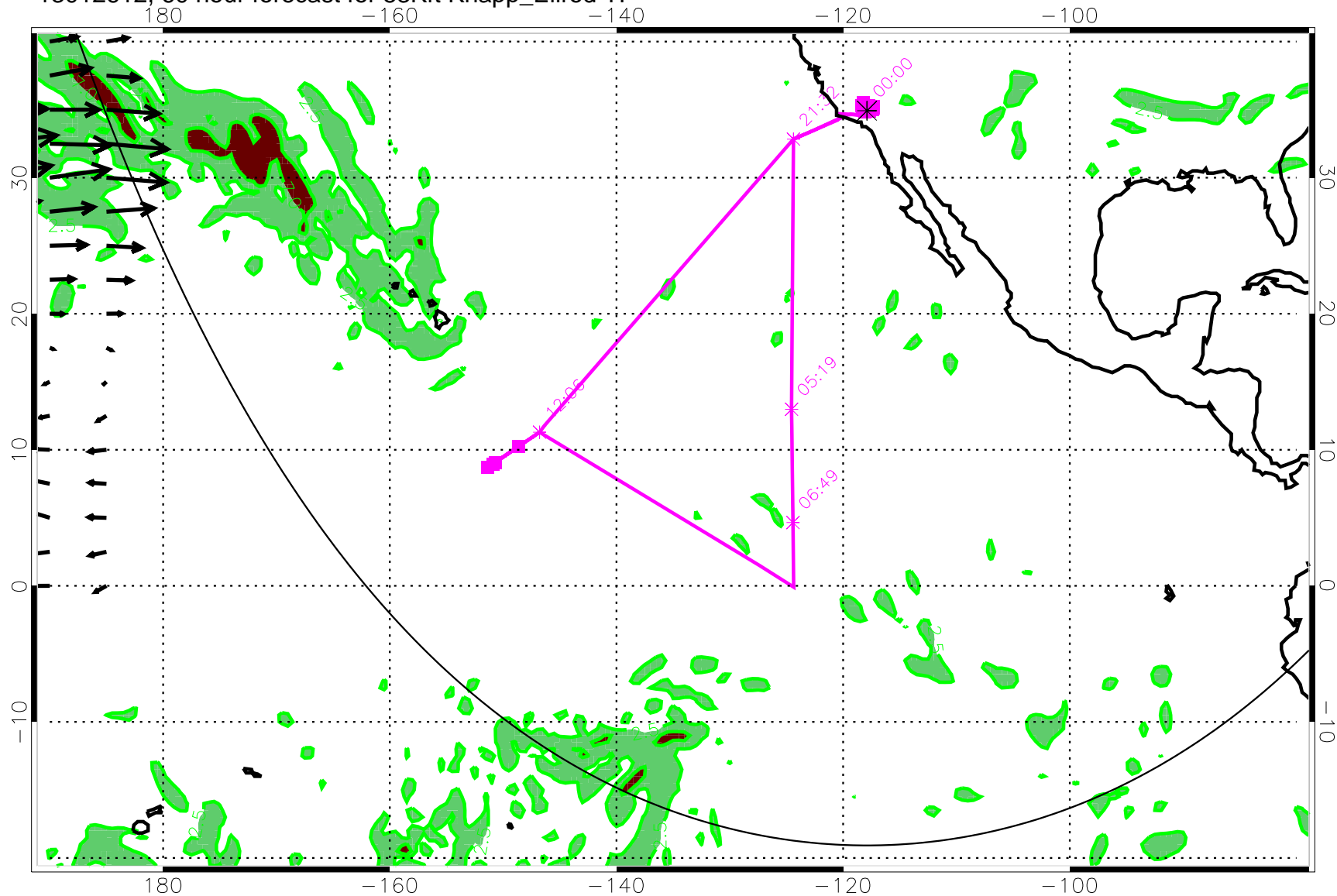
13012612, 60 hour forecast for 53Kft Knapp_Ellrod TI
