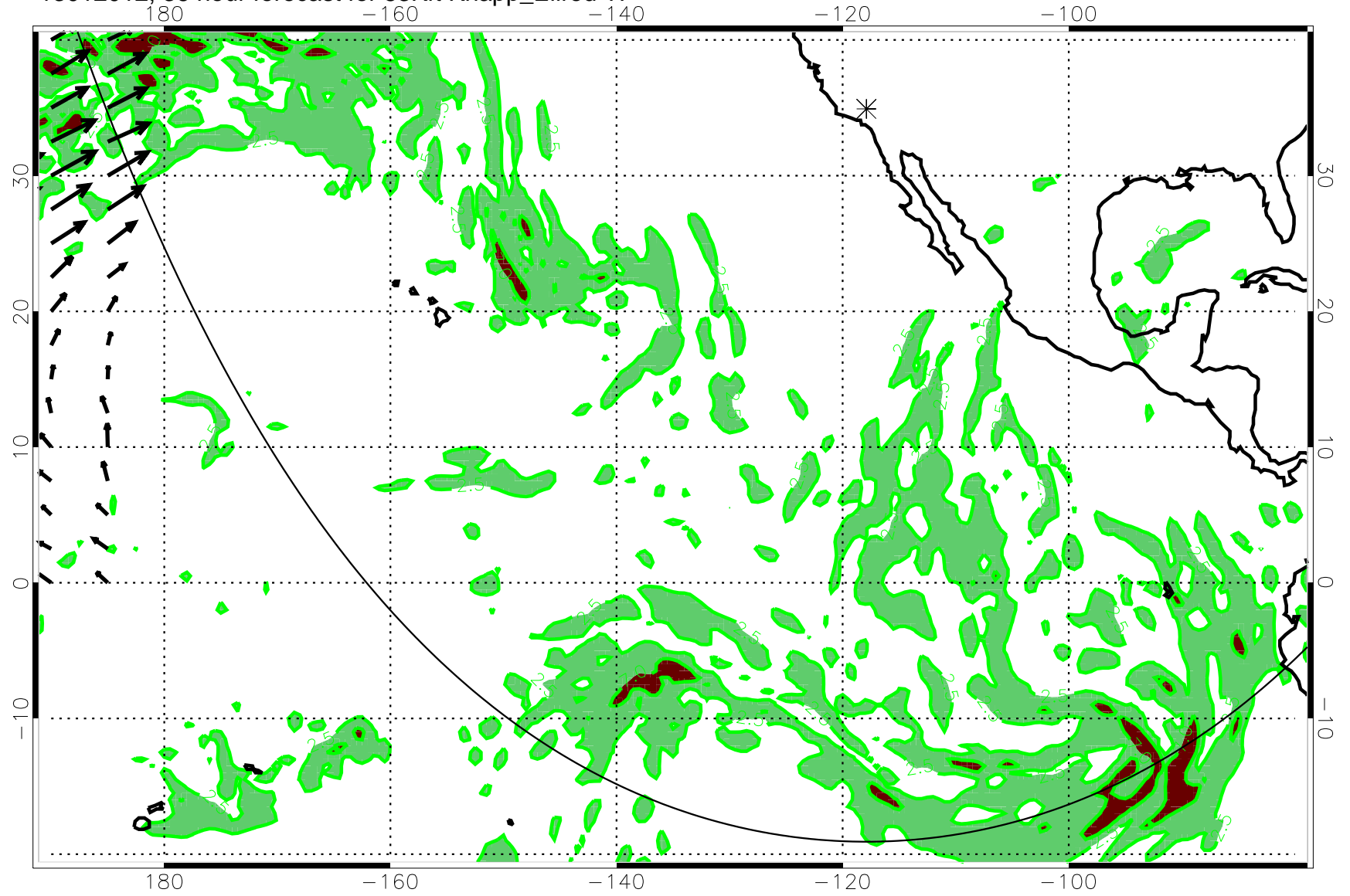
13012012, 36 hour forecast for 53Kft Knapp_Ellrod TI
