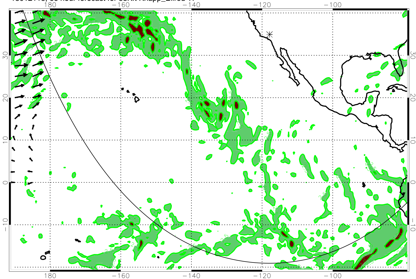
13012118, 66 hour forecast for 53Kft Knapp_Ellrod TI
