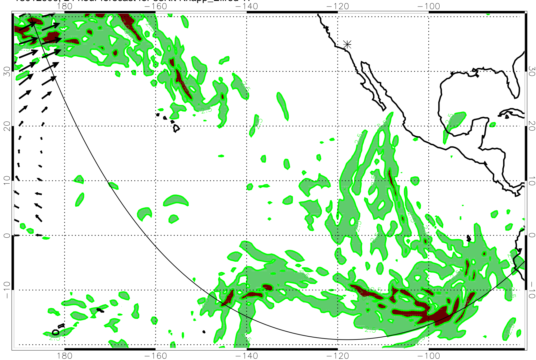
13012000, 24 hour forecast for 53Kft Knapp_Ellrod TI
