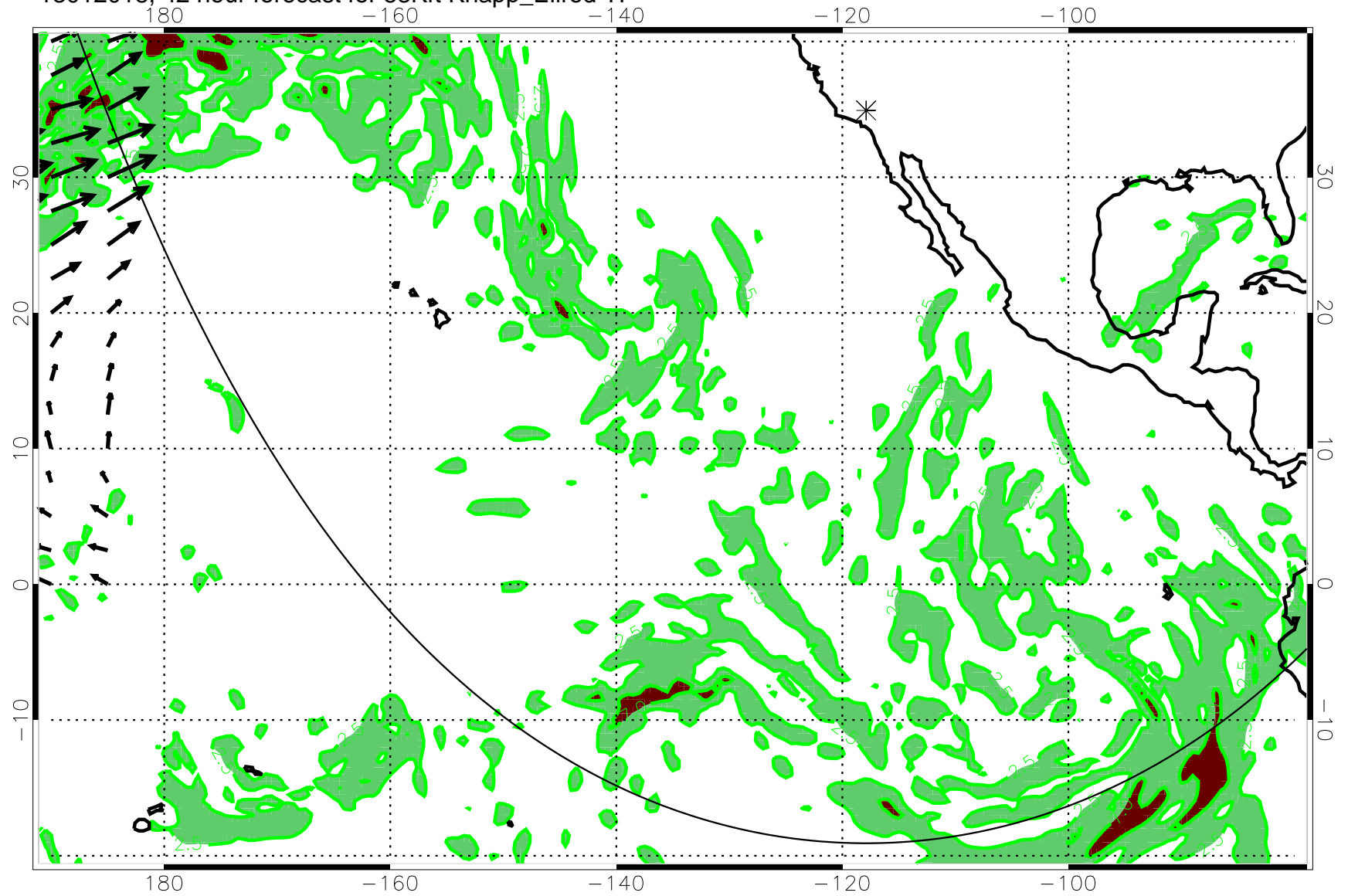
13012018, 42 hour forecast for 53Kft Knapp_Ellrod TI
