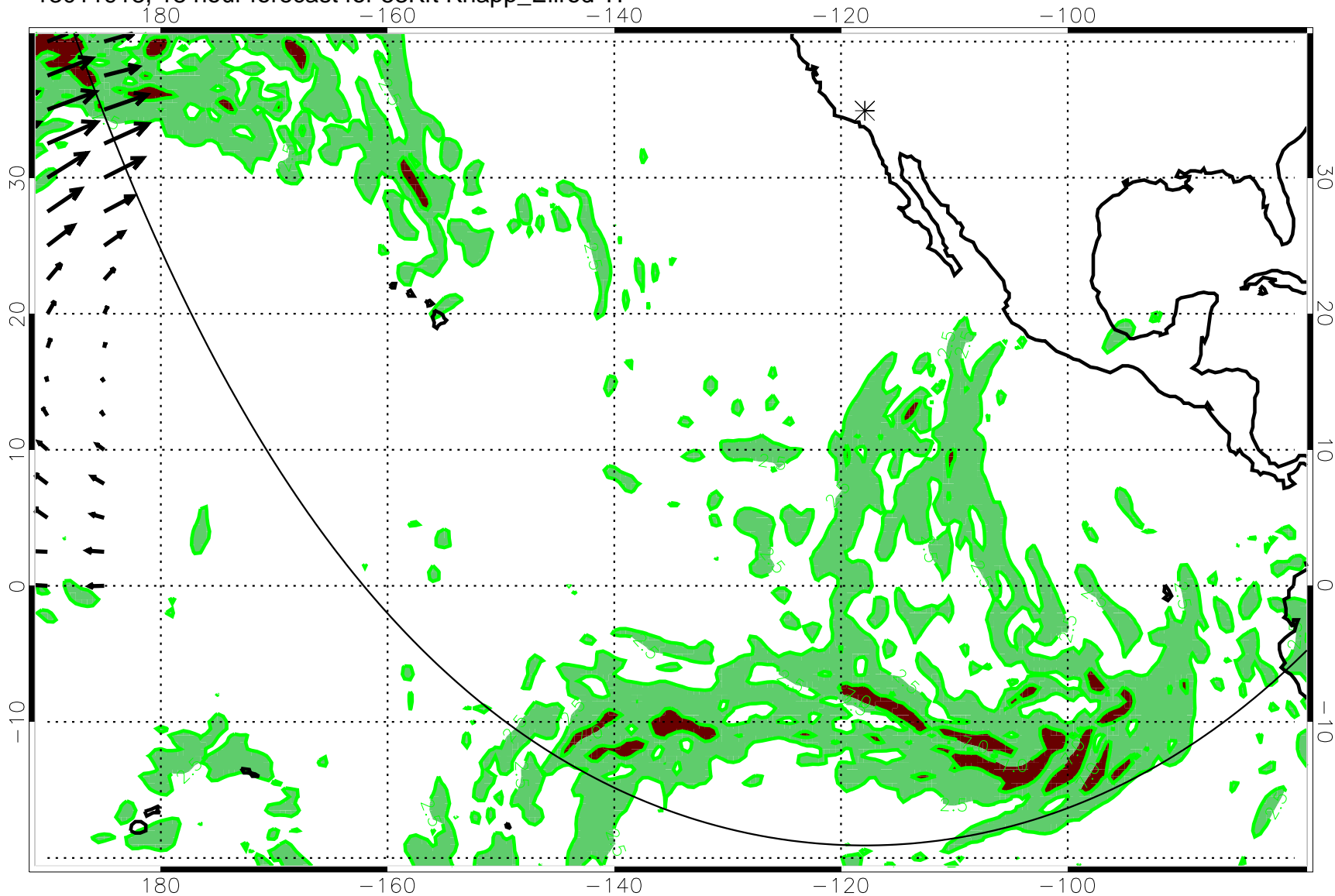
13011918, 18 hour forecast for 53Kft Knapp_Ellrod TI
