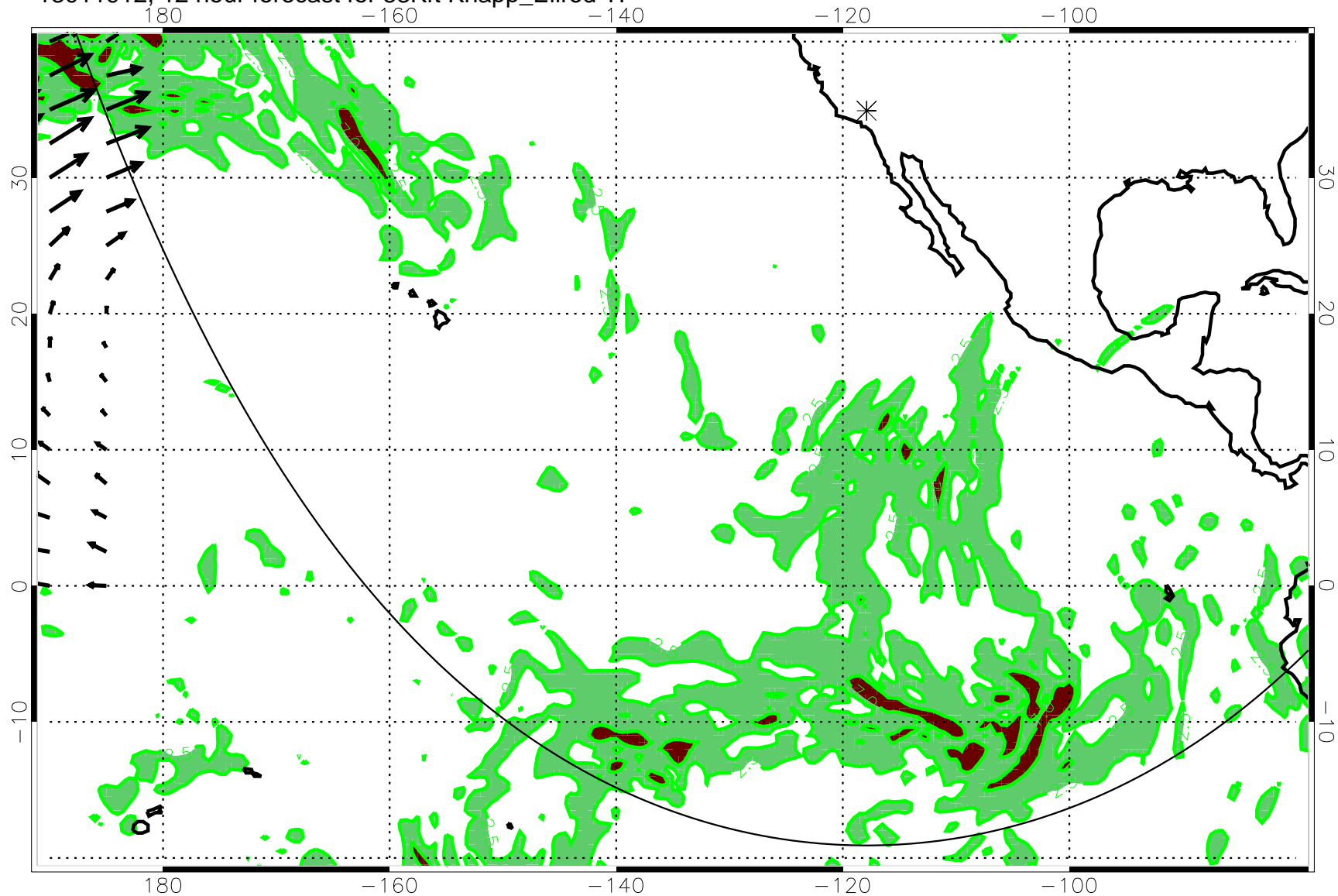
13011912, 12 hour forecast for 53Kft Knapp_Ellrod TI
