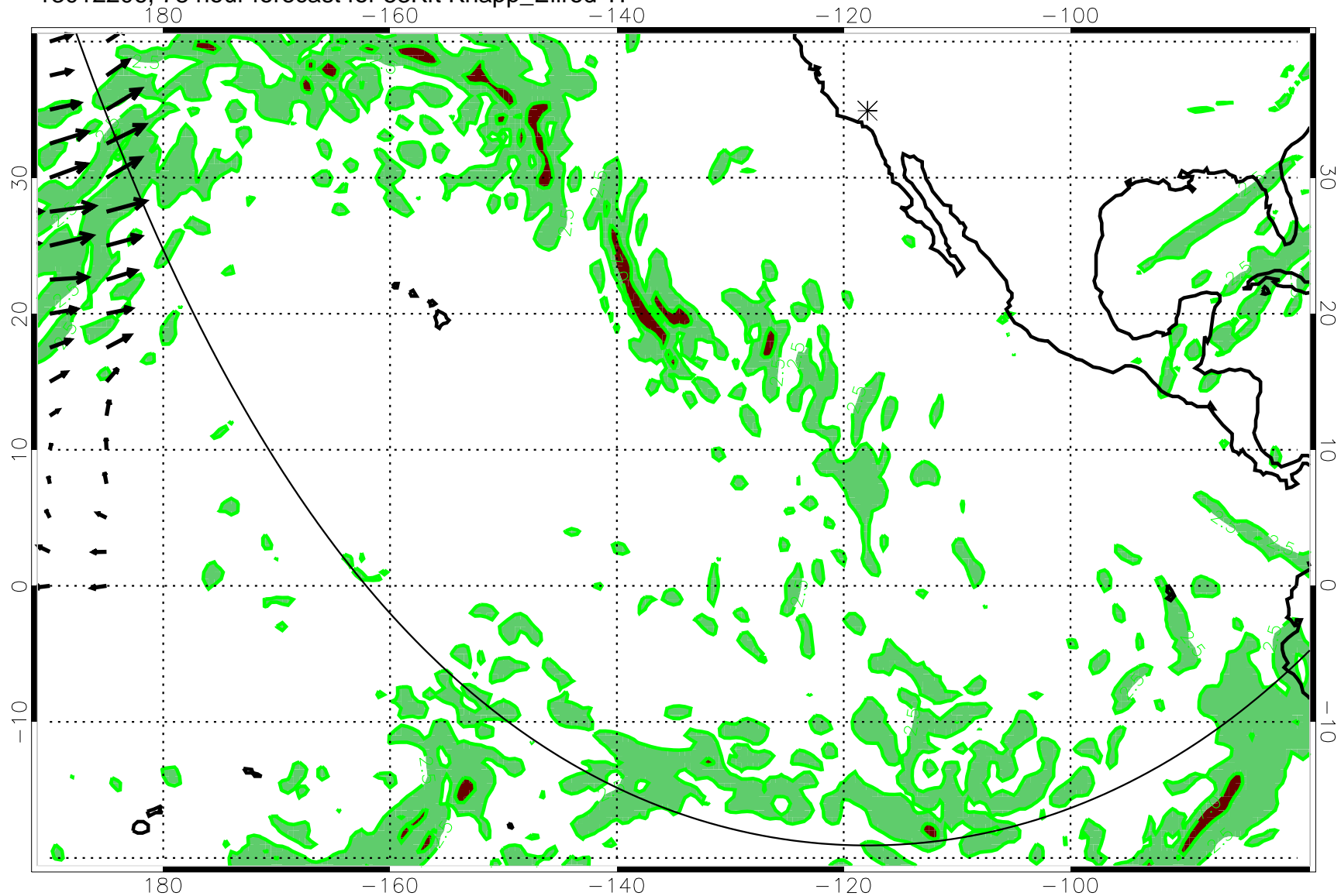
13012206, 78 hour forecast for 53Kft Knapp_Ellrod TI
