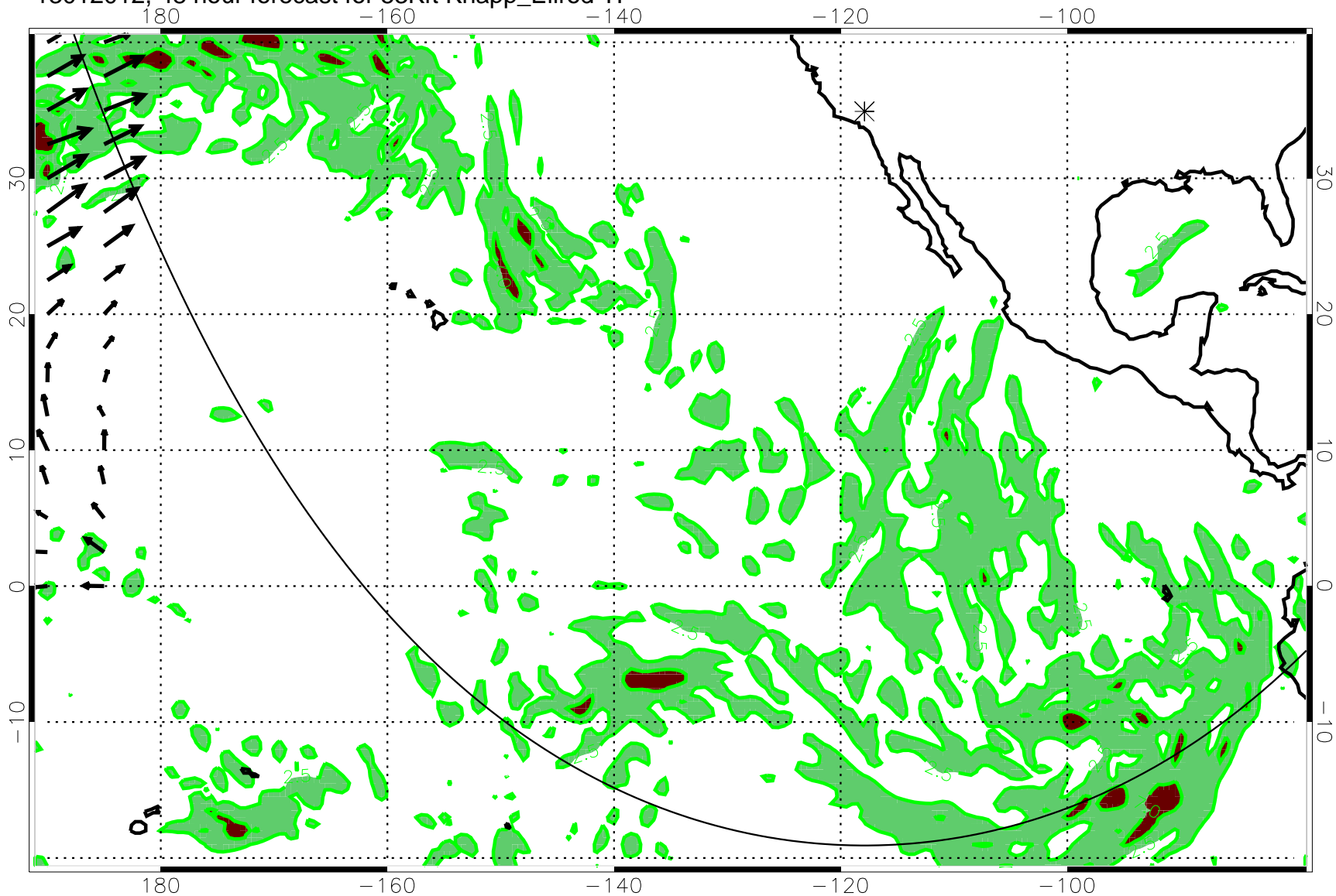
13012012, 48 hour forecast for 53Kft Knapp_Ellrod TI
