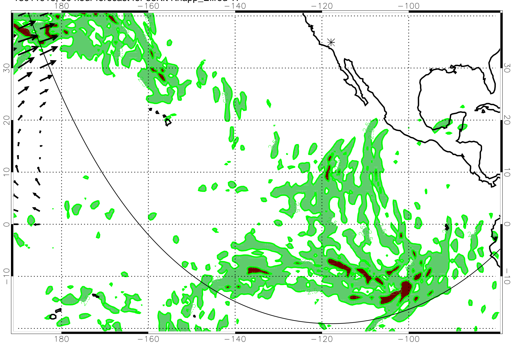
13011918, 30 hour forecast for 53Kft Knapp_Ellrod TI
