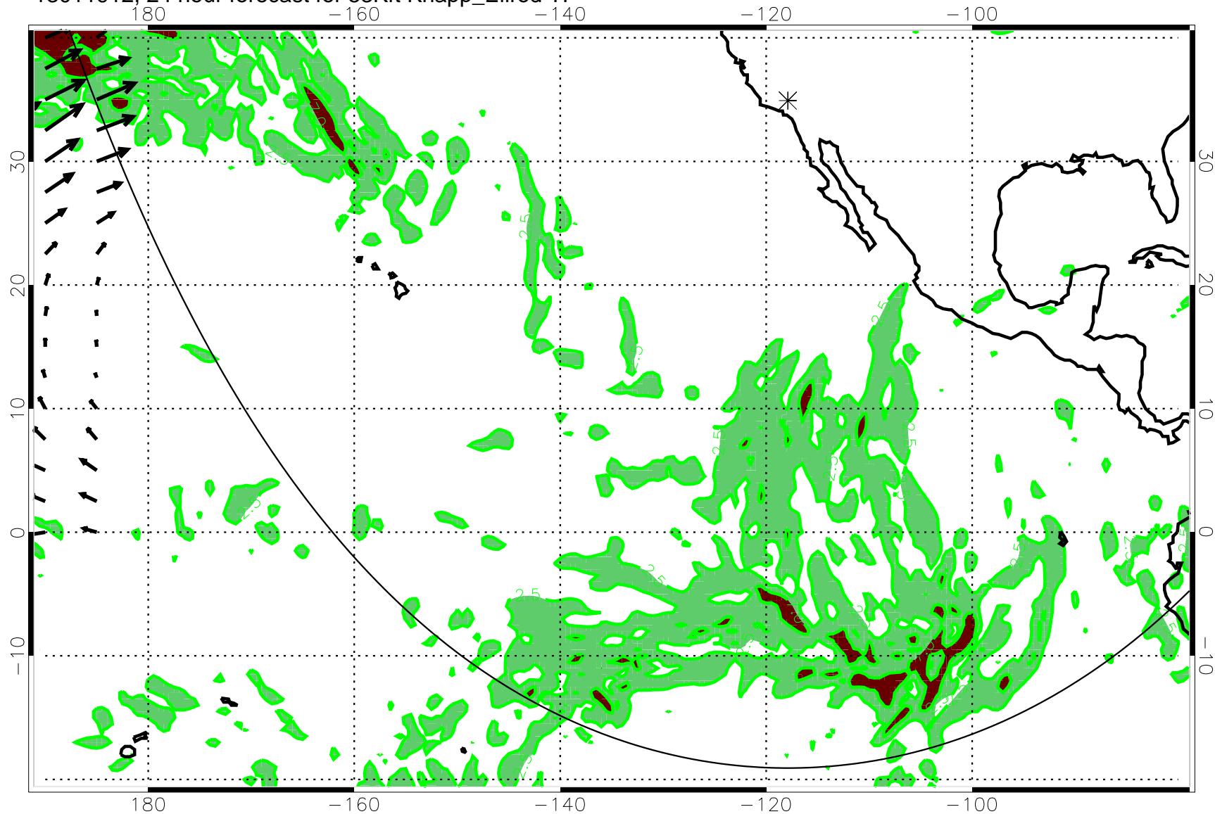
13011912, 24 hour forecast for 53Kft Knapp_Ellrod TI
