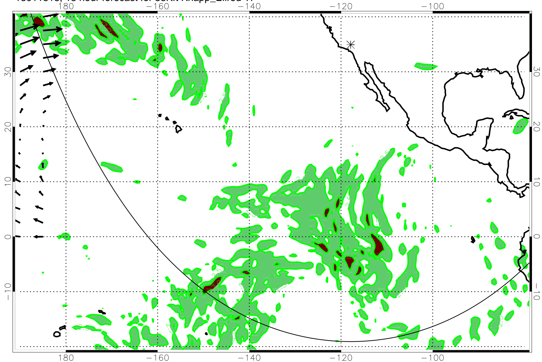
13011818, 18 hour forecast for 53Kft Knapp_Ellrod TI
