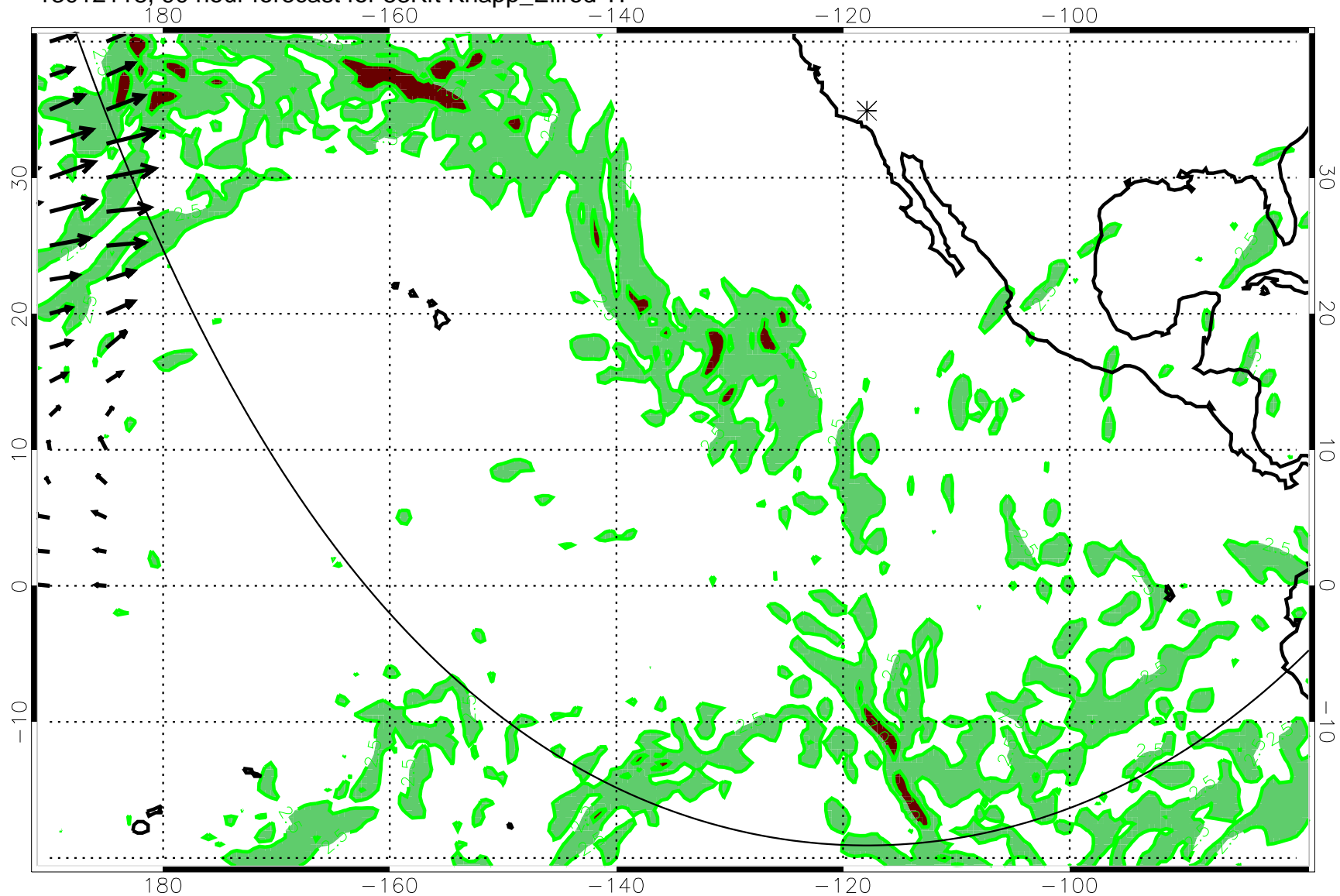
13012118, 90 hour forecast for 53Kft Knapp_Ellrod TI
