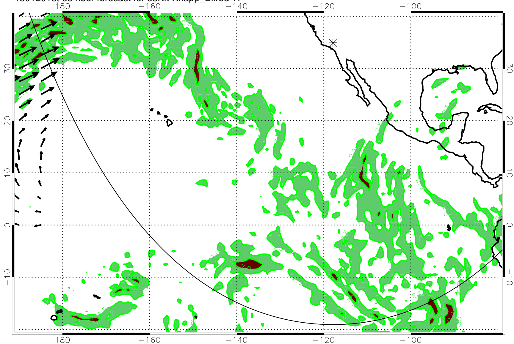
13012018, 66 hour forecast for 53Kft Knapp_Ellrod TI
