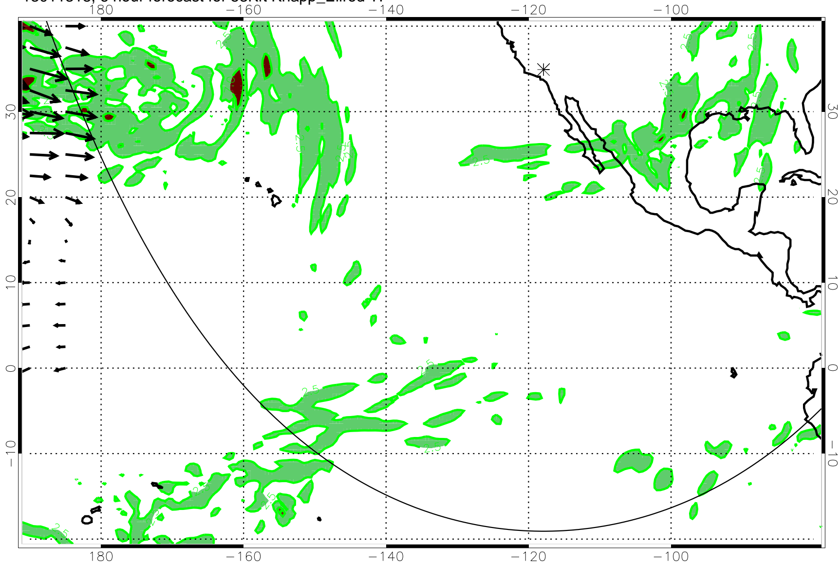
13011318, 6 hour forecast for 53Kft Knapp_Ellrod TI
