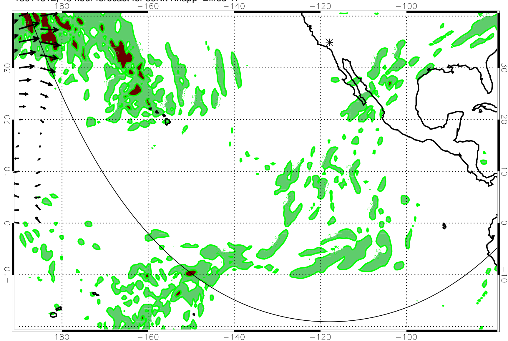
13011512, 48 hour forecast for 53Kft Knapp_Ellrod TI
