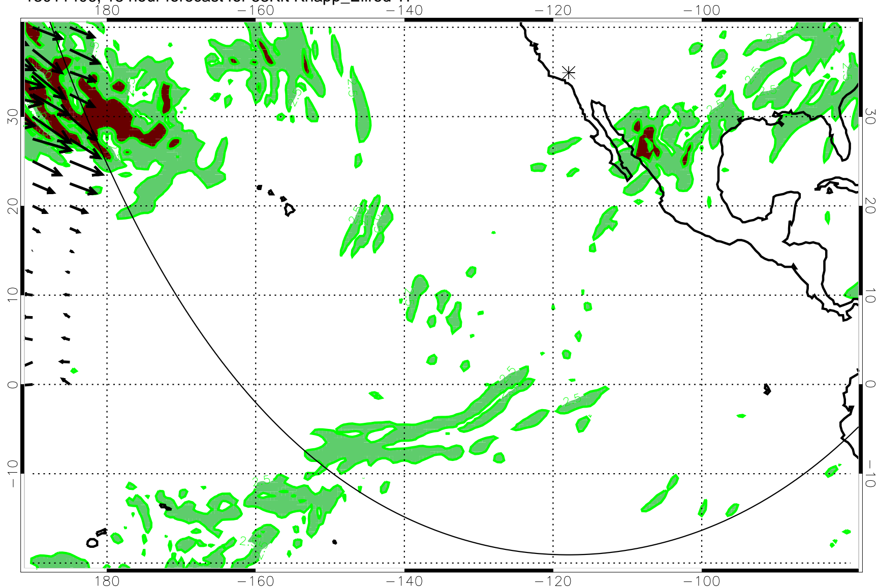
13011406, 18 hour forecast for 53Kft Knapp_Ellrod TI
