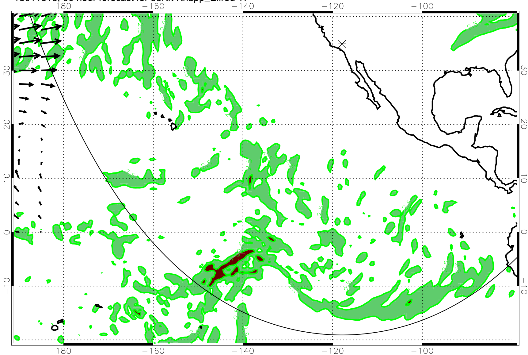
13011618, 90 hour forecast for 53Kft Knapp_Ellrod TI
