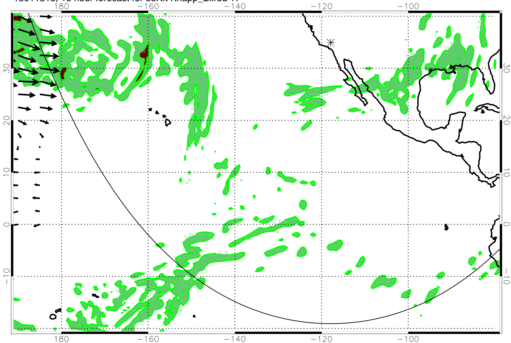
13011318, 18 hour forecast for 53Kft Knapp_Ellrod TI
