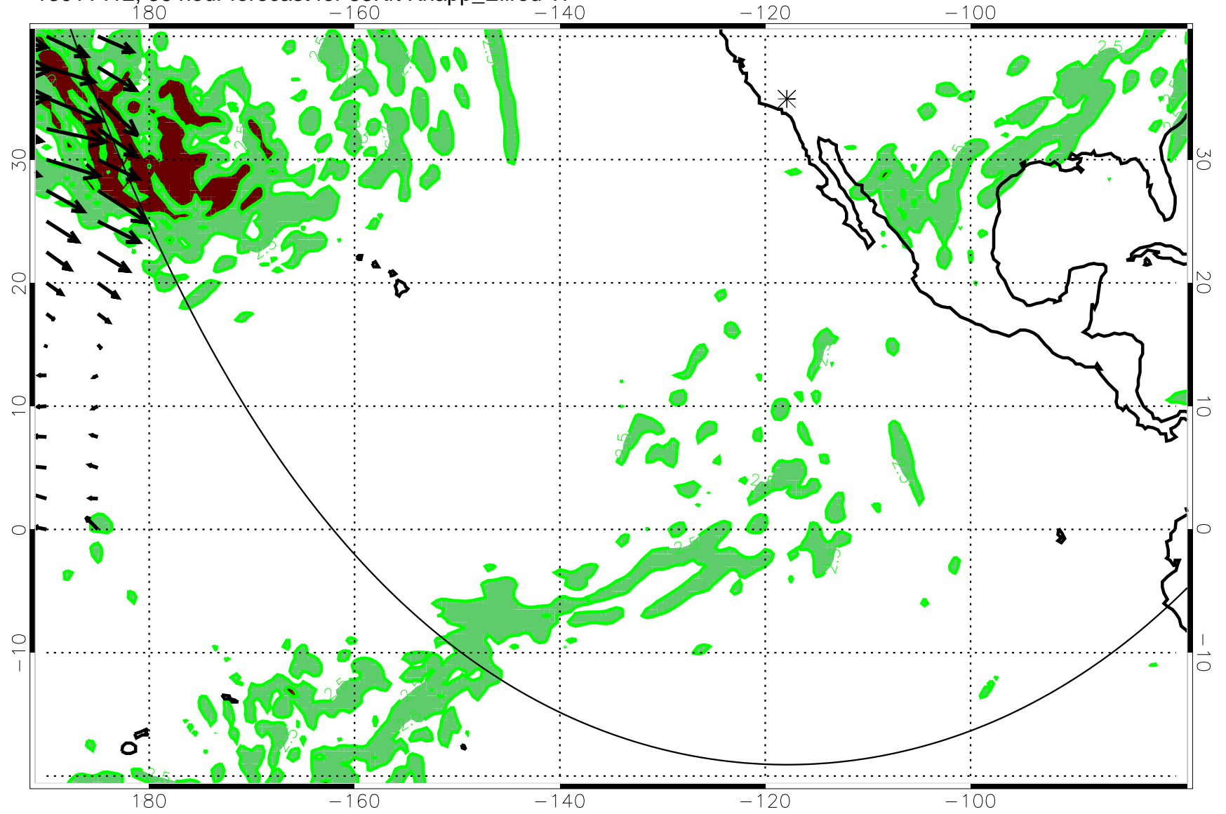
13011412, 36 hour forecast for 53Kft Knapp_Ellrod TI
