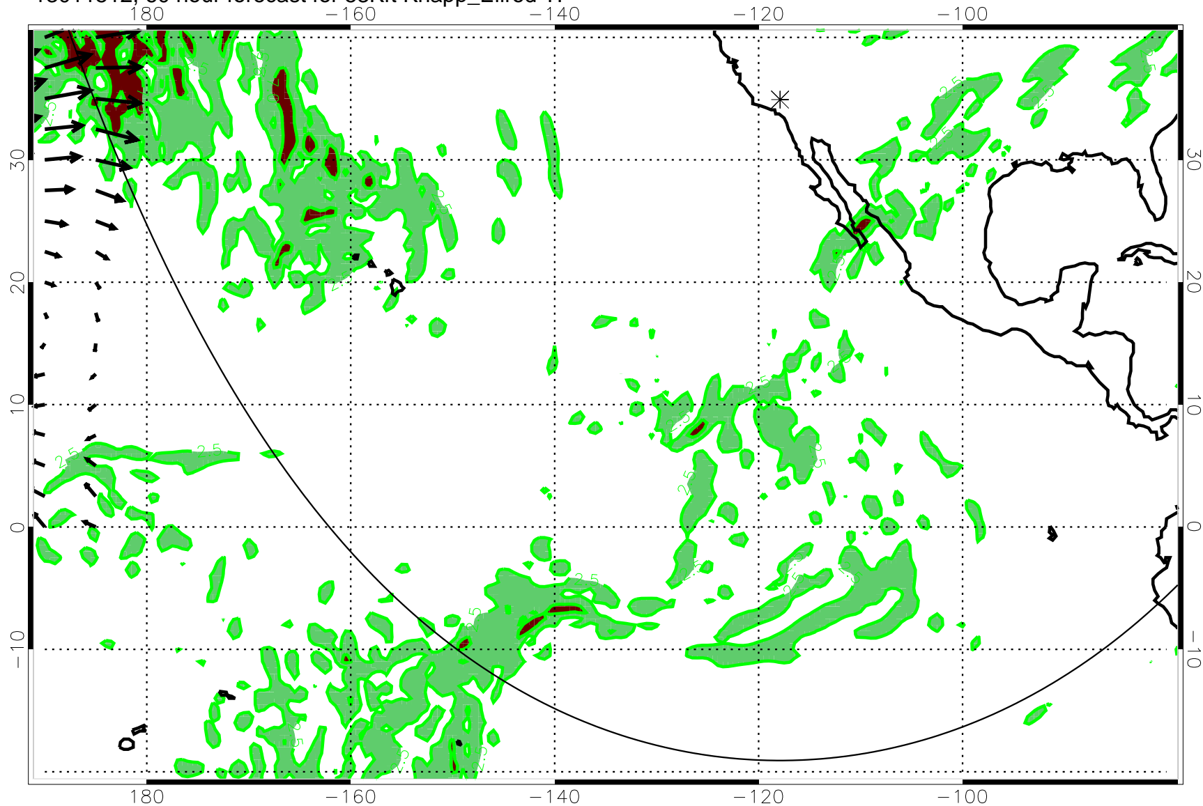
13011512, 60 hour forecast for 53Kft Knapp_Ellrod TI
