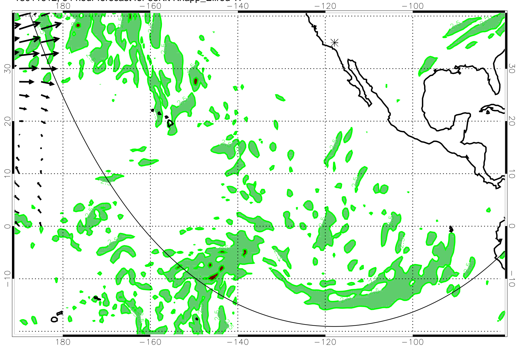
13011612, 84 hour forecast for 53Kft Knapp_Ellrod TI
