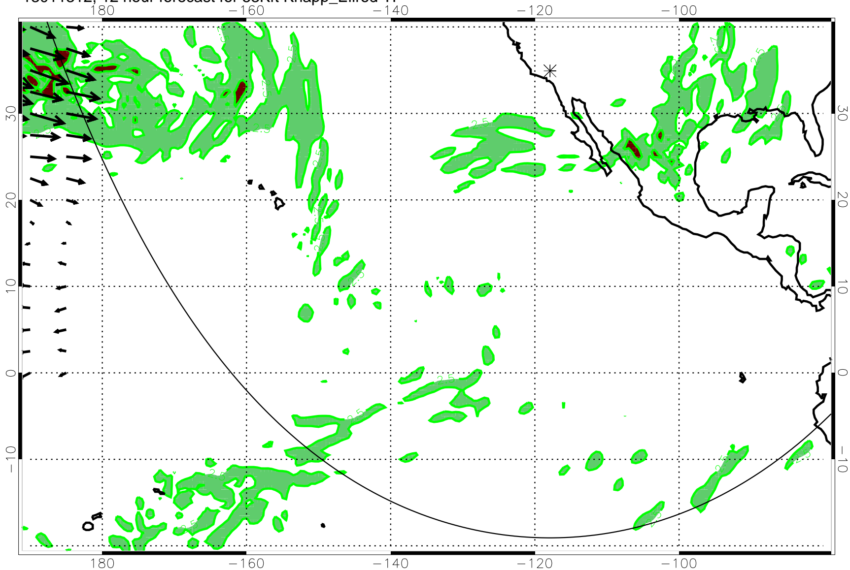
13011312, 12 hour forecast for 53Kft Knapp_Ellrod TI
