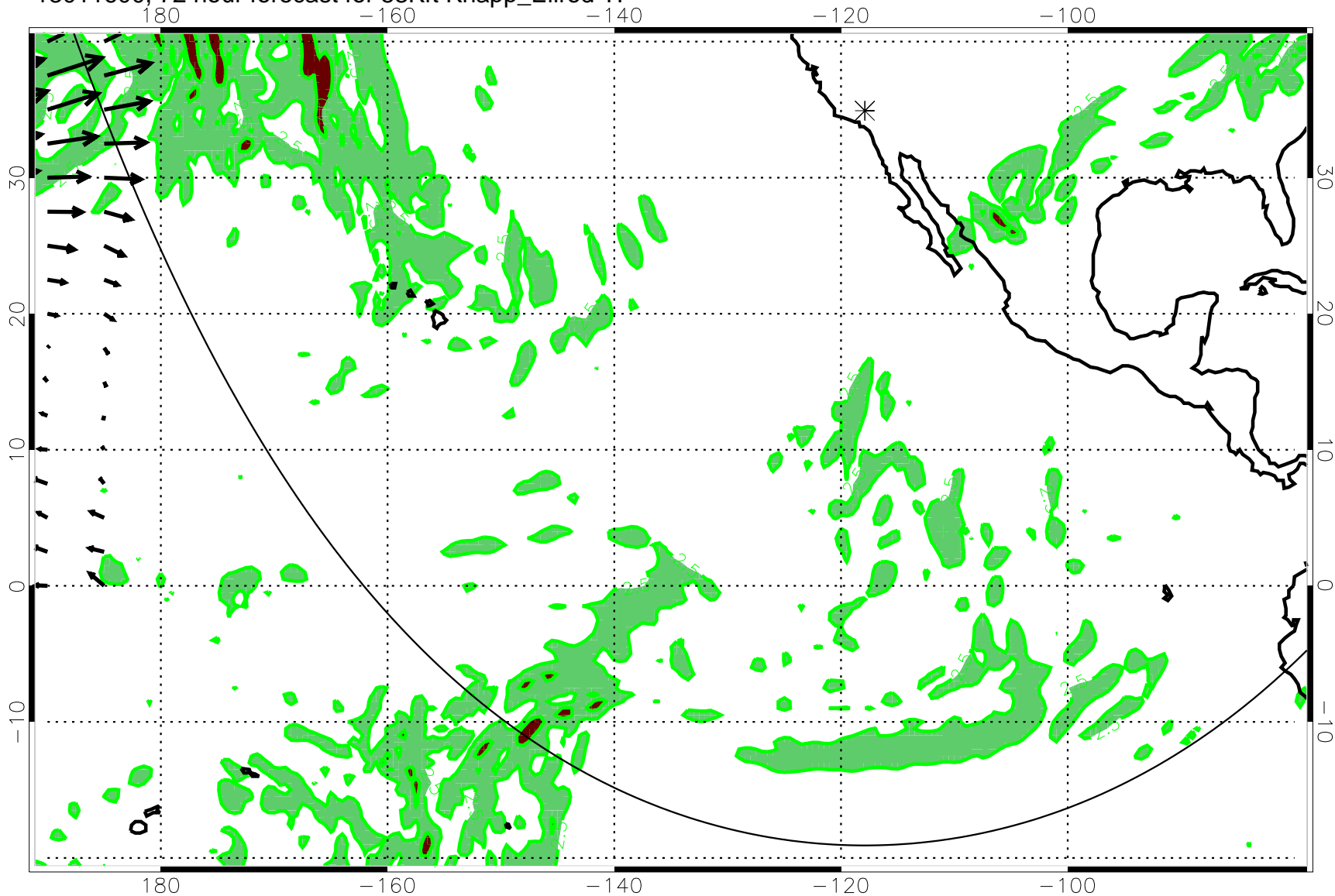
13011600, 72 hour forecast for 53Kft Knapp_Ellrod TI
