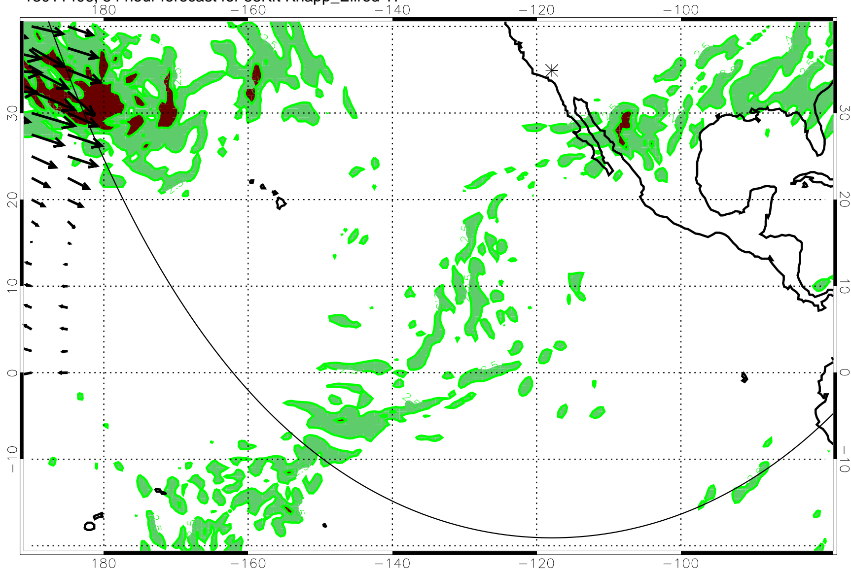
13011406, 54 hour forecast for 53Kft Knapp_Ellrod TI
