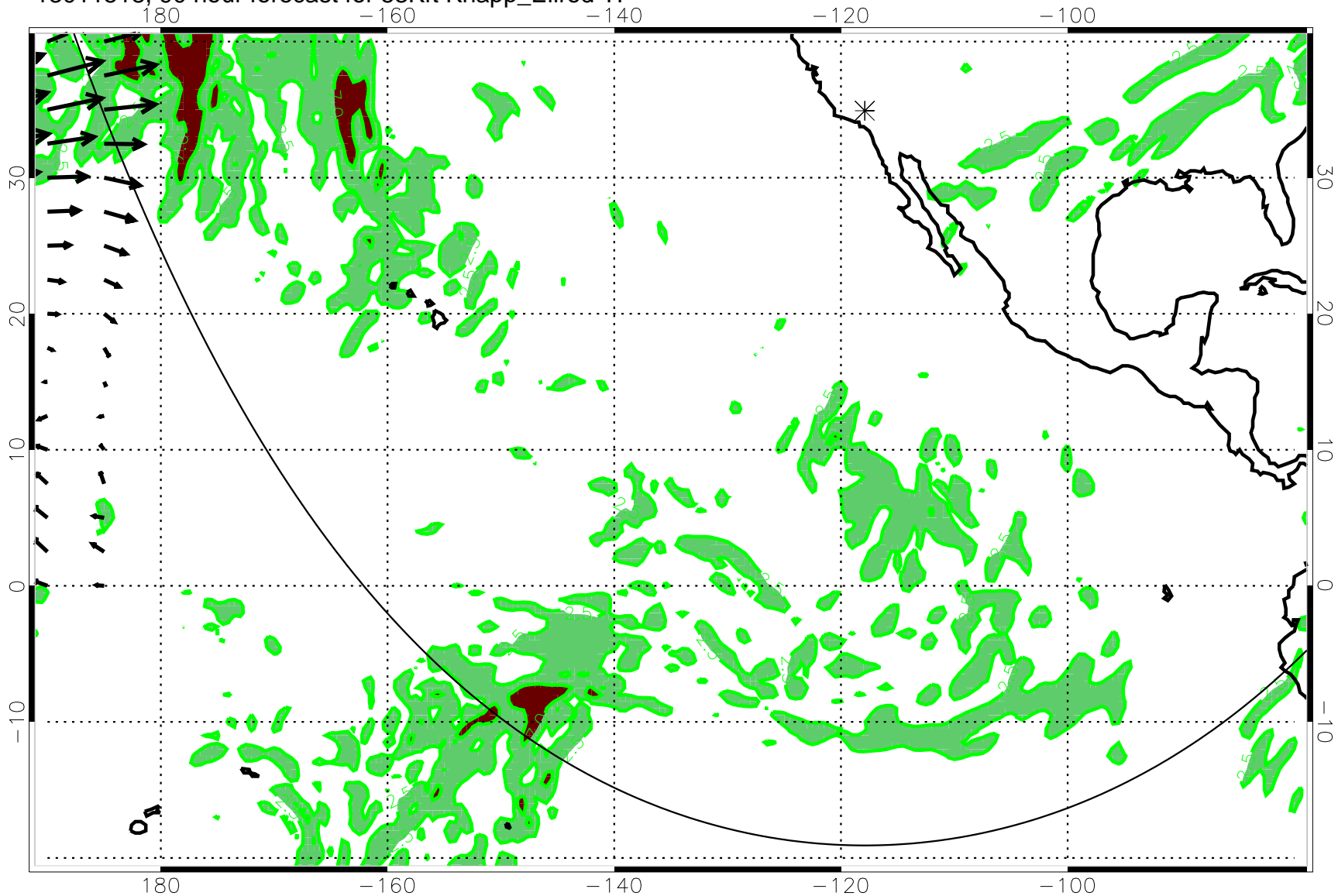
13011518, 90 hour forecast for 53Kft Knapp_Ellrod TI
