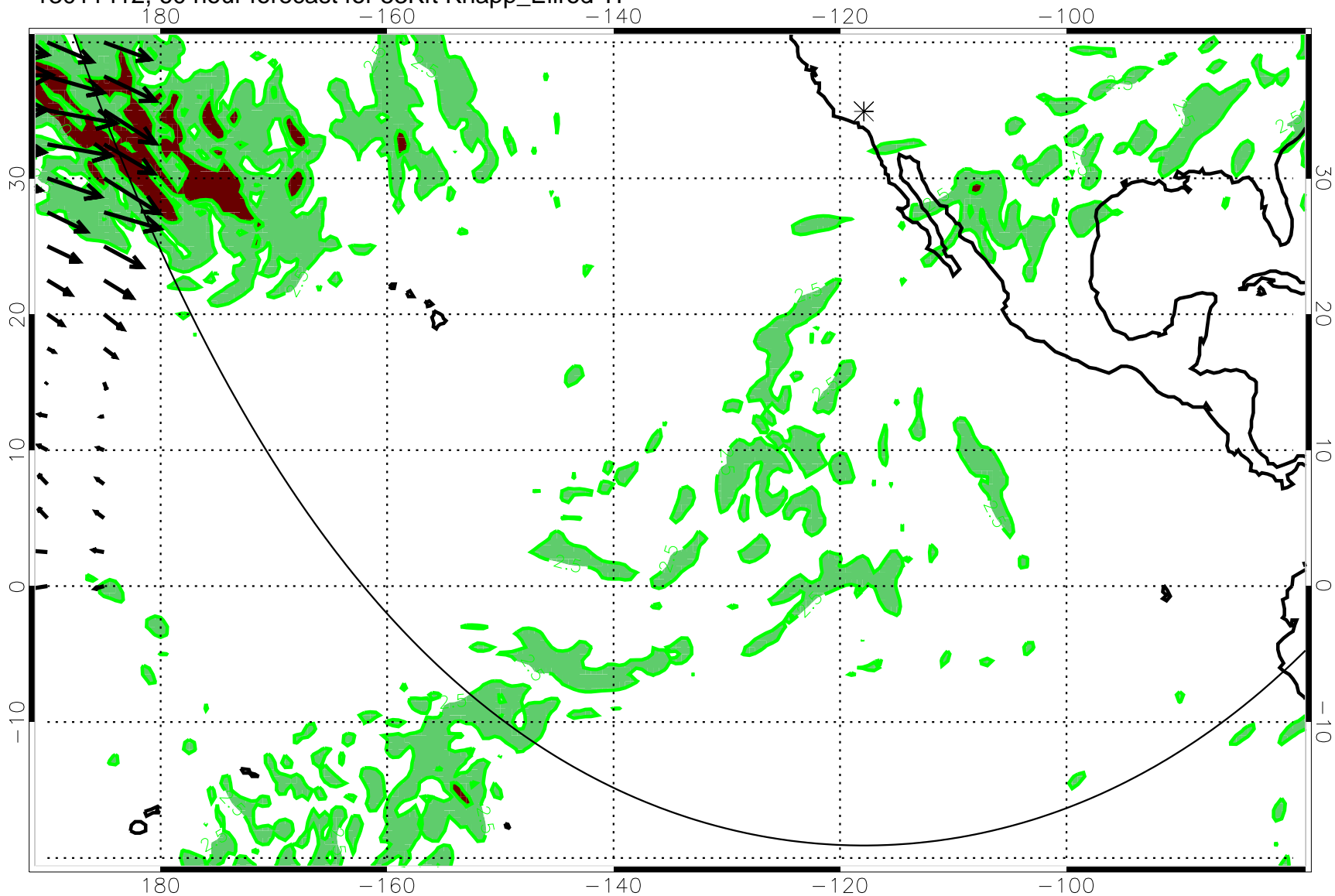
13011412, 60 hour forecast for 53Kft Knapp_Ellrod TI
