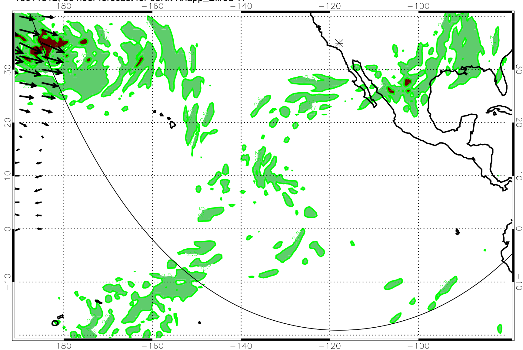
13011312, 36 hour forecast for 53Kft Knapp_Ellrod TI
