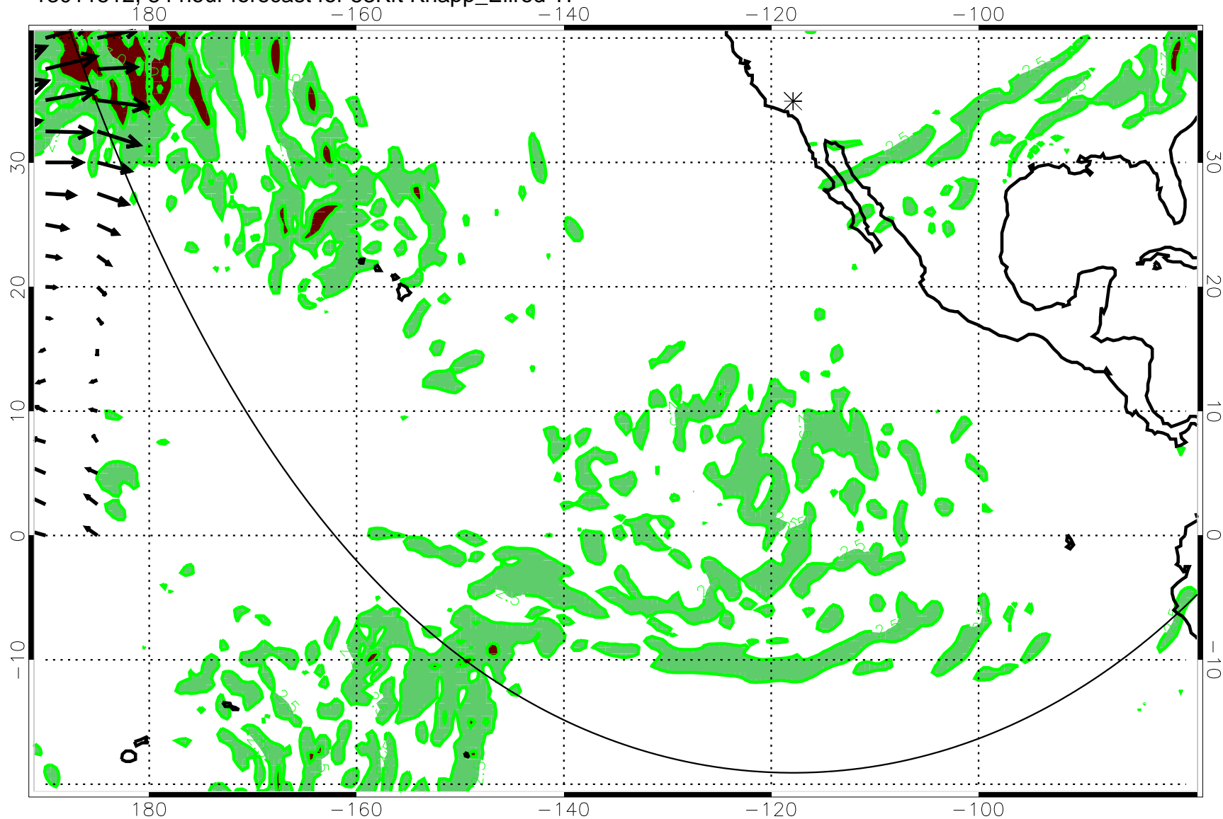
13011512, 84 hour forecast for 53Kft Knapp_Ellrod TI
