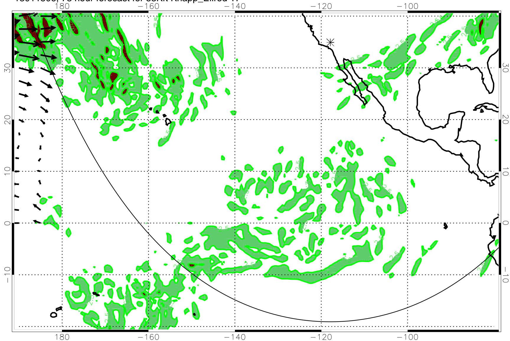
13011506, 78 hour forecast for 53Kft Knapp_Ellrod TI
