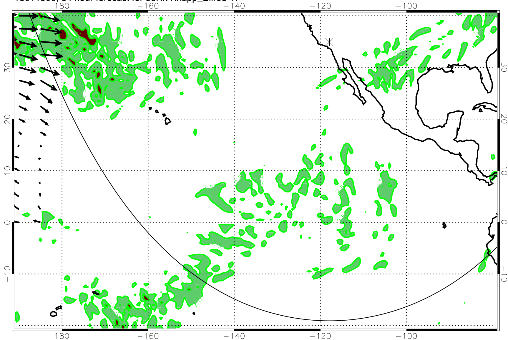
13011500, 84 hour forecast for 53Kft Knapp_Ellrod TI
