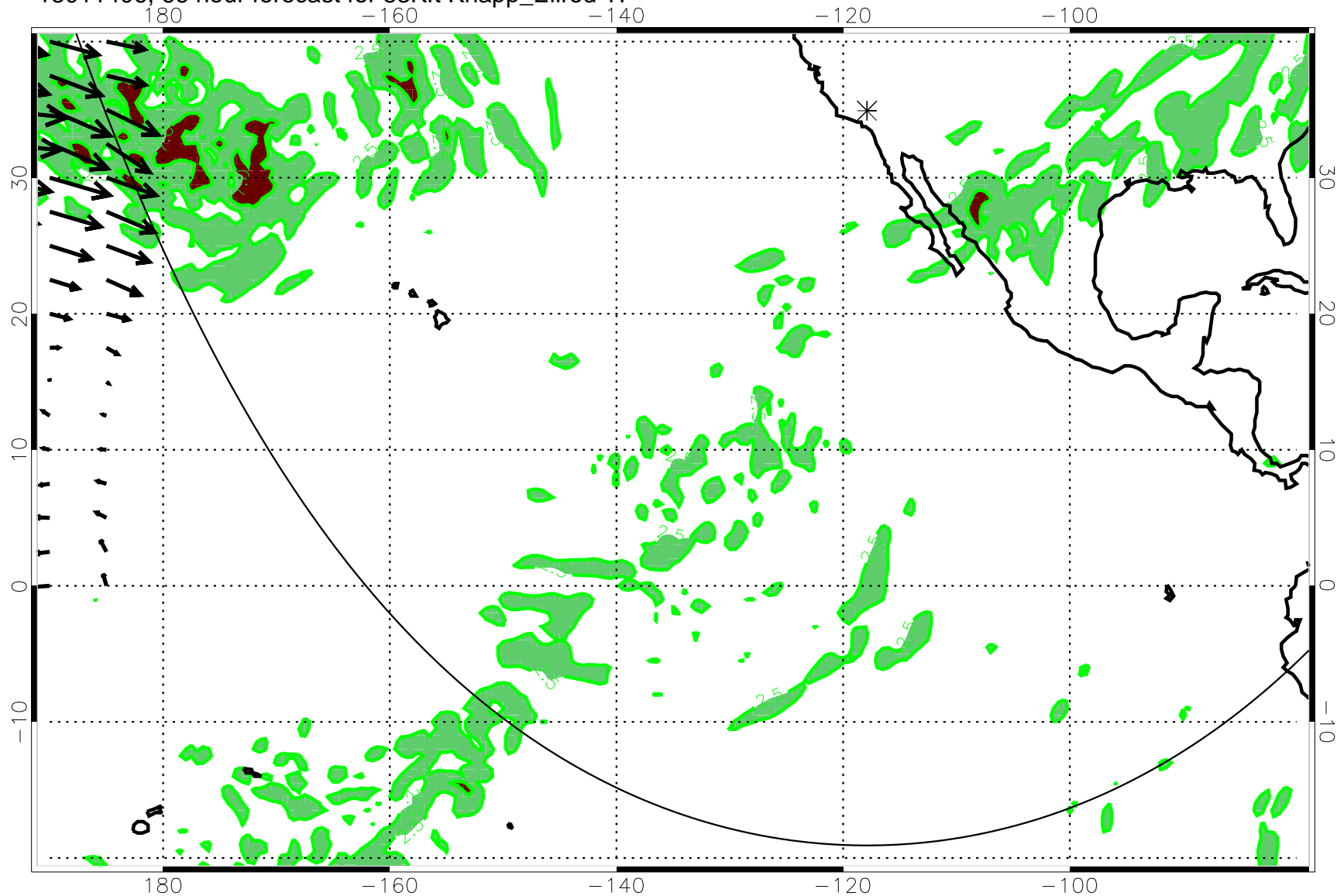
13011406, 66 hour forecast for 53Kft Knapp_Ellrod TI
