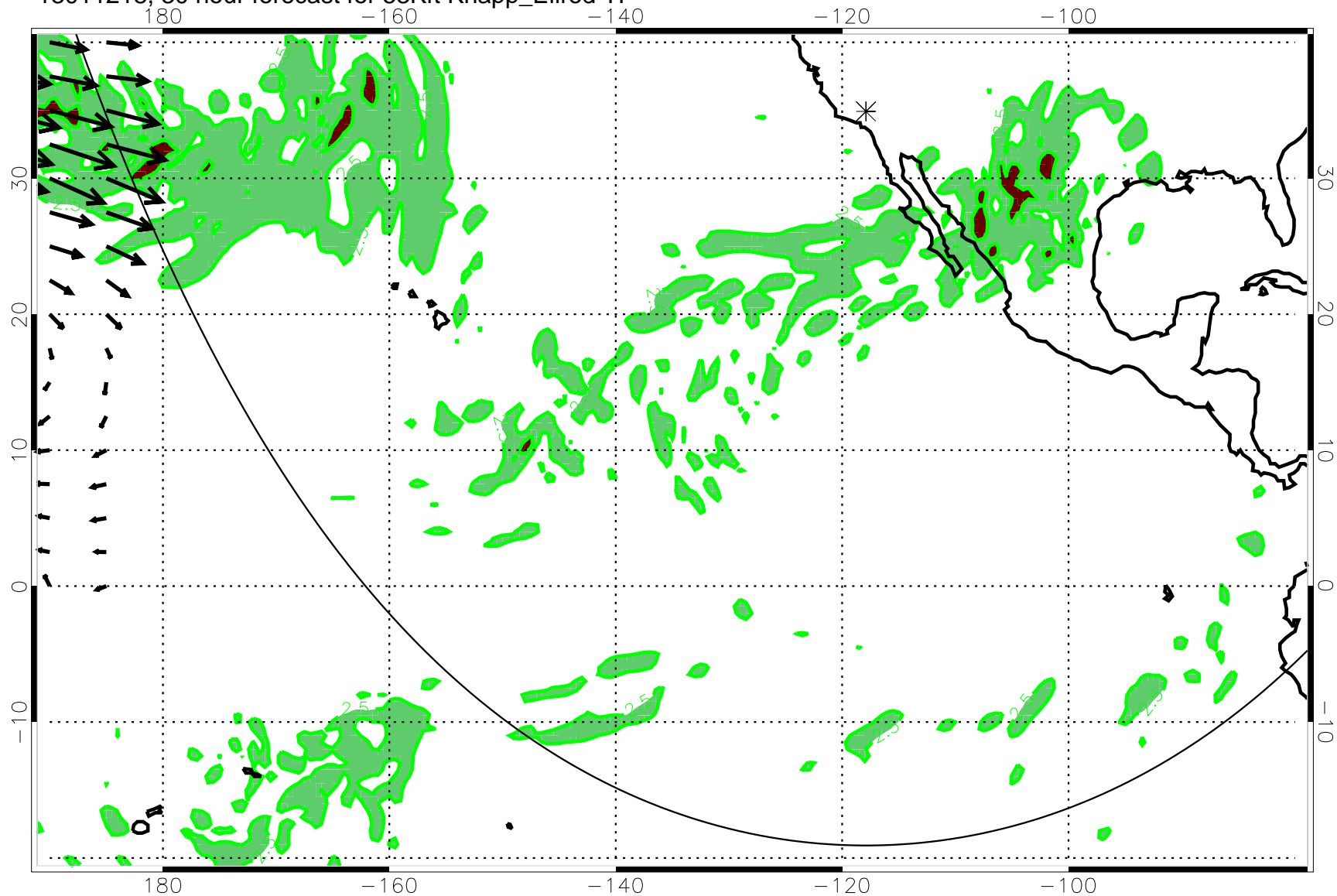
13011218, 30 hour forecast for 53Kft Knapp_Ellrod TI
