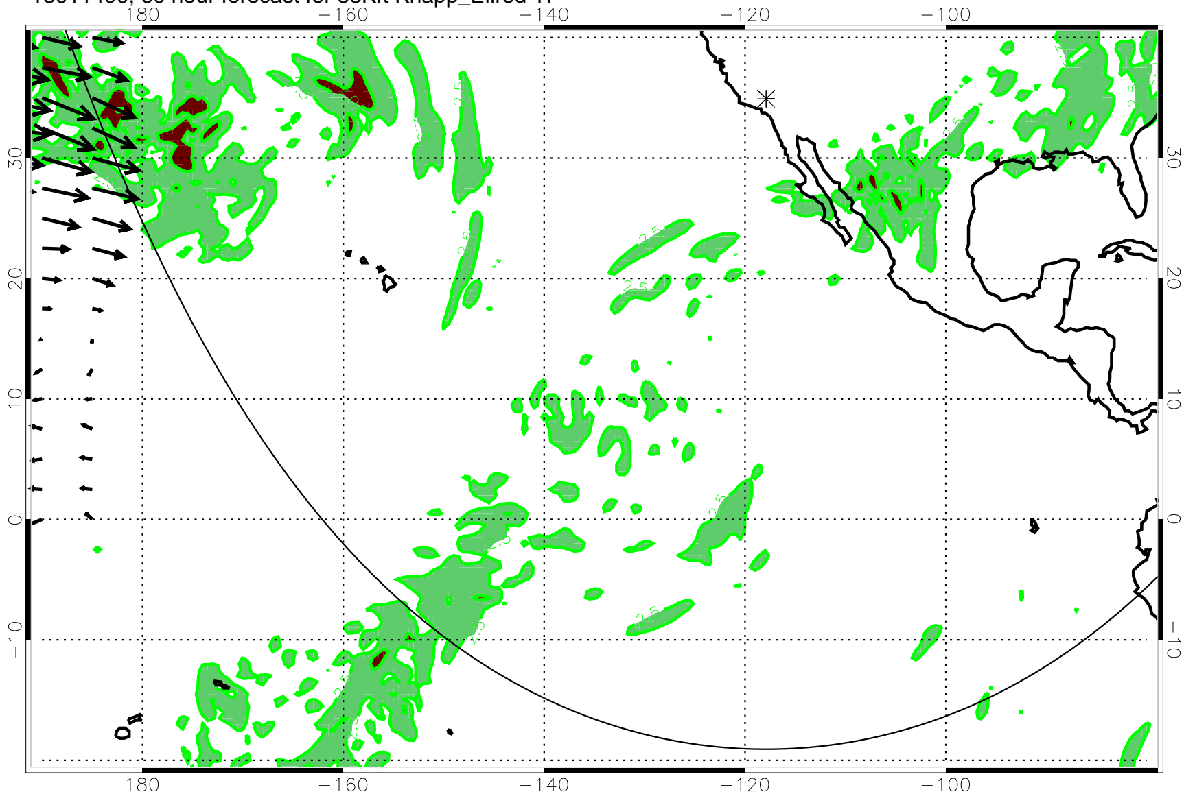
13011400, 60 hour forecast for 53Kft Knapp_Ellrod TI
