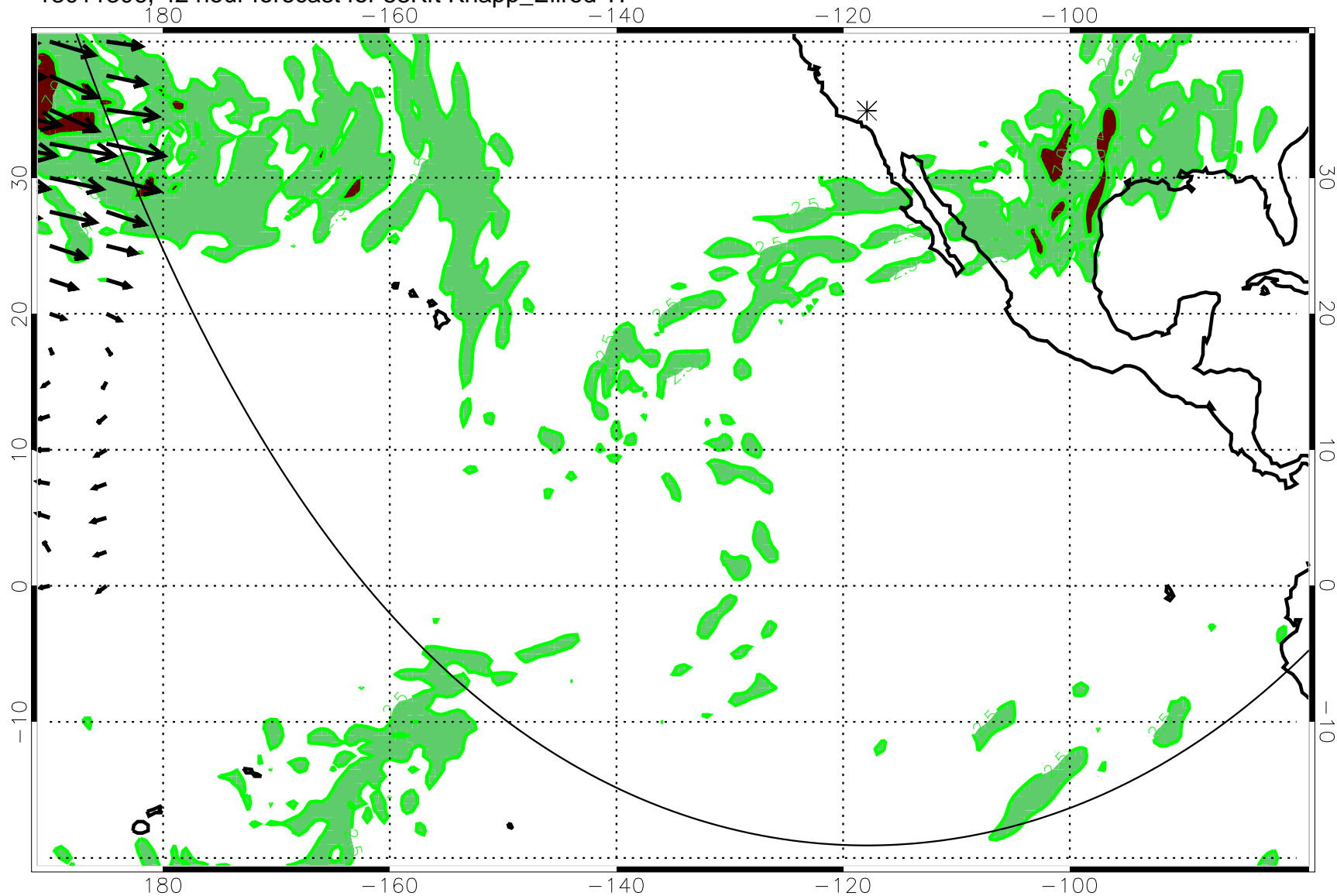
13011306, 42 hour forecast for 53Kft Knapp_Ellrod TI
