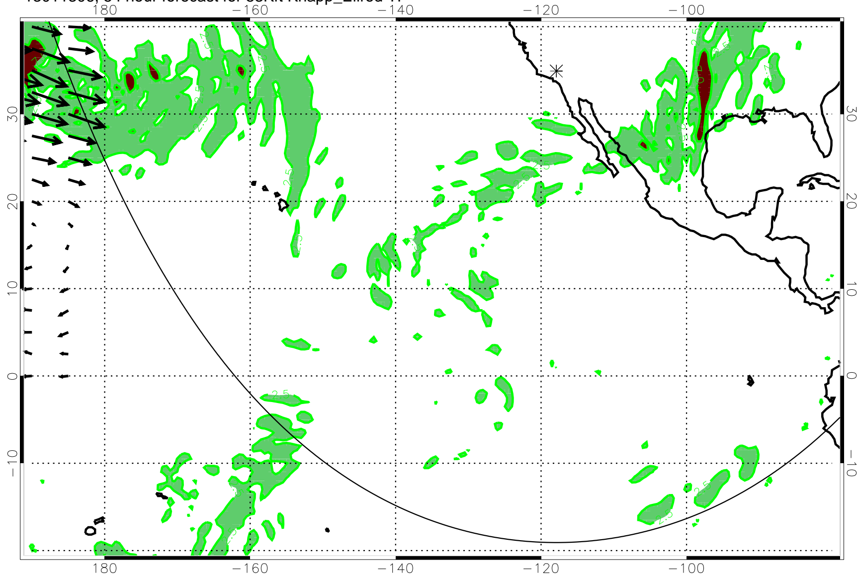
13011306, 54 hour forecast for 53Kft Knapp_Ellrod TI
