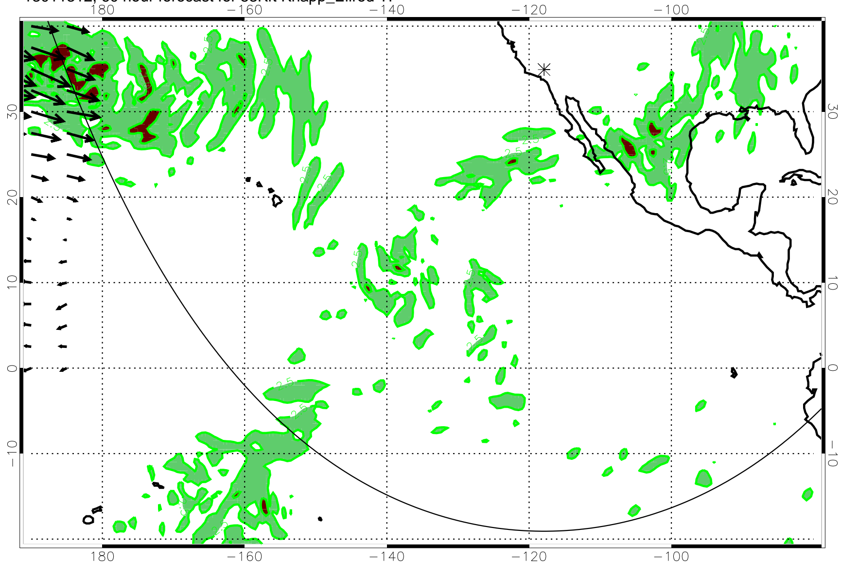
13011312, 60 hour forecast for 53Kft Knapp_Ellrod TI
