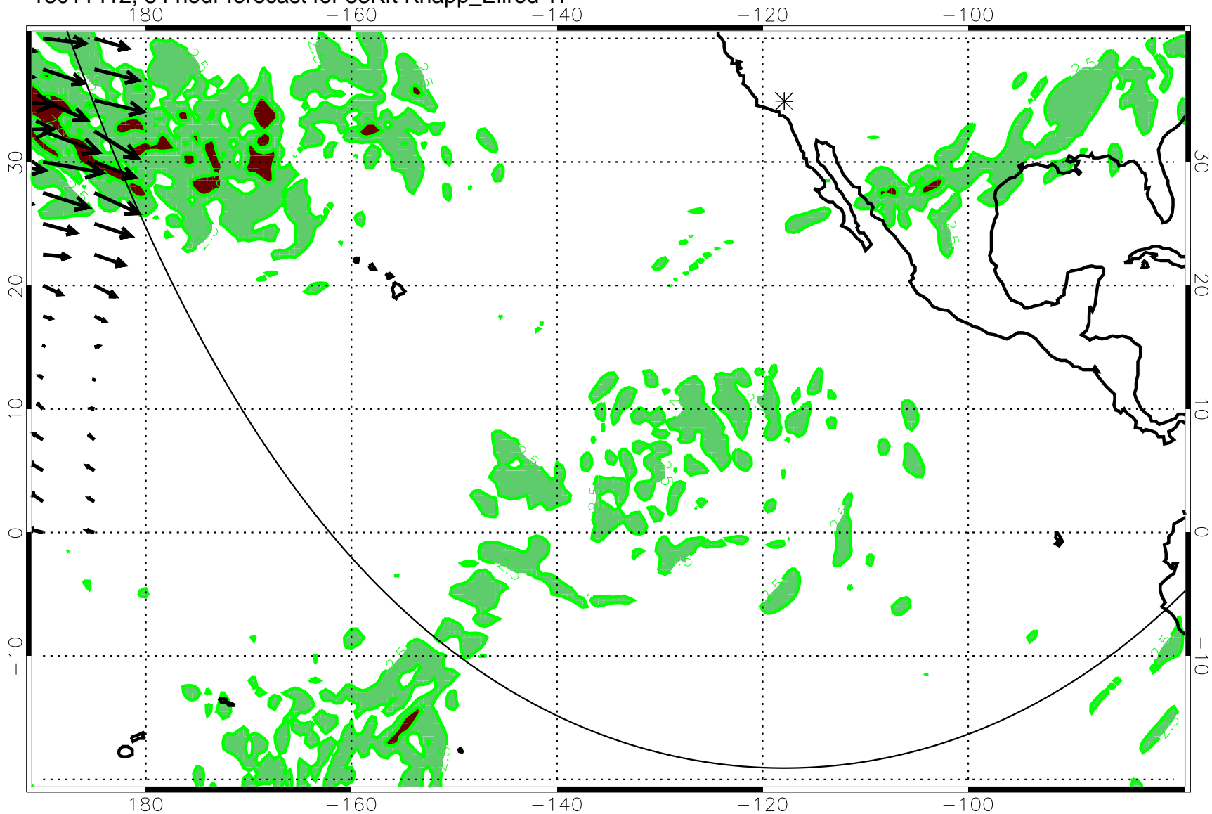
13011412, 84 hour forecast for 53Kft Knapp_Ellrod TI
