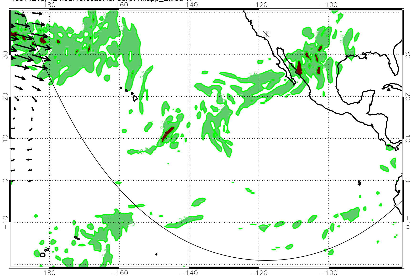
13011218, 42 hour forecast for 53Kft Knapp_Ellrod TI
