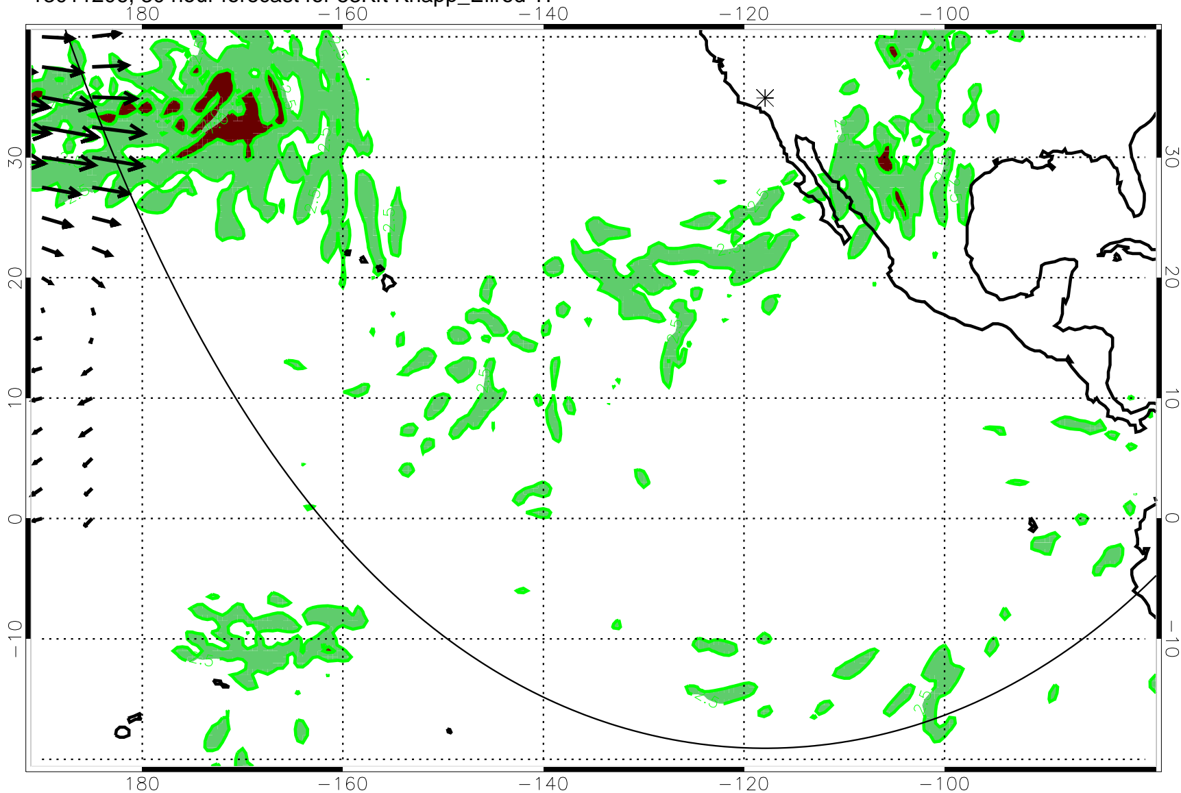
13011206, 30 hour forecast for 53Kft Knapp_Ellrod TI
