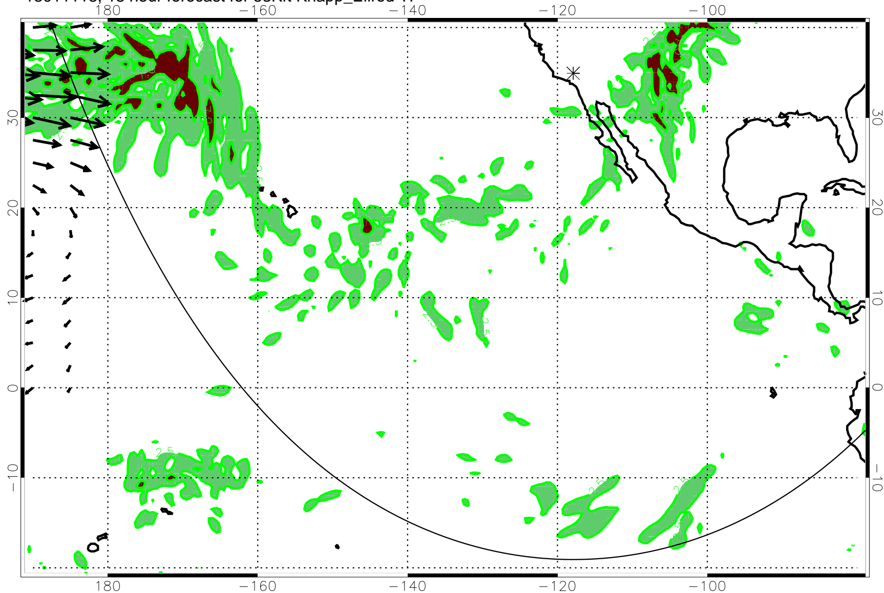
13011118, 18 hour forecast for 53Kft Knapp_Ellrod TI
