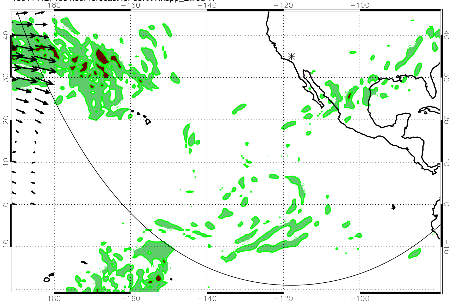
13011412, 108 hour forecast for 53Kft Knapp_Ellrod T1
