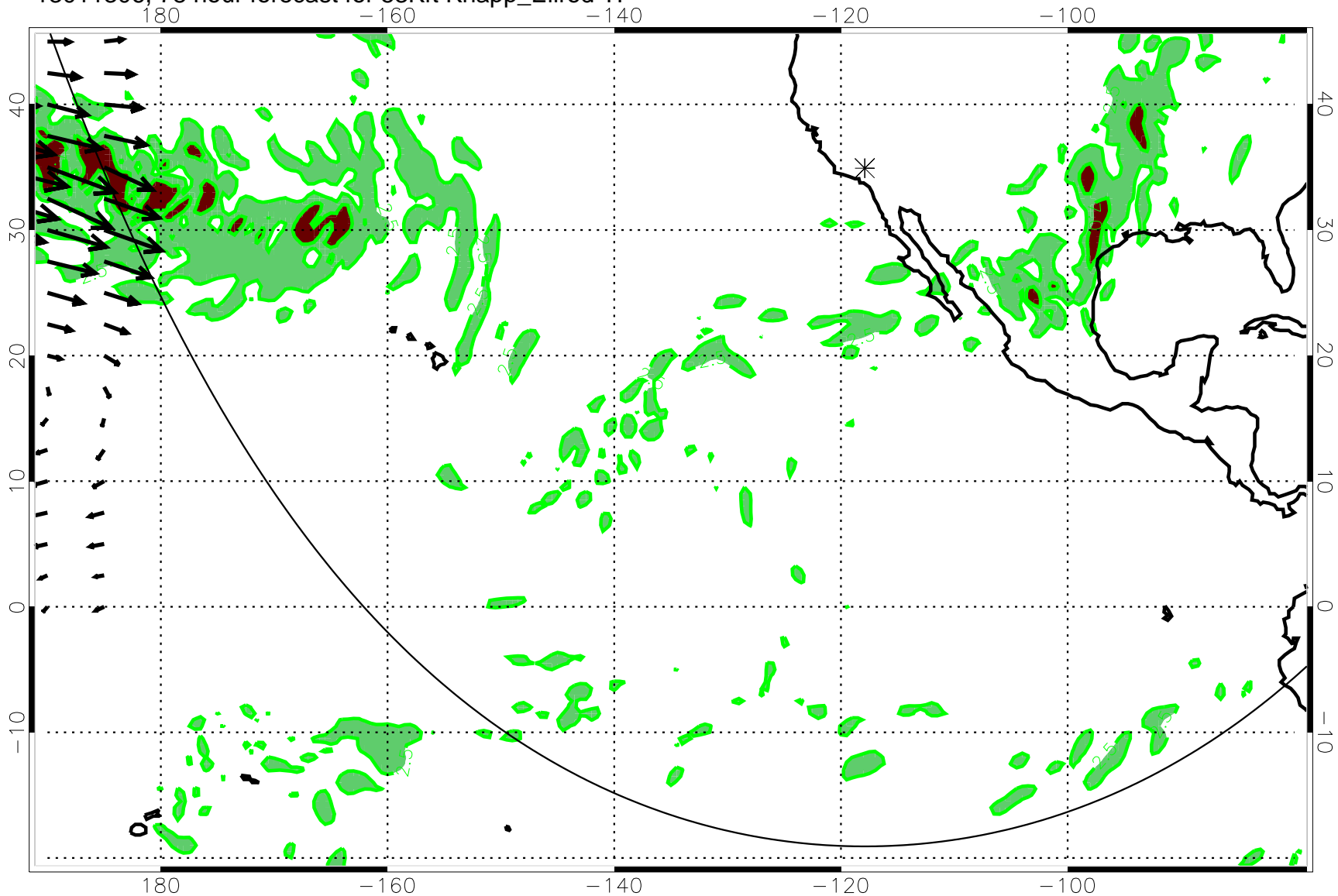
13011306, 78 hour forecast for 53Kft Knapp_Ellrod TI
