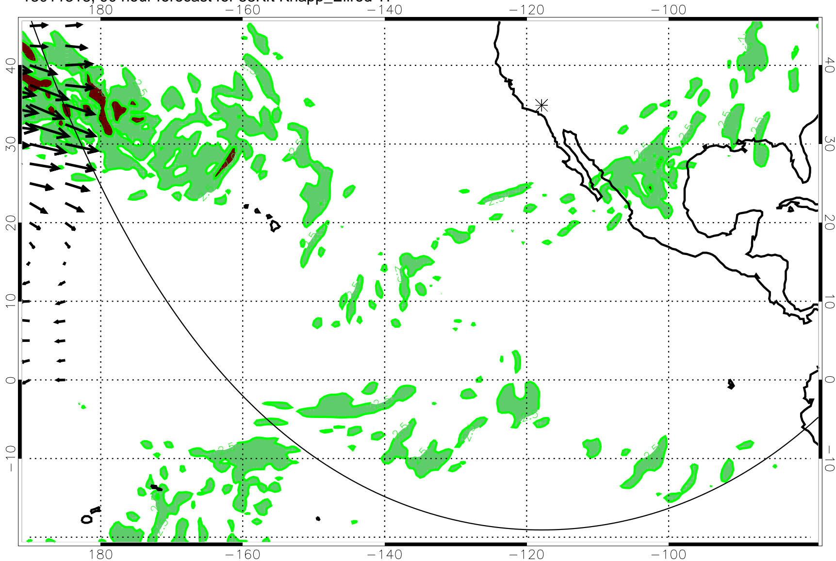
13011318, 90 hour forecast for 53Kft Knapp_Ellrod TI
