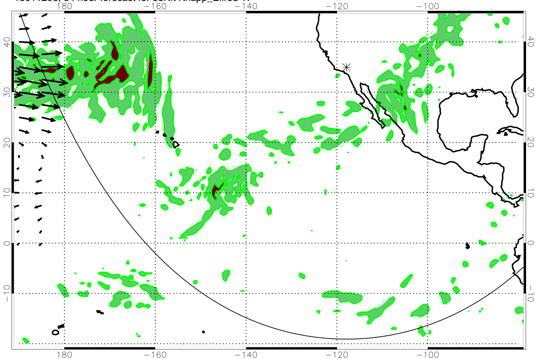
13011206, 54 hour forecast for 53Kft Knapp_Ellrod TI
