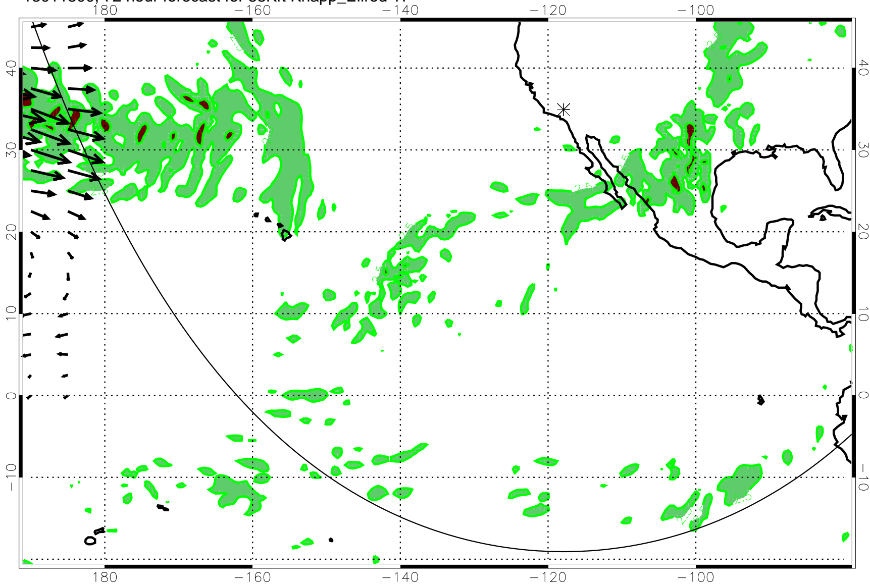
13011300, 72 hour forecast for 53Kft Knapp_Ellrod TI
