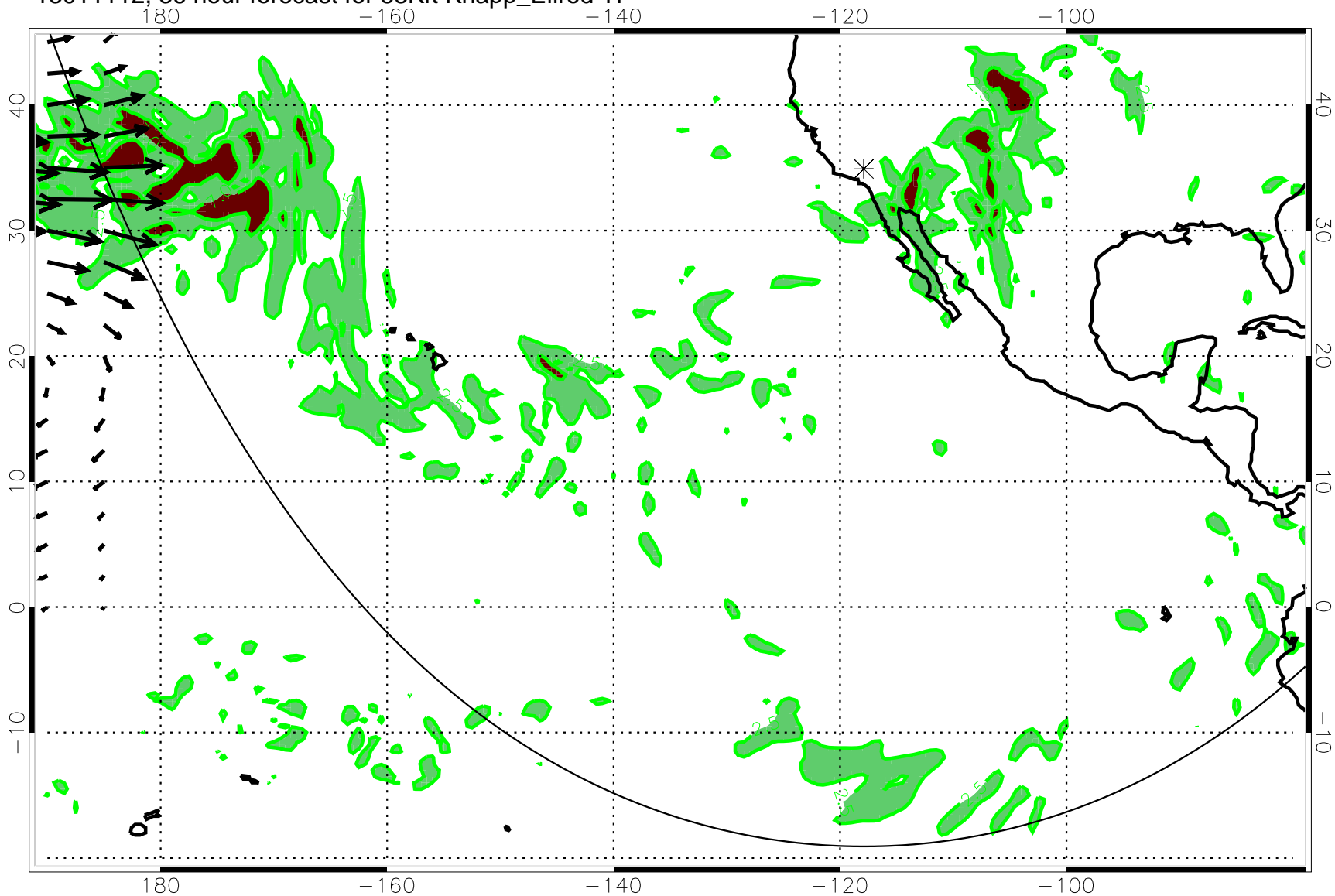
13011112, 36 hour forecast for 53Kft Knapp_Ellrod TI
