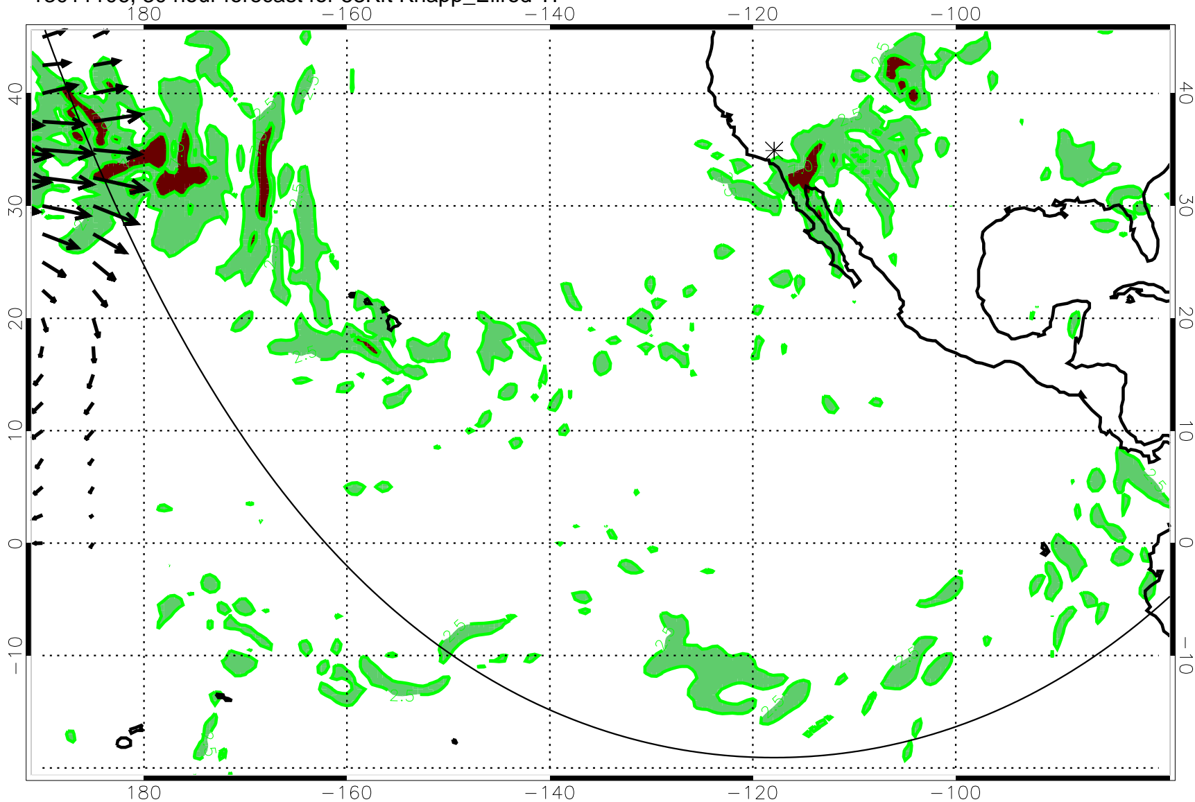
13011106, 30 hour forecast for 53Kft Knapp_Ellrod TI
