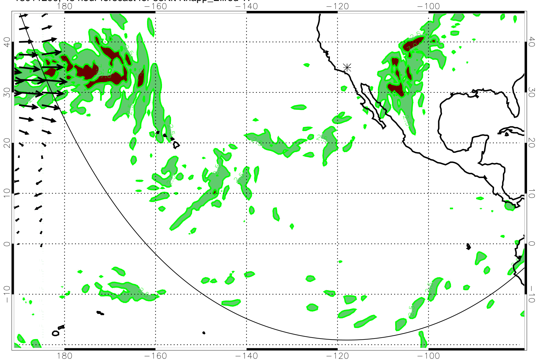
13011200, 48 hour forecast for 53Kft Knapp_Ellrod TI
