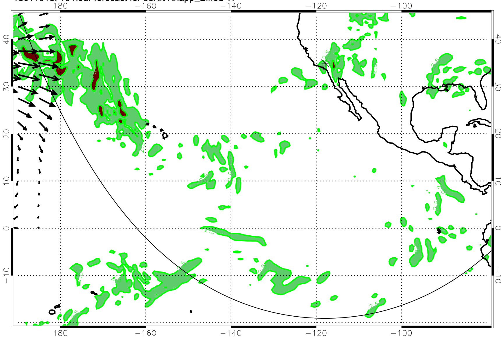
13011018, 18 hour forecast for 53Kft Knapp_Ellrod TI
