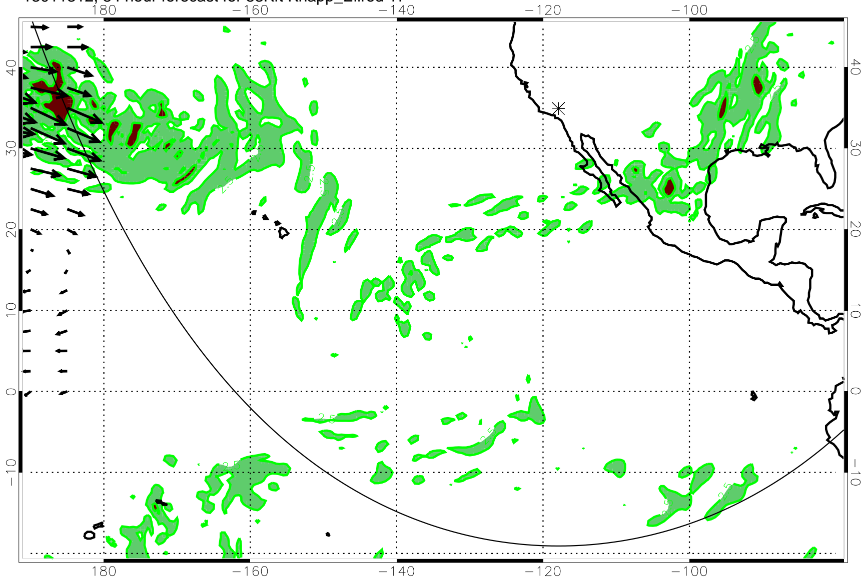
13011312, 84 hour forecast for 53Kft Knapp_Ellrod TI
