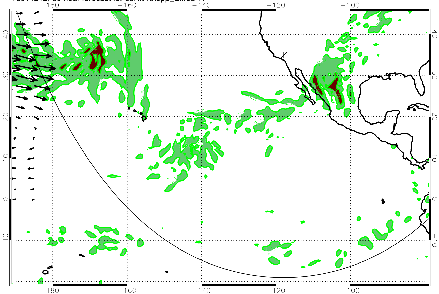
13011212, 60 hour forecast for 53Kft Knapp_Ellrod TI
