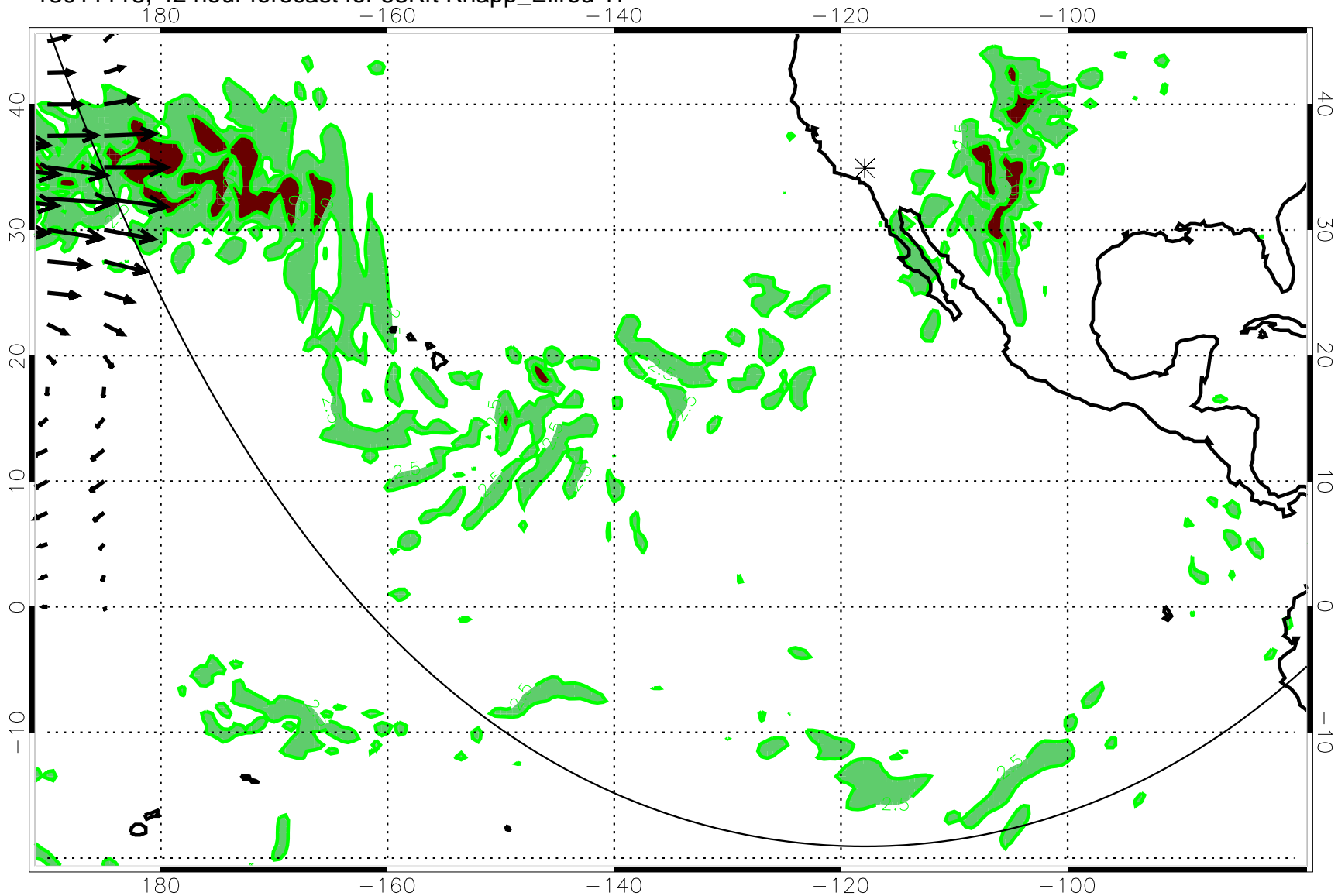
13011118, 42 hour forecast for 53Kft Knapp_Ellrod TI
