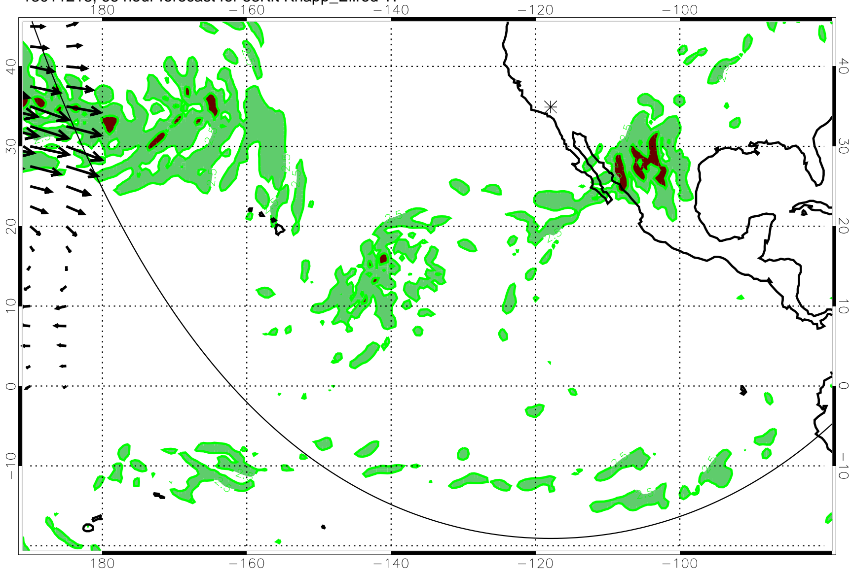
13011218, 66 hour forecast for 53Kft Knapp_Ellrod TI
