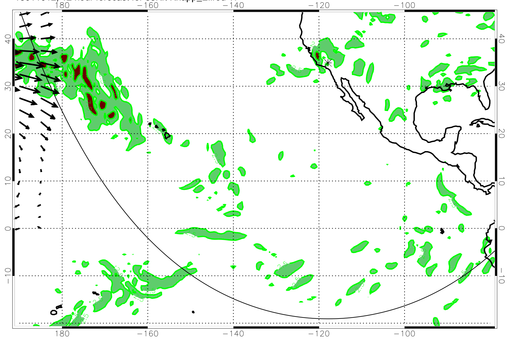
13011012, 12 hour forecast for 53Kft Knapp_Ellrod TI
