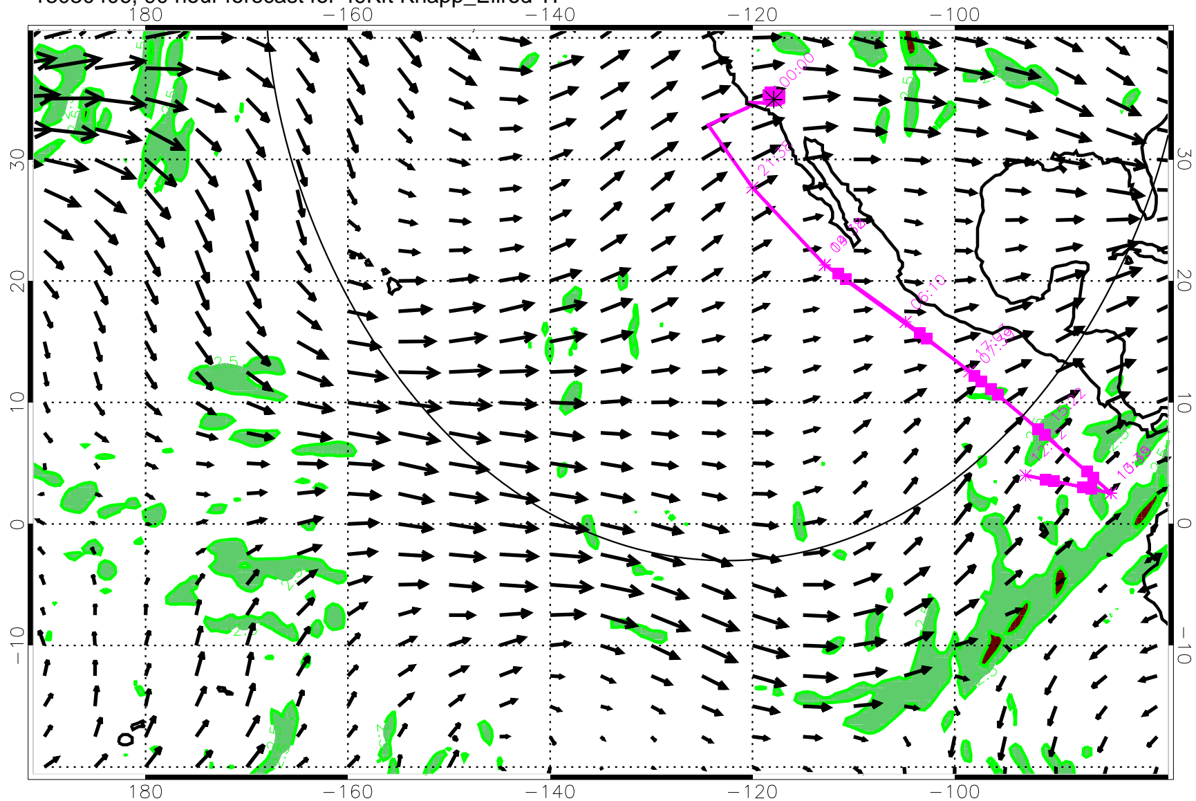
13030406, 90 hour forecast for 49Kft Knapp_Ellrod TI
