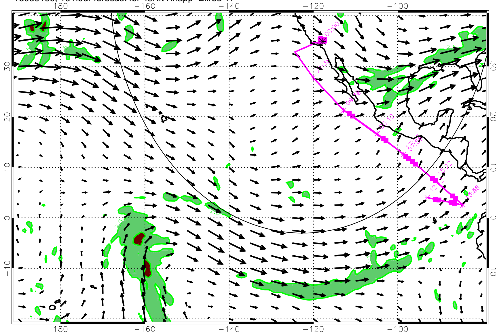
13030106, 18 hour forecast for 49Kft Knapp_Ellrod TI
