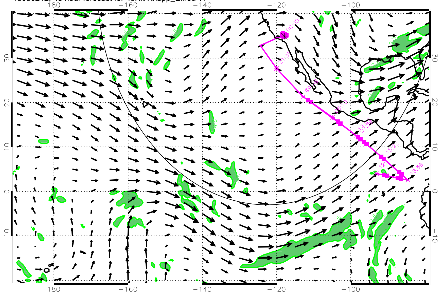
13030212, 48 hour forecast for 49Kft Knapp_Ellrod TI
