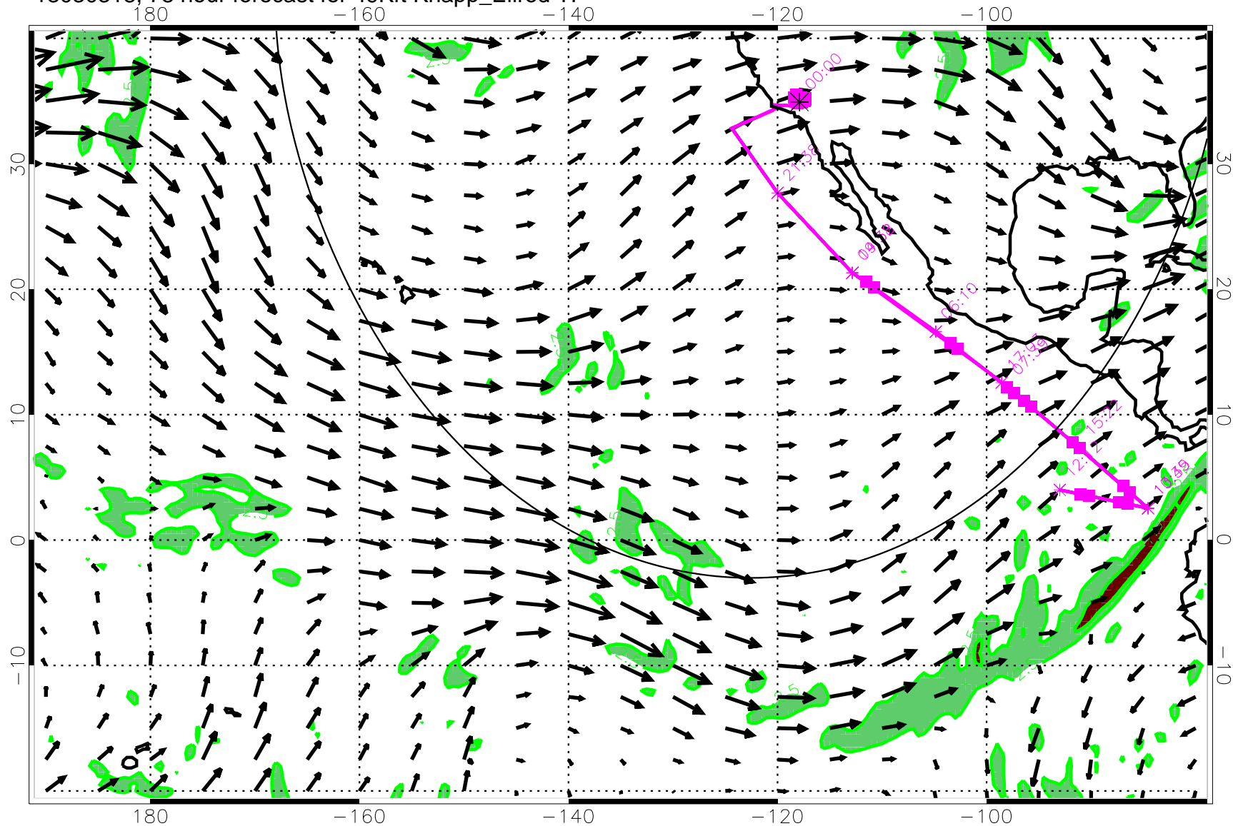
13030318, 78 hour forecast for 49Kft Knapp_Ellrod TI
