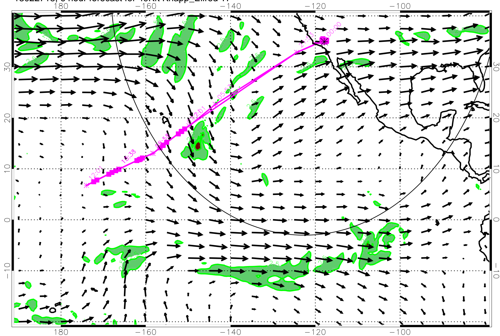
13022718, 6 hour forecast for 49Kft Knapp_Ellrod TI
