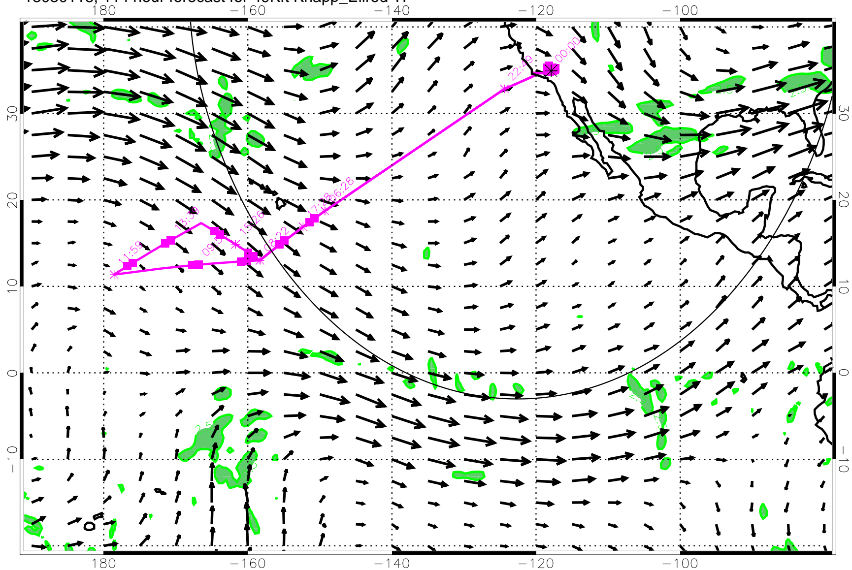
13030118, 114 hour forecast for 49Kft Knapp_Ellrod TI
