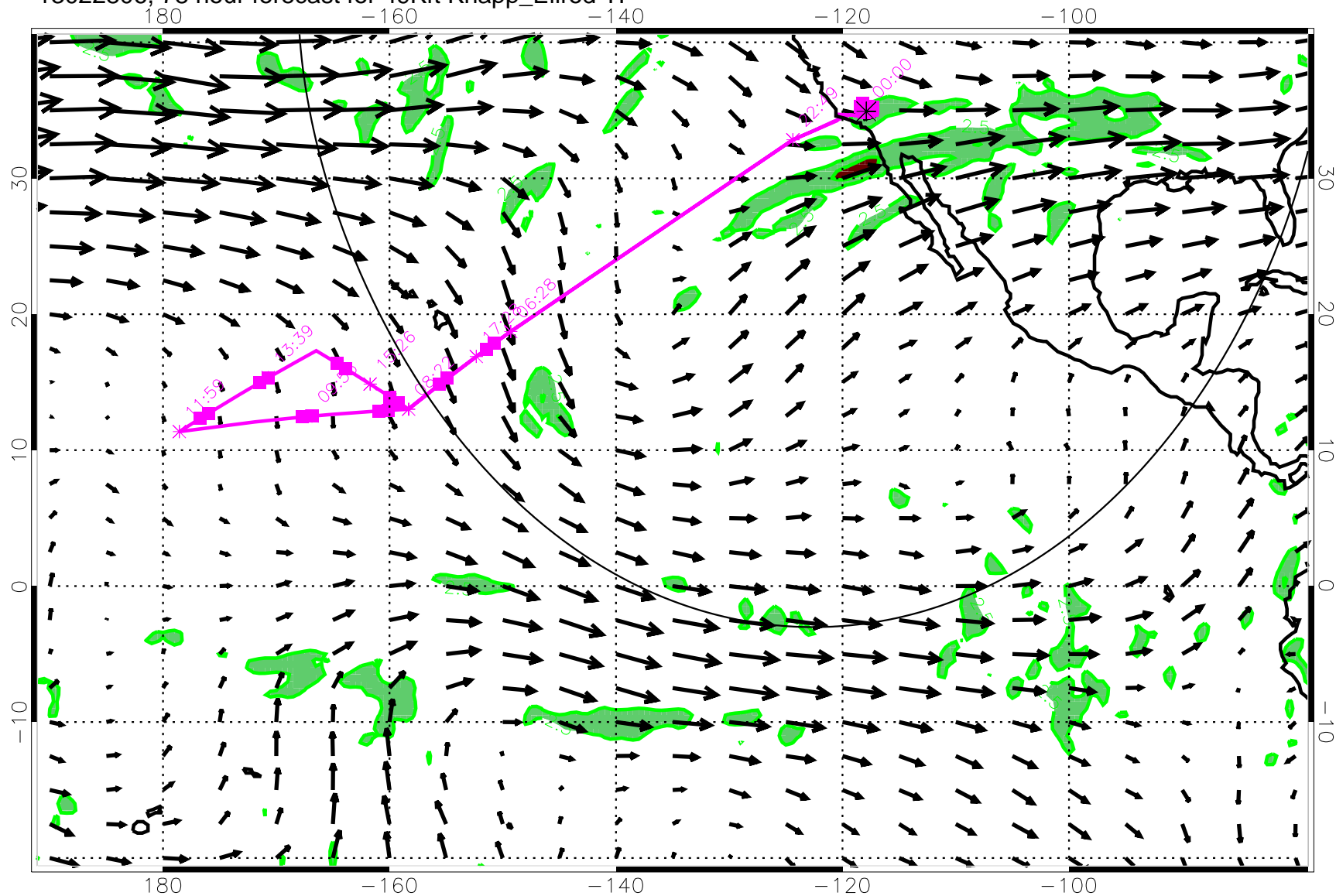
13022806, 78 hour forecast for 49Kft Knapp_Ellrod TI
