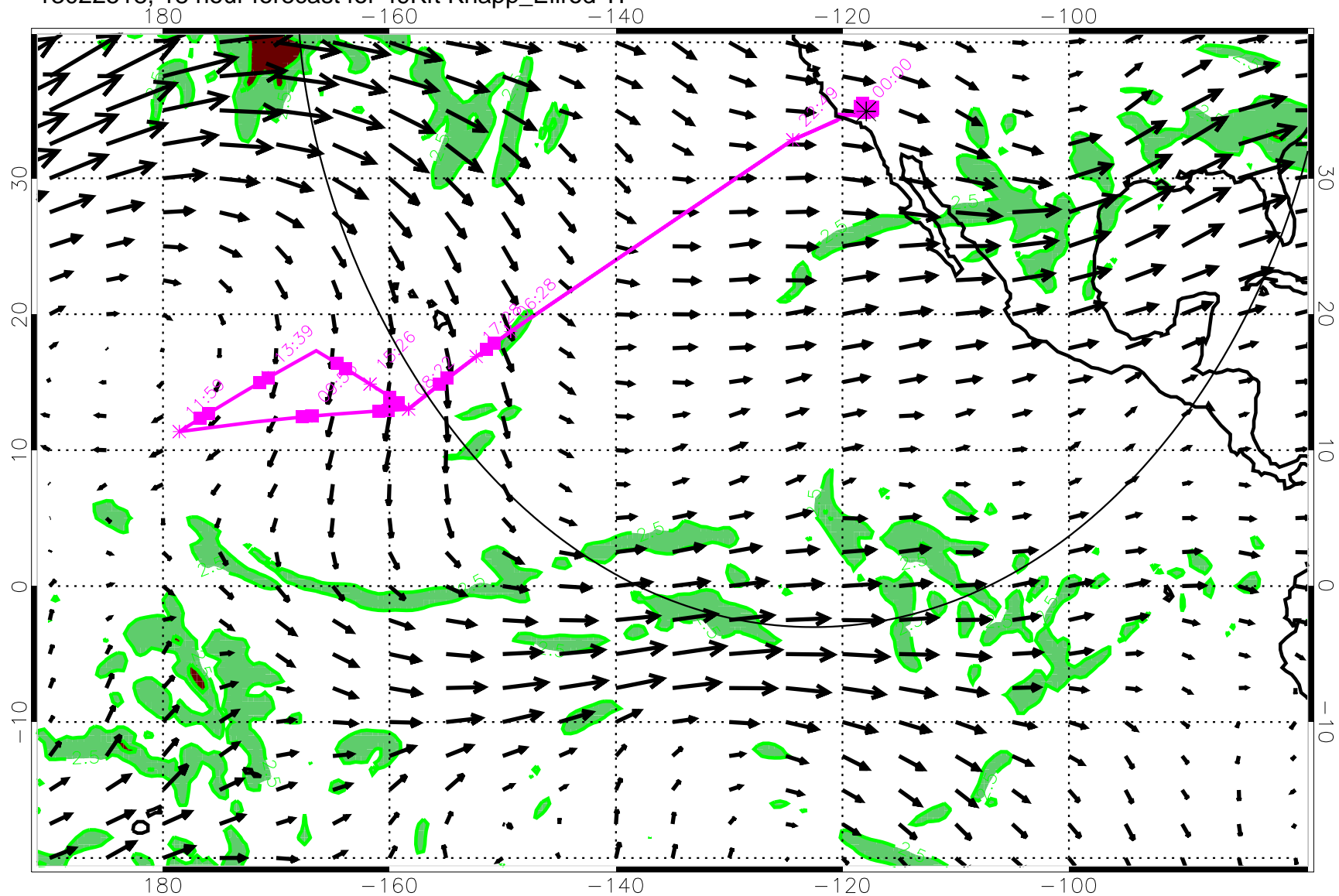
13022518, 18 hour forecast for 49Kft Knapp_Ellrod TI
