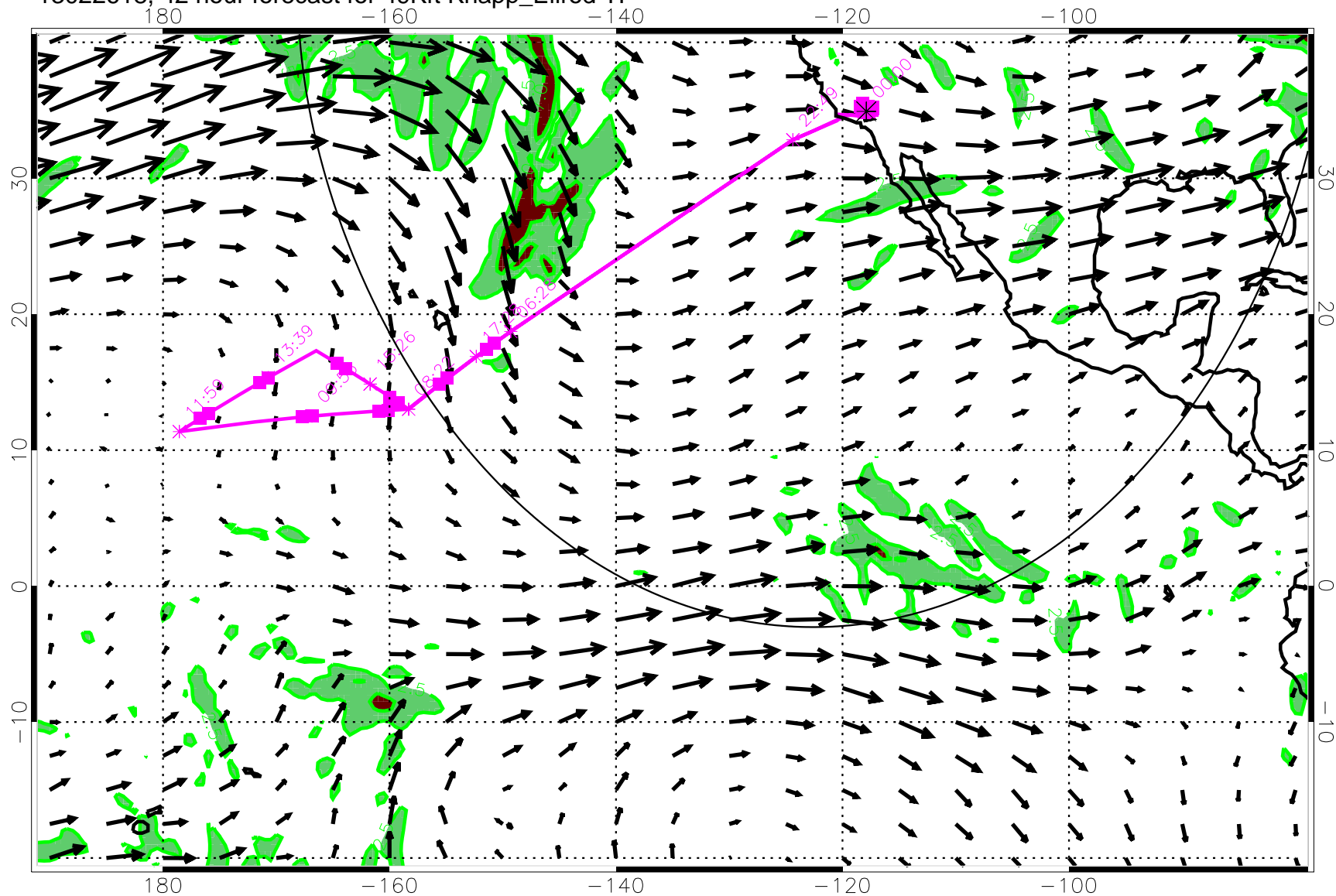
13022618, 42 hour forecast for 49Kft Knapp_Ellrod TI
