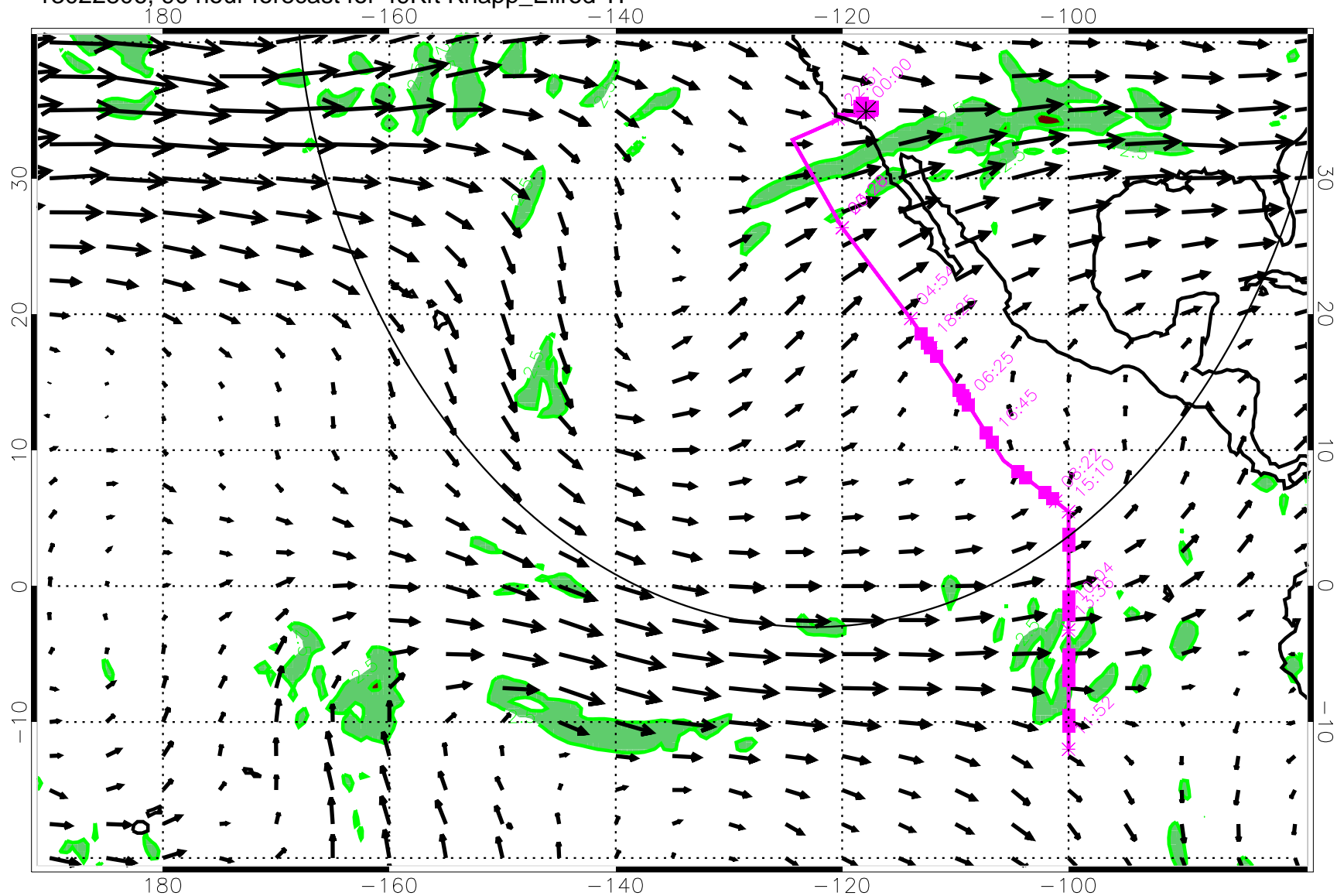
13022806, 90 hour forecast for 49Kft Knapp_Ellrod TI
