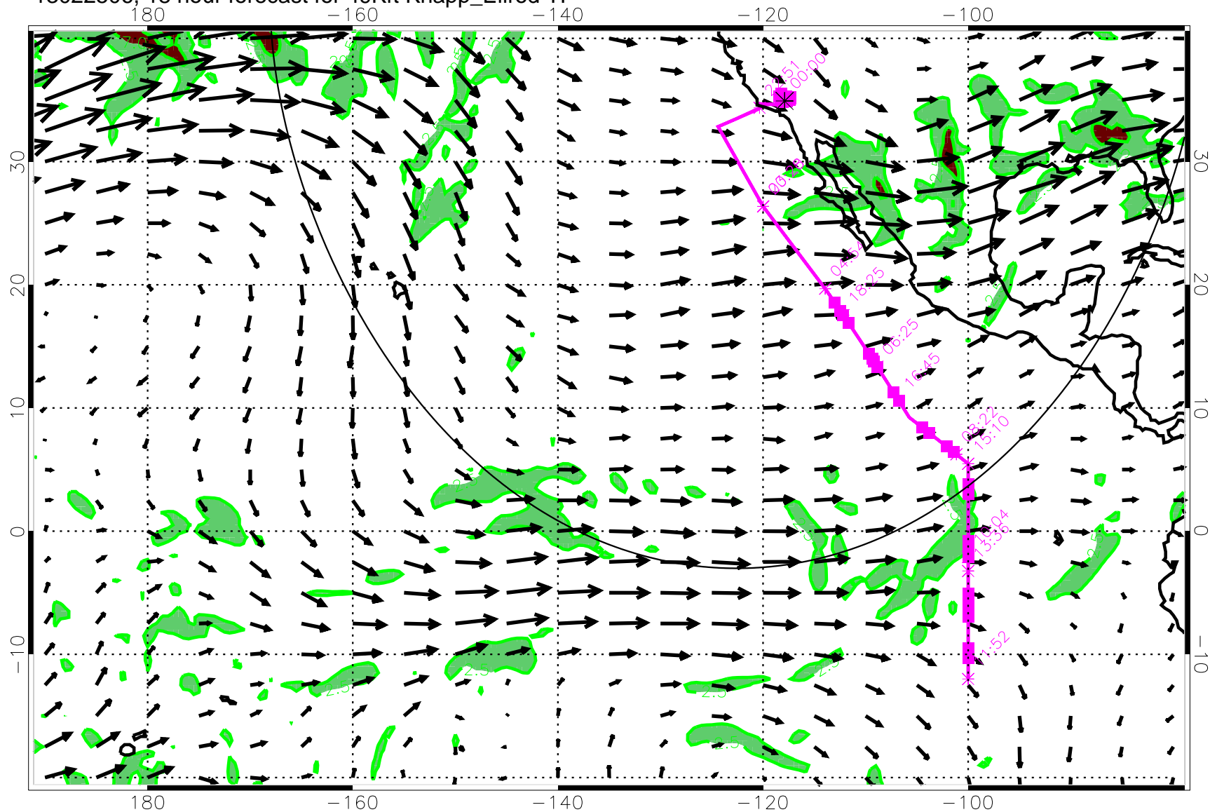
13022506, 18 hour forecast for 49Kft Knapp_Ellrod TI
