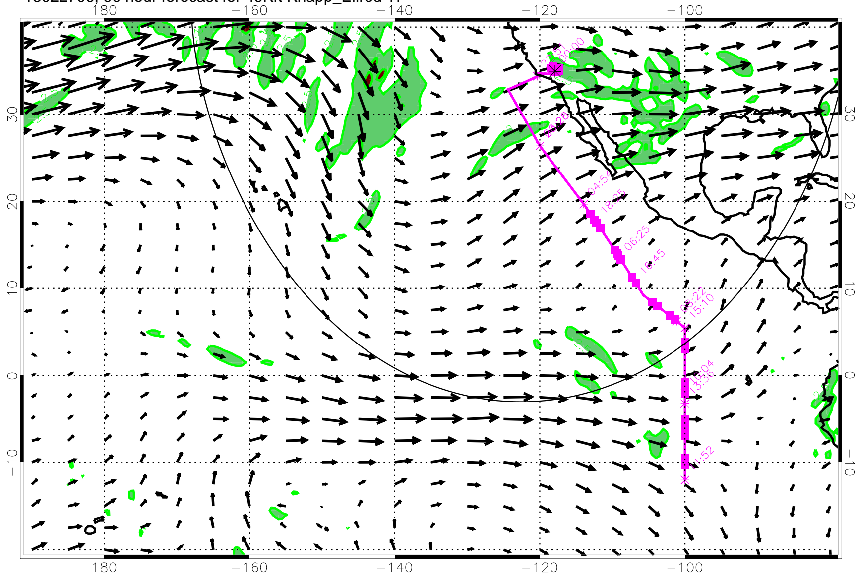
13022706, 90 hour forecast for 49Kft Knapp_Ellrod TI
