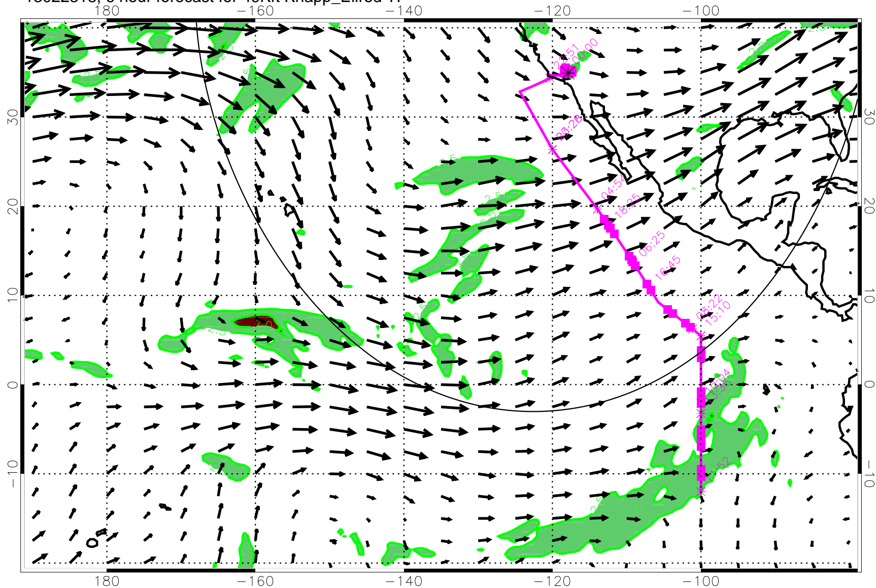
13022318, 6 hour forecast for 49Kft Knapp_Ellrod TI
