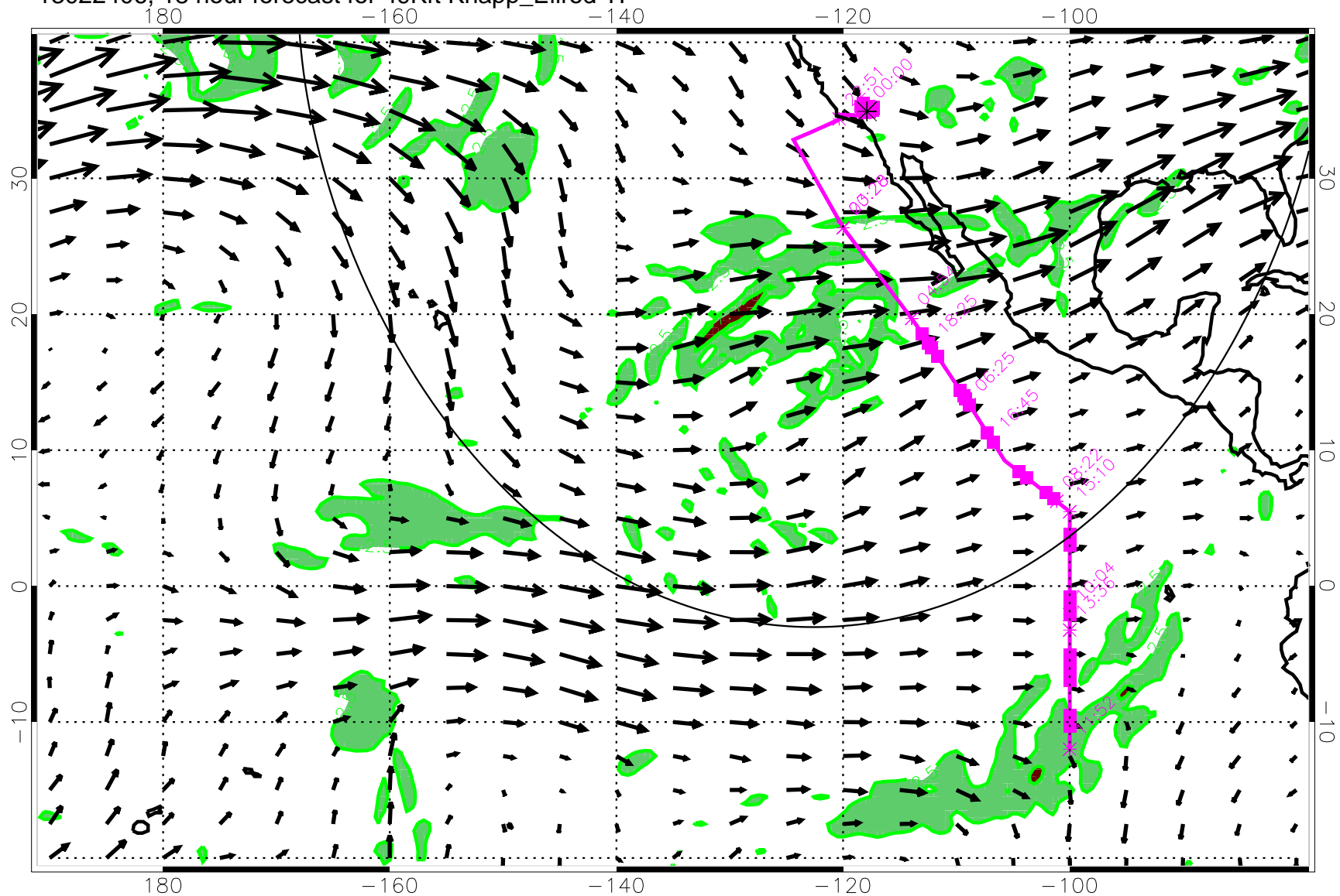
13022406, 18 hour forecast for 49Kft Knapp_Ellrod TI
