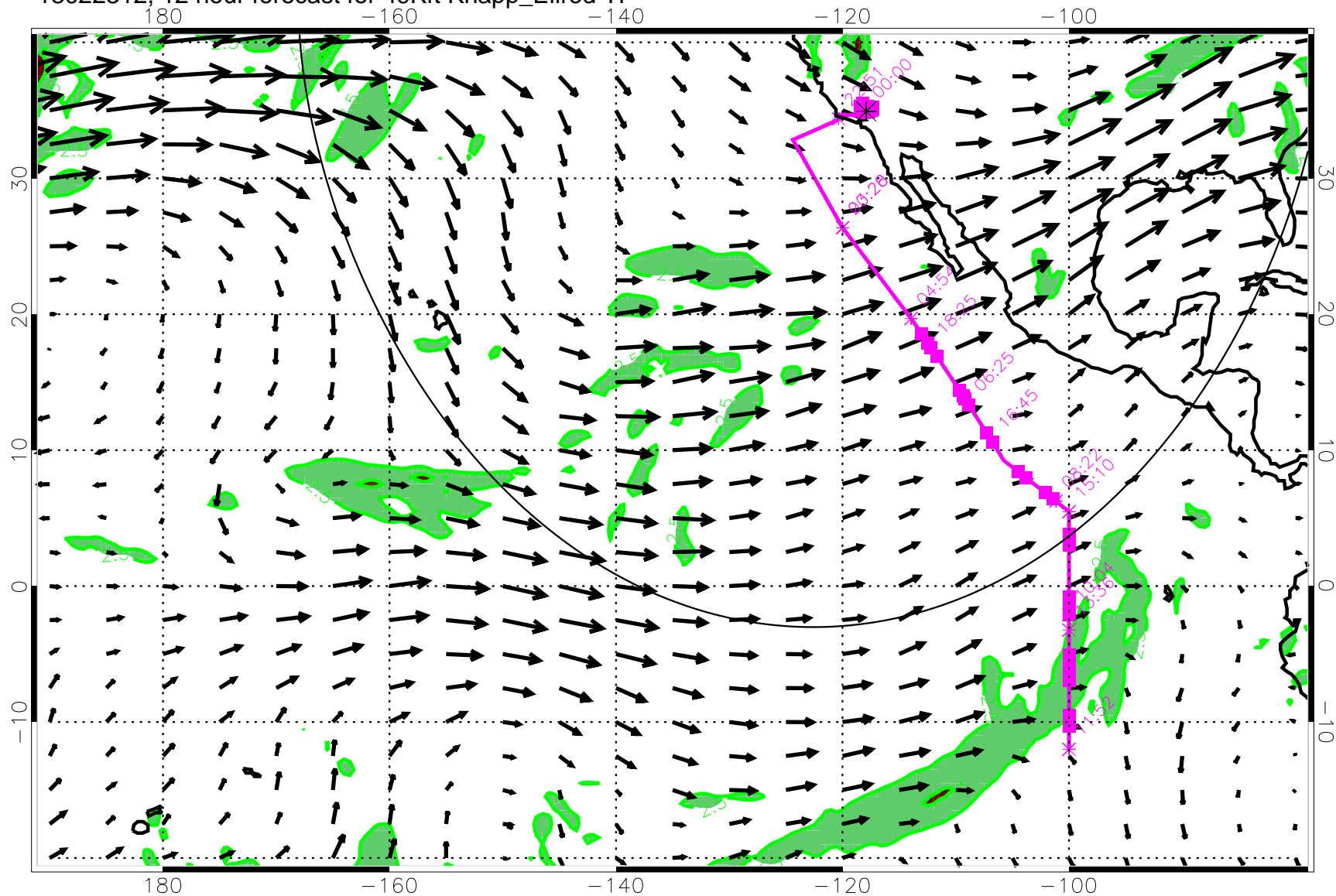
13022312, 12 hour forecast for 49Kft Knapp_Ellrod TI
