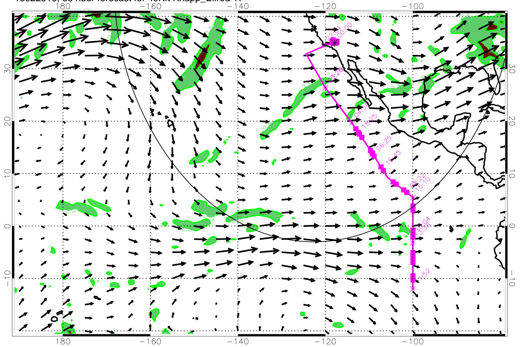
13022518, 66 hour forecast for 49Kft Knapp_Ellrod TI
