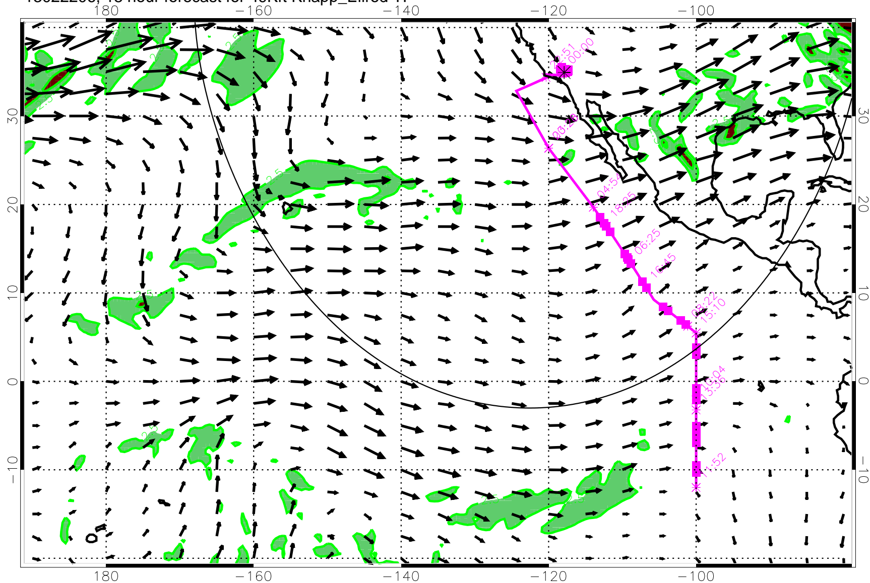
13022206, 18 hour forecast for 49Kft Knapp_Ellrod TI
