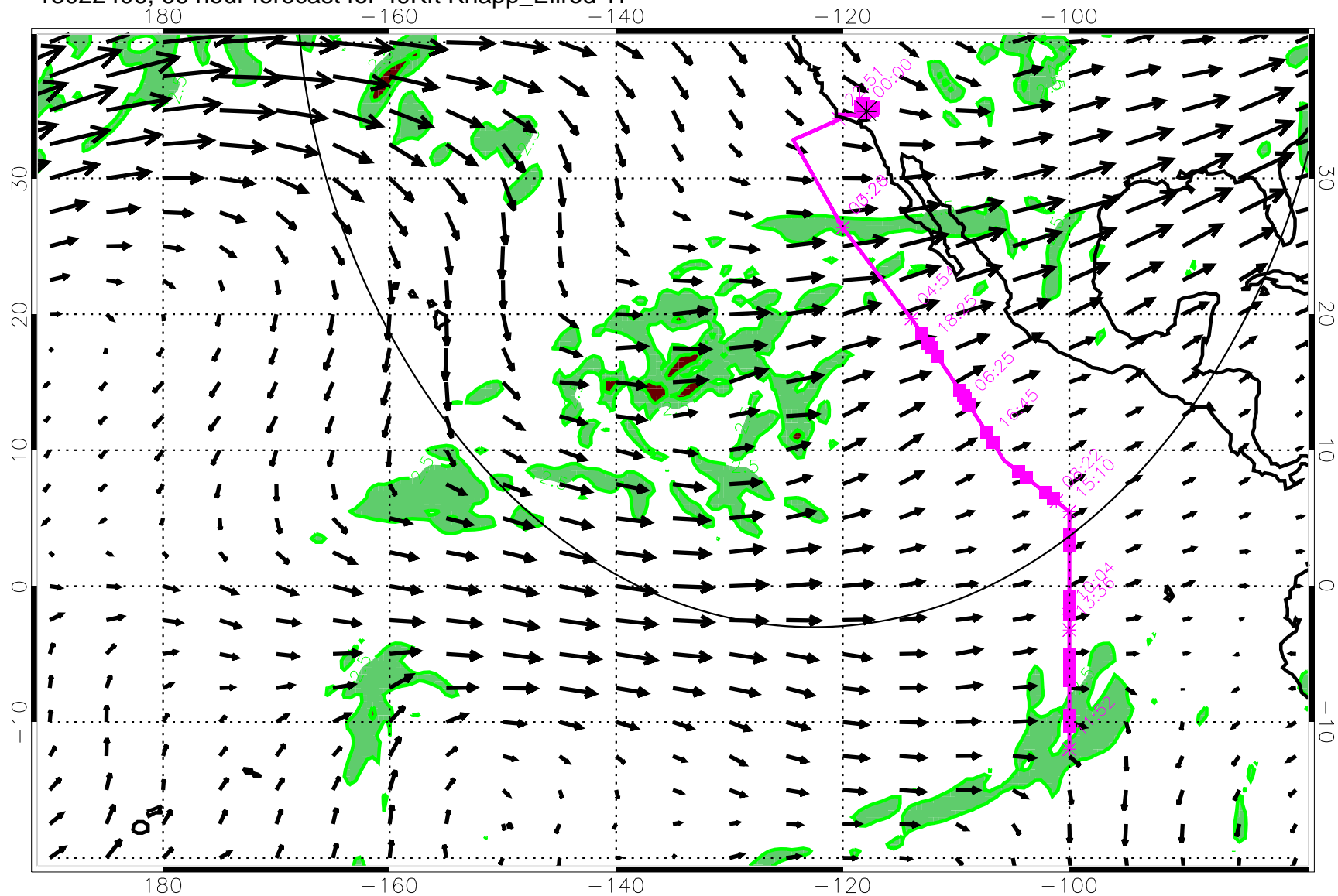
13022406, 66 hour forecast for 49Kft Knapp_Ellrod TI
