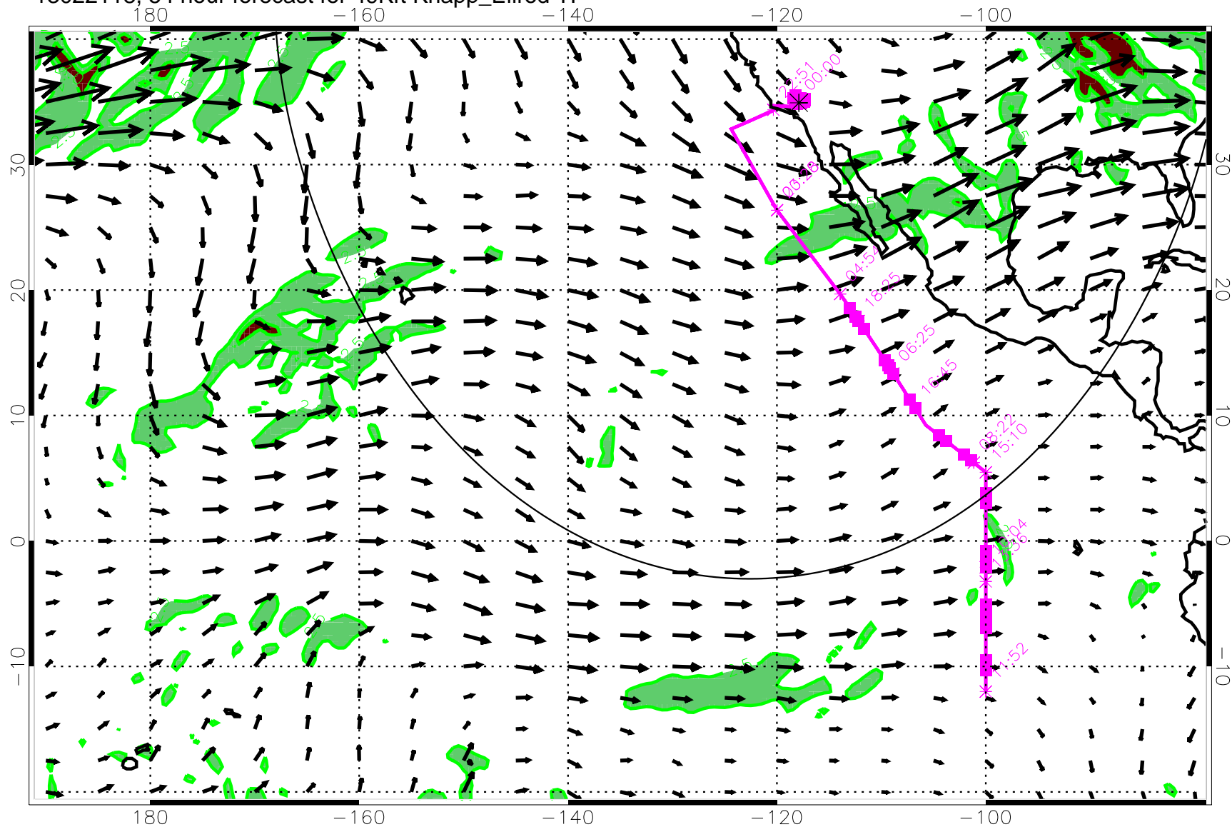
13022118, 54 hour forecast for 49Kft Knapp_Ellrod TI
