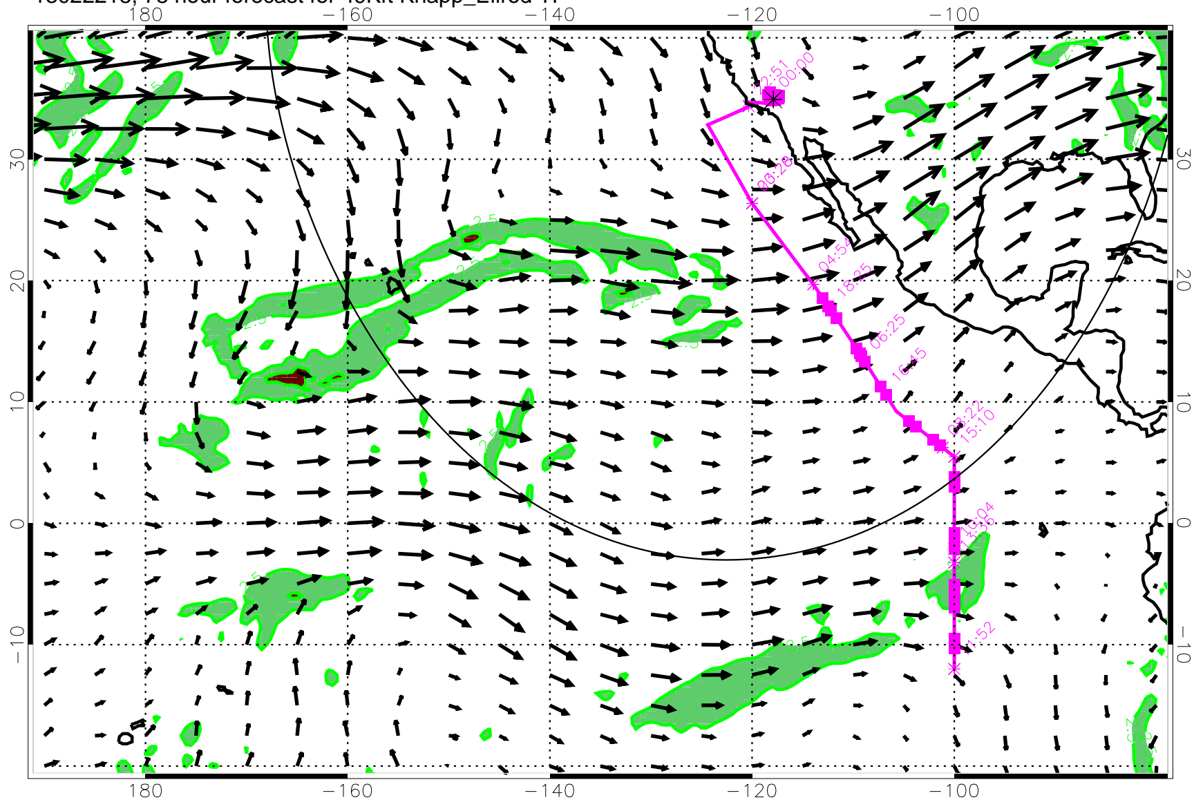
13022218, 78 hour forecast for 49Kft Knapp_Ellrod TI
