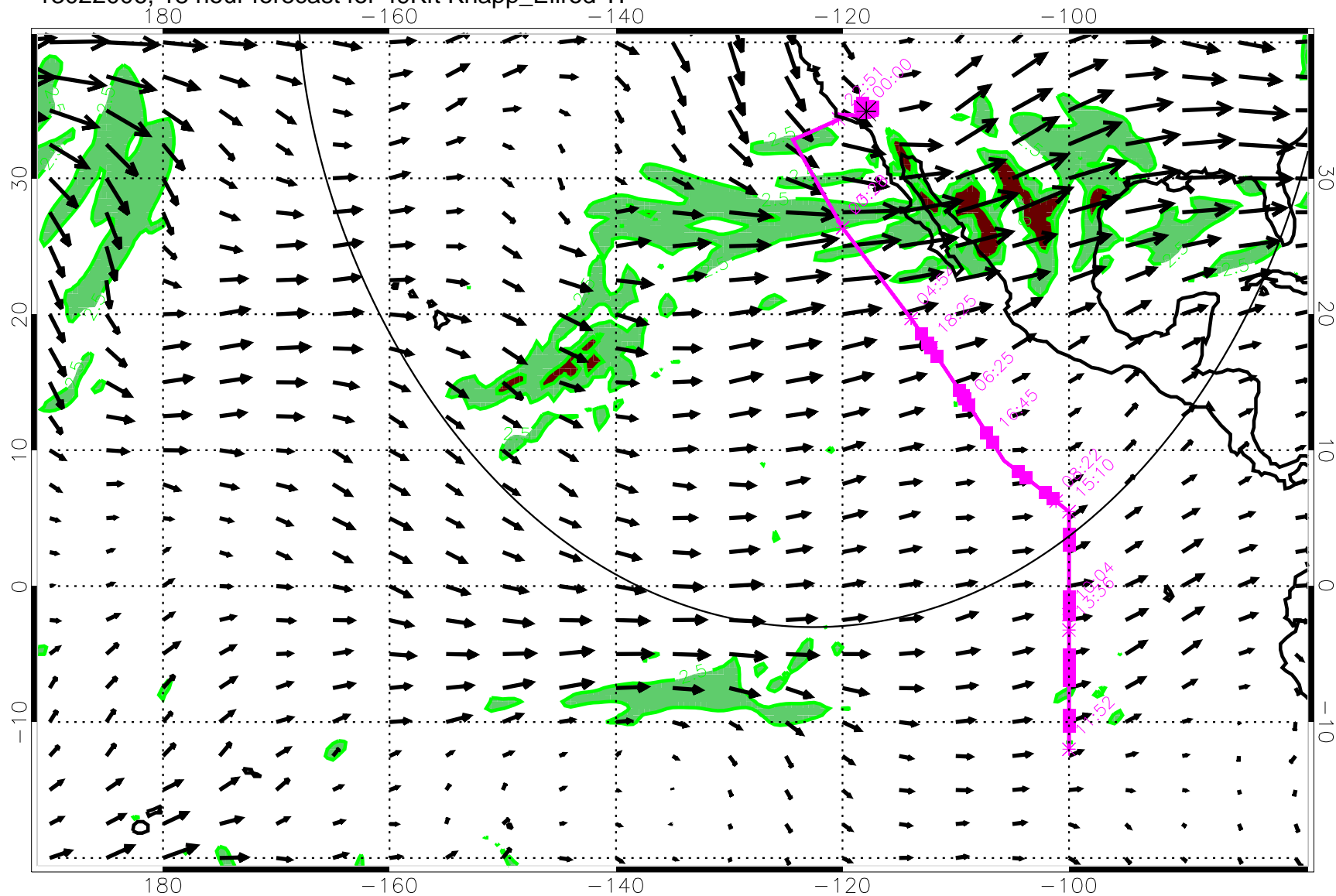
13022006, 18 hour forecast for 49Kft Knapp_Ellrod TI
