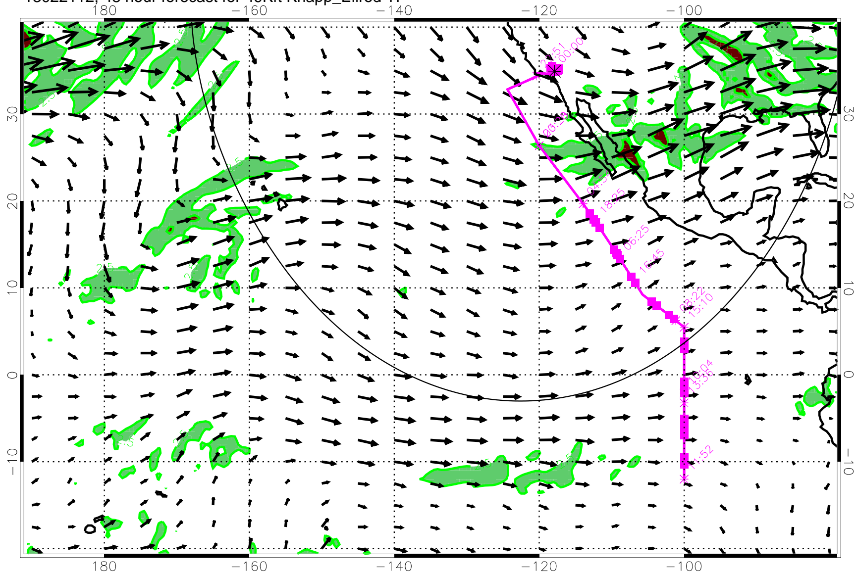
13022112, 48 hour forecast for 49Kft Knapp_Ellrod TI
