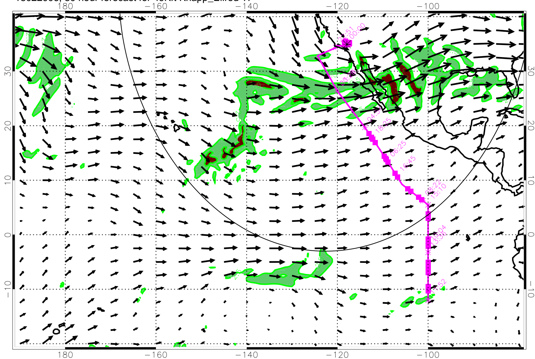
13022006, 30 hour forecast for 49Kft Knapp_Ellrod TI
