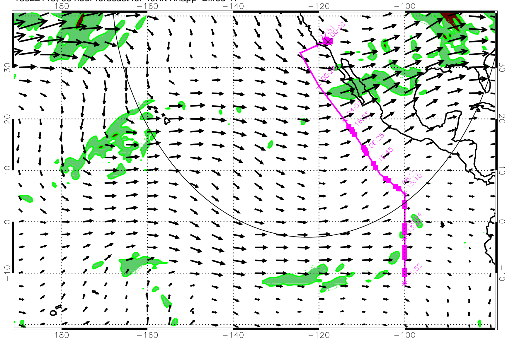
13022118, 66 hour forecast for 49Kft Knapp_Ellrod TI
