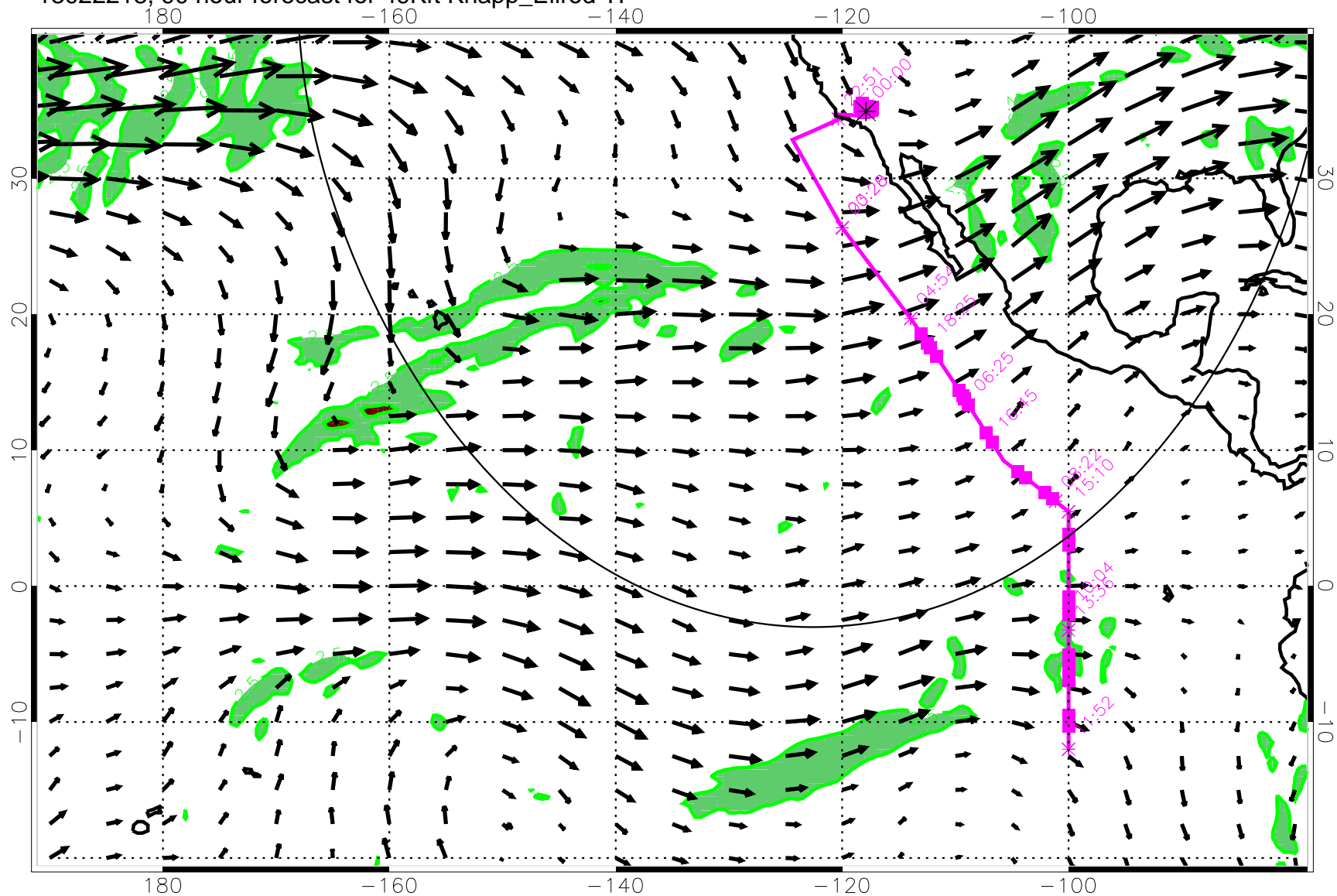
13022218, 90 hour forecast for 49Kft Knapp_Ellrod TI
