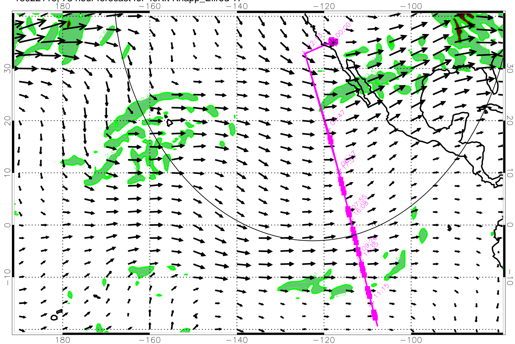
13022118, 78 hour forecast for 49Kft Knapp_Ellrod TI
