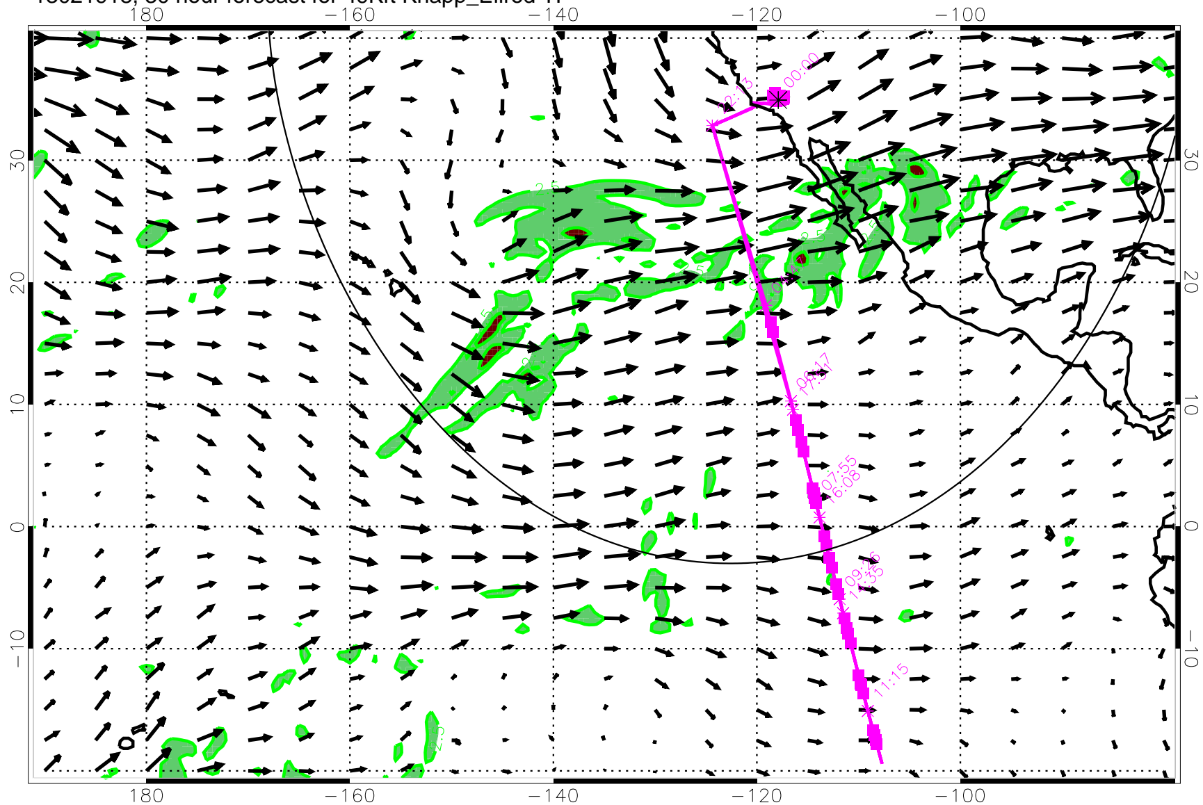
13021918, 30 hour forecast for 49Kft Knapp_Ellrod TI
