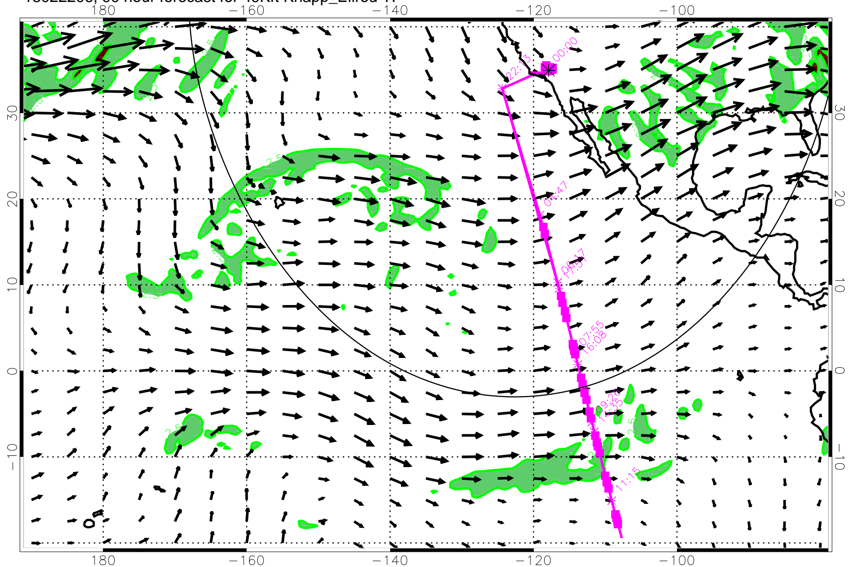
13022206, 90 hour forecast for 49Kft Knapp_Ellrod TI
