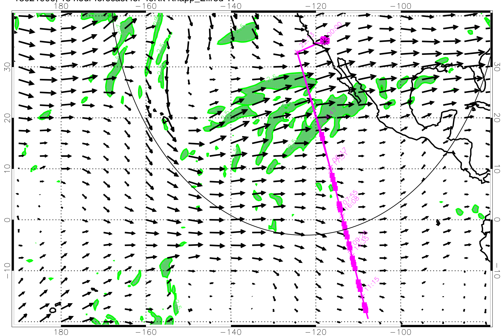
13021906, 18 hour forecast for 49Kft Knapp_Ellrod TI
