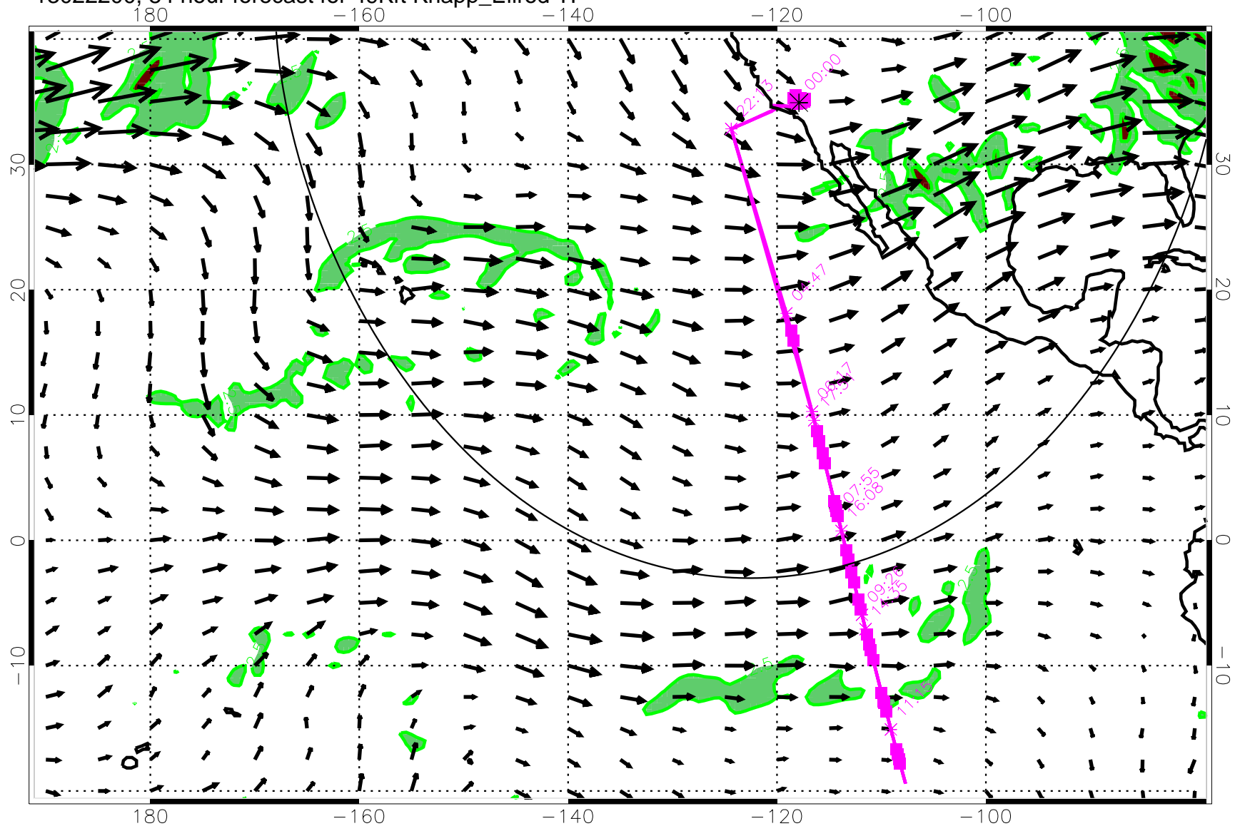
13022200, 84 hour forecast for 49Kft Knapp_Ellrod TI
