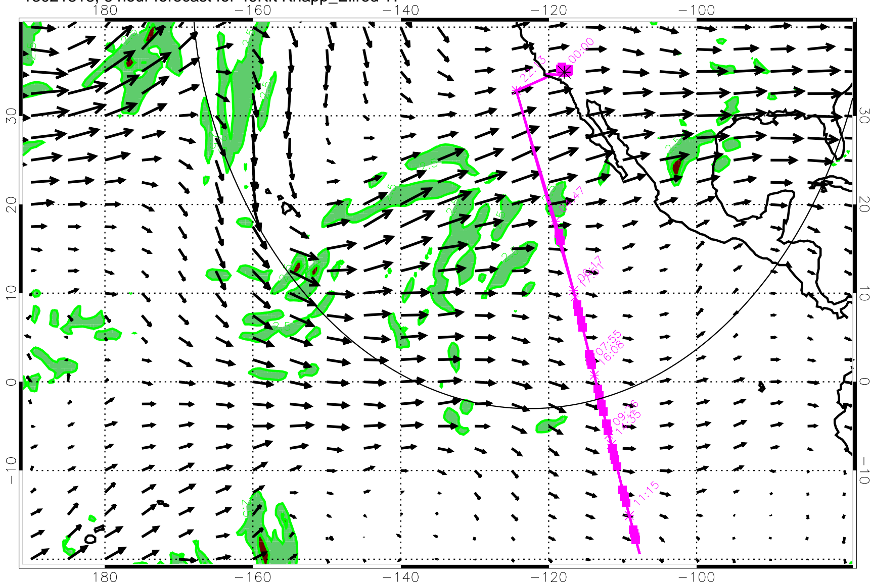
13021818, 6 hour forecast for 49Kft Knapp_Ellrod TI
