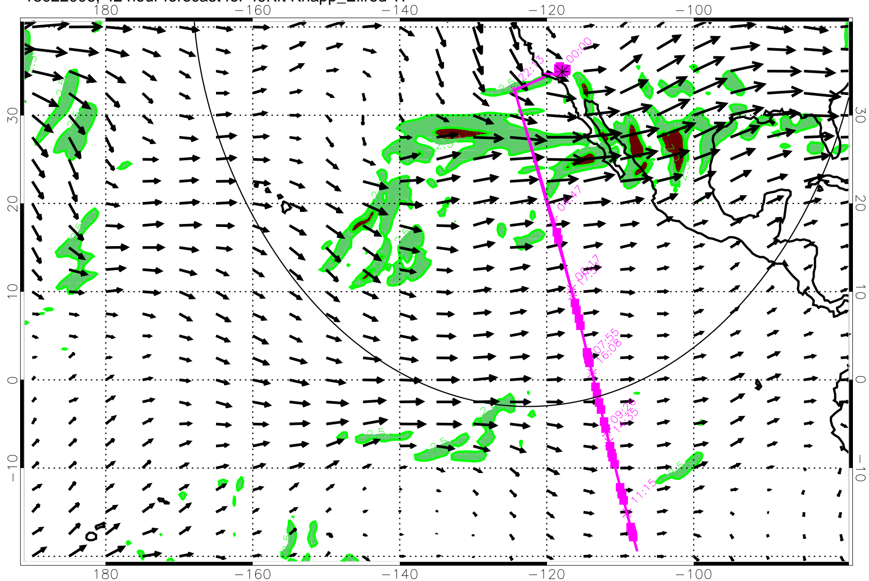
13022006, 42 hour forecast for 49Kft Knapp_Ellrod TI
