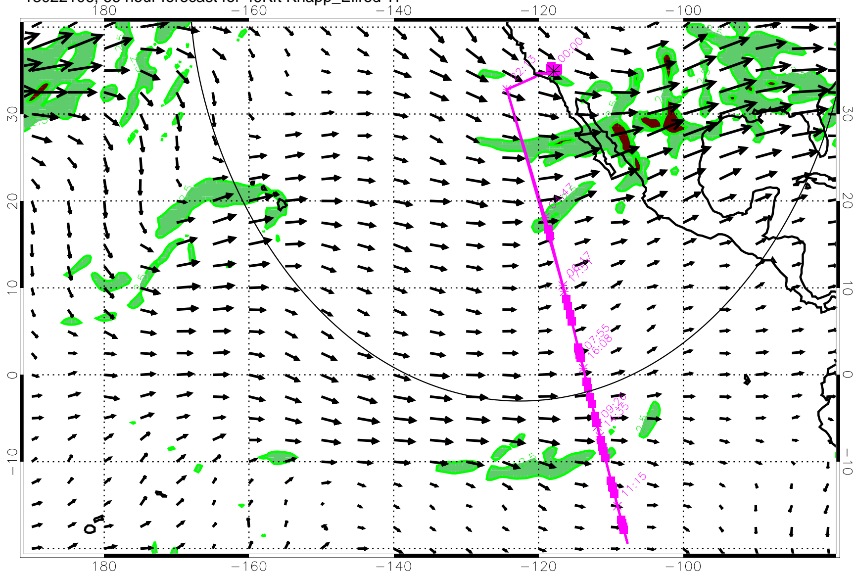
13022106, 66 hour forecast for 49Kft Knapp_Ellrod TI
