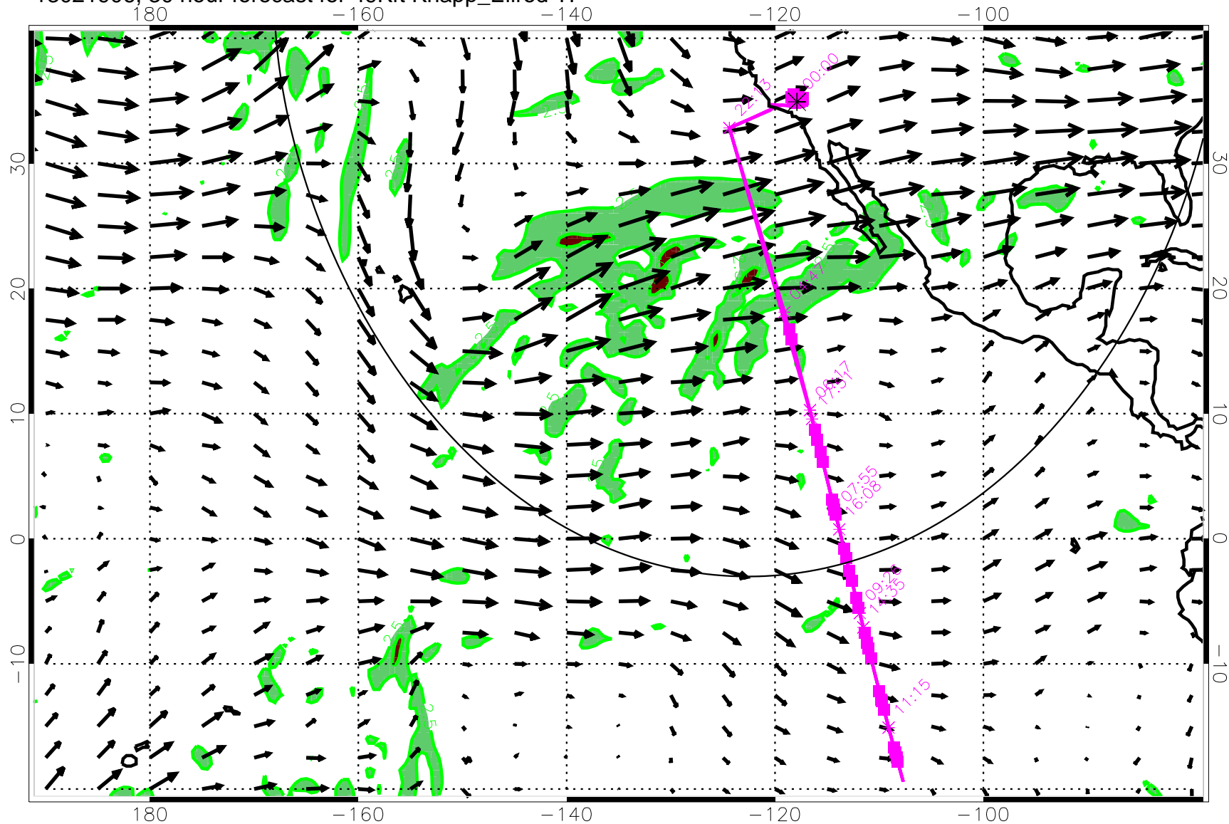
13021906, 30 hour forecast for 49Kft Knapp_Ellrod TI
