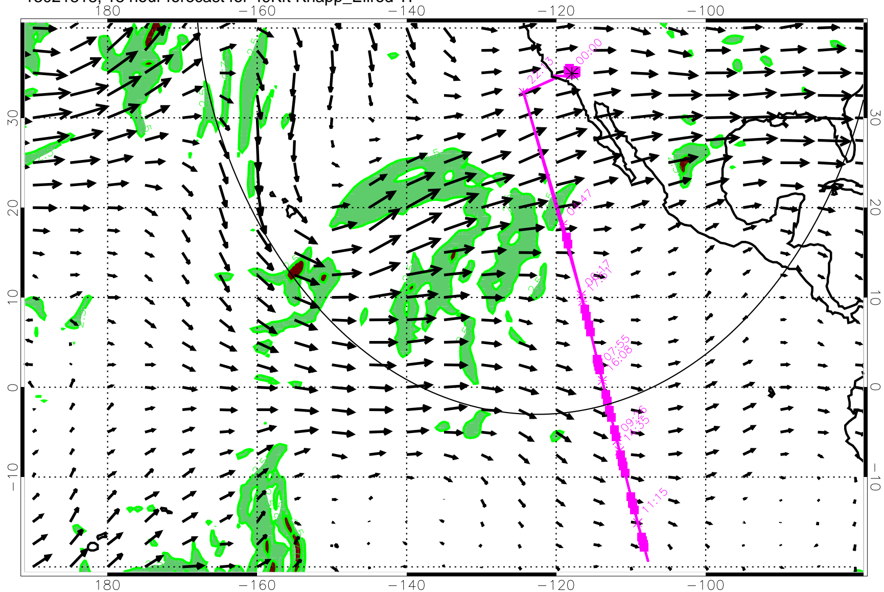
13021818, 18 hour forecast for 49Kft Knapp_Ellrod TI
