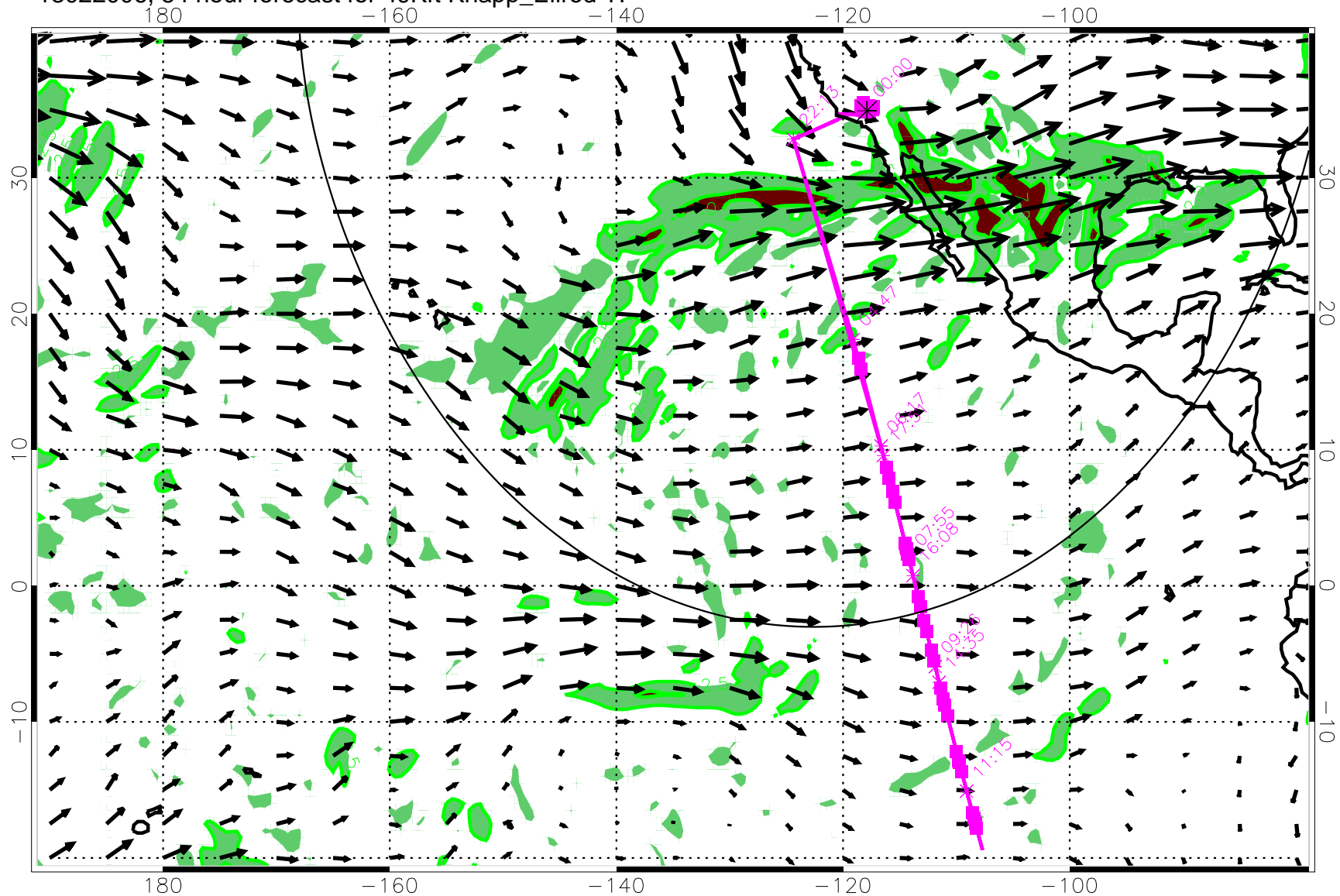
13022006, 54 hour forecast for 49Kft Knapp_Ellrod TI
