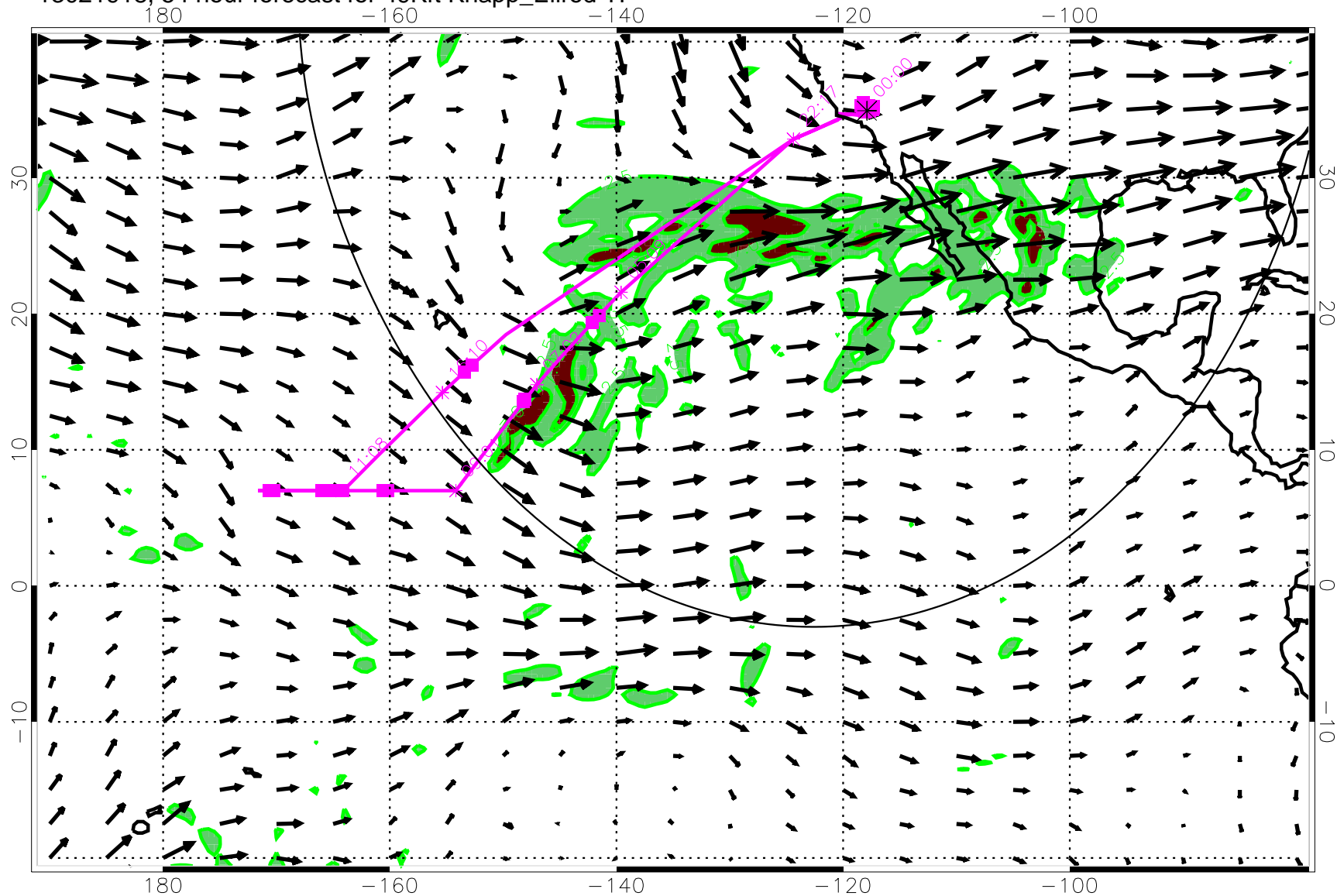
13021918, 54 hour forecast for 49Kft Knapp_Ellrod TI
