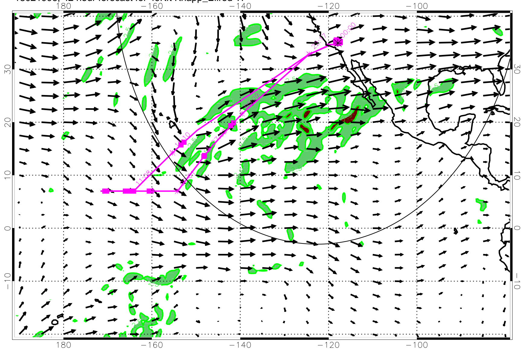
13021906, 42 hour forecast for 49Kft Knapp_Ellrod TI
