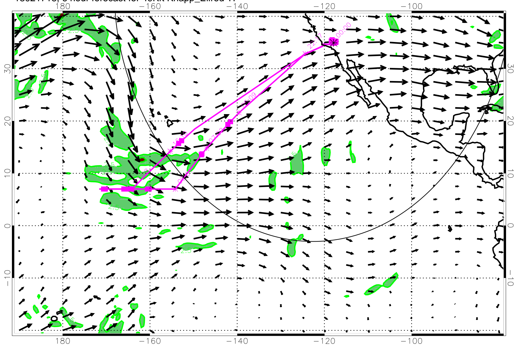
13021718, 6 hour forecast for 49Kft Knapp_Ellrod TI
