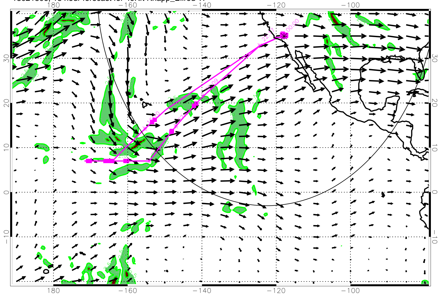
13021806, 18 hour forecast for 49Kft Knapp_Ellrod TI
