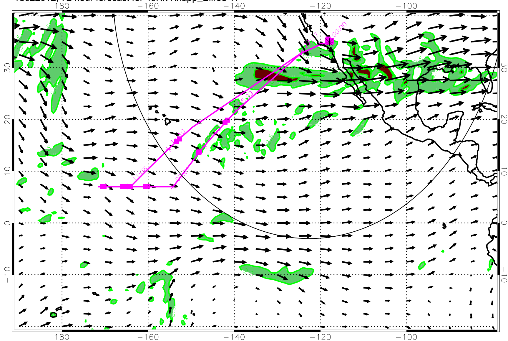
13022012, 72 hour forecast for 49Kft Knapp_Ellrod TI
