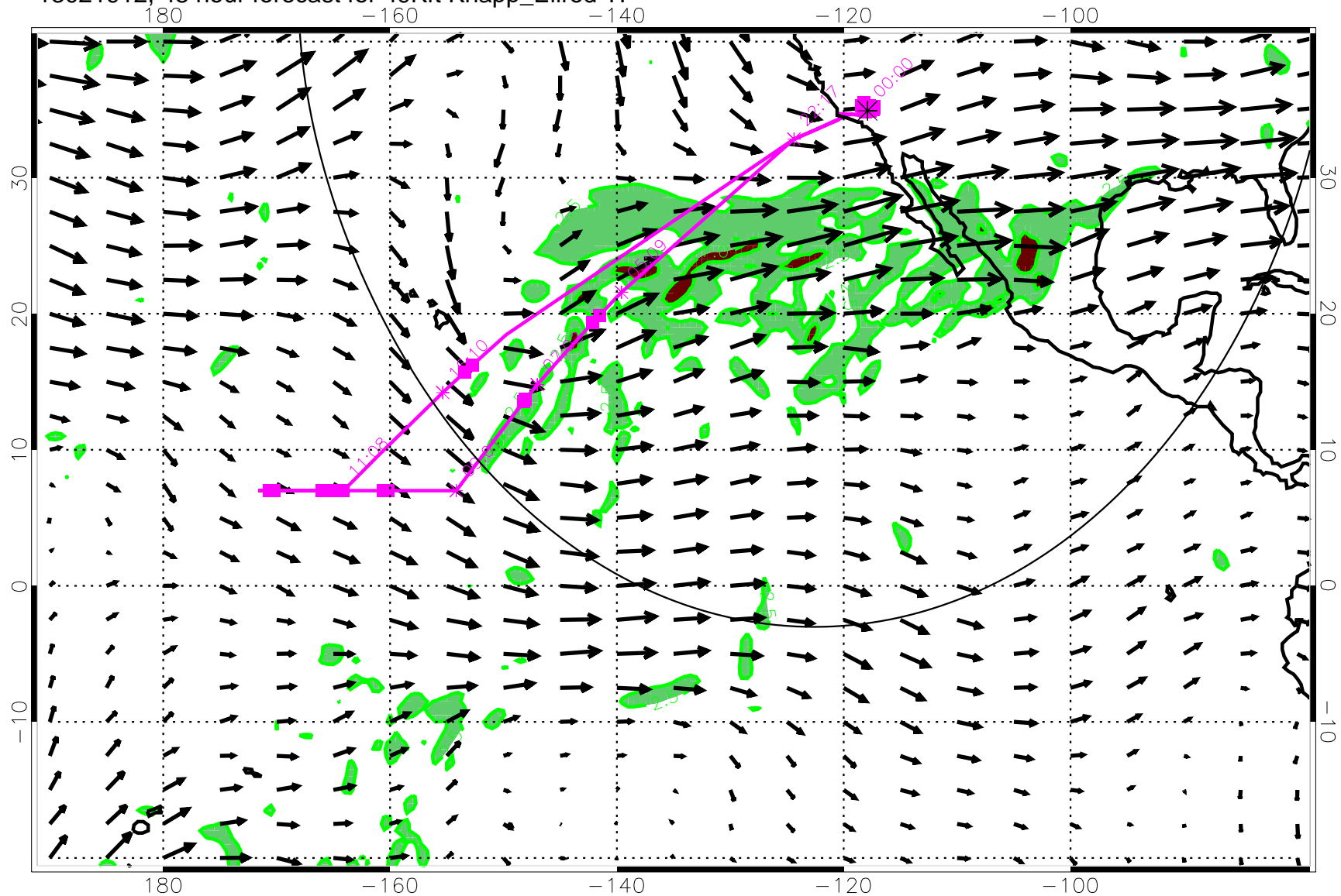
13021912, 48 hour forecast for 49Kft Knapp_Ellrod TI
