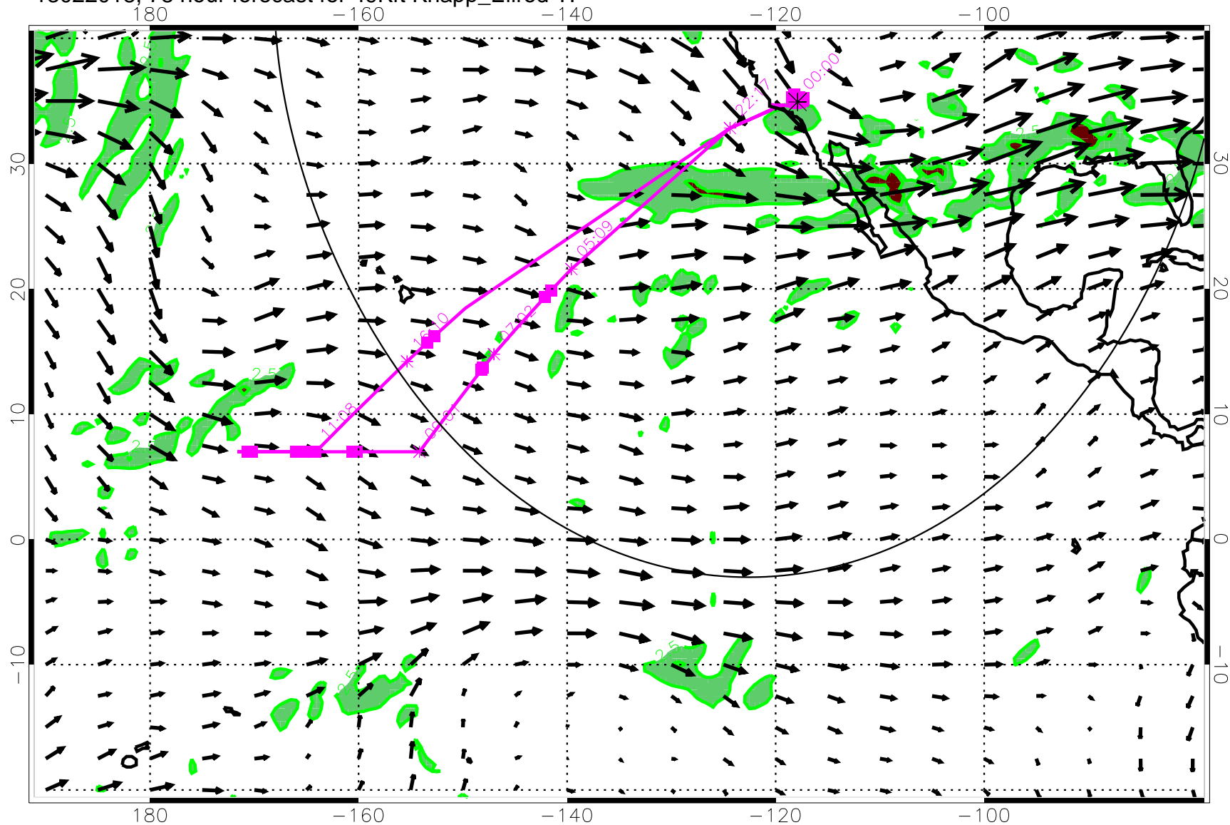
13022018, 78 hour forecast for 49Kft Knapp_Ellrod TI
