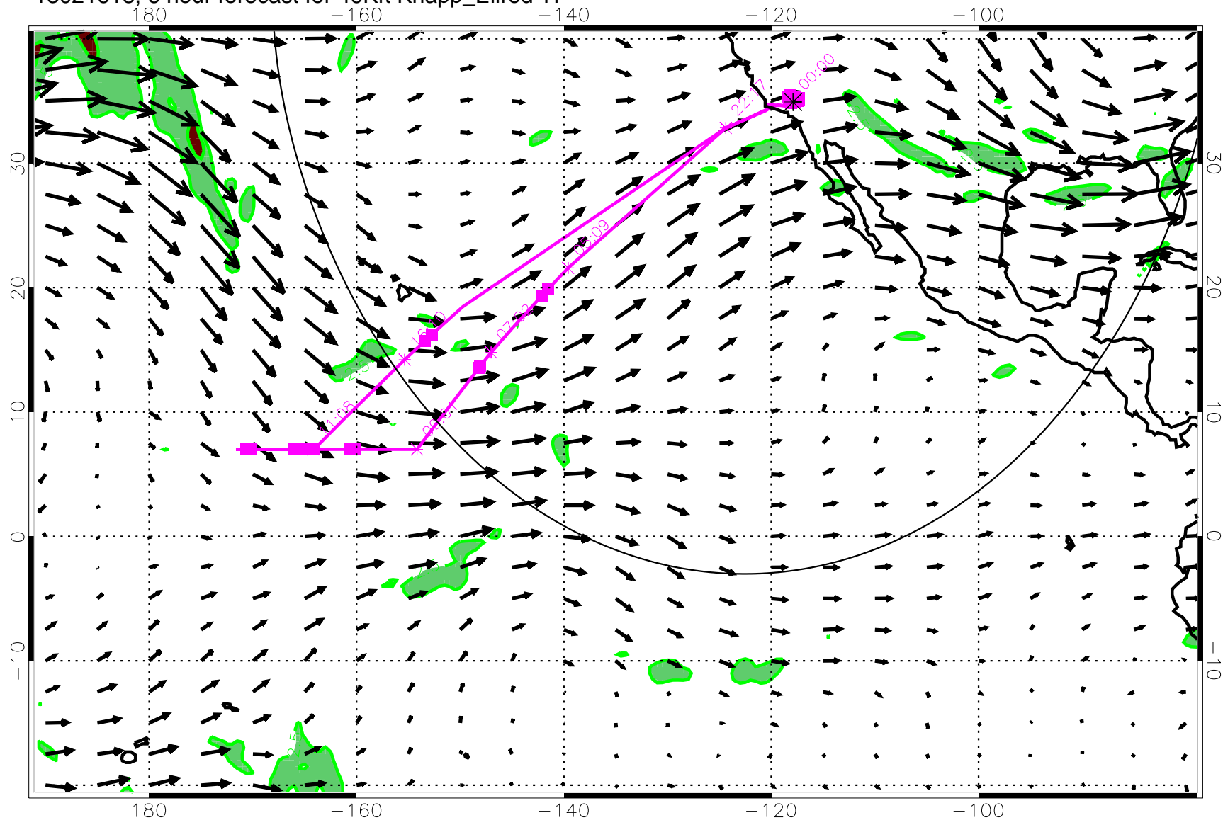
13021618, 6 hour forecast for 49Kft Knapp_Ellrod TI
