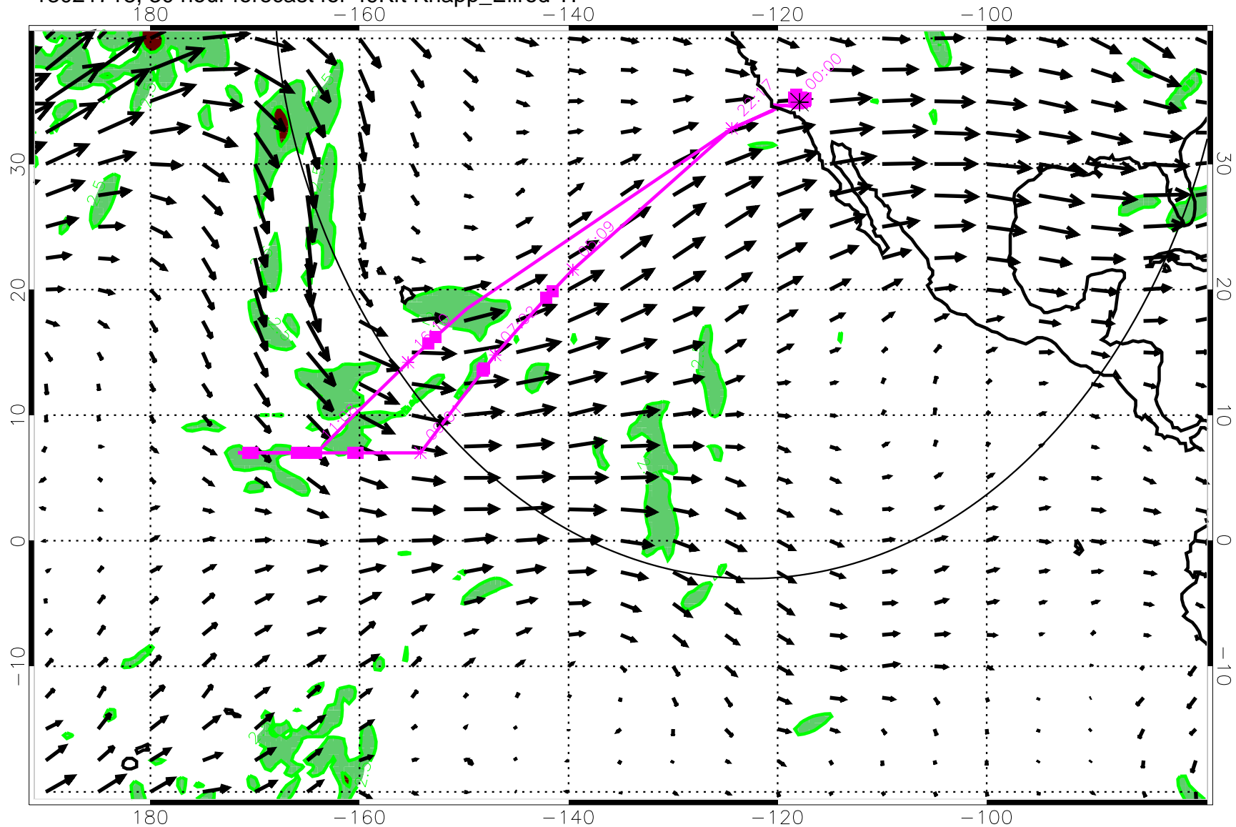
13021718, 30 hour forecast for 49Kft Knapp_Ellrod TI
