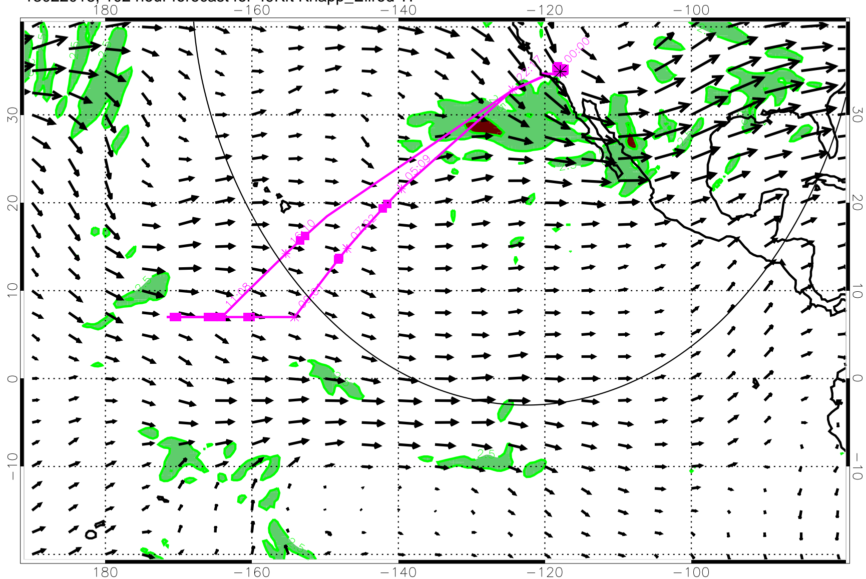
13022018, 102 hour forecast for 49Kft Knapp_Ellrod TI
