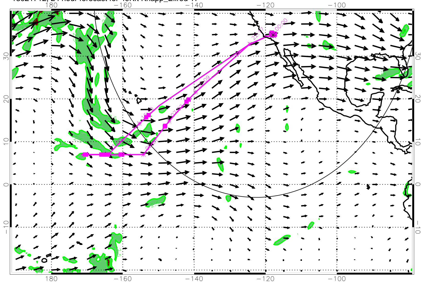
13021712, 24 hour forecast for 49Kft Knapp_Ellrod TI
