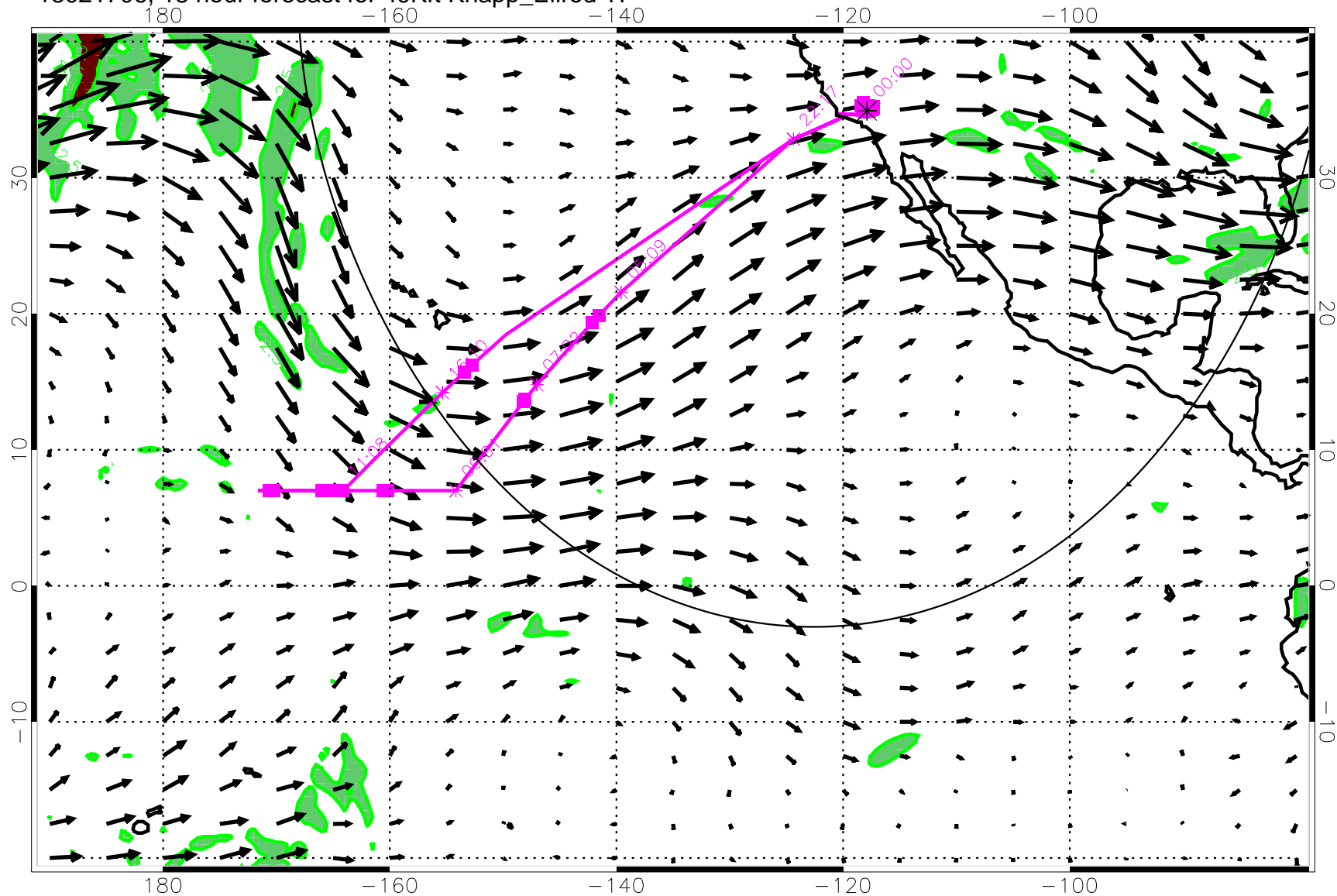
13021706, 18 hour forecast for 49Kft Knapp_Ellrod TI
