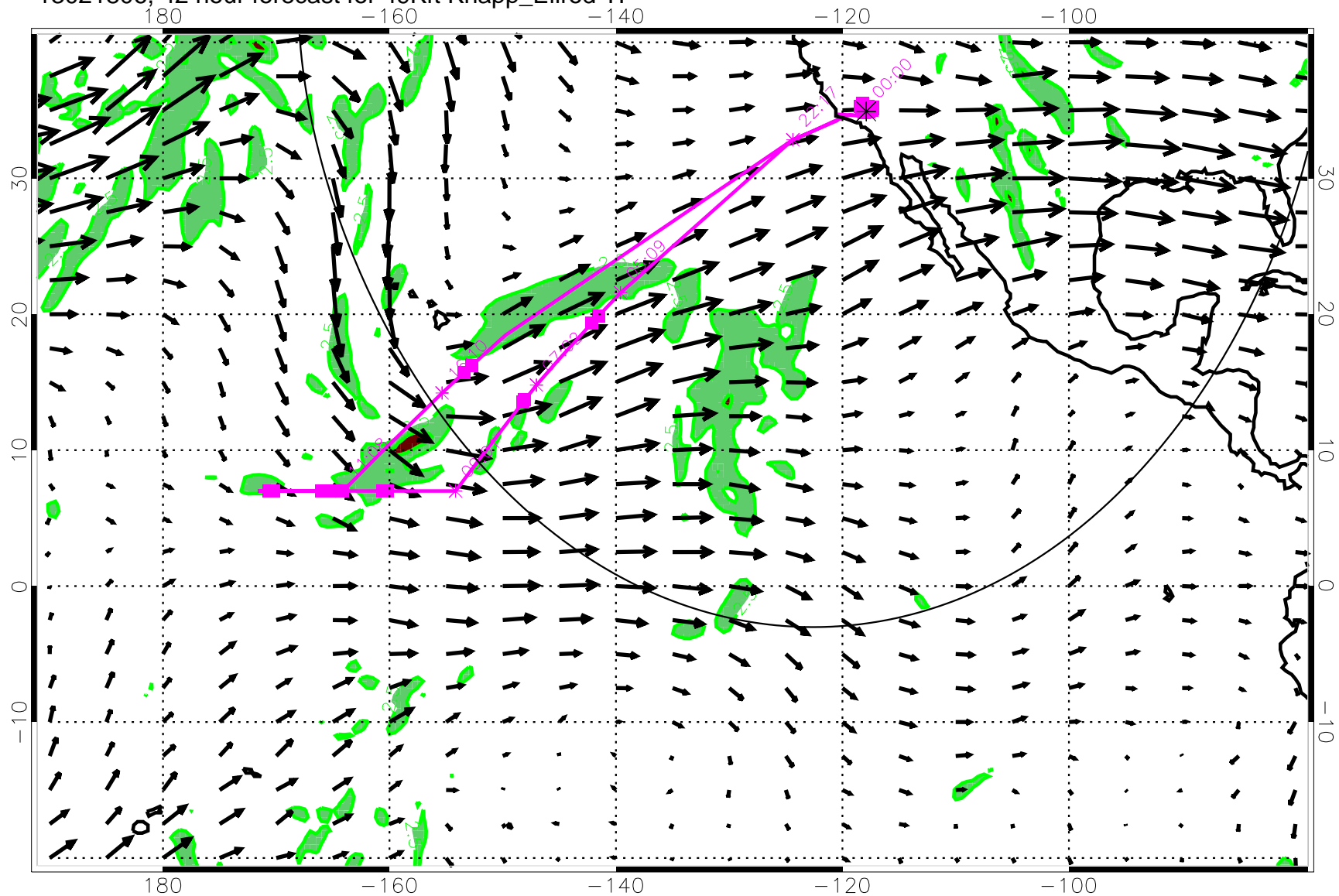
13021806, 42 hour forecast for 49Kft Knapp_Ellrod TI
