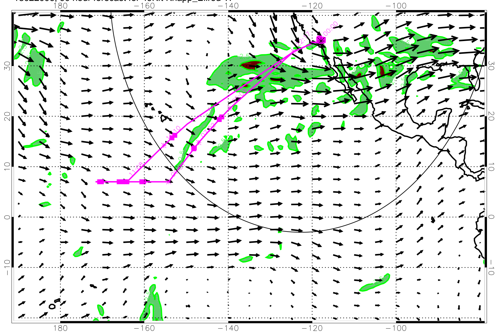
13022006, 90 hour forecast for 49Kft Knapp_Ellrod TI
