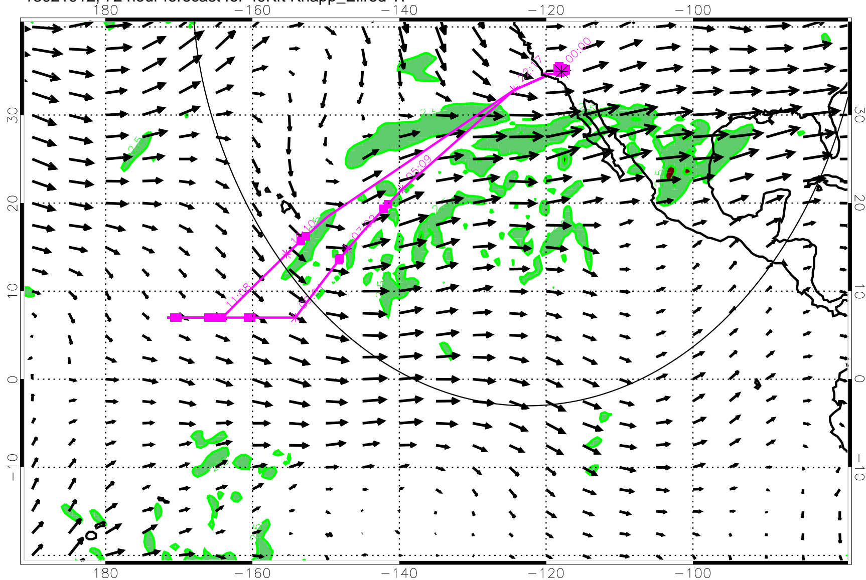
13021912, 72 hour forecast for 49Kft Knapp_Ellrod TI
