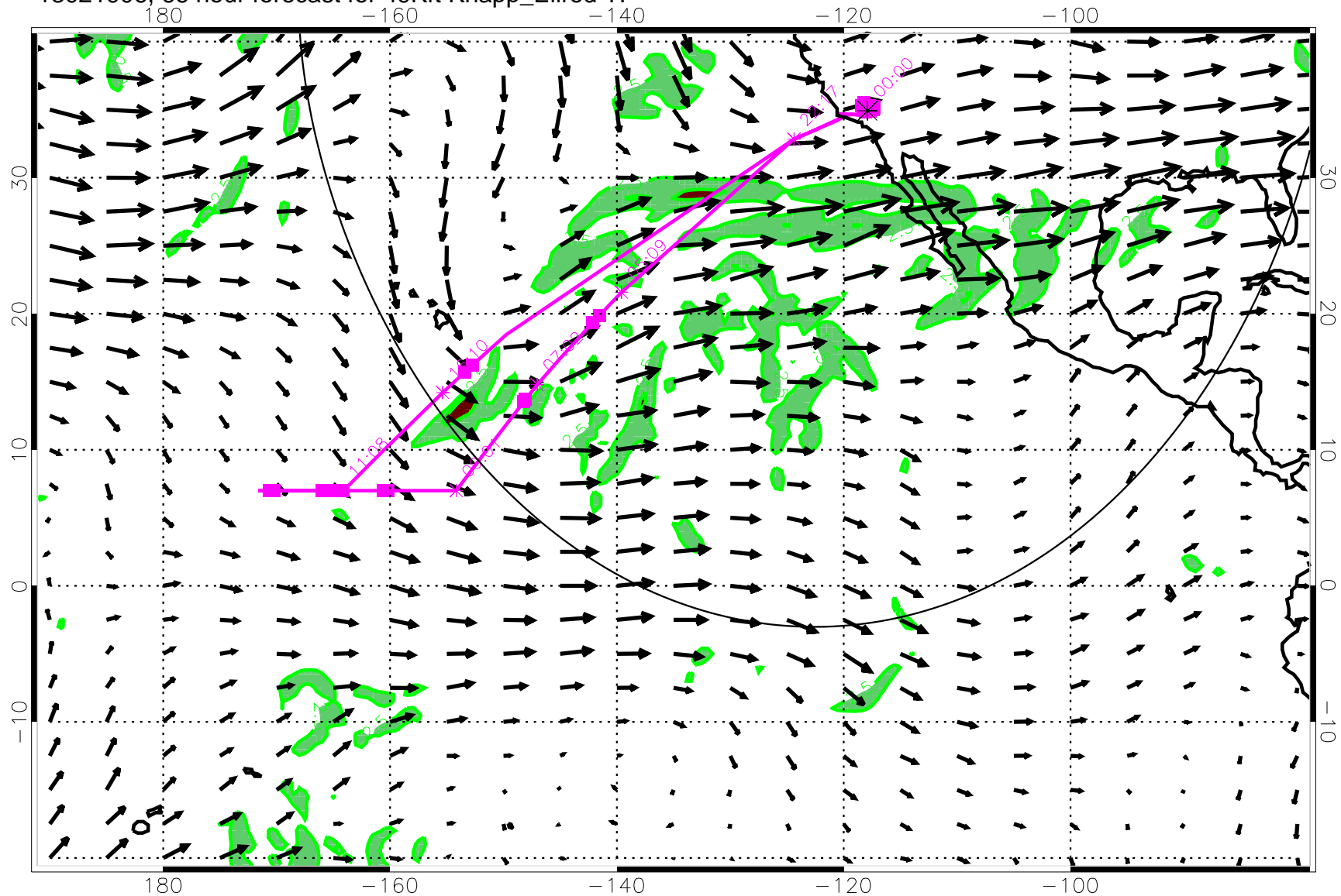
13021906, 66 hour forecast for 49Kft Knapp_Ellrod TI
