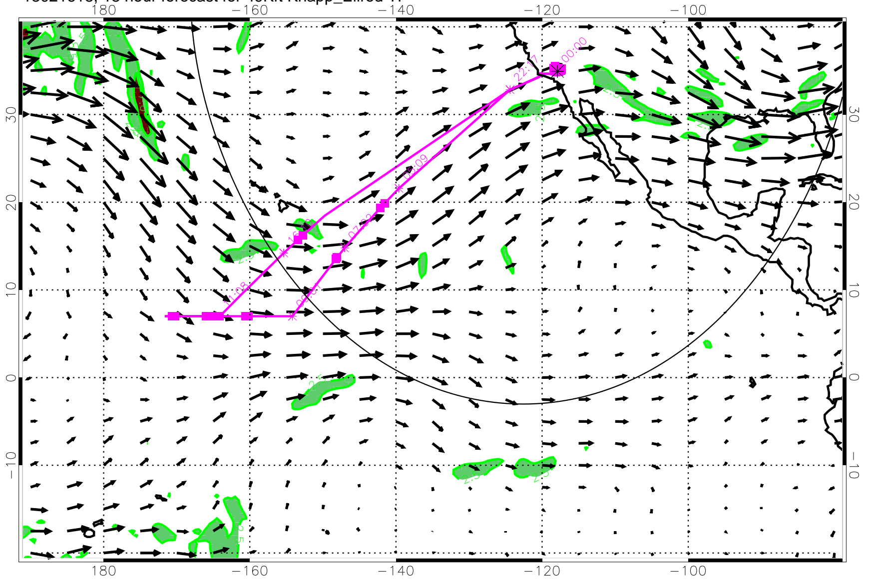
13021618, 18 hour forecast for 49Kft Knapp_Ellrod TI
