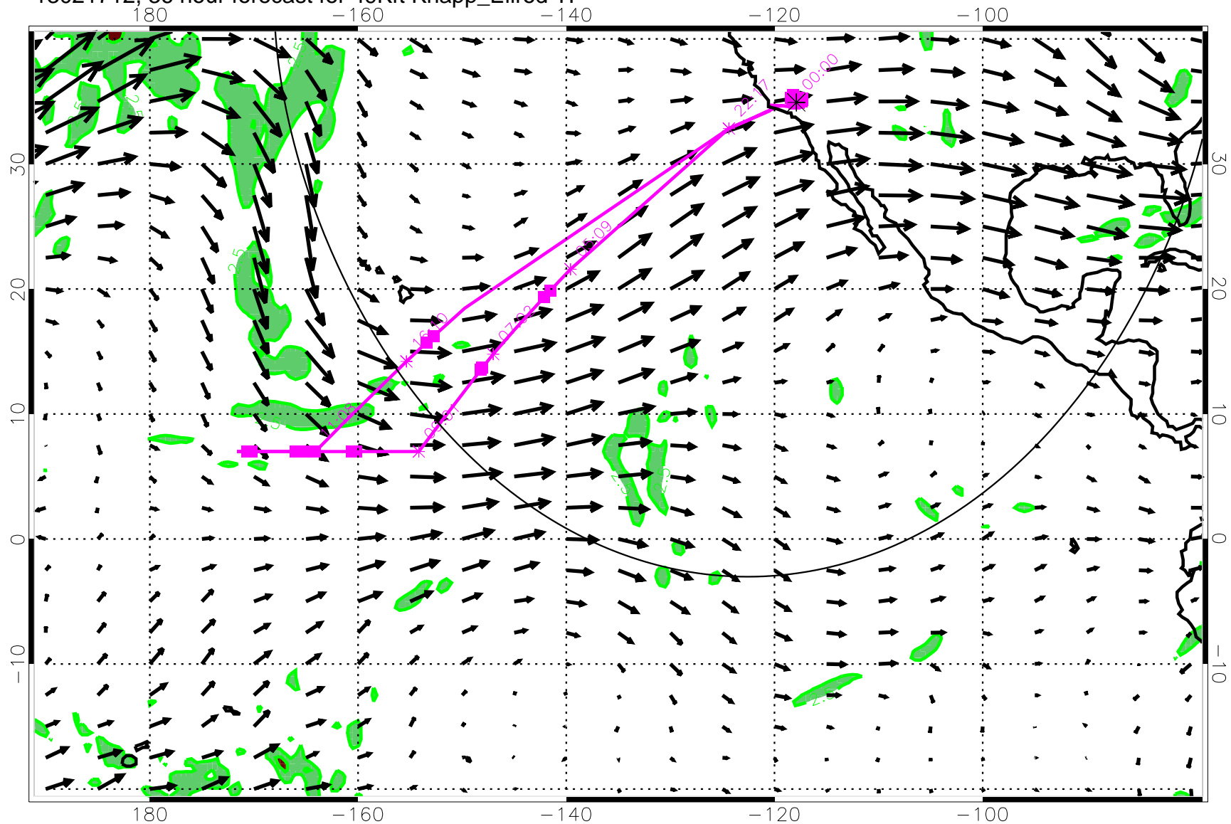
13021712, 36 hour forecast for 49Kft Knapp_Ellrod TI
