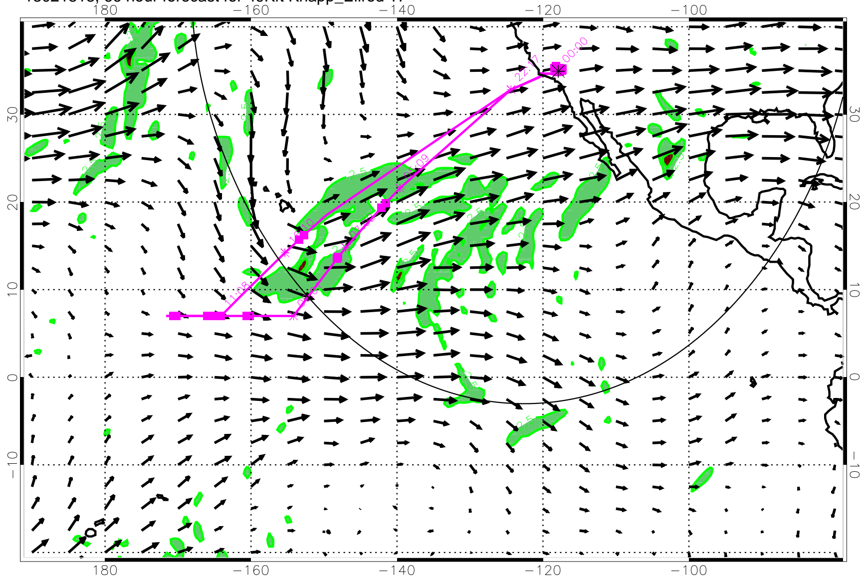
13021818, 66 hour forecast for 49Kft Knapp_Ellrod TI
