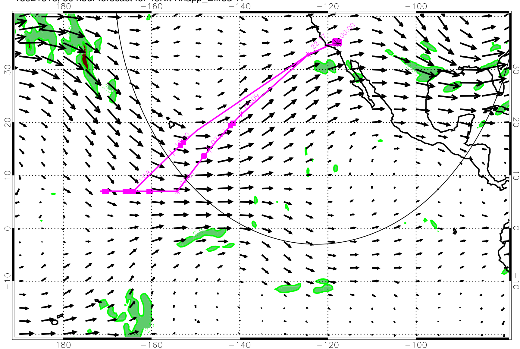
13021618, 30 hour forecast for 49Kft Knapp_Ellrod TI
