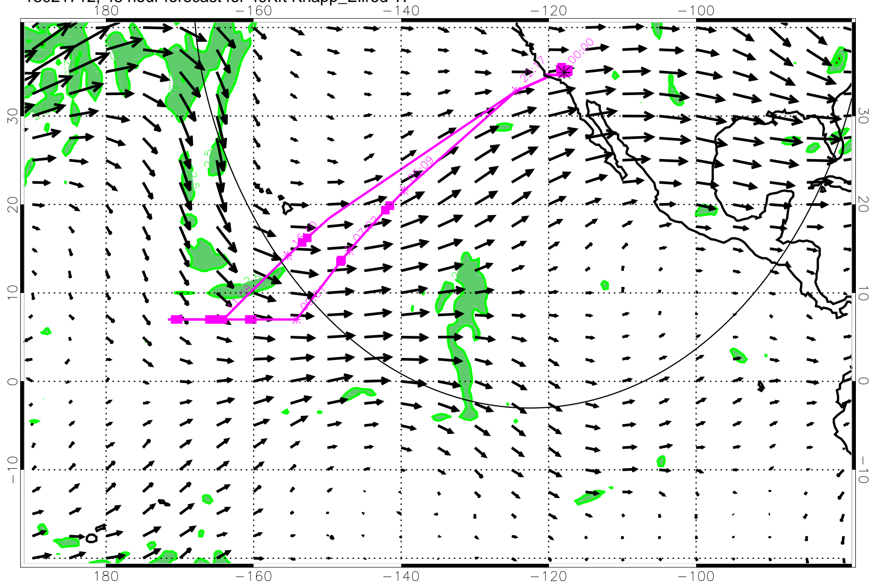
13021712, 48 hour forecast for 49Kft Knapp_Ellrod TI
