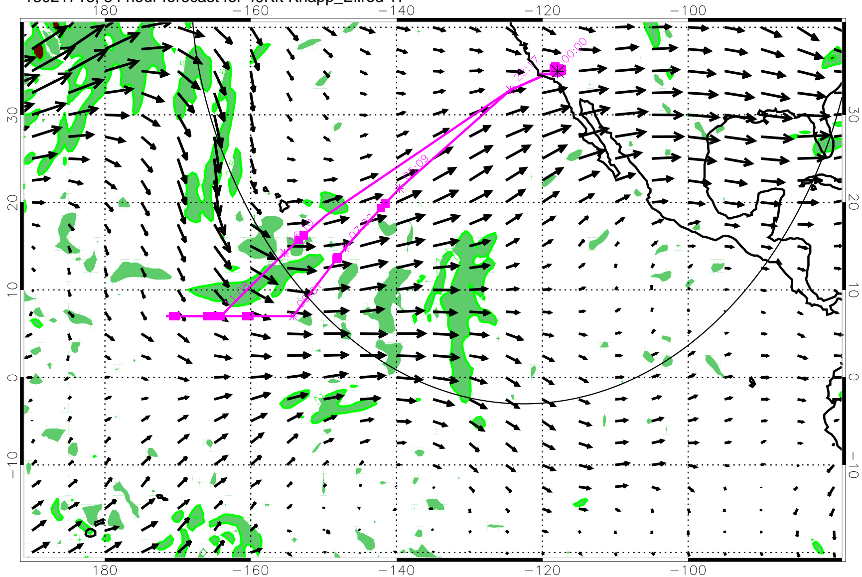
13021718, 54 hour forecast for 49Kft Knapp_Ellrod TI
