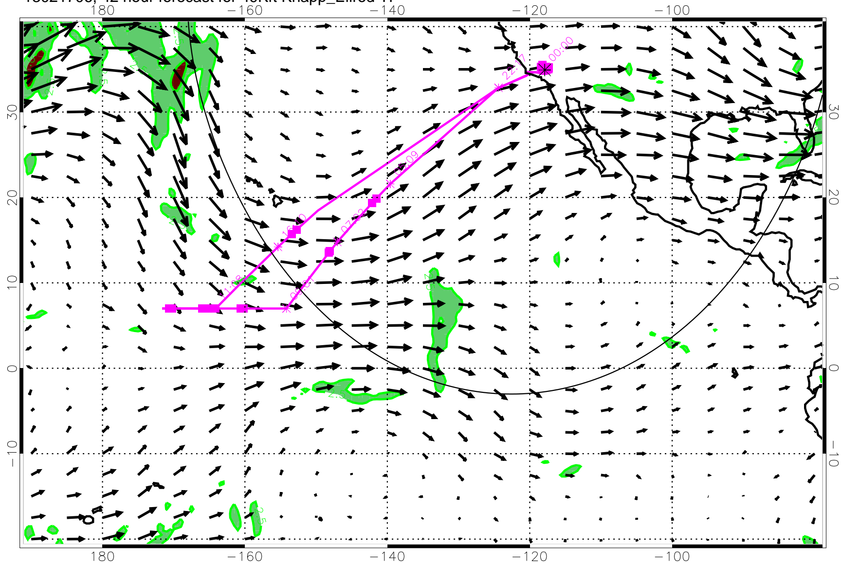
13021706, 42 hour forecast for 49Kft Knapp_Ellrod TI
