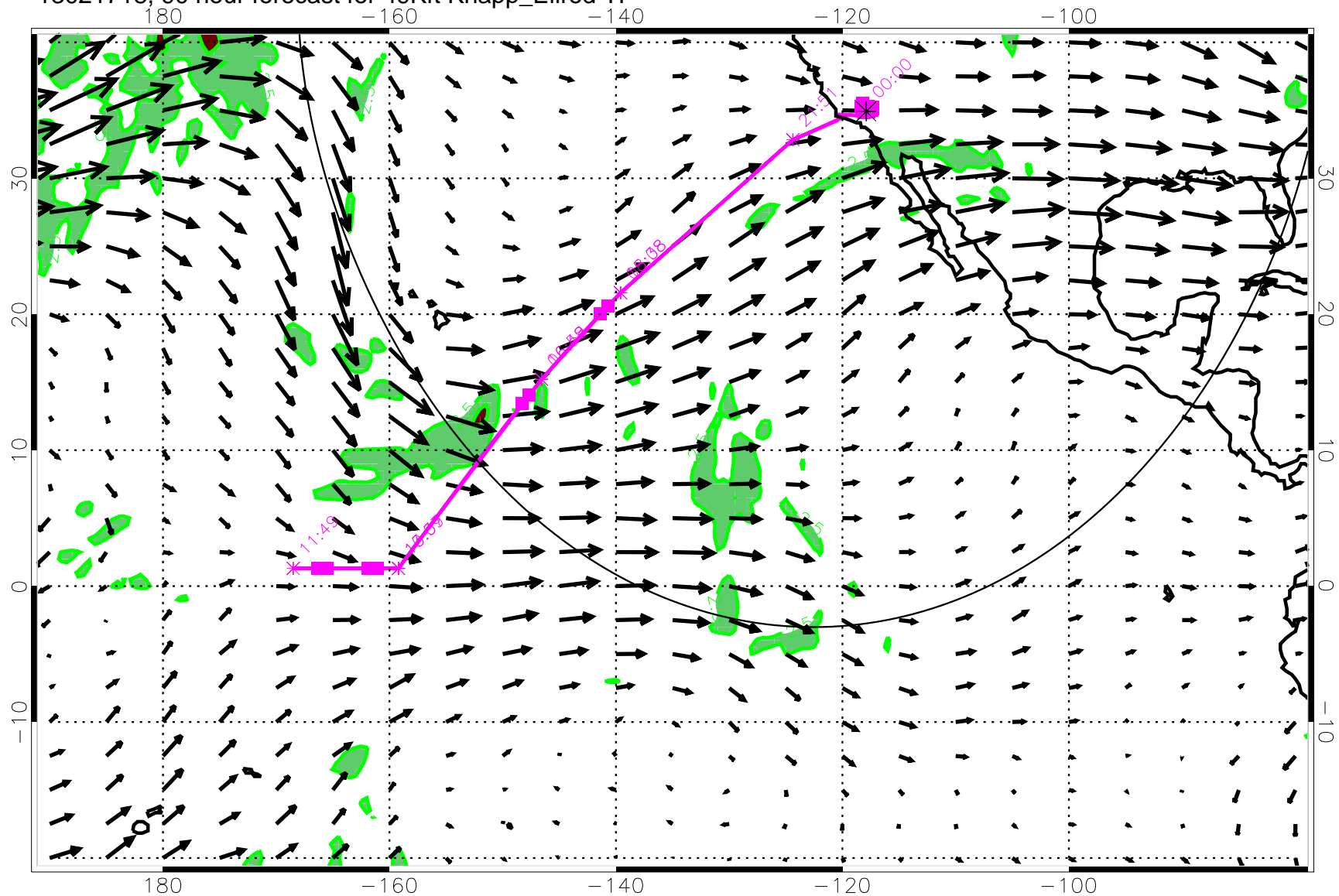
13021718, 90 hour forecast for 49Kft Knapp_Ellrod TI
