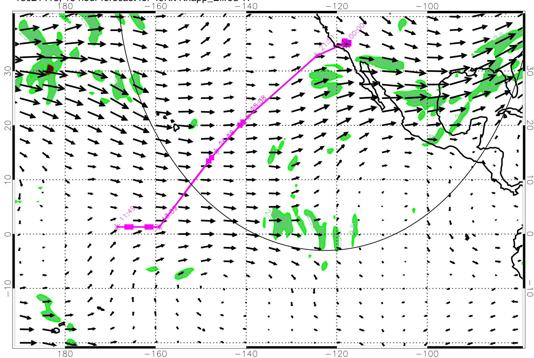
13021418, 18 hour forecast for 49Kft Knapp_Ellrod TI
