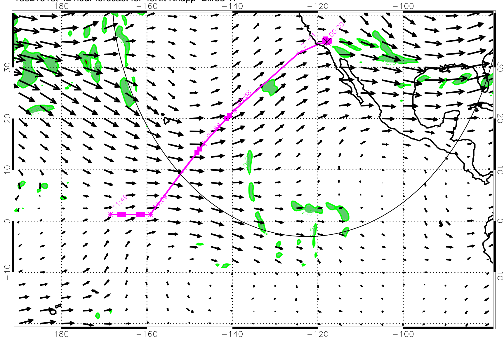
13021518, 42 hour forecast for 49Kft Knapp_Ellrod TI
