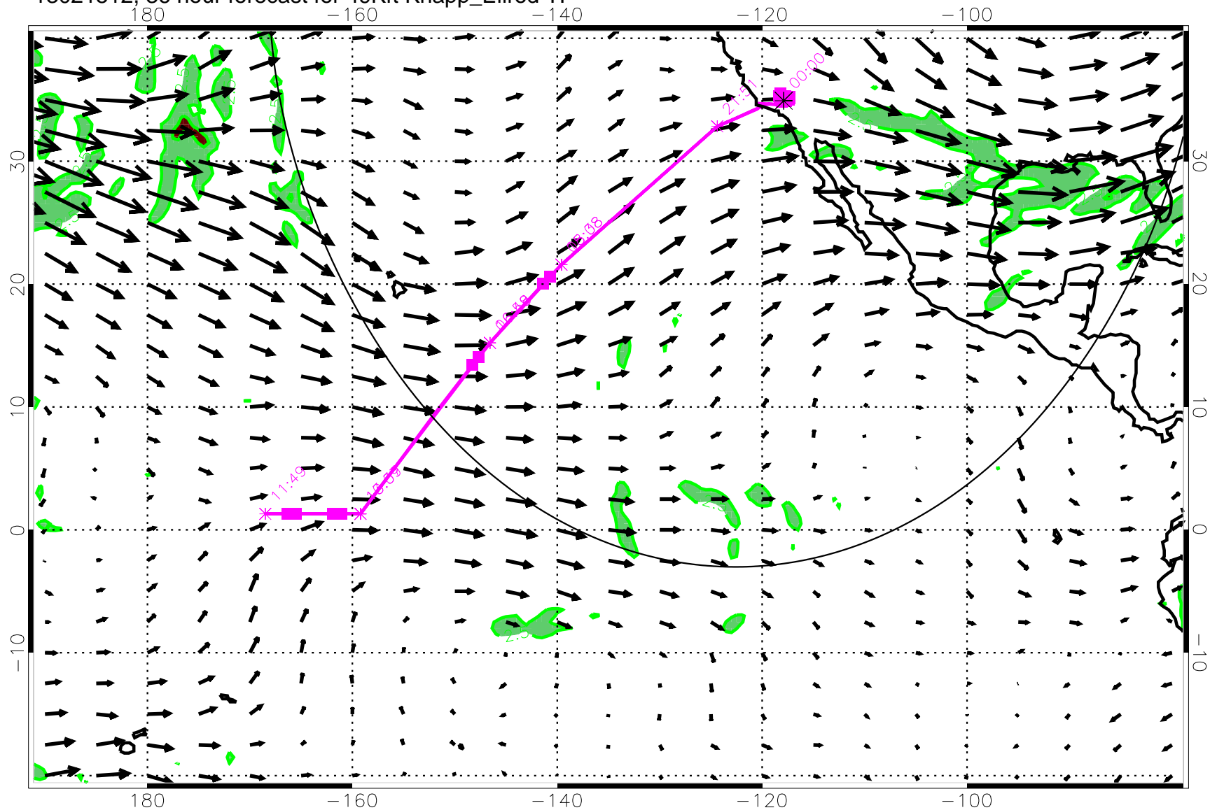
13021512, 36 hour forecast for 49Kft Knapp_Ellrod TI
