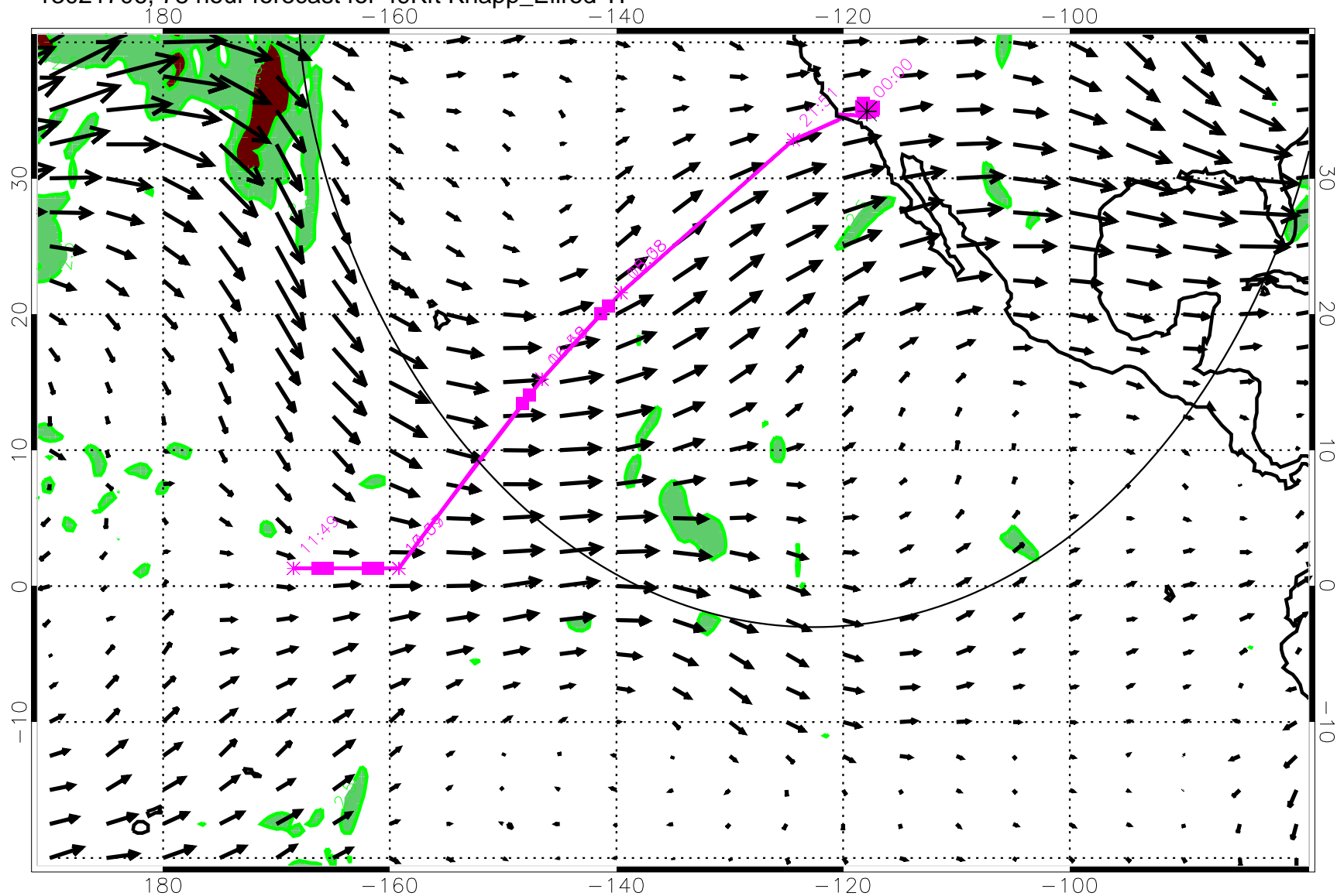
13021706, 78 hour forecast for 49Kft Knapp_Ellrod TI
