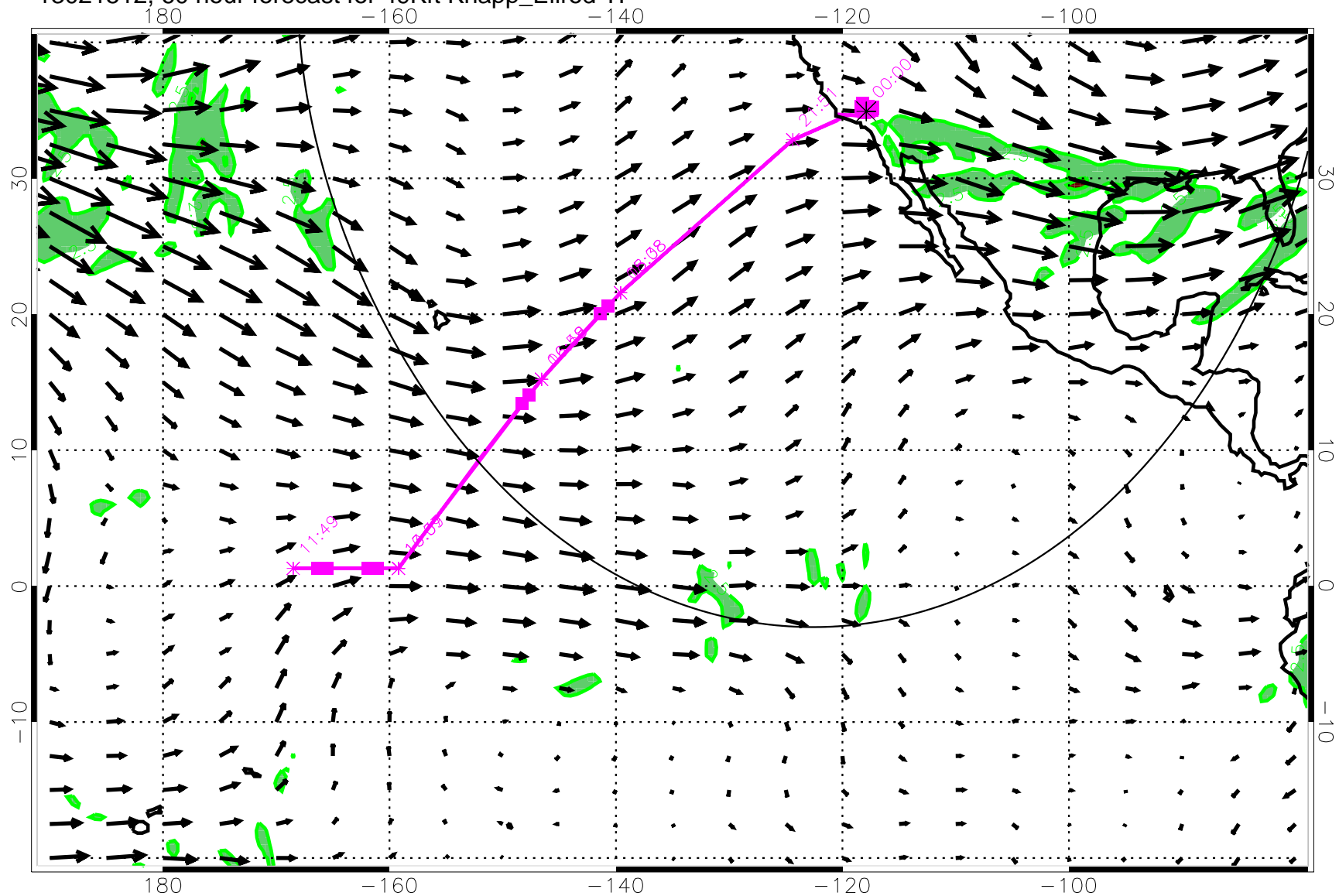
13021512, 60 hour forecast for 49Kft Knapp_Ellrod TI
