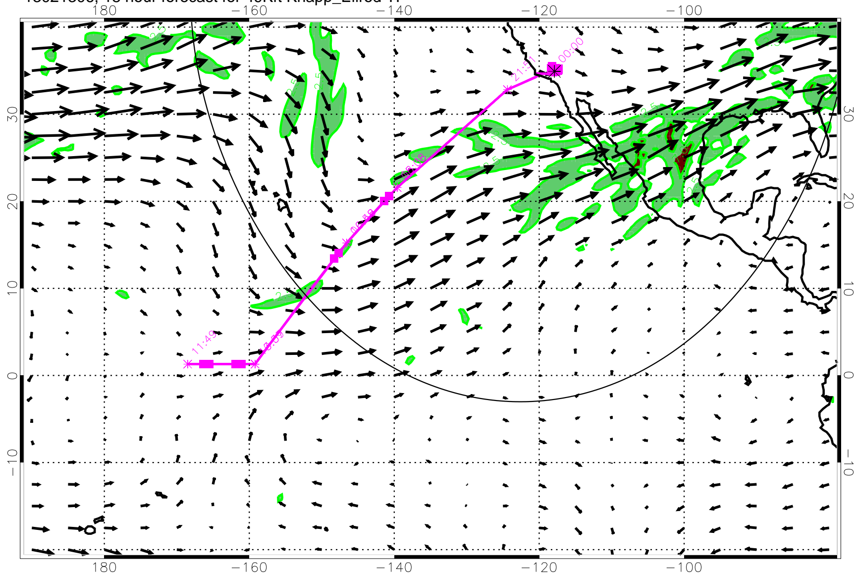
13021306, 18 hour forecast for 49Kft Knapp_Ellrod TI
