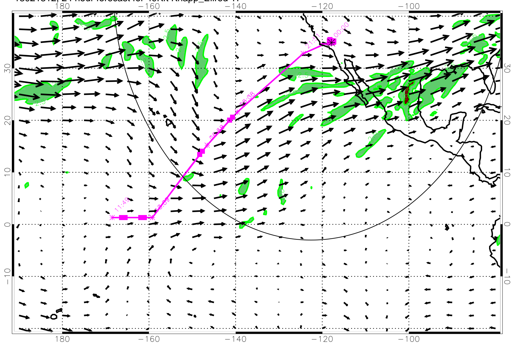
13021312, 24 hour forecast for 49Kft Knapp_Ellrod TI
