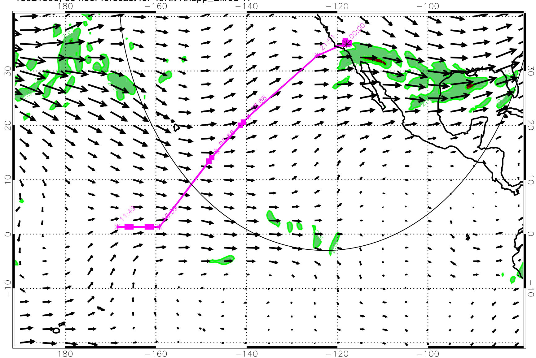
13021506, 66 hour forecast for 49Kft Knapp_Ellrod TI
