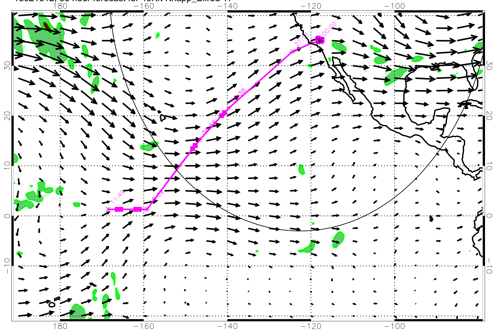
13021612, 96 hour forecast for 49Kft Knapp_Ellrod TI
