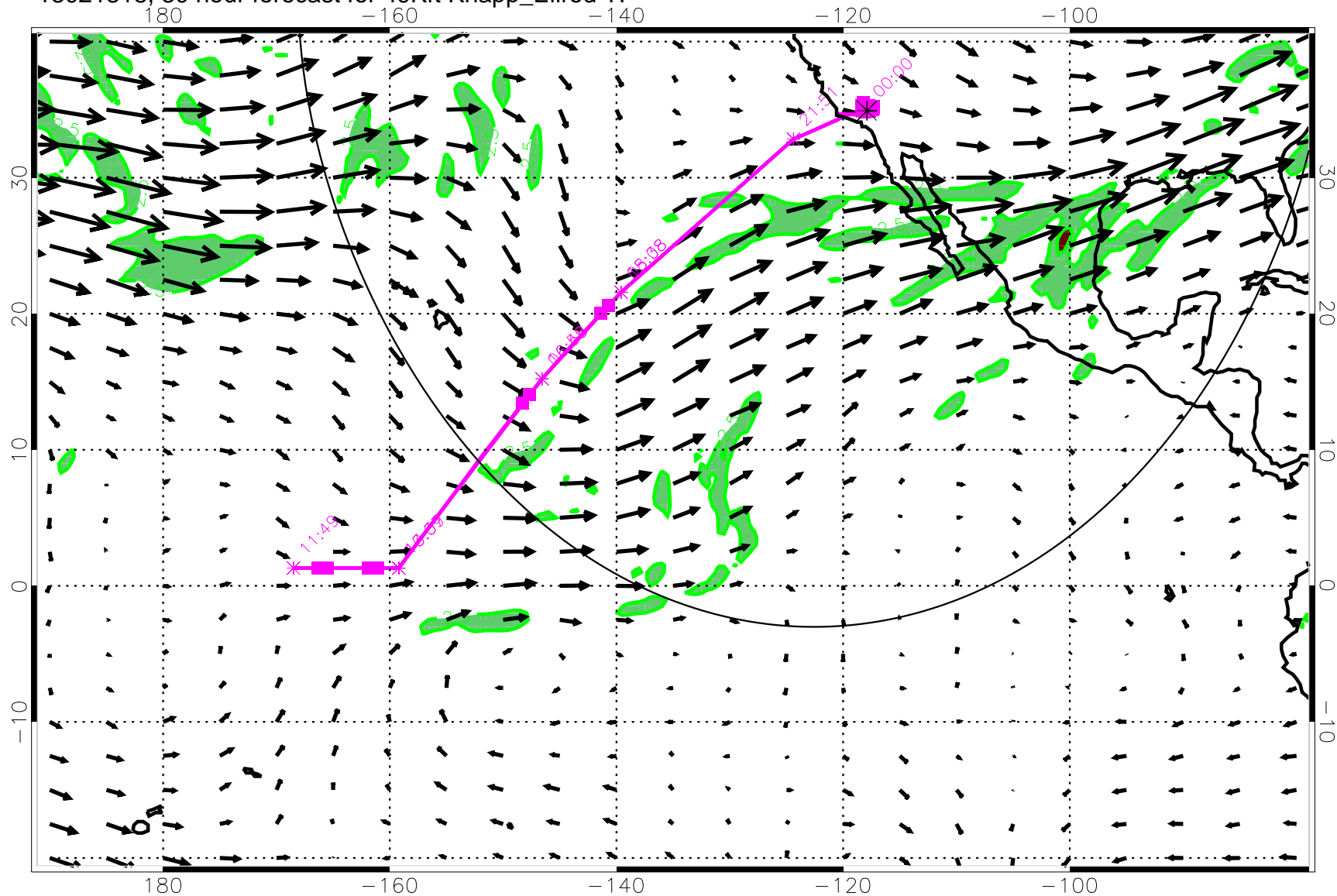
13021318, 30 hour forecast for 49Kft Knapp_Ellrod TI
