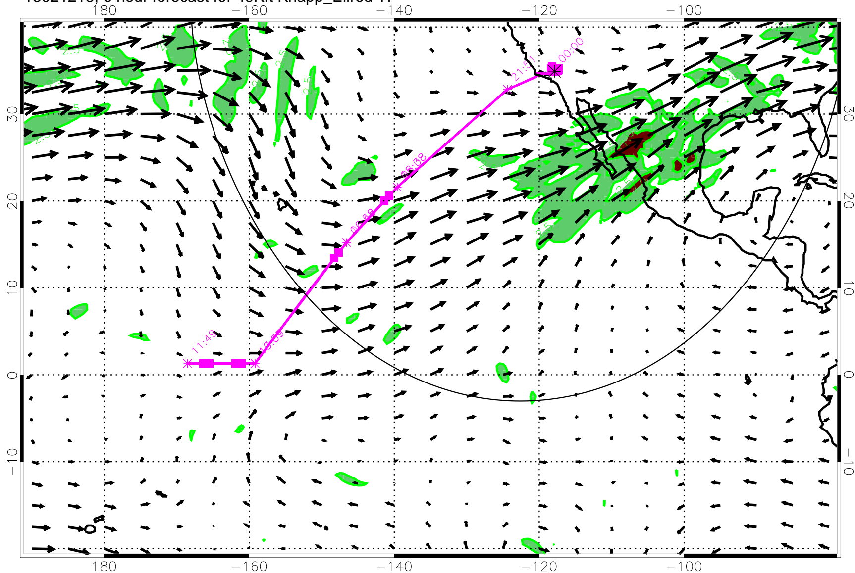
13021218, 6 hour forecast for 49Kft Knapp_Ellrod TI
