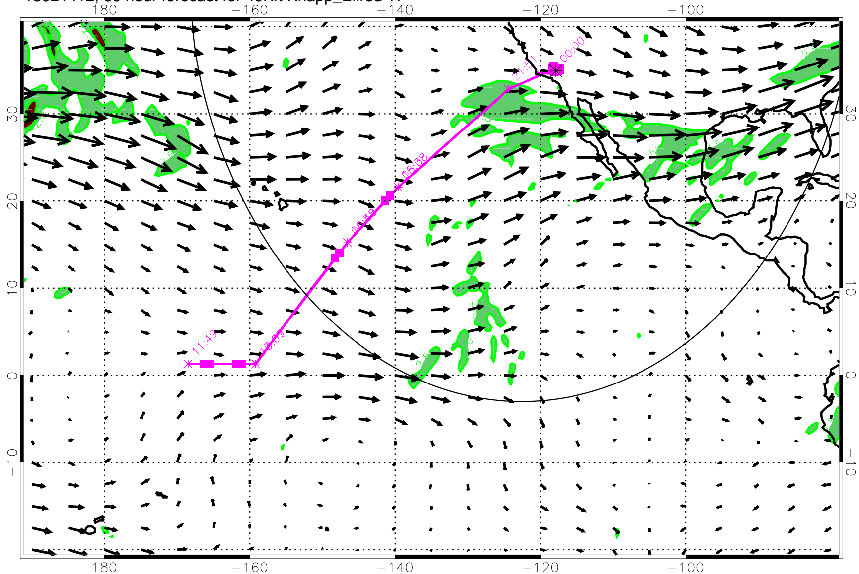
13021412, 60 hour forecast for 49Kft Knapp_Ellrod TI
