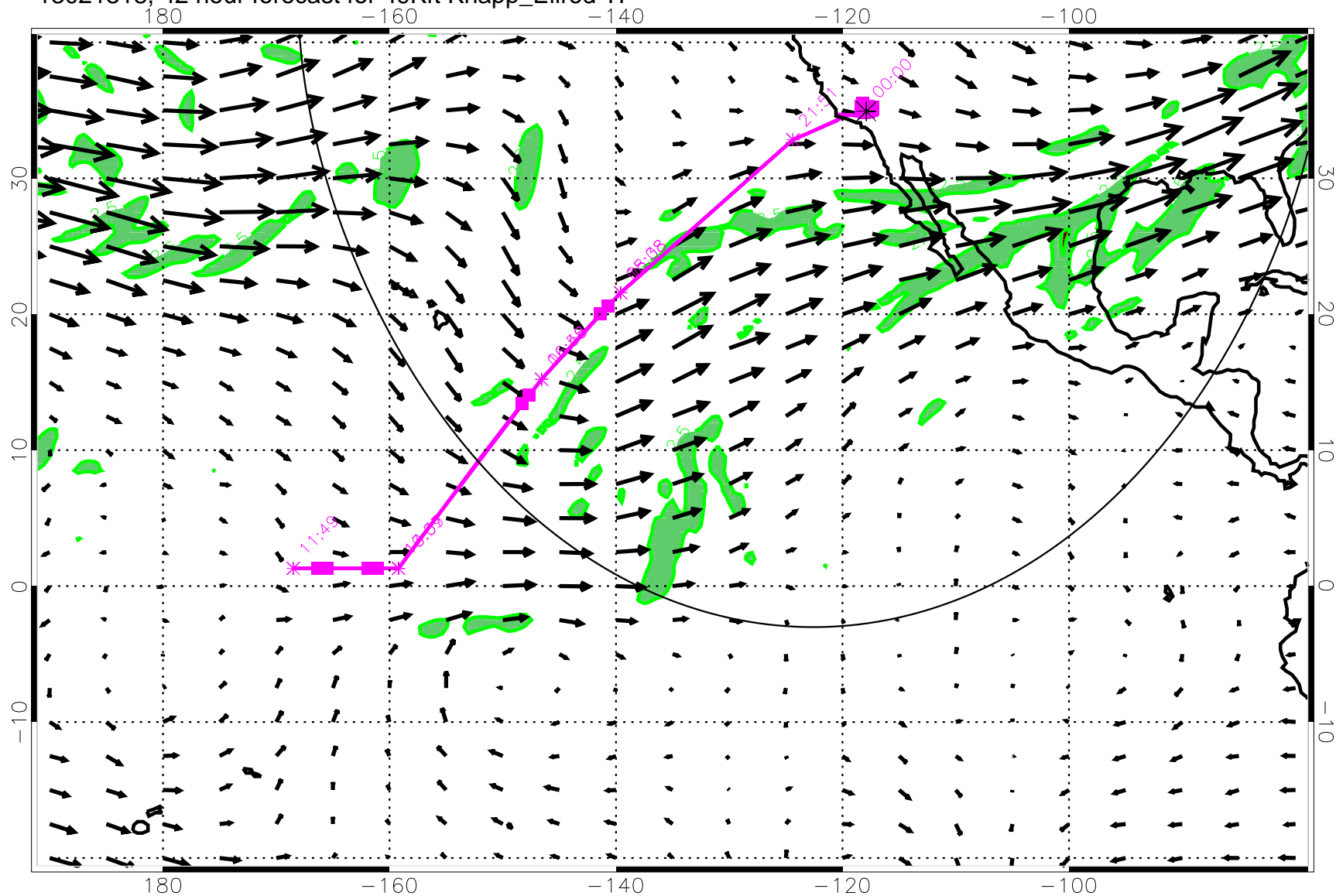
13021318, 42 hour forecast for 49Kft Knapp_Ellrod TI
