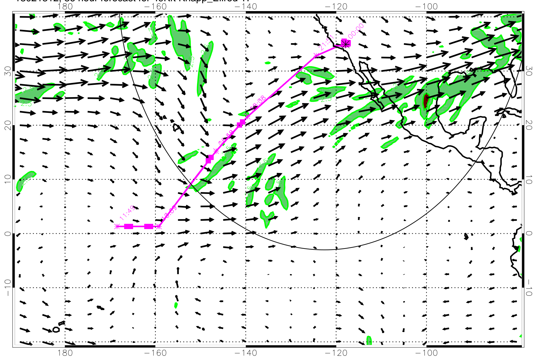
13021312, 36 hour forecast for 49Kft Knapp_Ellrod TI
