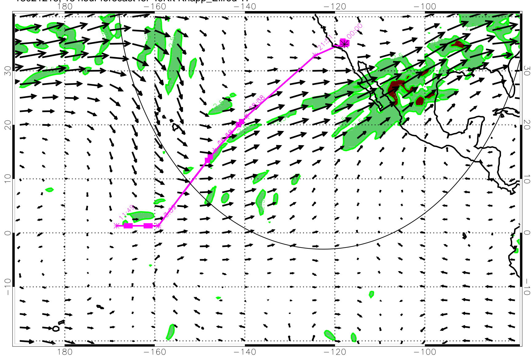
13021218, 18 hour forecast for 49Kft Knapp_Ellrod TI
