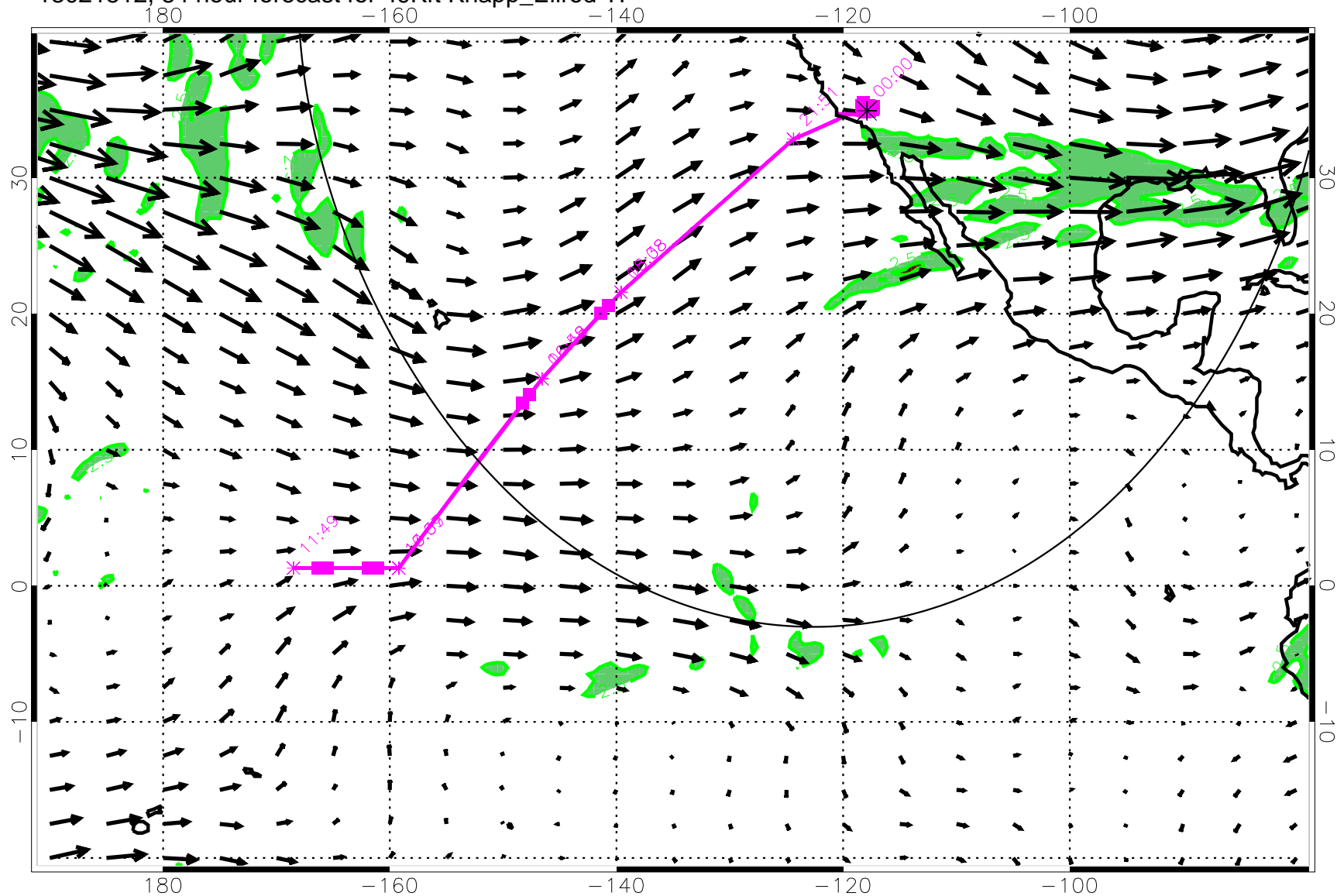
13021512, 84 hour forecast for 49Kft Knapp_Ellrod TI
