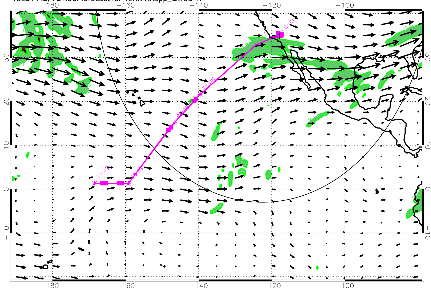
13021412, 72 hour forecast for 49Kft Knapp_Ellrod TI
