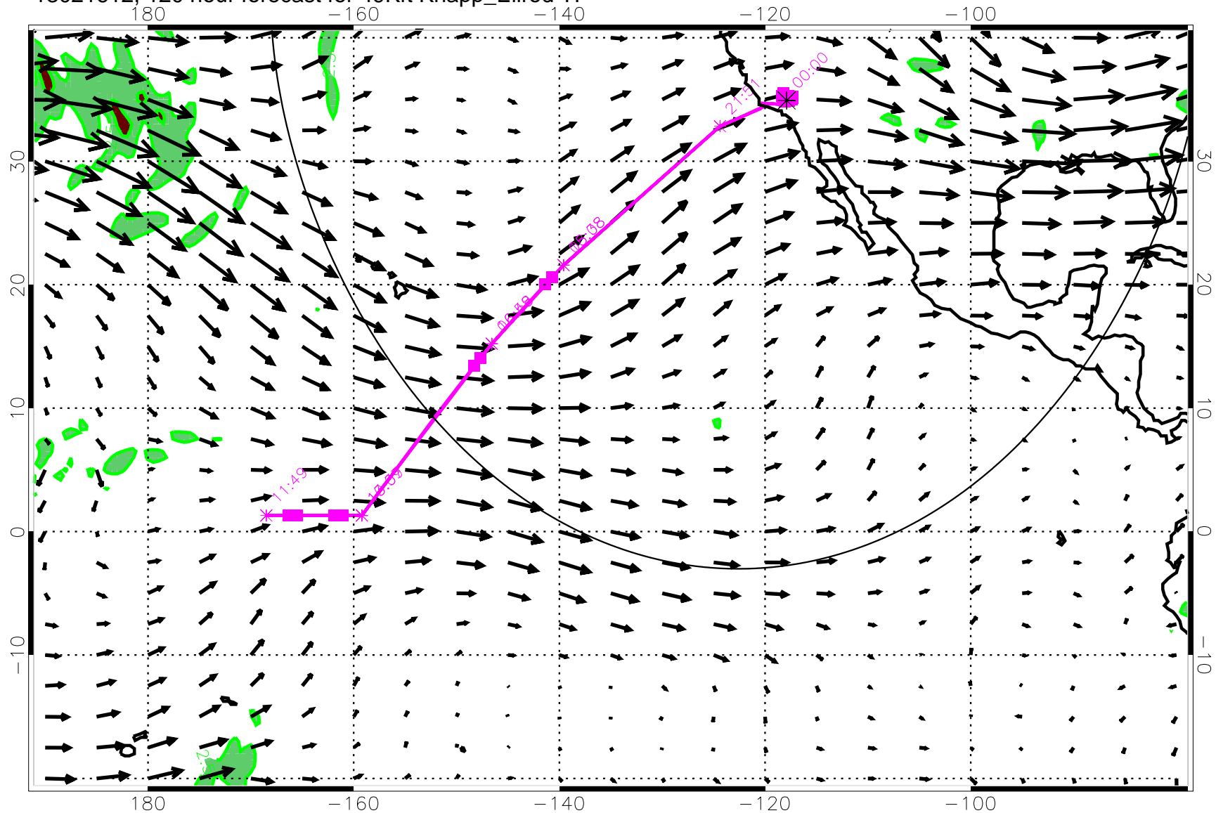
13021612, 120 hour forecast for 49Kft Knapp_Ellrod T1
