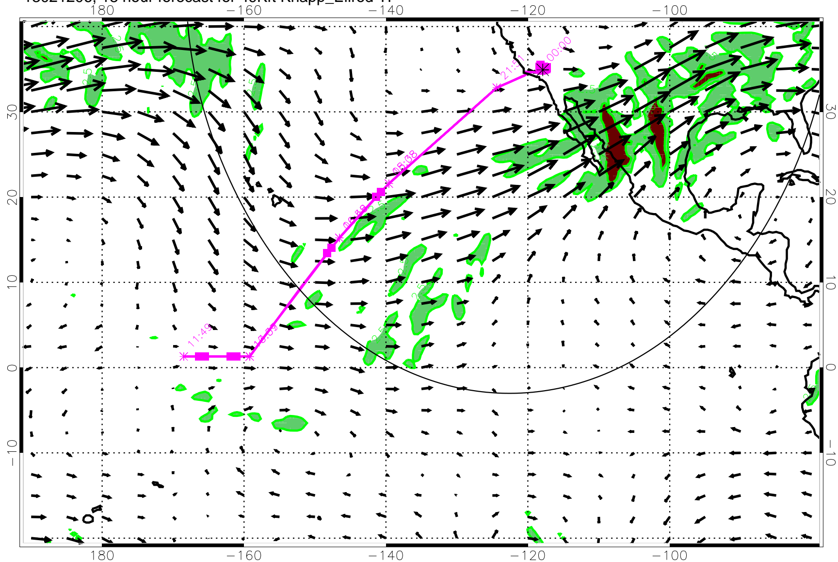
13021206, 18 hour forecast for 49Kft Knapp_Ellrod TI
