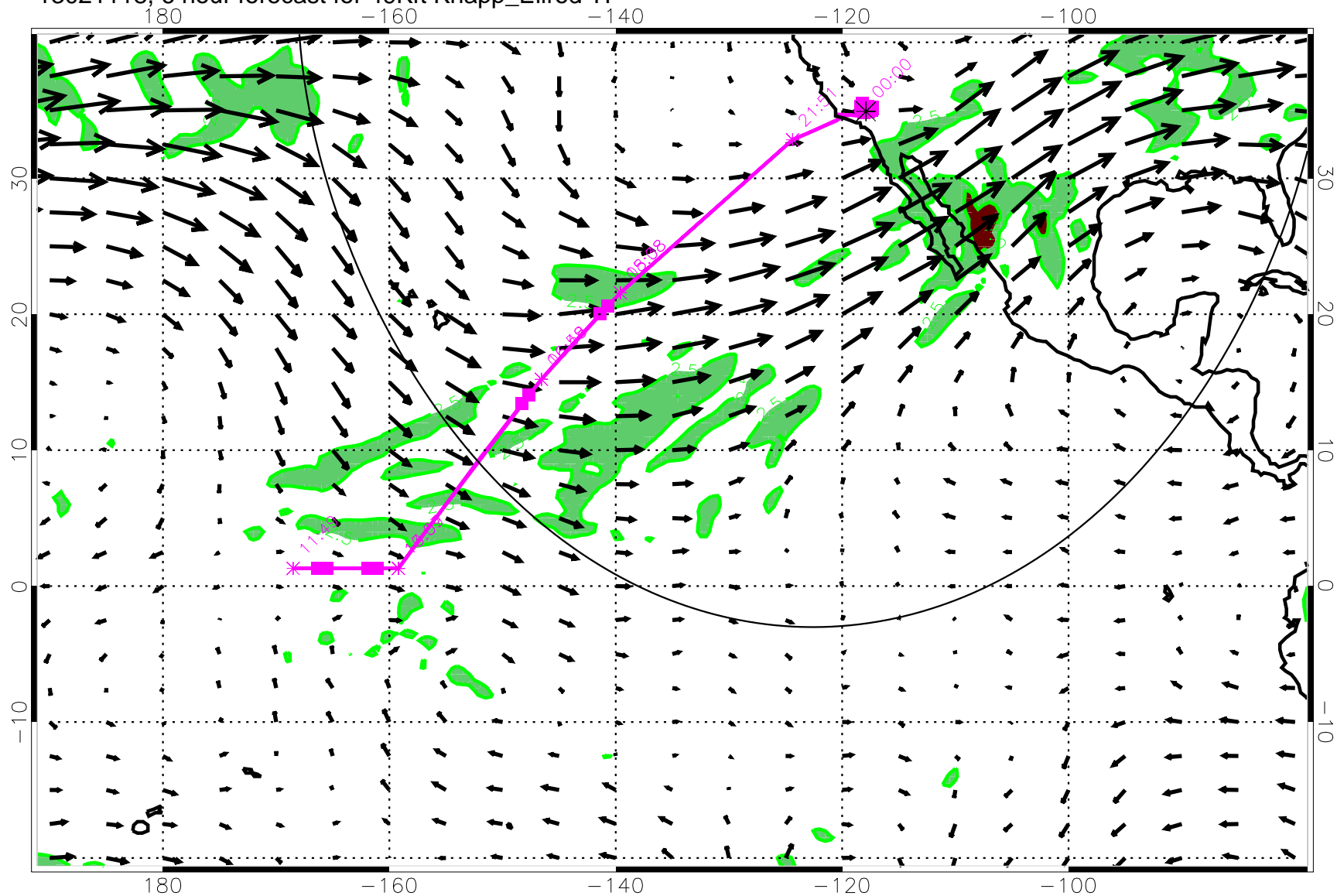
13021118, 6 hour forecast for 49Kft Knapp_Ellrod TI
