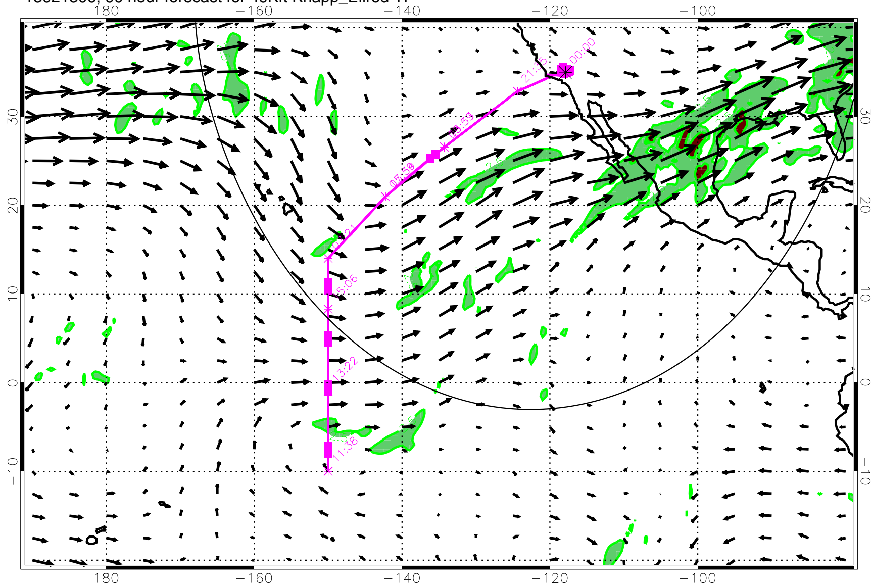
13021306, 90 hour forecast for 49Kft Knapp_Ellrod TI
