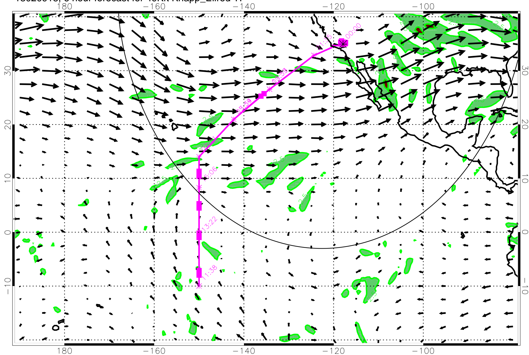
13020918, 6 hour forecast for 49Kft Knapp_Ellrod TI
