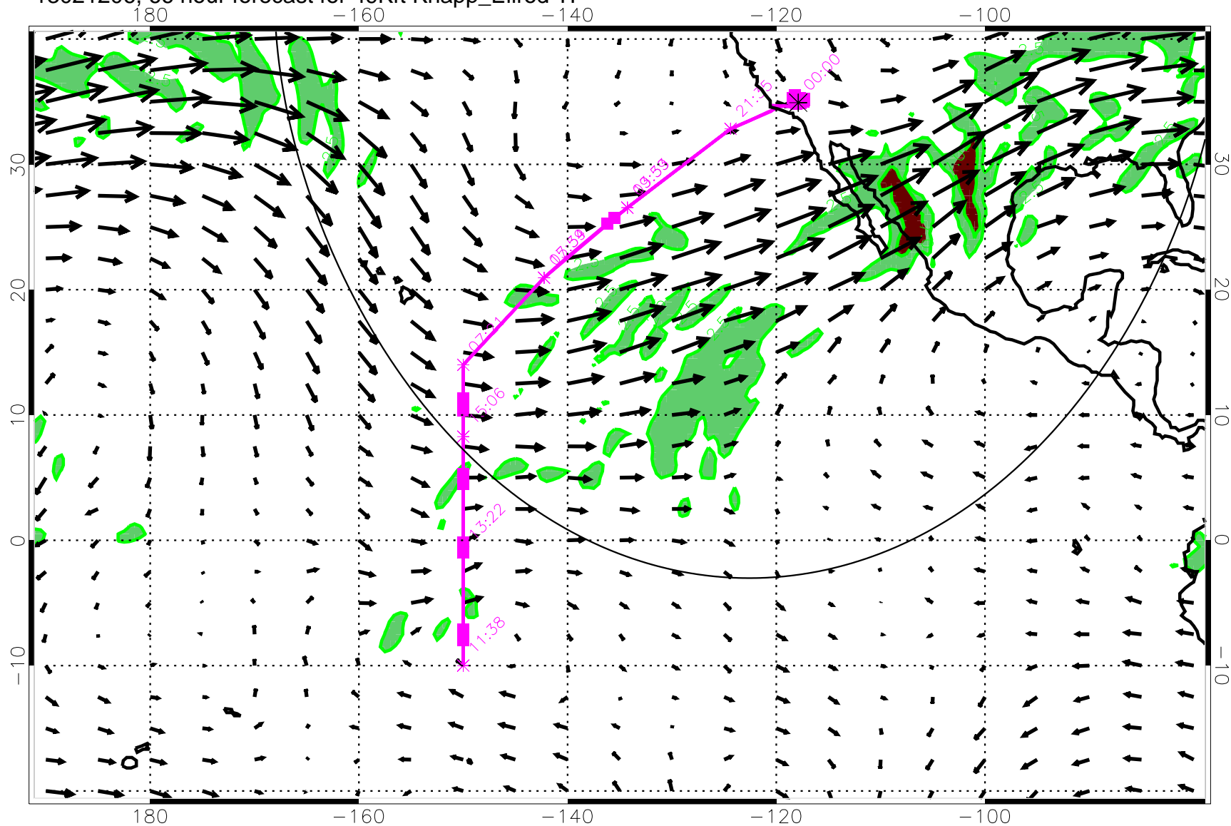
13021206, 66 hour forecast for 49Kft Knapp_Ellrod TI
