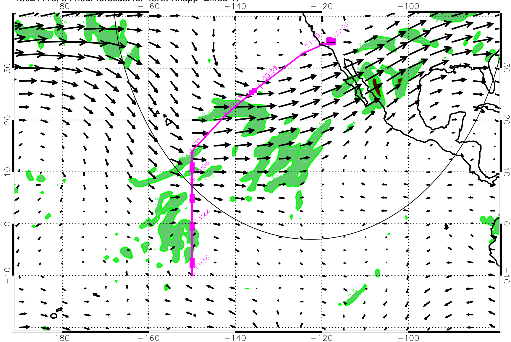
13021118, 54 hour forecast for 49Kft Knapp_Ellrod TI
