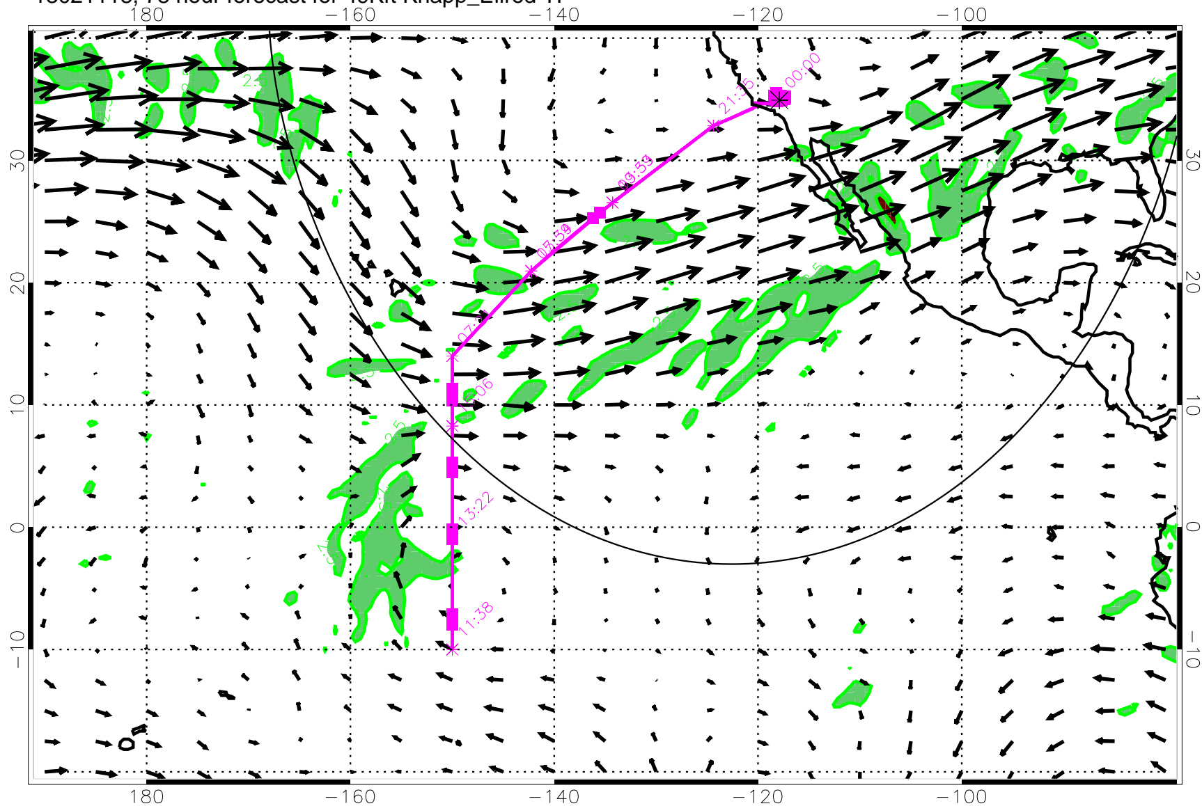
13021118, 78 hour forecast for 49Kft Knapp_Ellrod TI
