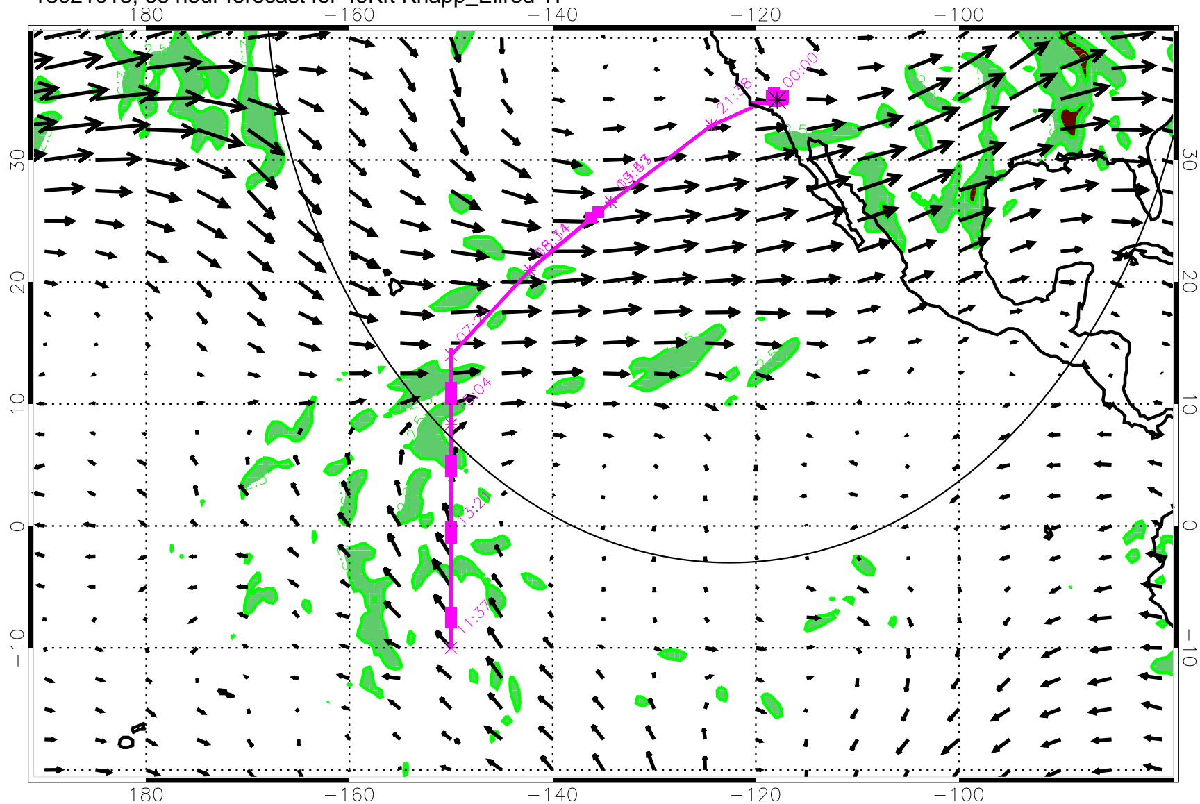
13021018, 66 hour forecast for 49Kft Knapp_Ellrod TI
