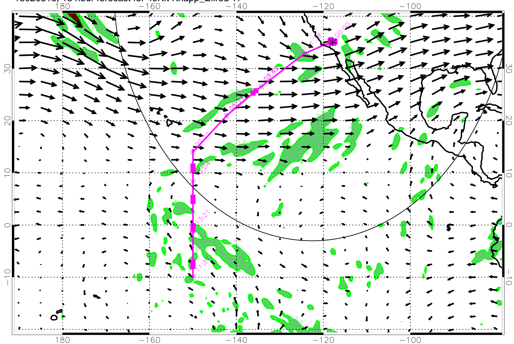
13020818, 18 hour forecast for 49Kft Knapp_Ellrod TI
