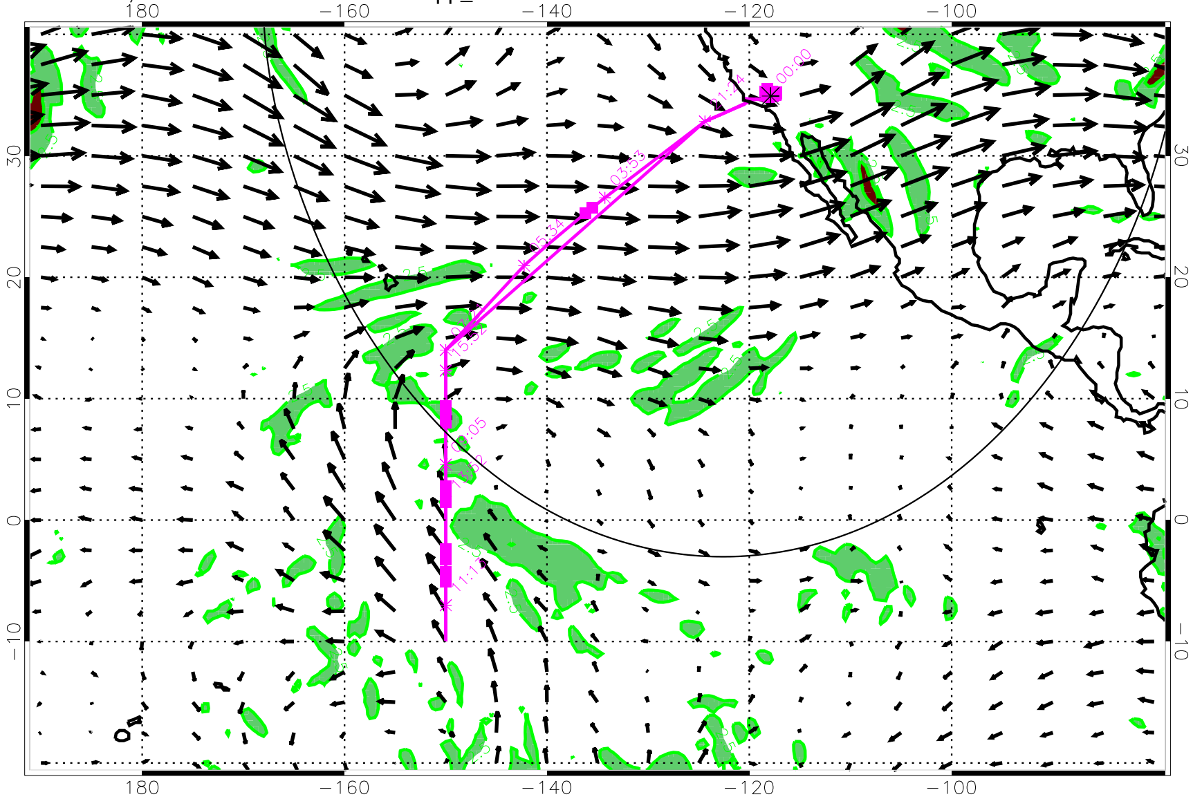
13020912, 72 hour forecast for 49Kft Knapp_Ellrod TI
