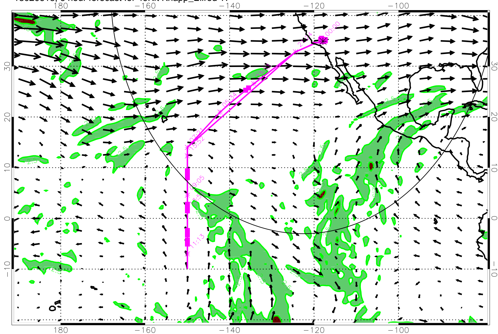
13020618, 6 hour forecast for 49Kft Knapp_Ellrod TI
