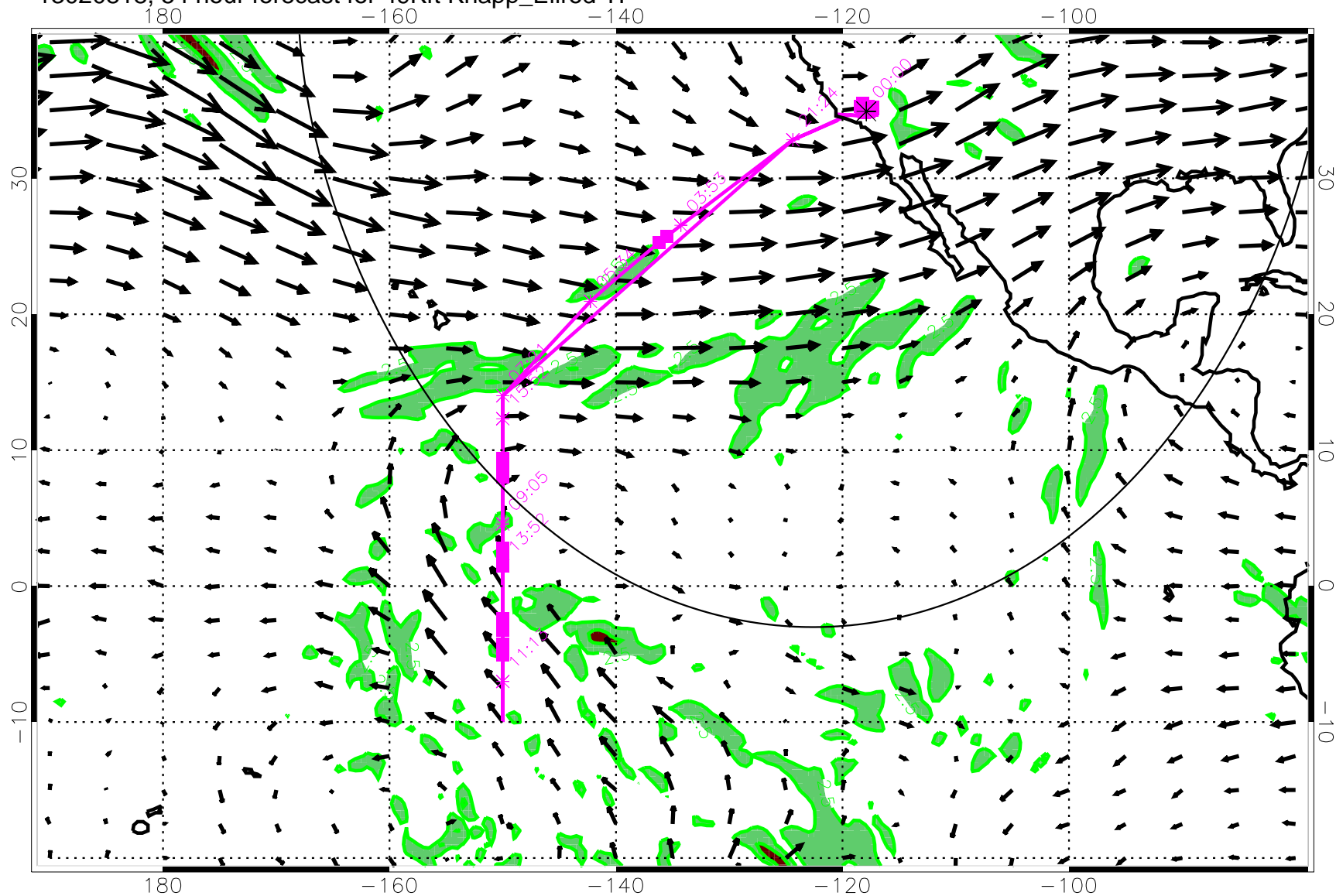
13020818, 54 hour forecast for 49Kft Knapp_Ellrod TI
