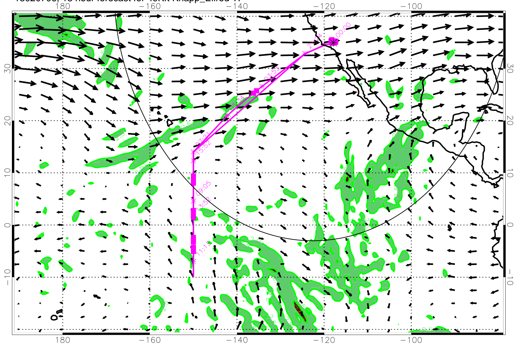
13020706, 18 hour forecast for 49Kft Knapp_Ellrod T1
