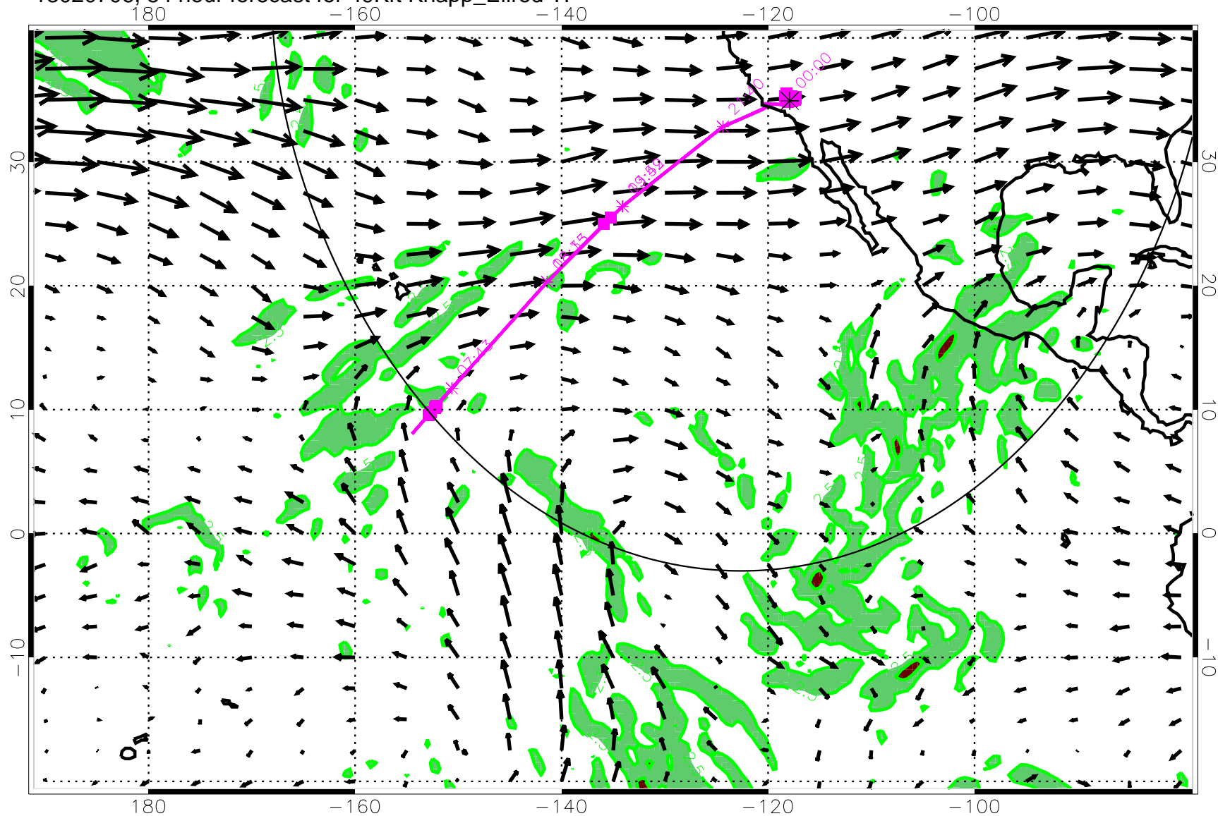
13020706, 54 hour forecast for 49Kft Knapp_Ellrod TI
