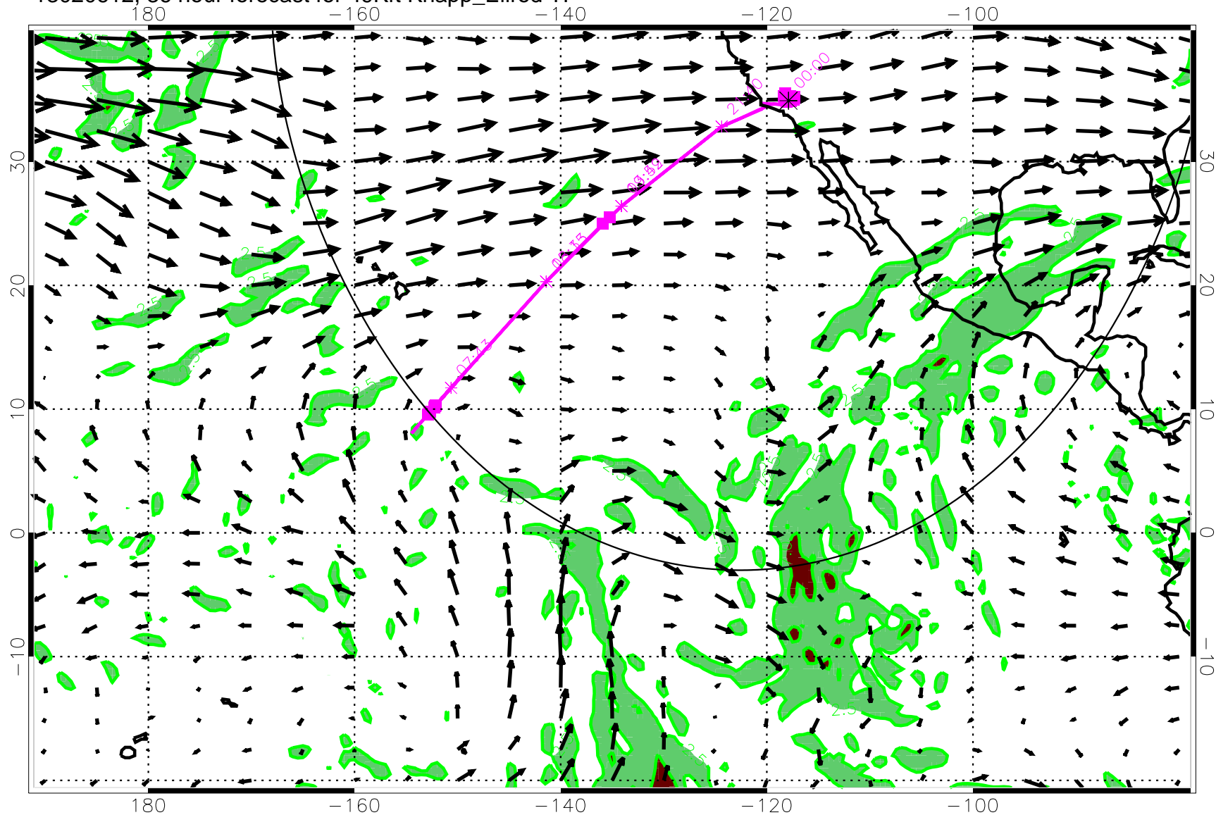
13020612, 36 hour forecast for 49Kft Knapp_Ellrod TI
