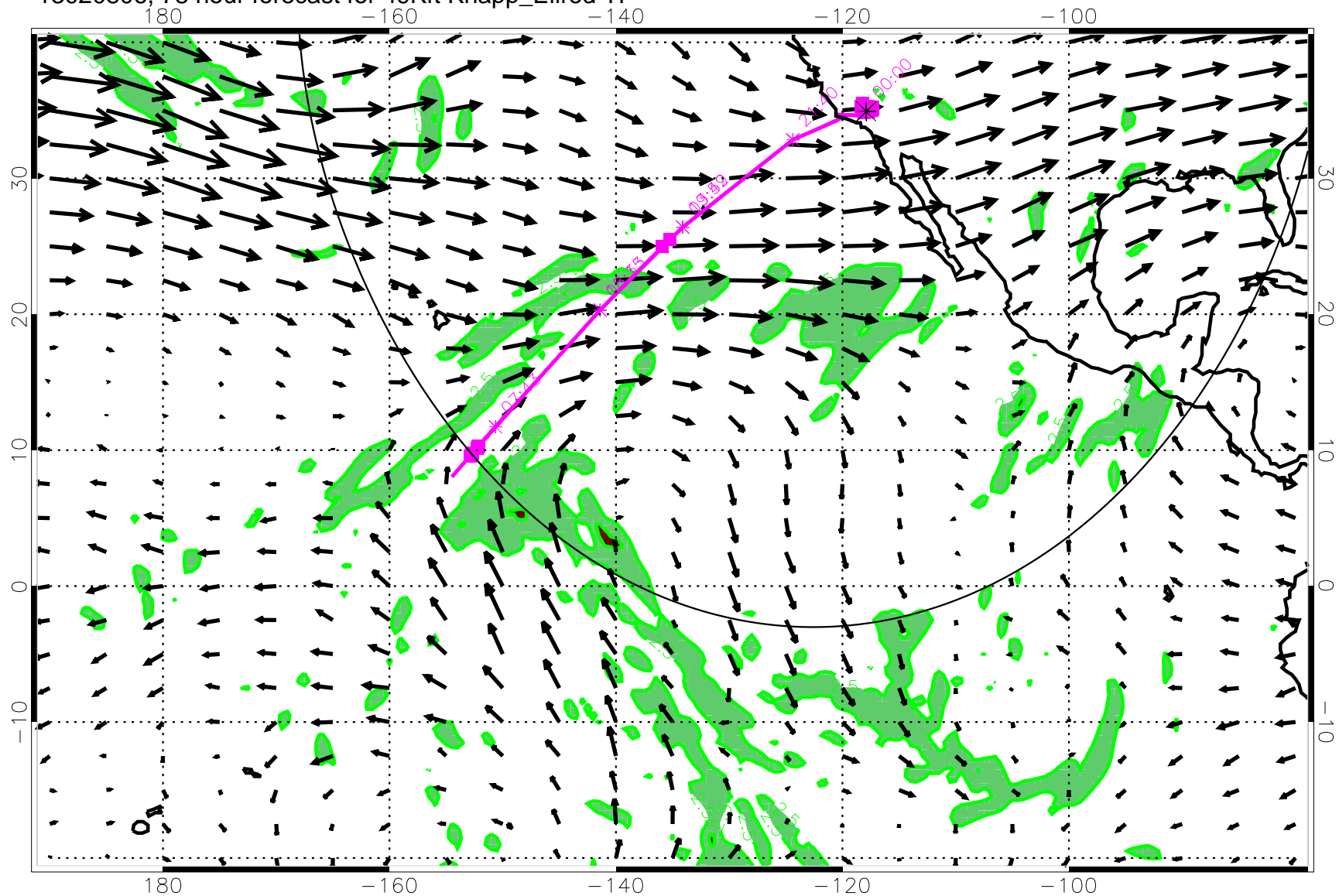
13020806, 78 hour forecast for 49Kft Knapp_Ellrod TI
