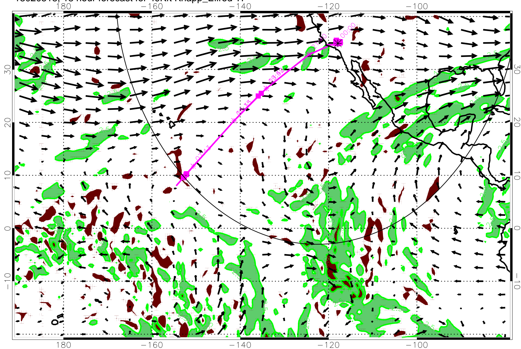
13020518, 18 hour forecast for 49Kft Knapp_Ellrod TI
