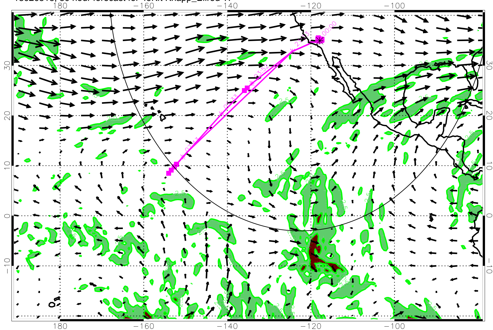
13020518, 30 hour forecast for 49Kft Knapp_Ellrod TI
