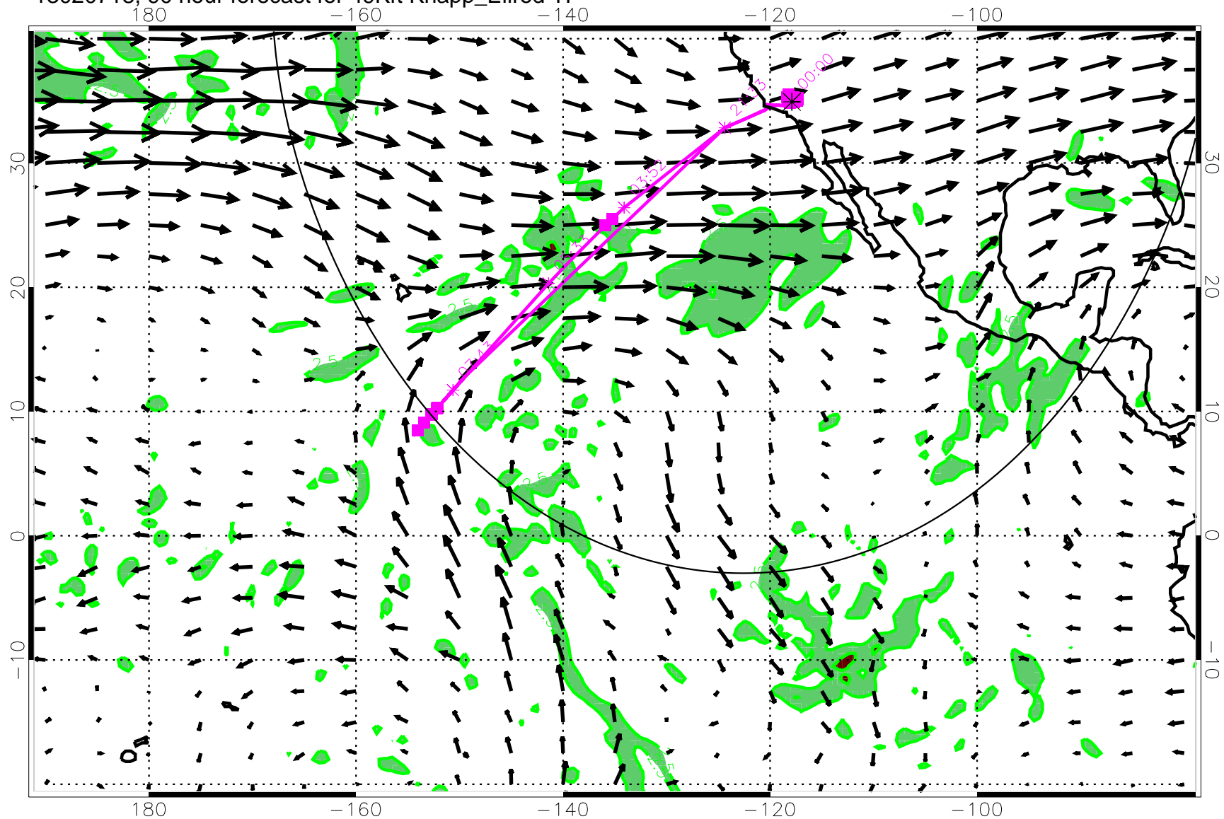
13020718, 90 hour forecast for 49Kft Knapp_Ellrod TI
