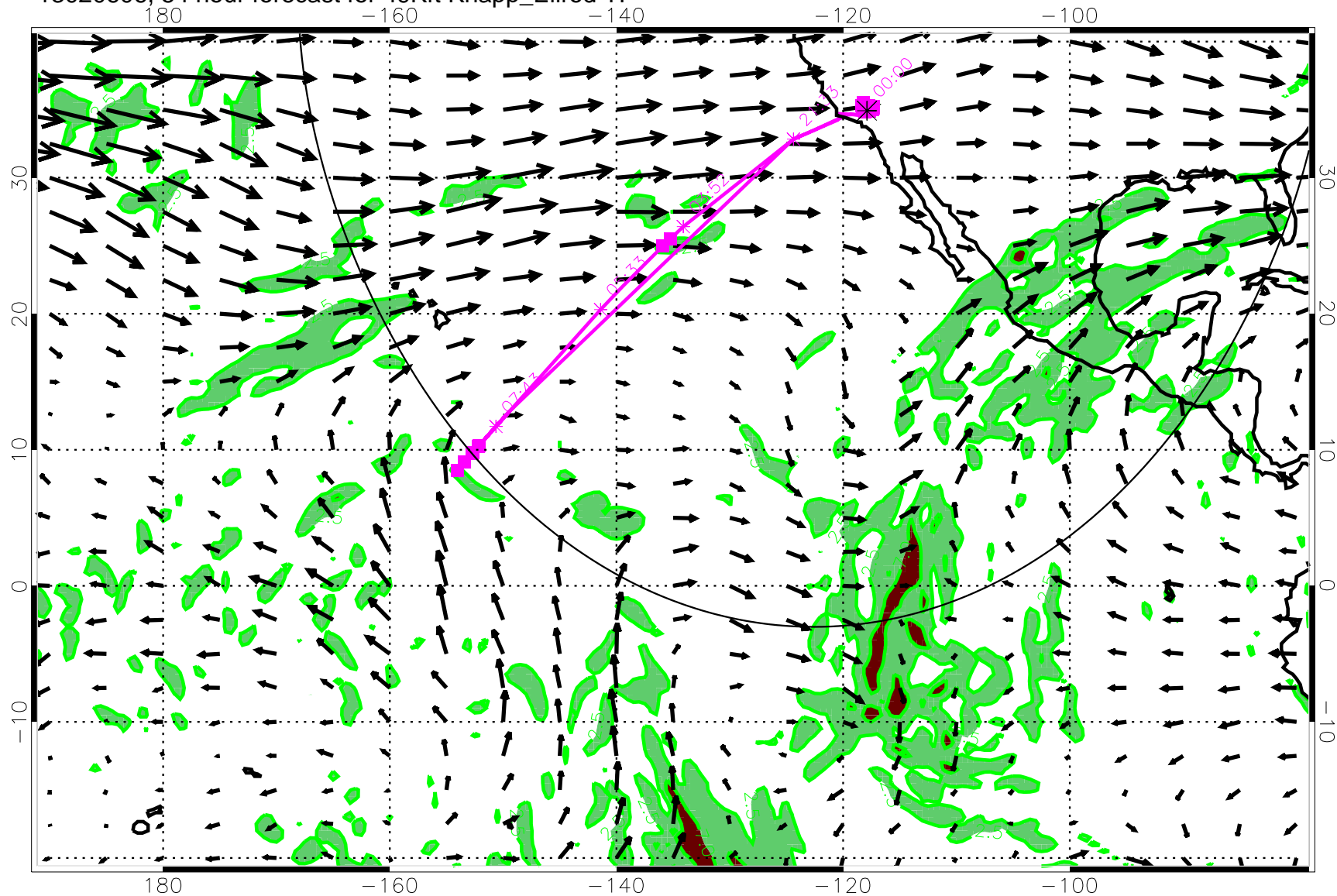
13020606, 54 hour forecast for 49Kft Knapp_Ellrod TI
