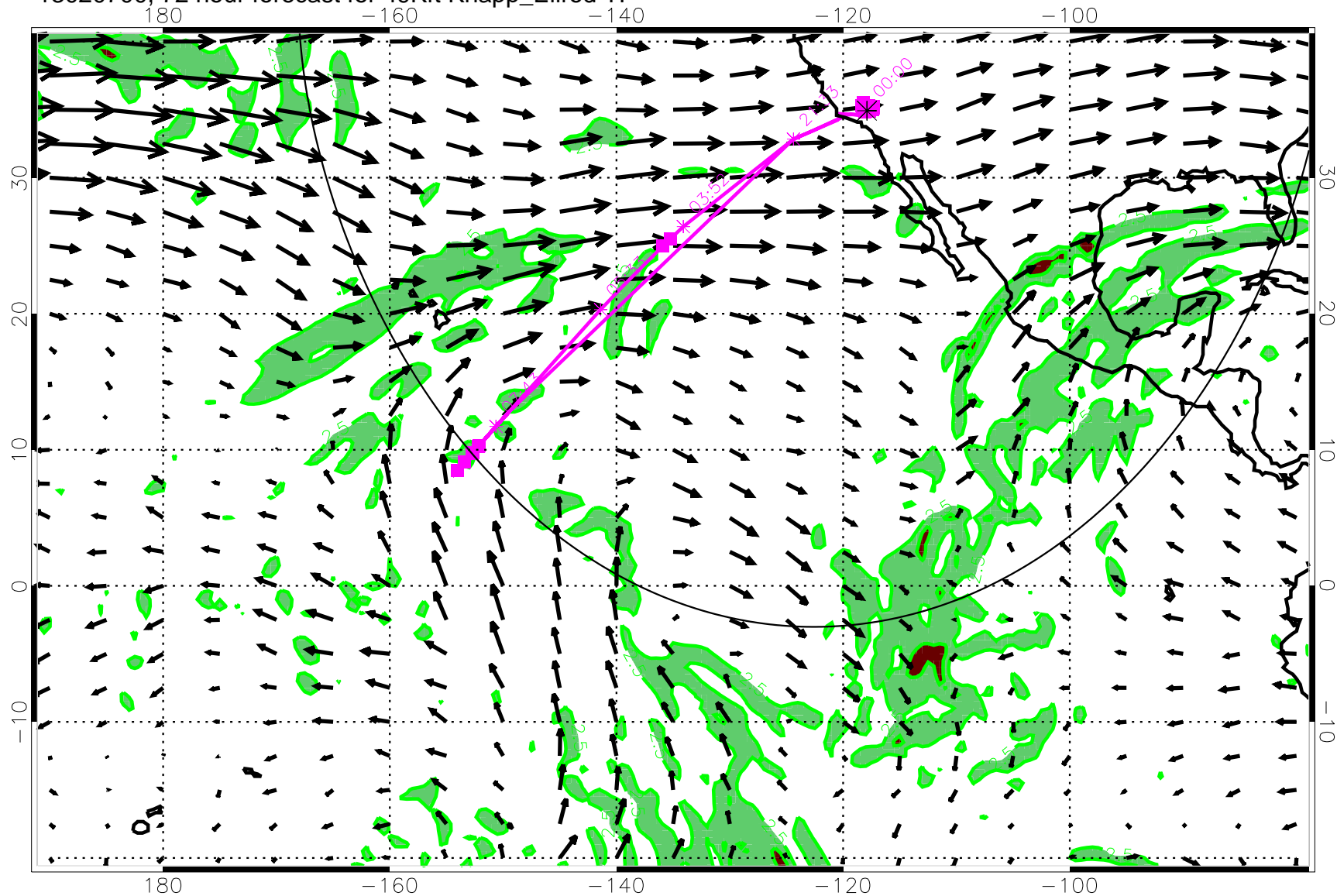
13020700, 72 hour forecast for 49Kft Knapp_Ellrod TI
