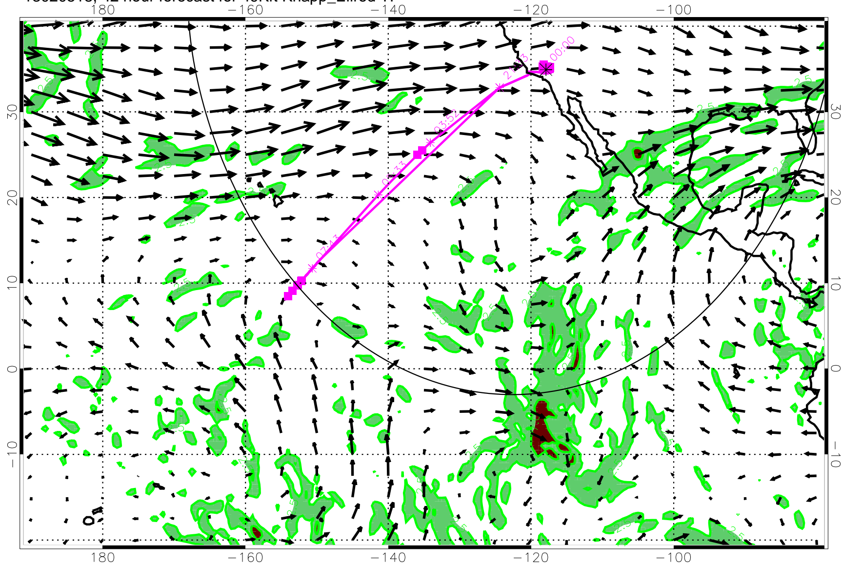
13020518, 42 hour forecast for 49Kft Knapp_Ellrod TI
