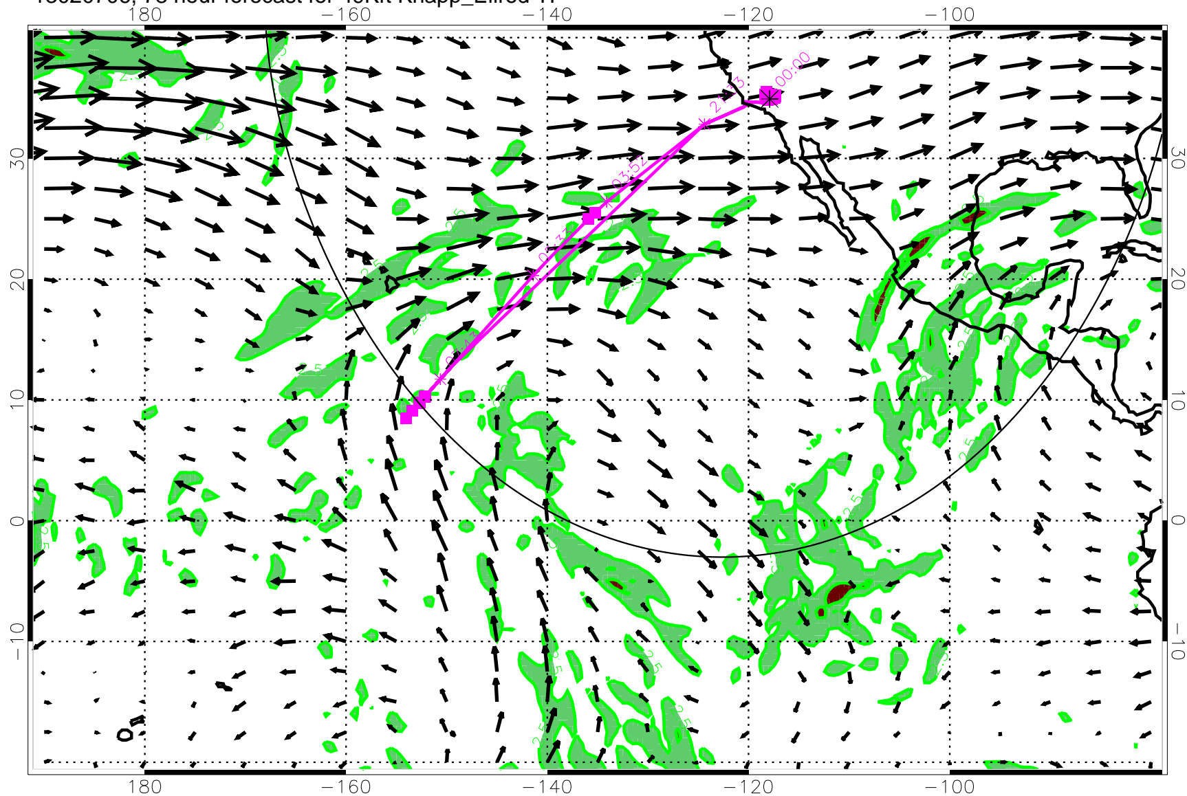
13020706, 78 hour forecast for 49Kft Knapp_Ellrod TI
