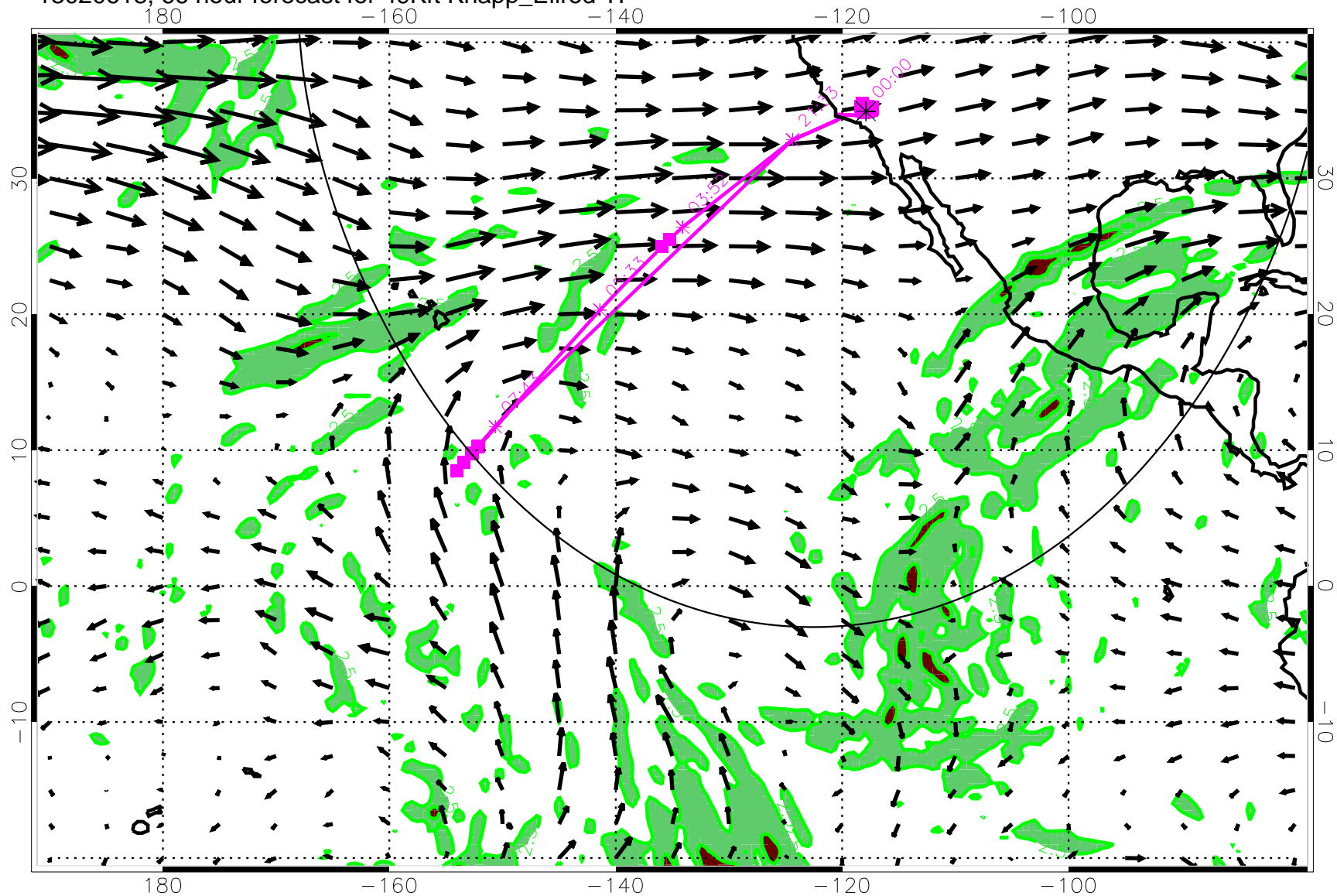
13020618, 66 hour forecast for 49Kft Knapp_Ellrod TI
