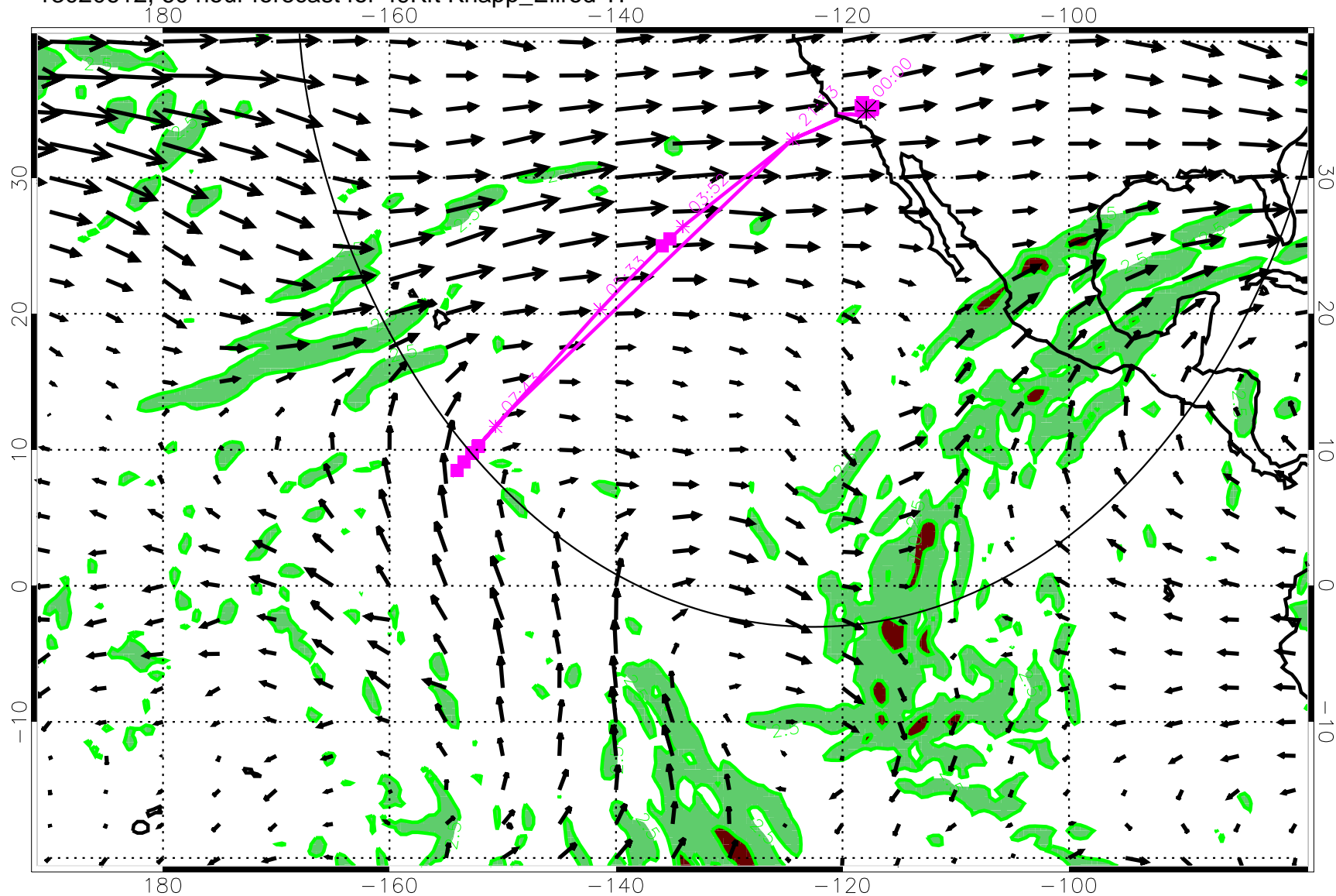
13020612, 60 hour forecast for 49Kft Knapp_Ellrod TI
